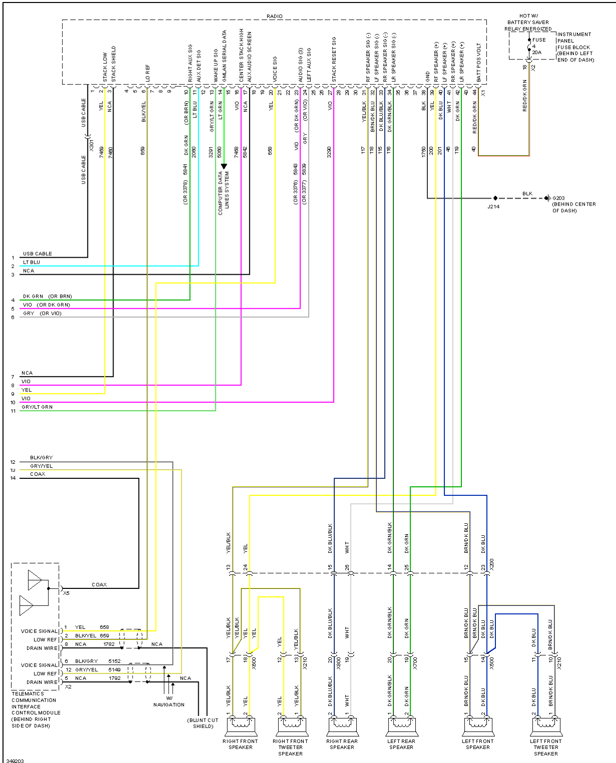
Fig. 45: Navigation Circuit, W/O Amplifier (3 of 3)
