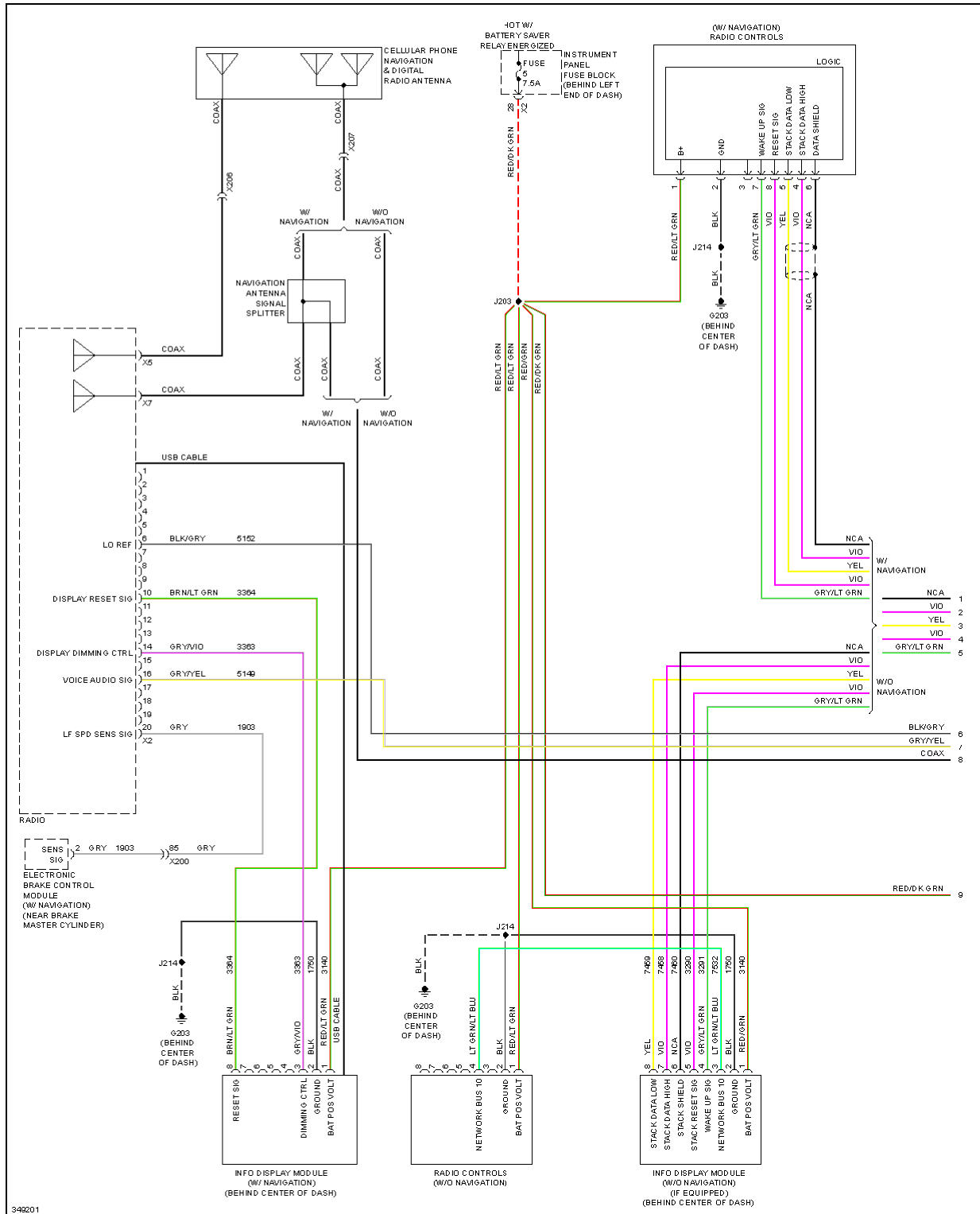
Fig. 63: Radio Circuit, W/O Amplifier (1 of 3)
