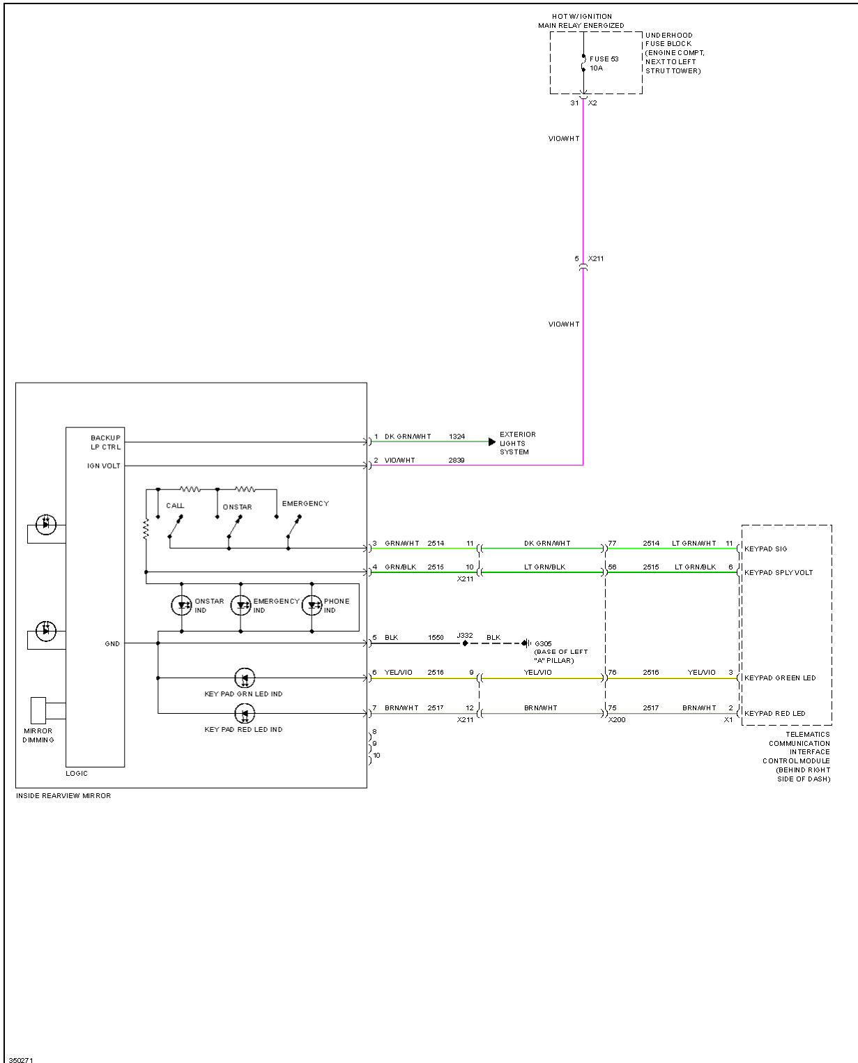
Fig. 53: Electrochromic Mirror Circuit
