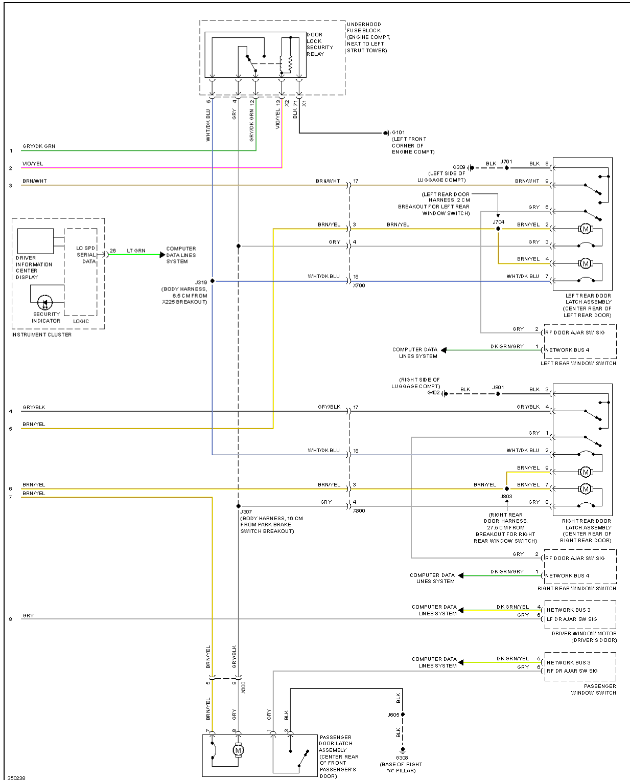
Fig. 52: Power Door Locks Circuit (2 of 2)
