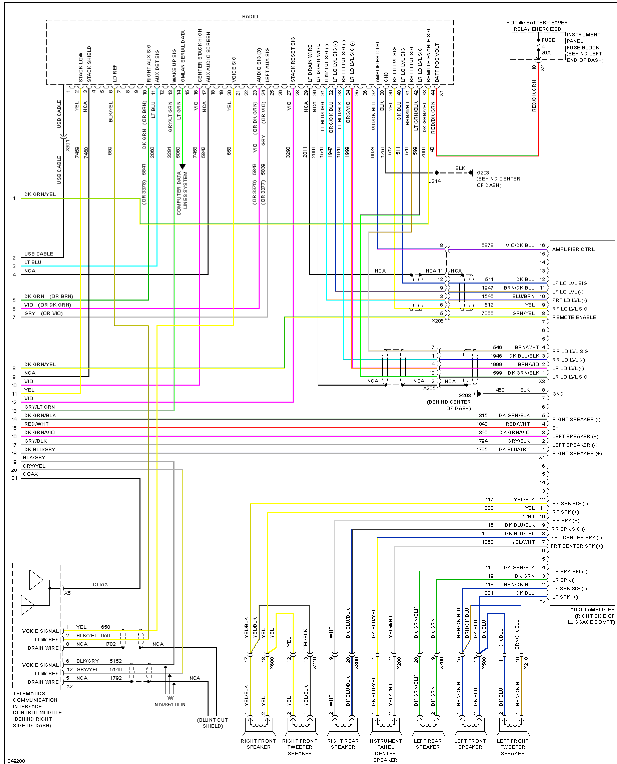
Fig. 62: Radio Circuit, W/ Amplifier (3 of 3)
