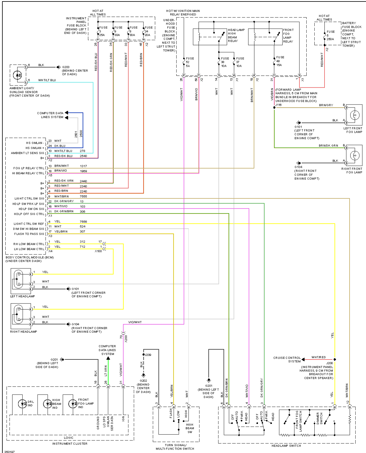
Fig. 34: Headlights Circuit
