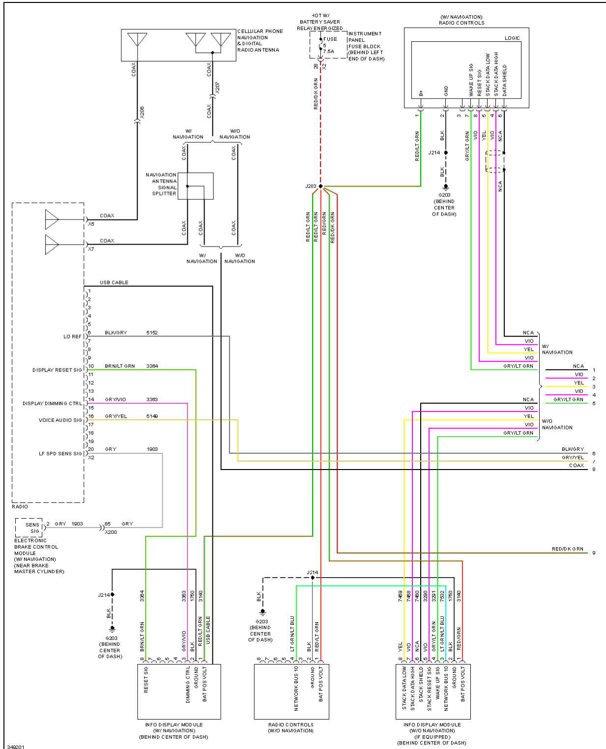
Fig. 43: Navigation Circuit, W/O Amplifier (1 of 3)
