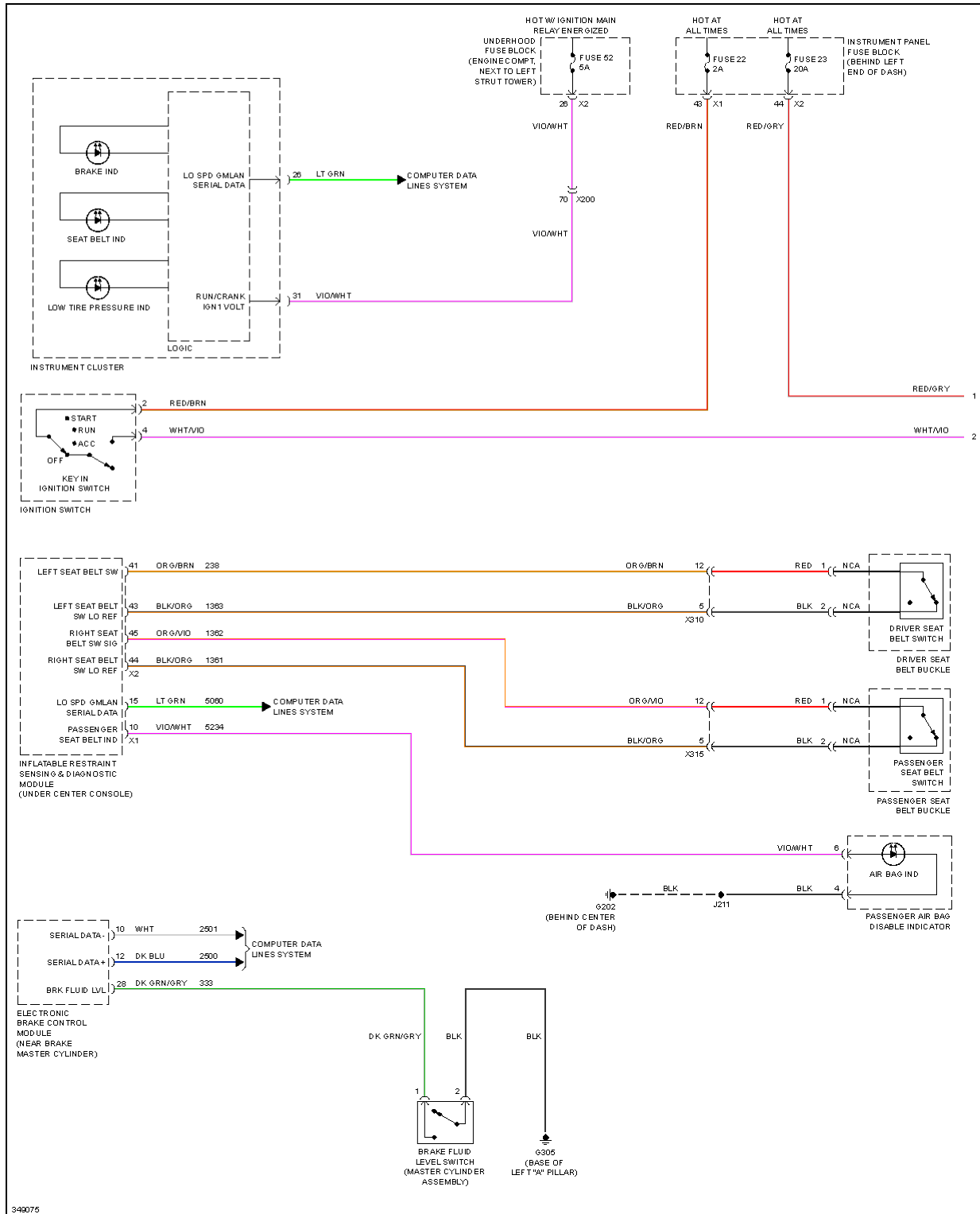
Fig. 75: Warning Systems Circuit (1 of 2)
