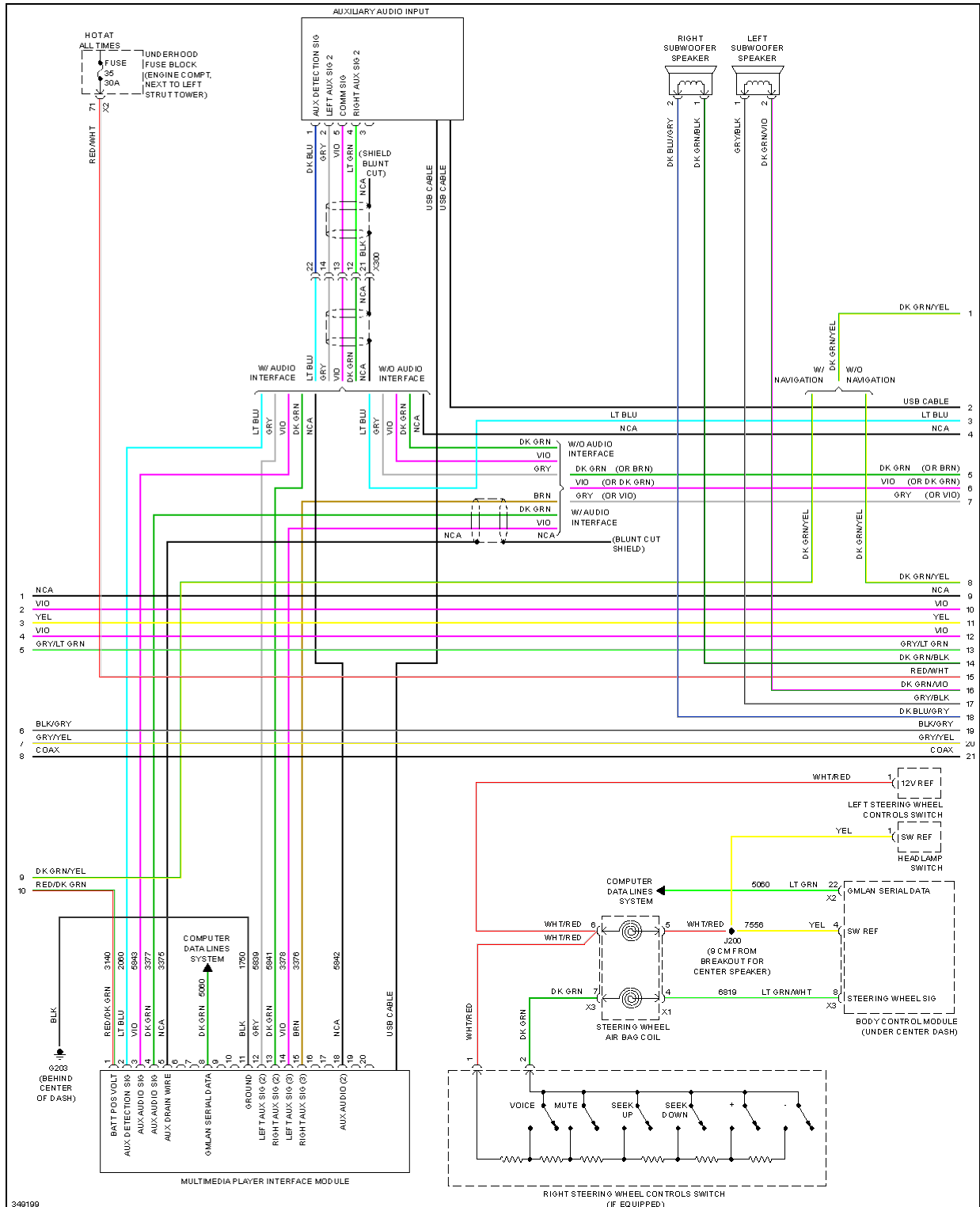
Fig. 41: Navigation Circuit, W/ Amplifier (2 of 3)
