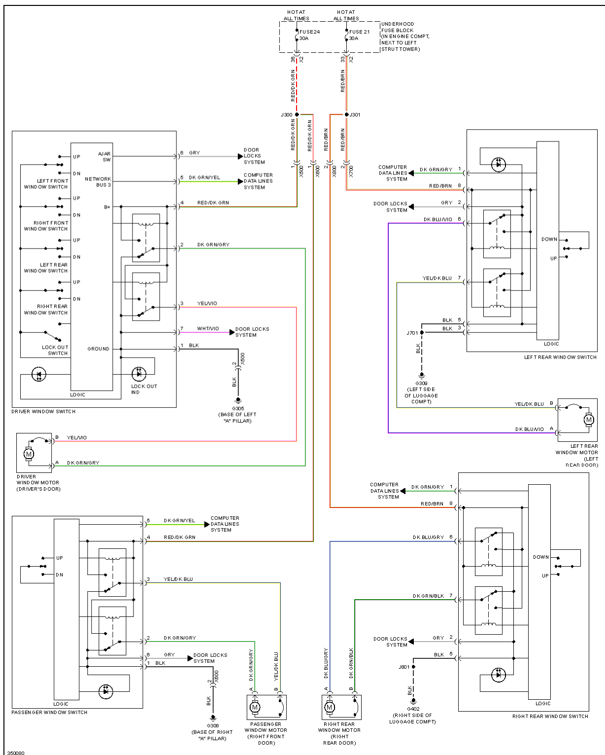
Fig. 59: Power Windows Circuit, W/O Express Up/Down
