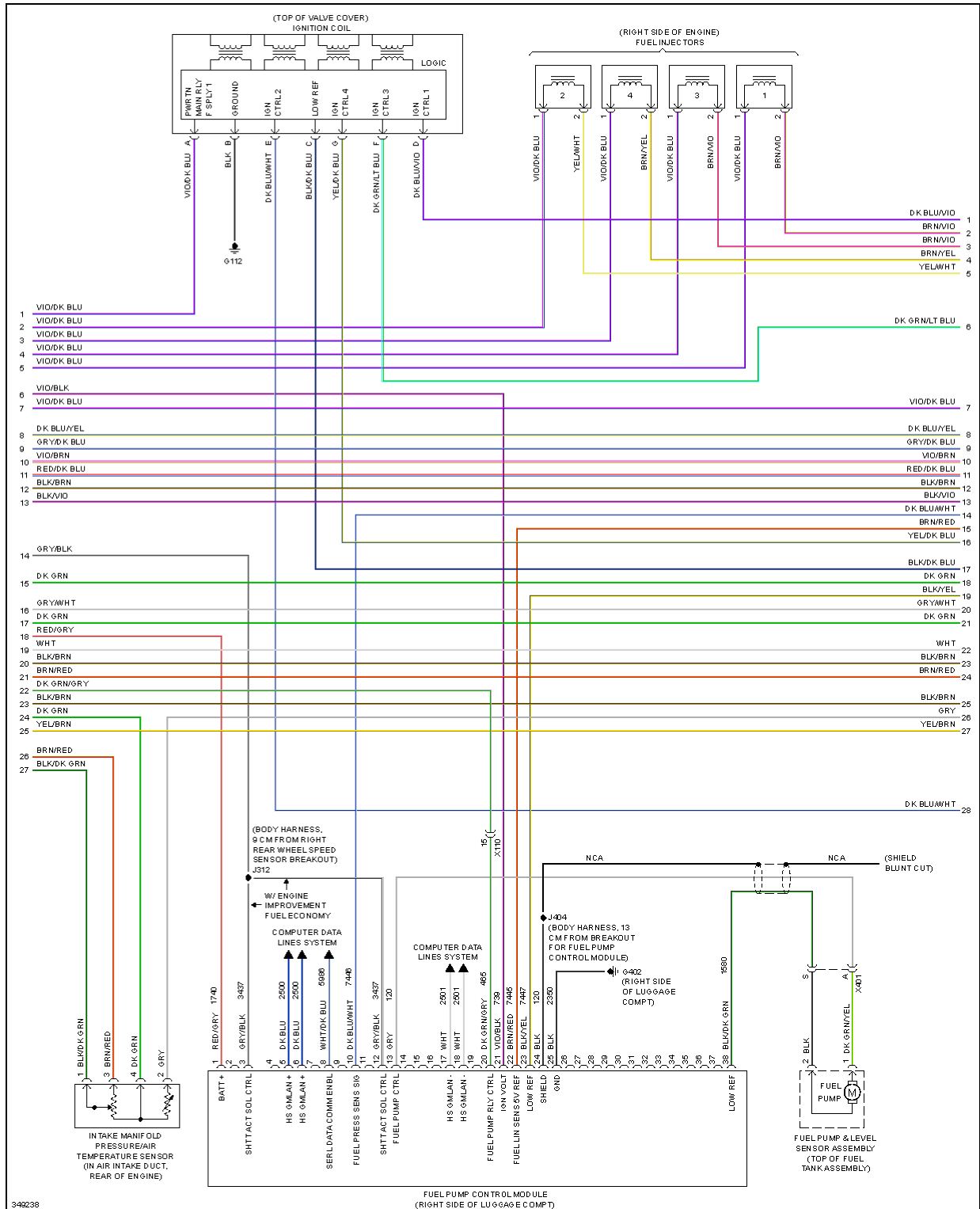
Fig. 21: 1.4L VIN 9, Engine Performance Circuit (4 of 6)
