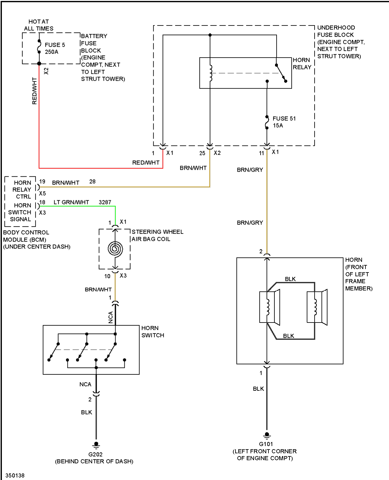
Fig. 35: Horn Circuit
