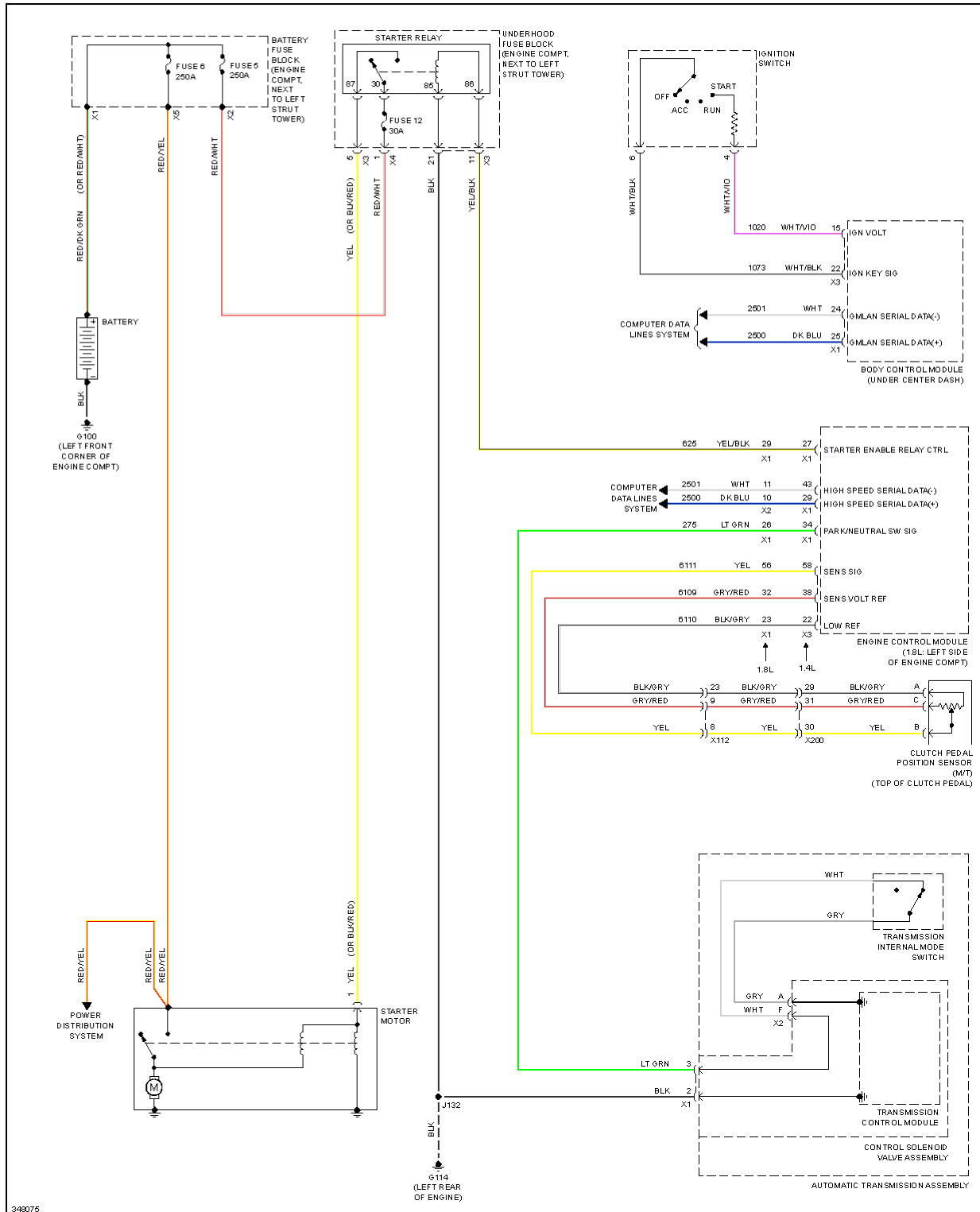
Fig. 70: Starting Circuit
