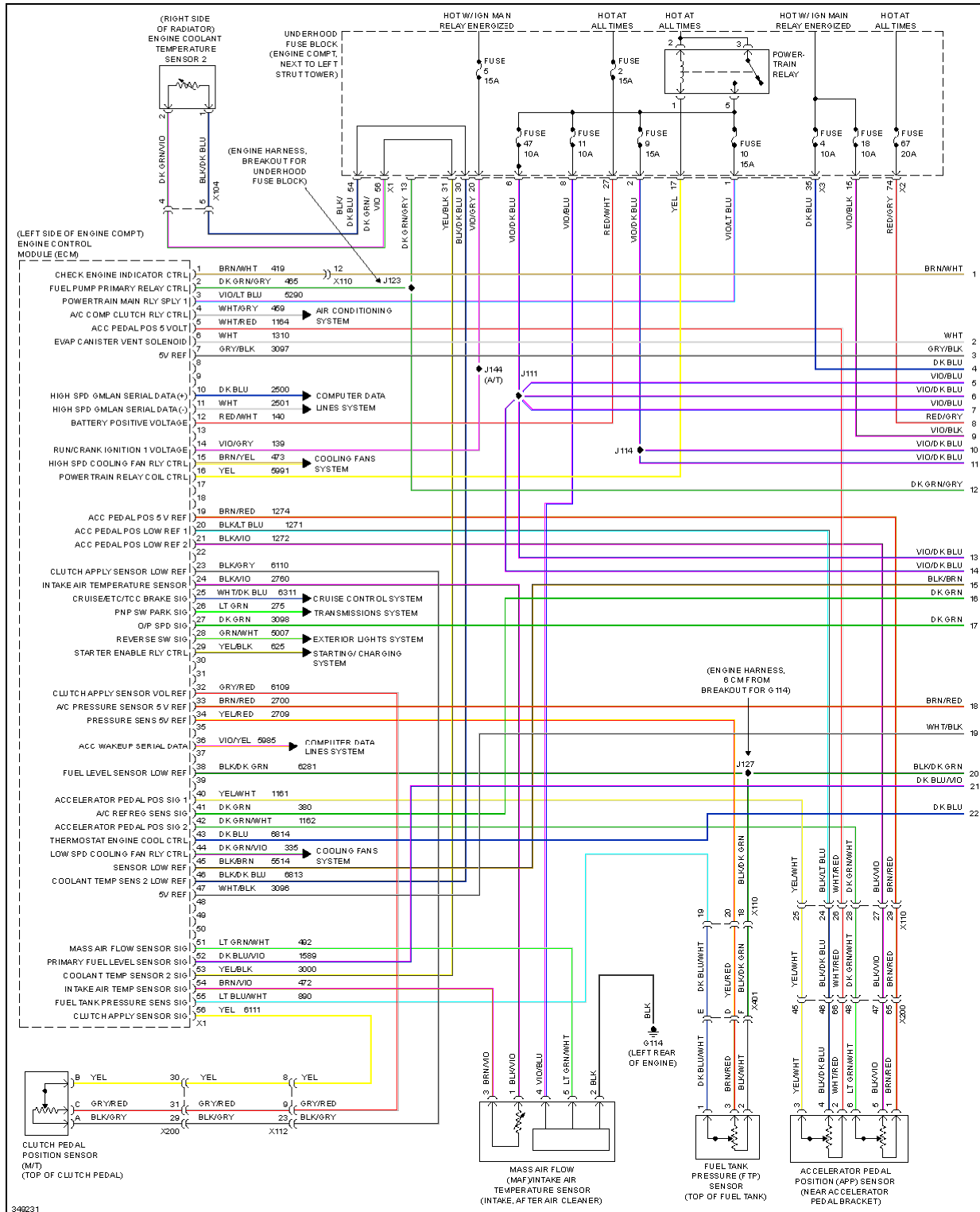
Fig. 24: 1.8L VIN H, Engine Performance Circuit (1 of 4)
