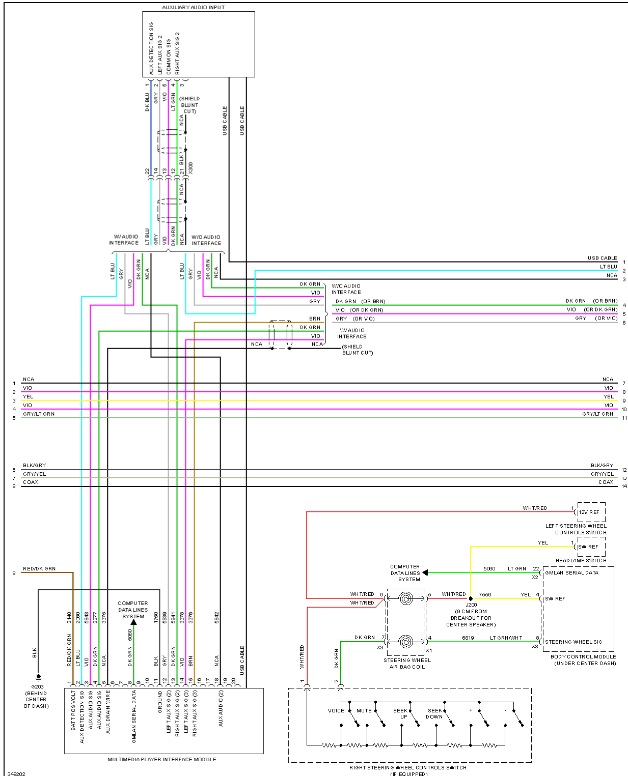
Fig. 64: Radio Circuit, W/O Amplifier (2 of 3)
