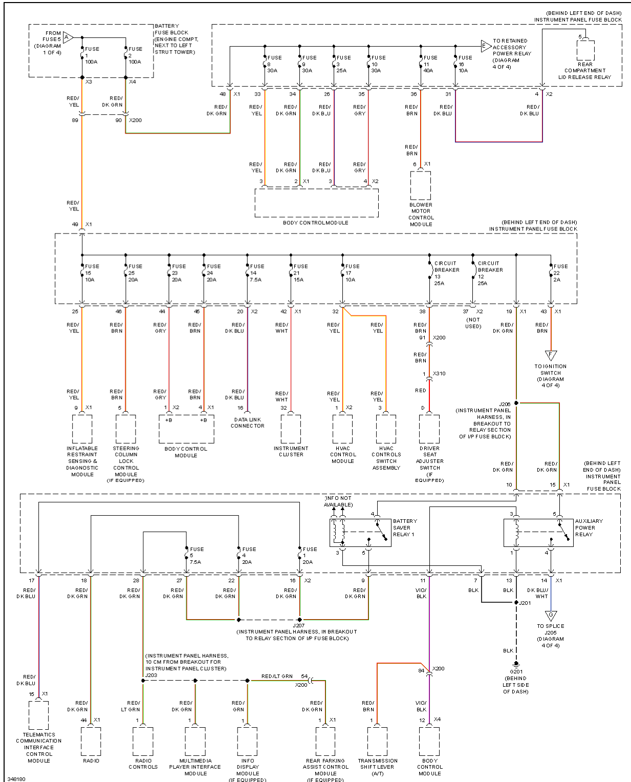
Fig. 49: Power Distribution Circuit (3 of 4)
