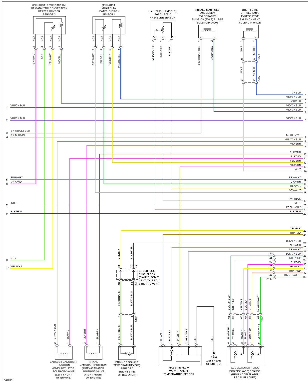
Fig. 19: 1.4L VIN 9, Engine Performance Circuit (2 of 6)
