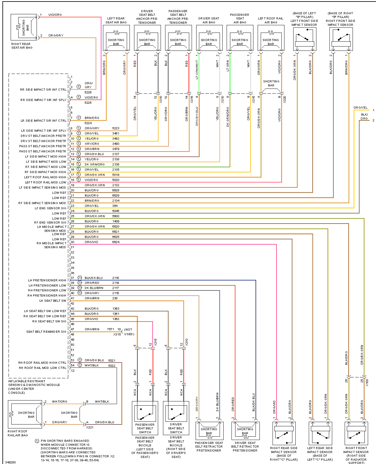
Fig. 71: Supplemental Restraints Circuit (1 of 2)
