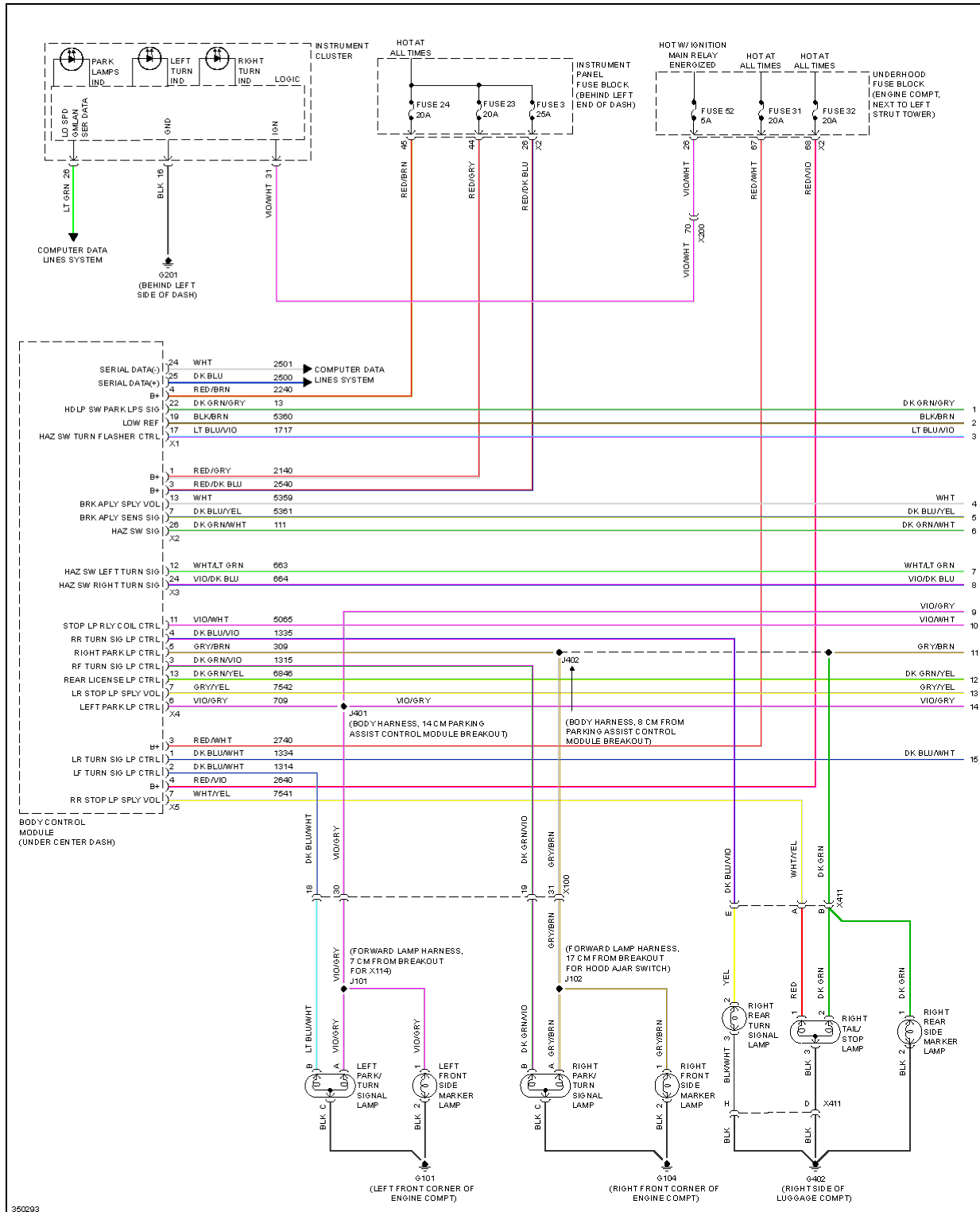
Fig. 29: Exterior Lamps Circuit (1 of 2)
