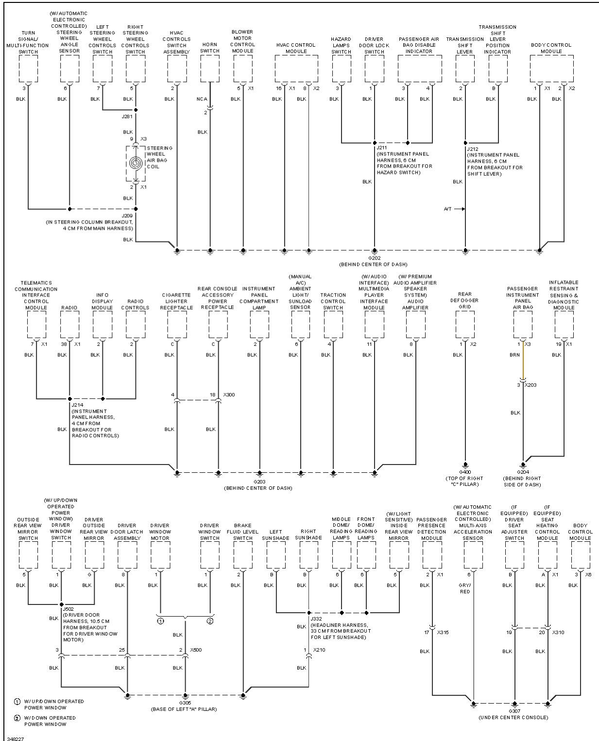
Fig. 32: Ground Distribution Circuit (2 of 3)
