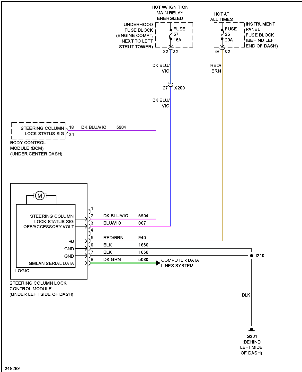
Fig. 68: Steering Lock Circuit
