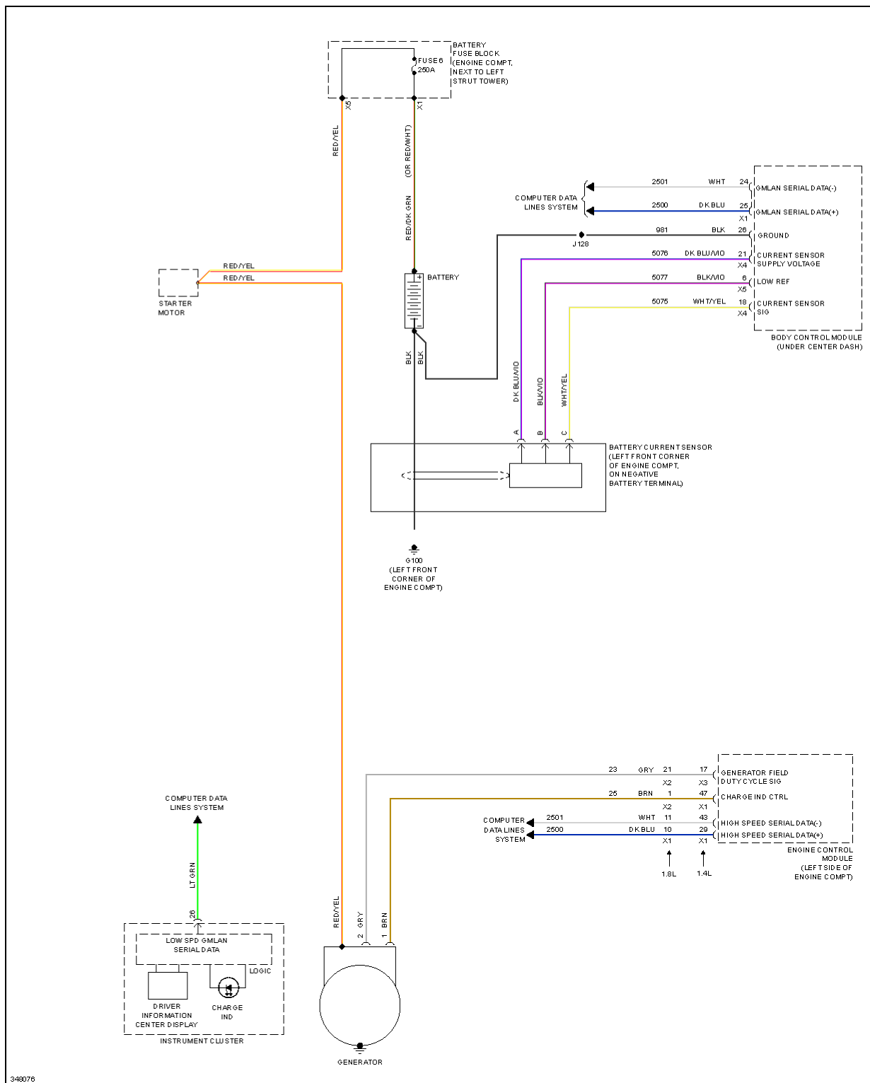
Fig. 69: Charging Circuit
