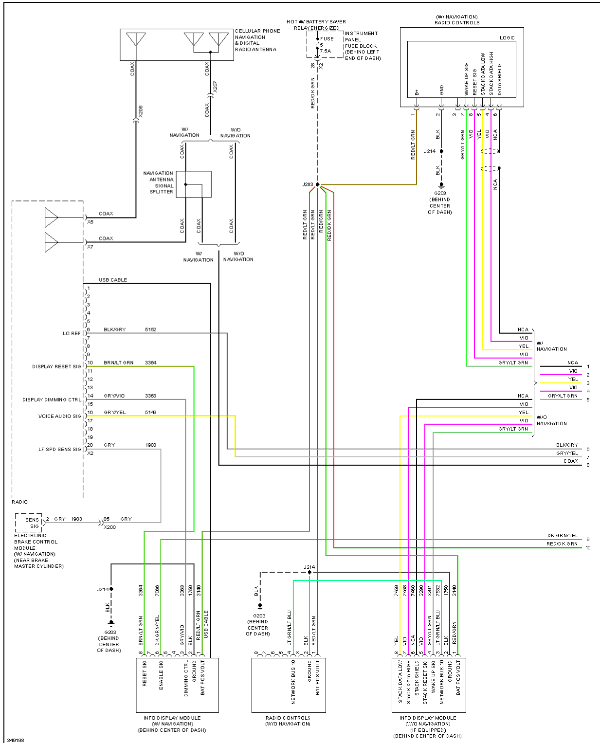
Fig. 40: Navigation Circuit, W/ Amplifier (1 of 3)
