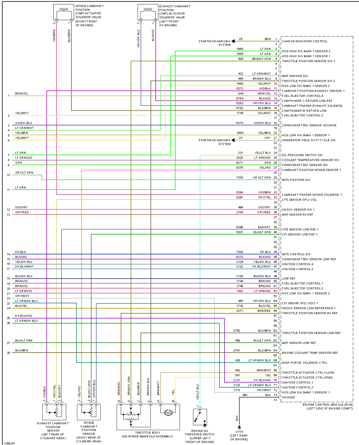
Fig. 27: 1.8L VIN H, Engine Performance Circuit (4 of 4)
