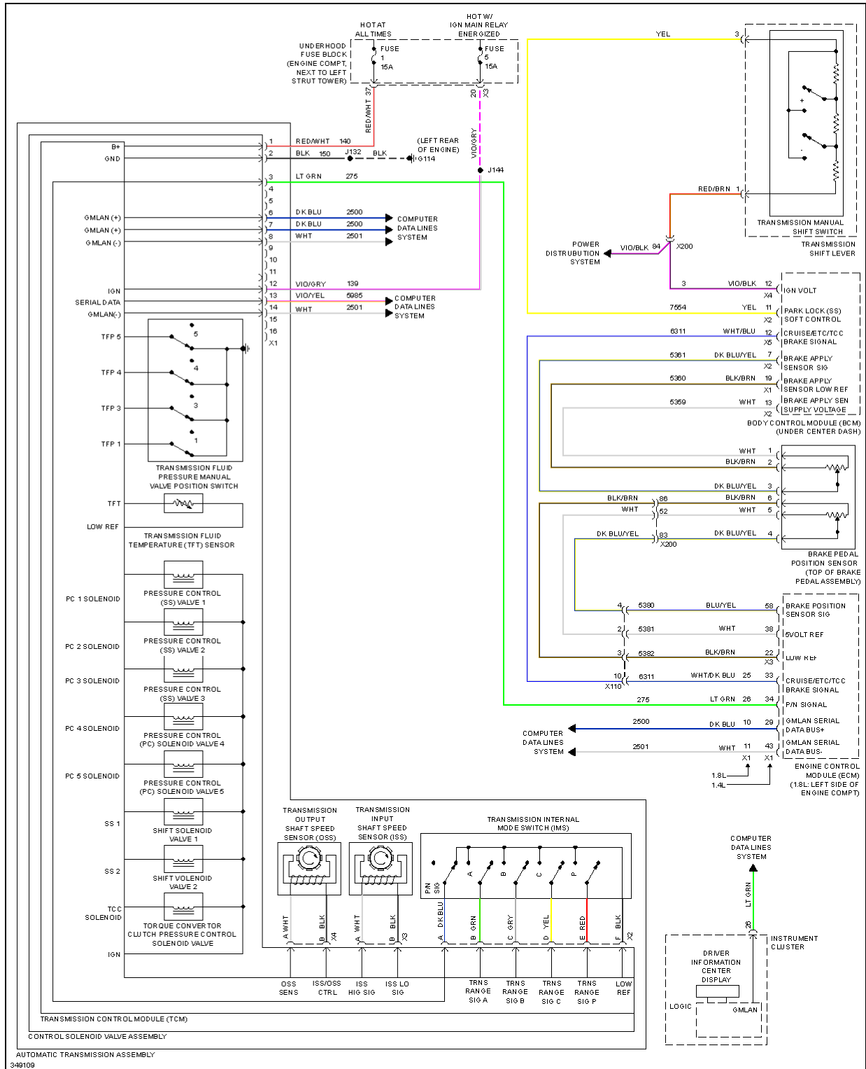
Fig. 73: Transmission Circuit
