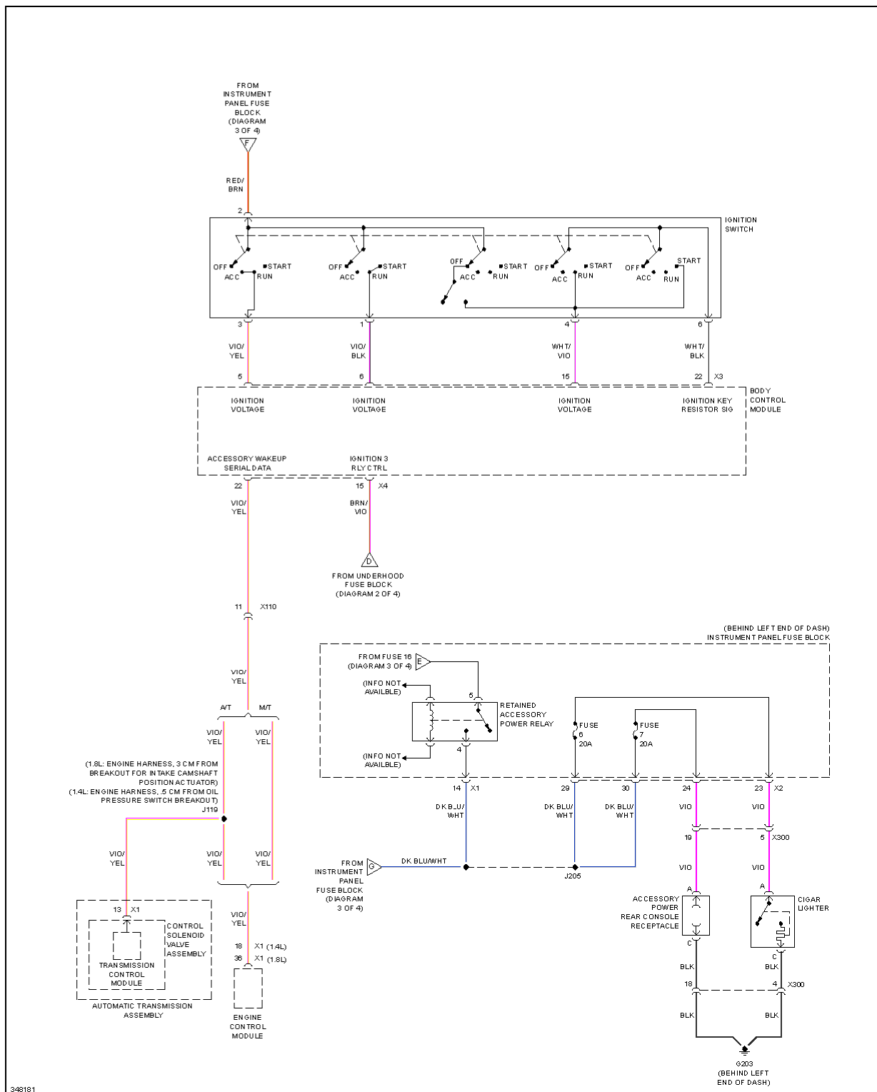
Fig. 50: Power Distribution Circuit (4 of 4)
