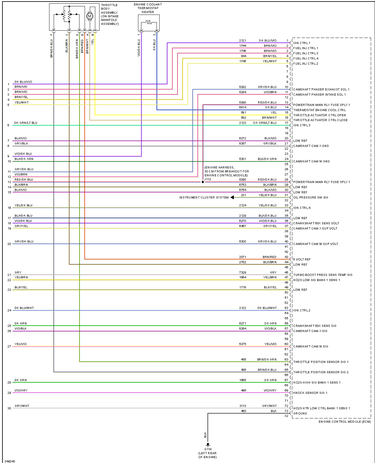
Fig. 23: 1.4L VIN 9, Engine Performance Circuit (6 of 6)
