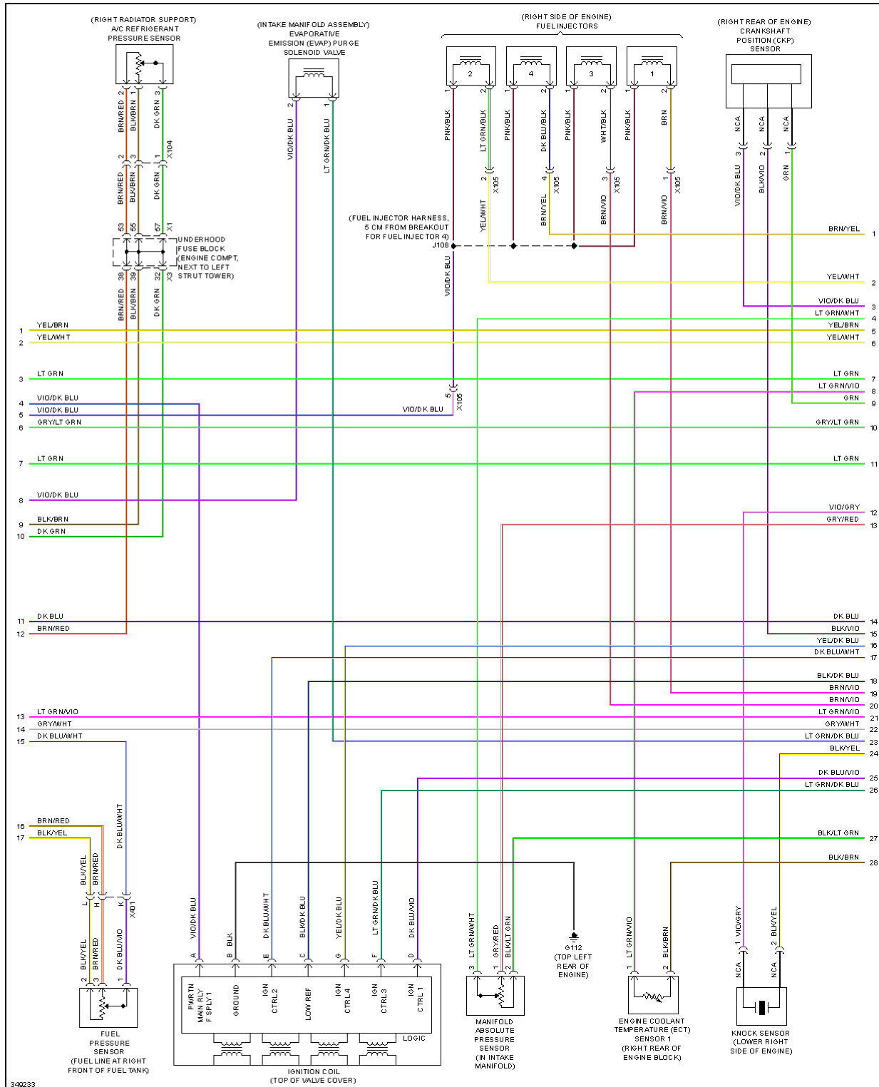
Fig. 26: 1.8L VIN H, Engine Performance Circuit (3 of 4)
