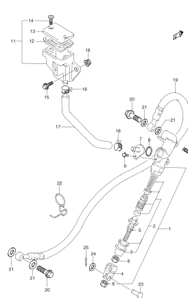
GS500KS P02_055A REAR MASTER CYLINDER
