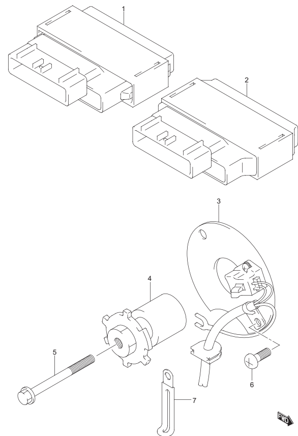
GS500K6 P02_022 SIGNAL GENERATOR
