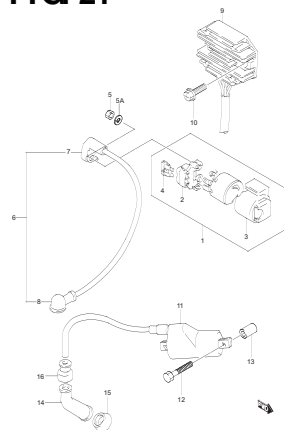
GS500K6 P02_024 ELECTRICAL
