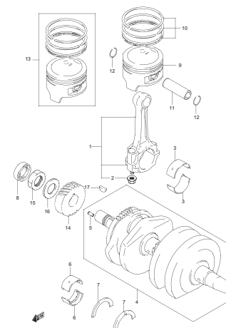
GS500K6 P02_008 CRANKSHAFT
