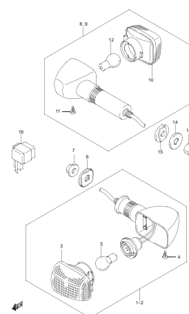
GS500K6 P02_029B TURN SIGNAL LAMP
