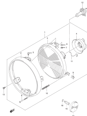
GS500K6 P02_027A HEADLAMP
