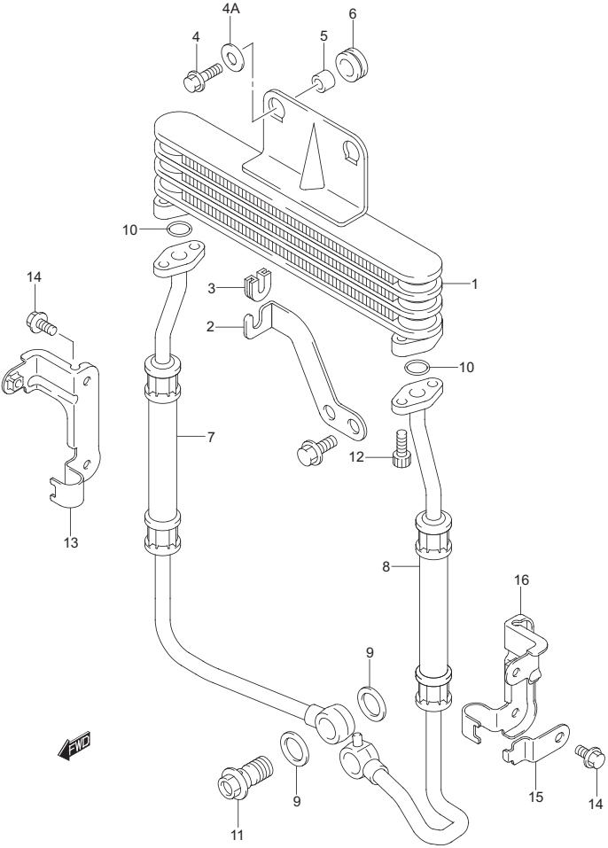
GS500K6 P02_015B OIL COOLER
