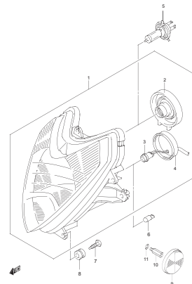
GS500K6 P02_027B HEADLAMP
