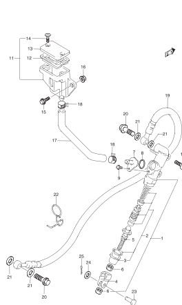
GS500KS P02_055 REAR MASTER CYLINDER
