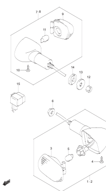
GS500K6 P02_028 TURN SIGNAL LAMP
