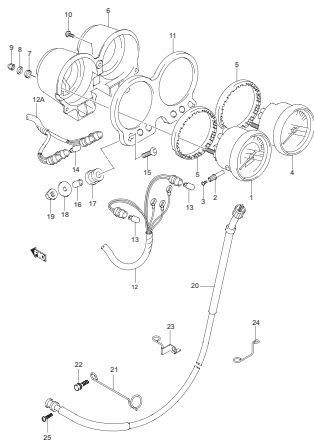
GS500K6 P02_025B SPEEDOMETER
