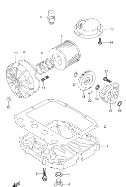
GS500K6 P02_007 OIL FILTER/OIL PUMP
