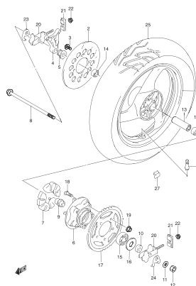
GS500KS P02_053 REAR WHEEL
