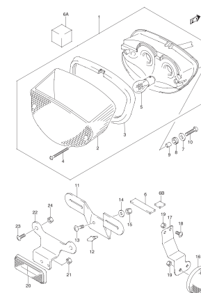
GS500K6 P02_030 REAR COMBINATION LAMP
