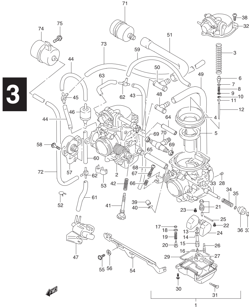
GS500K6 P02_014 CARBURETOR
