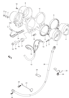
GS500K6 P02_025 SPEEDOMETER
