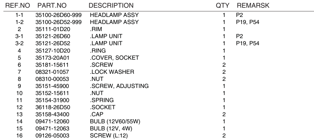
FIG.26 (E-10) HEADLAMP (GS500K3/UK3/HK3/HUK3 P2, P19, P54)
