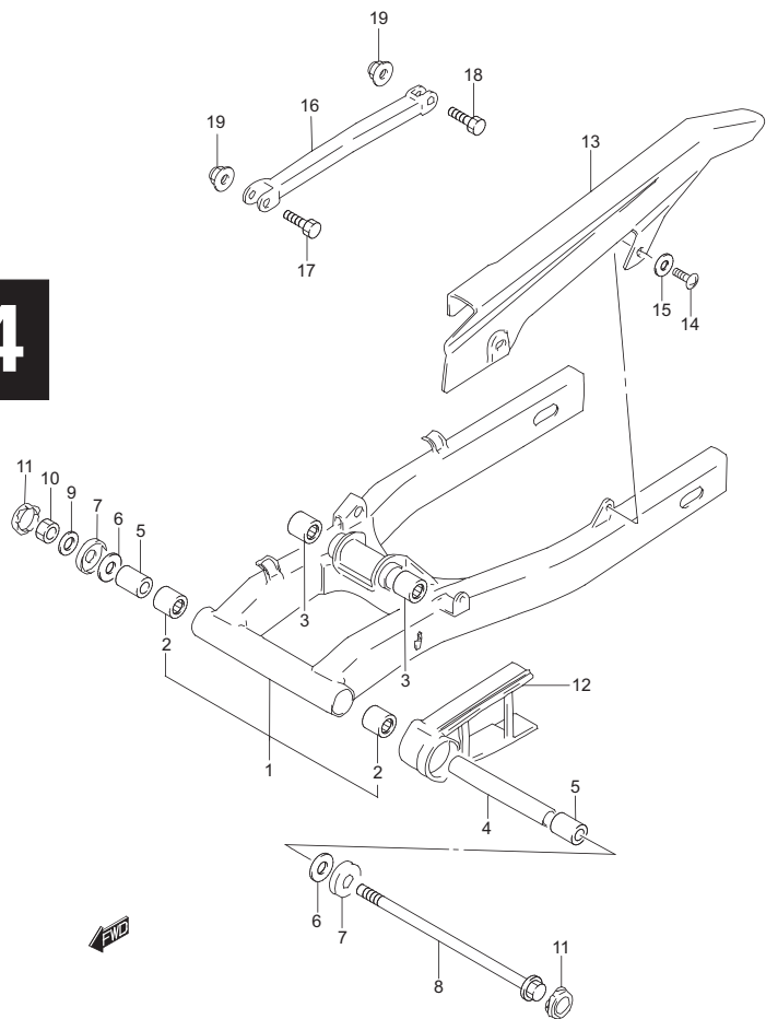
GS500K6 P02_051A REAR SWINGING ARM
