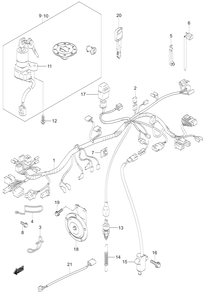
GS500K6 P02_031 WIRING HARNESS
