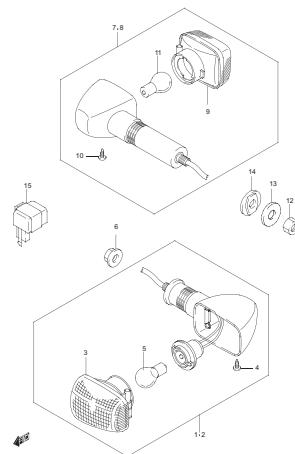
GS500K6 P02_029A TURN SIGNAL LAMP
