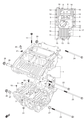
GS500K6 P02_005 CRANKCASE
