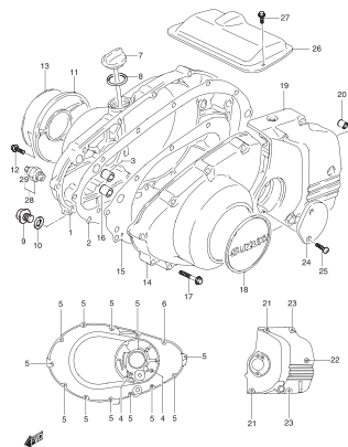
GS500K6 P02_006 CRANKCASE COVER
