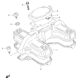
GS500K6 P02_002 CYLINDER HEAD COVER
