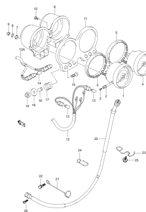
GS500K6 P02_025A SPEEDOMETER
