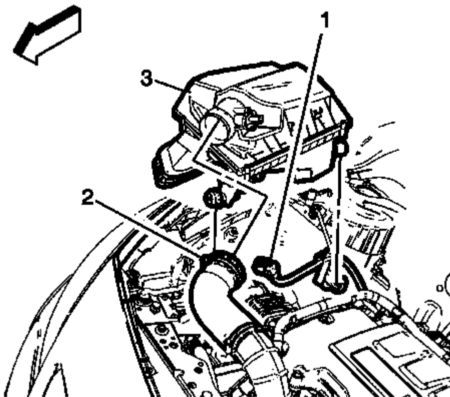
Fig. 205: Air Cleaner Assembly, Electrical Connector And Clamp Courtesy of GENERAL MOTORS COMPANY
