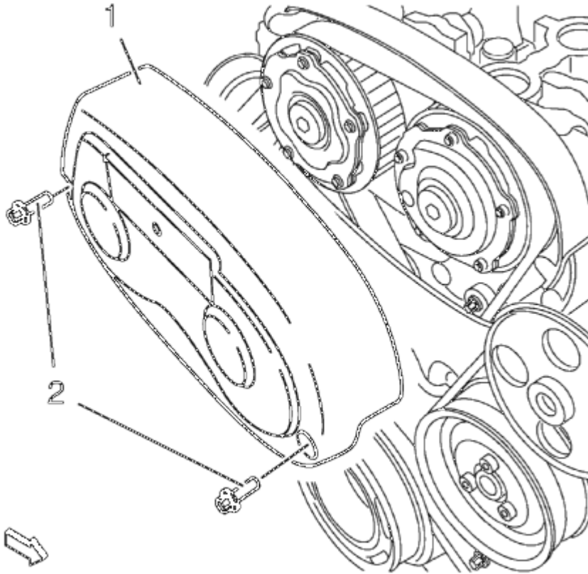
Fig. 257: Timing Belt Upper Front Cover Courtesy of GENERAL MOTORS COMPANY
