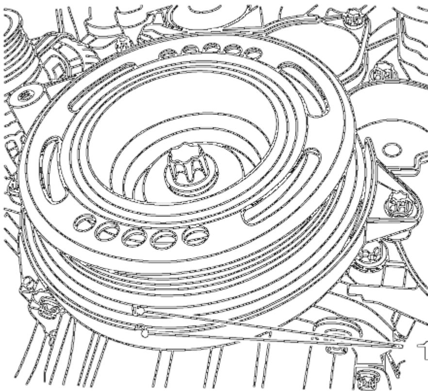
Fig. 258: Crankshaft TDC Position
