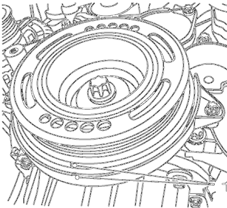
Fig. 117: Crankshaft TDC Position
