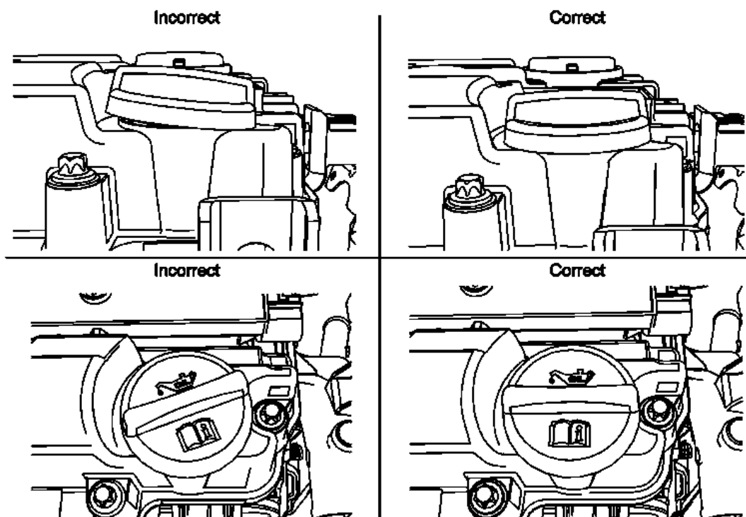
Fig. 247: Proper Oil Filler Cap Seating
