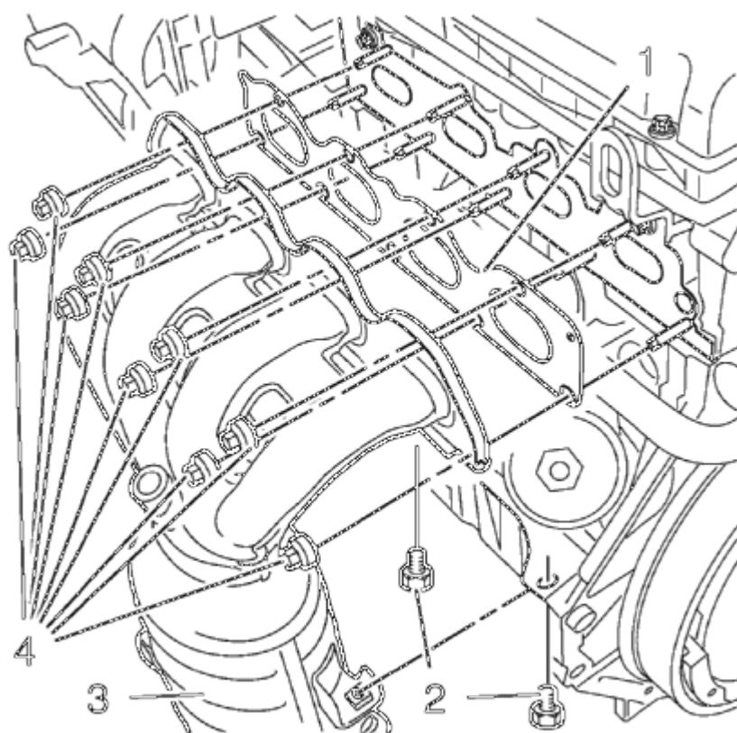
Fig. 497: Exhaust Manifold And Bolts
