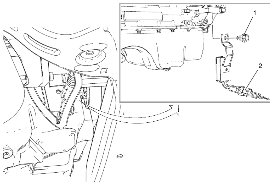
Fig. 195: Engine Oil Heater And Bolt
