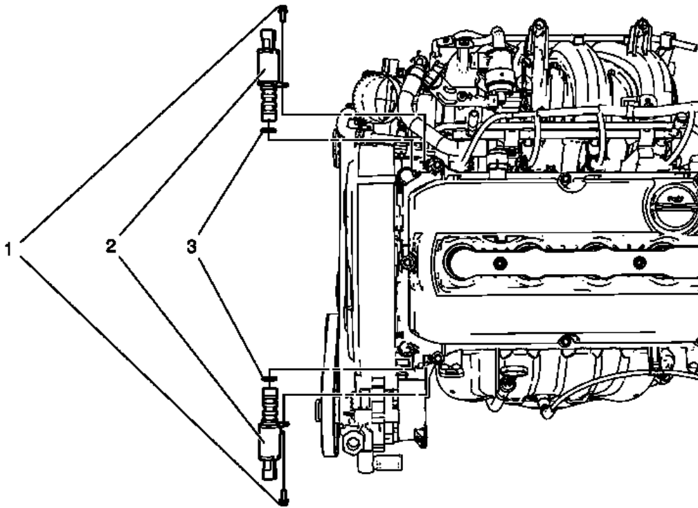
Fig. 283: Camshaft Position Actuator Solenoid Valve Courtesy of GENERAL MOTORS COMPANY
