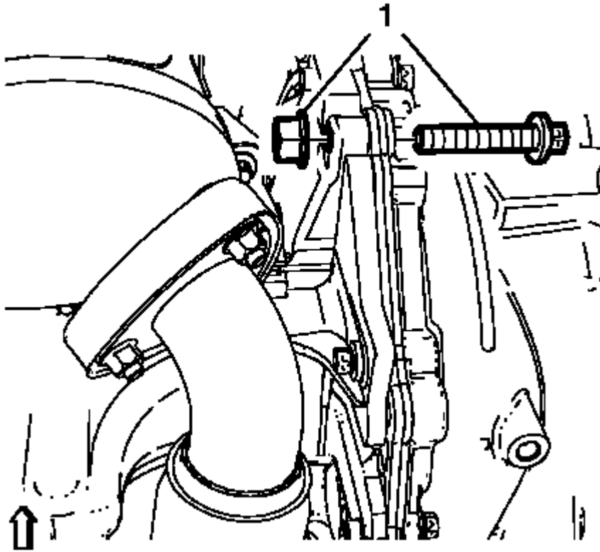
Fig. 80: Connection Bolt
