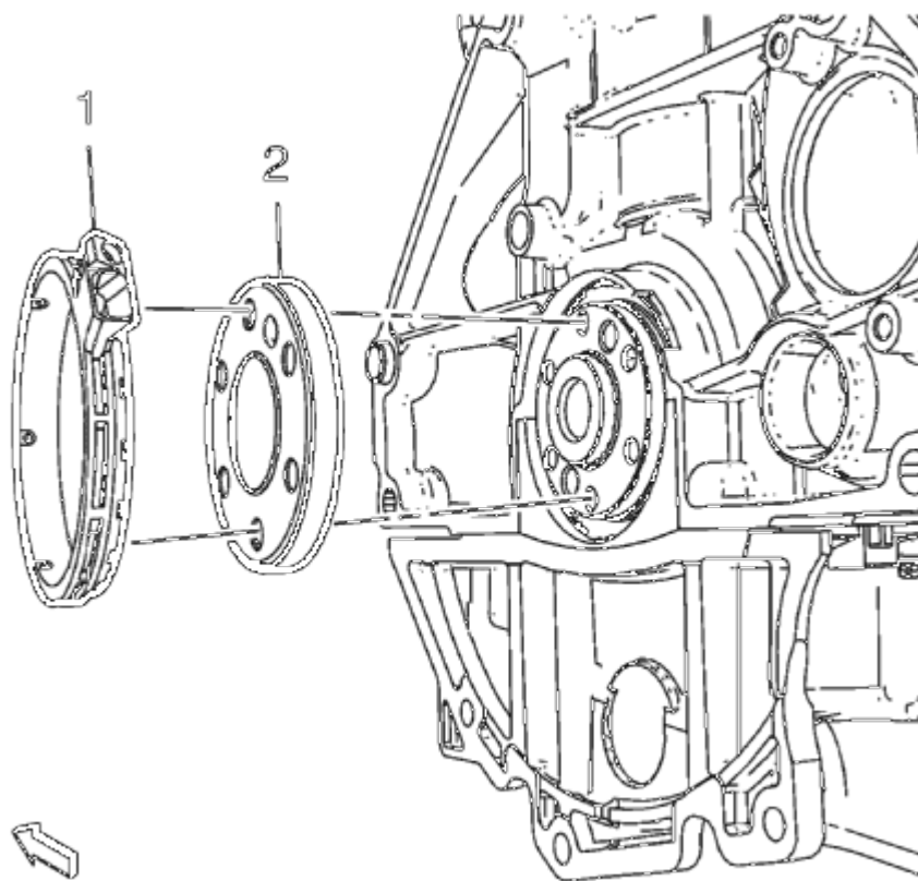
Fig. 539: Crankshaft Position Sensor Reluctor Ring And Oil Seal Housing Courtesy of GENERAL MOTORS COMPANY
