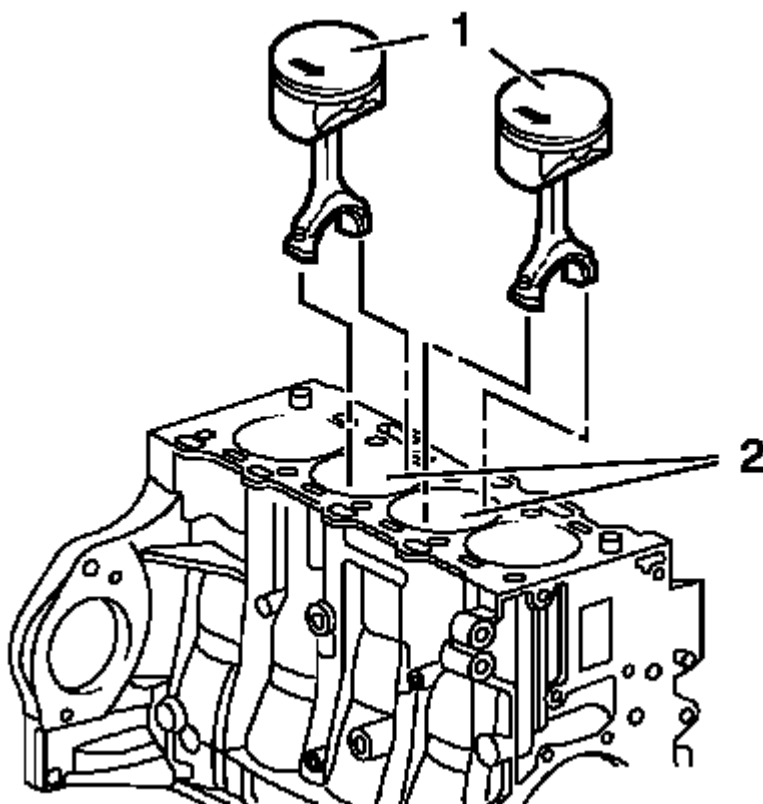
Fig. 402: Pistons 2, 3 And Cylinder Bore
