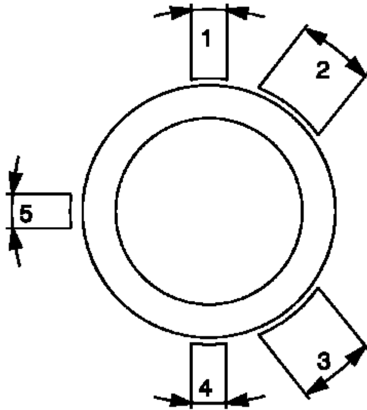
Fig. 459: Piston Ring Joint Positions
