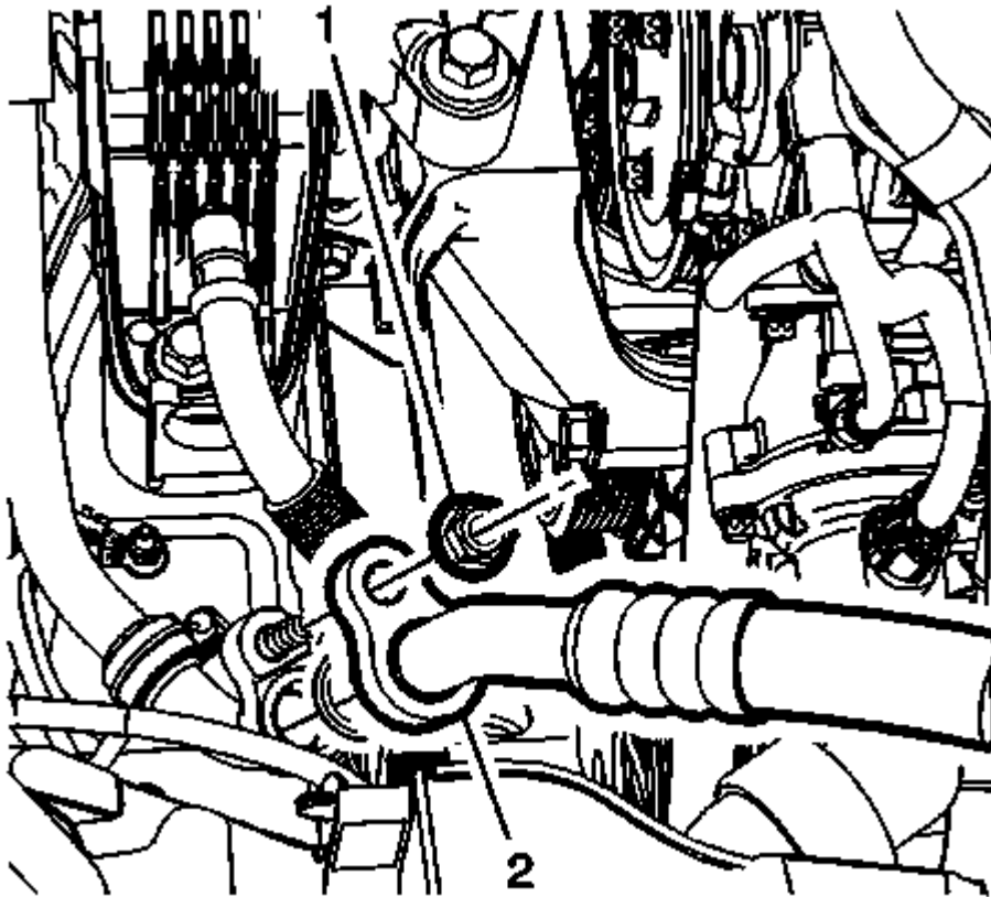
Fig. 207: Refrigerant Hose And Nut
