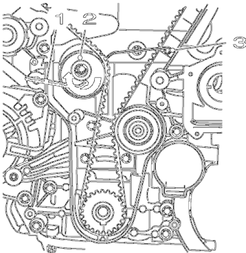
Fig. 93: Drive Belt Tensioner, Allen Key And Locking Pin Courtesy of GENERAL MOTORS COMPANY
