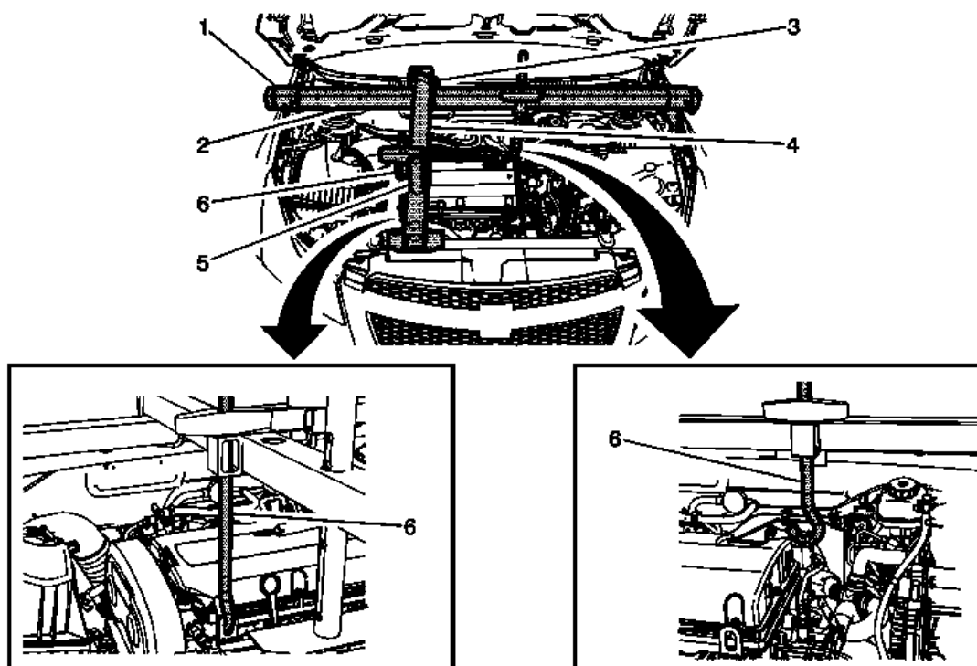
Fig. 307: Engine Support Fixture
