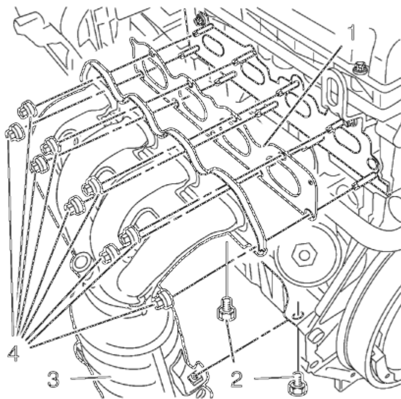
Fig. 378: Exhaust Manifold And Bolts
