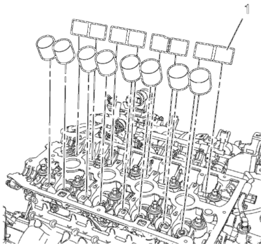
Fig. 395: Valve Lifters
