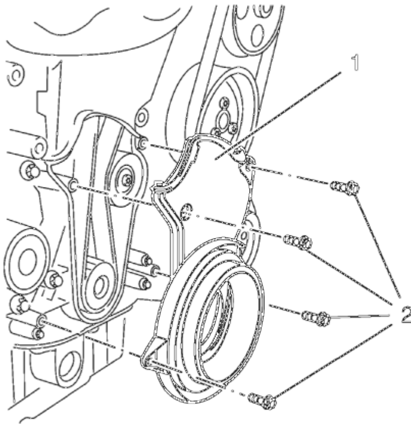
Fig. 319: Timing Belt Lower Front Cover Courtesy of GENERAL MOTORS COMPANY
