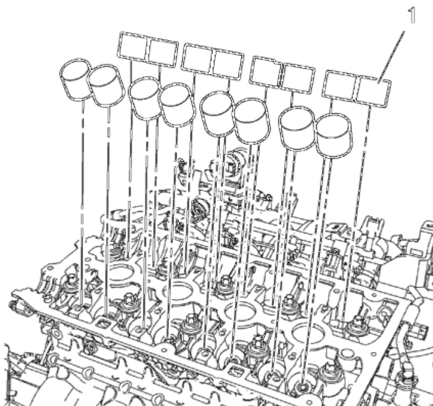
Fig. 113: Valve Lifters
