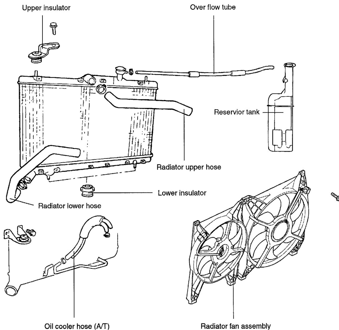
Fig. 112: Radiator Components Courtesy of HYUNDAI MOTOR CO.
