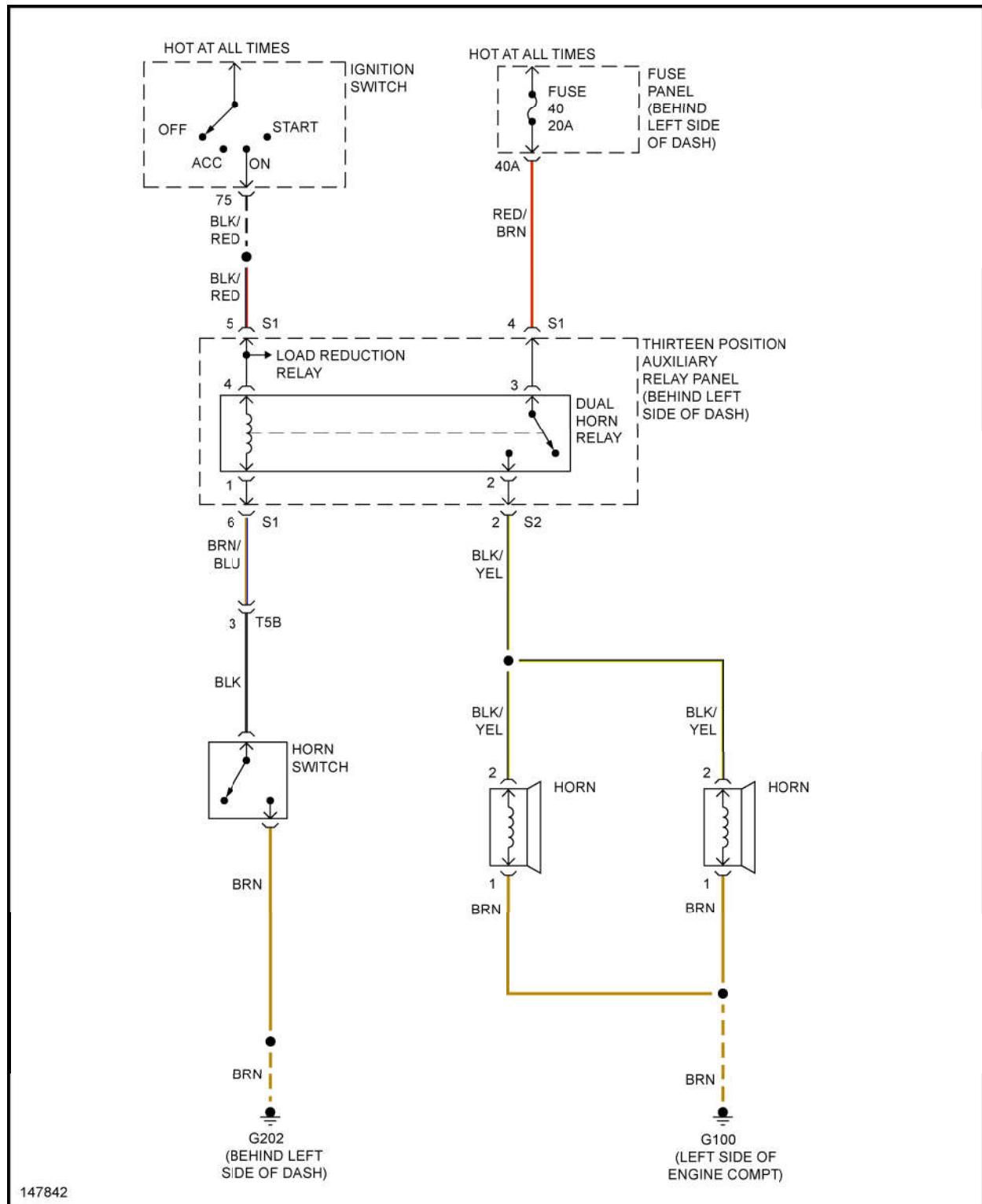
Fig. 41: Horn Circuit
