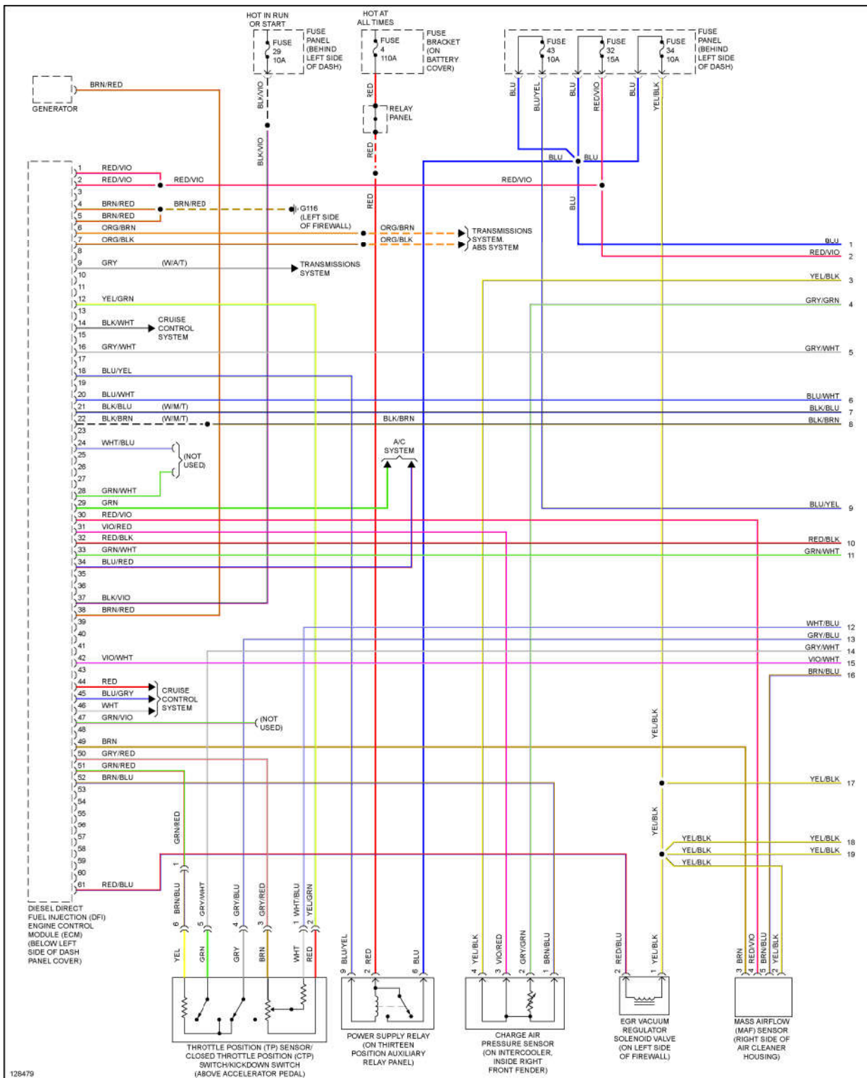
Fig. 25: 1.9L Turbo Diesel, Engine Performance Circuits (1 of 3)
