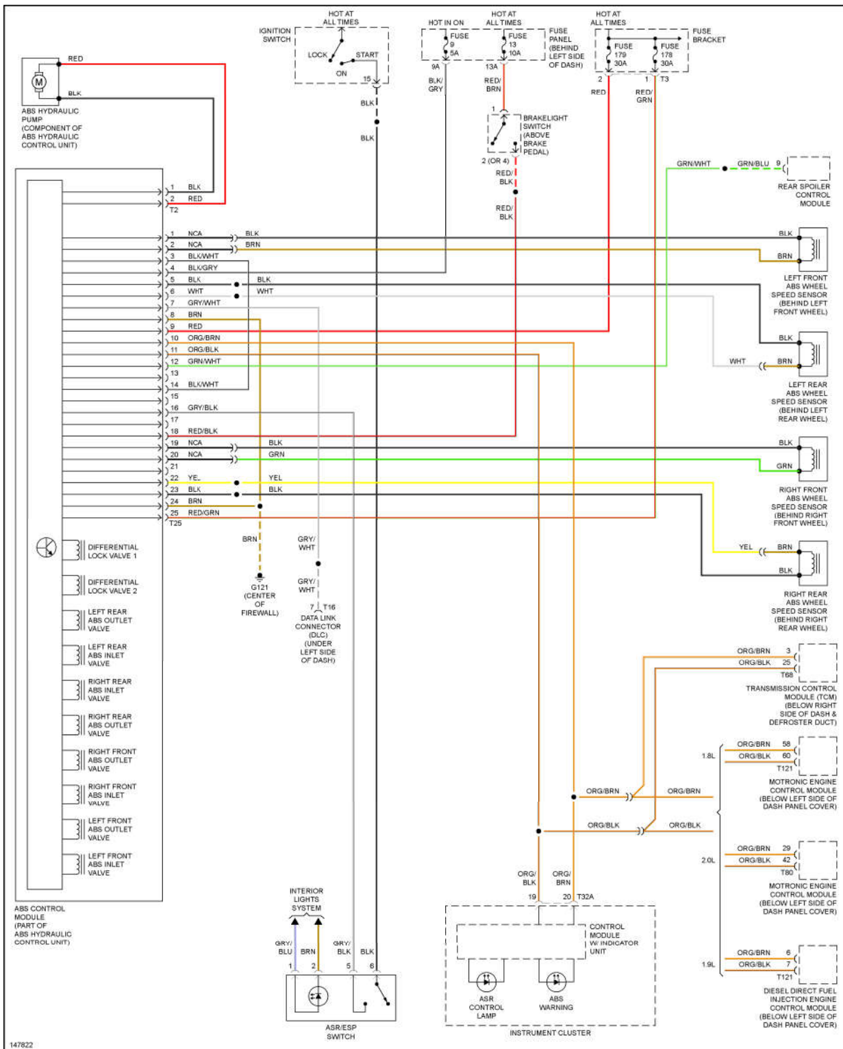
Fig. 5: Anti-lock Brake Circuits, Early Production
