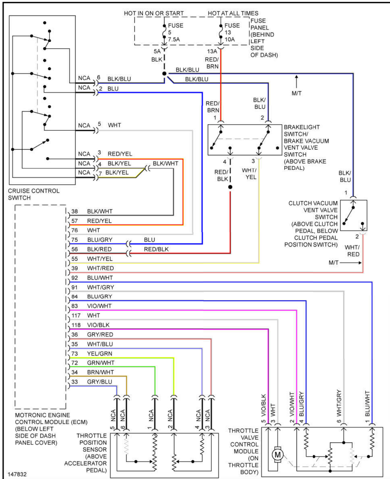
Fig. 16: 1.8L Turbo, Cruise Control Circuit
