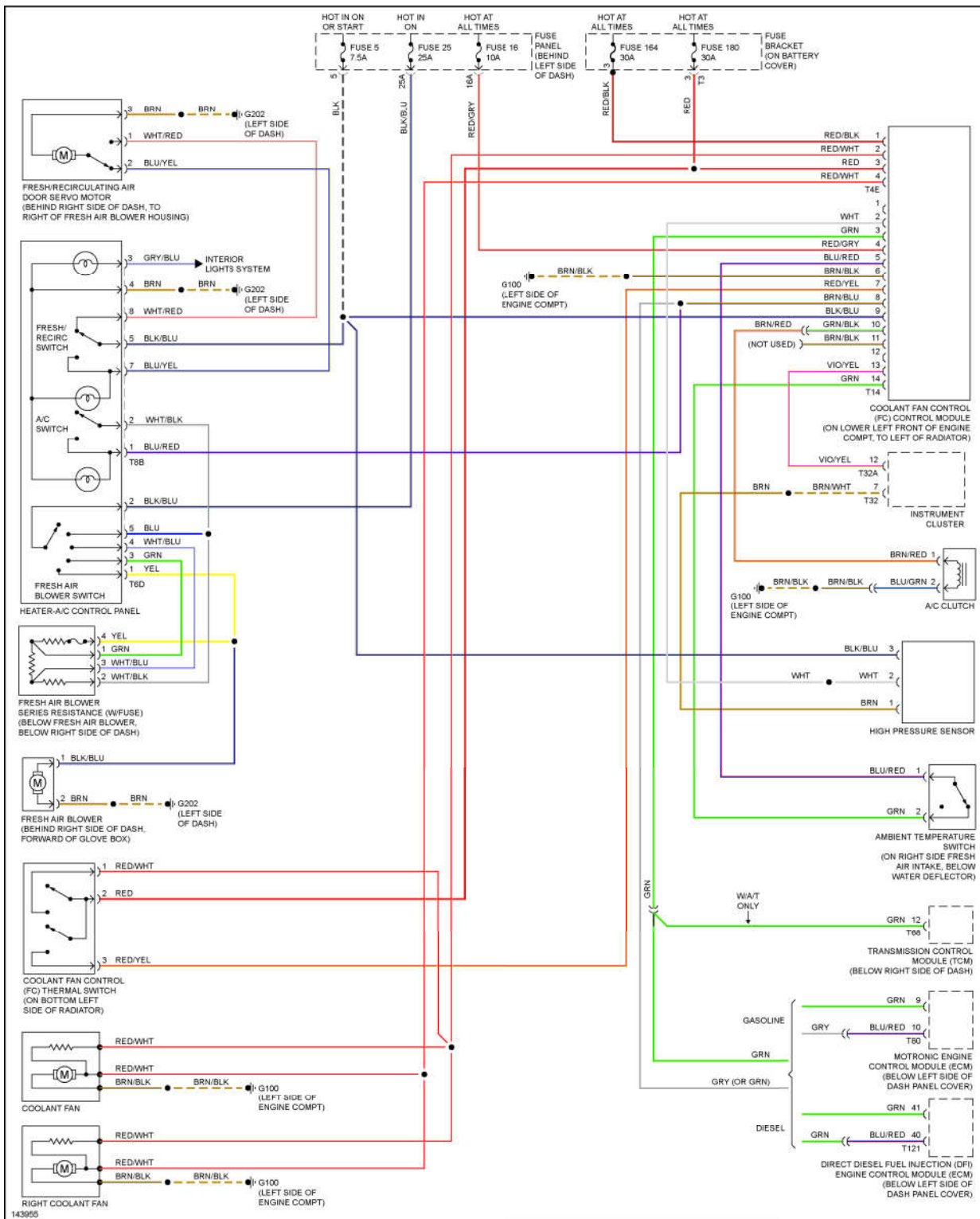
Fig. 4: 2.0L, Manual A/C Circuit
