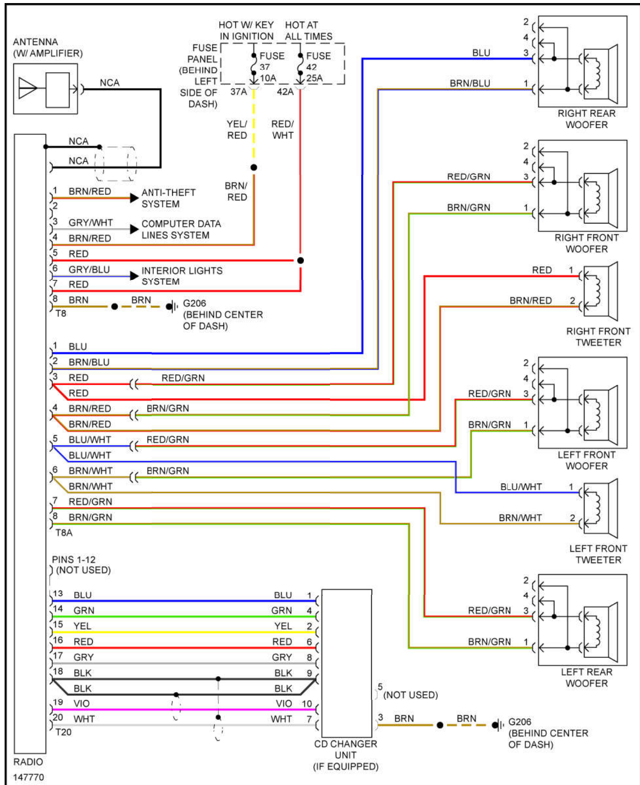
Fig. 61: Radio Circuits, Base Radio
