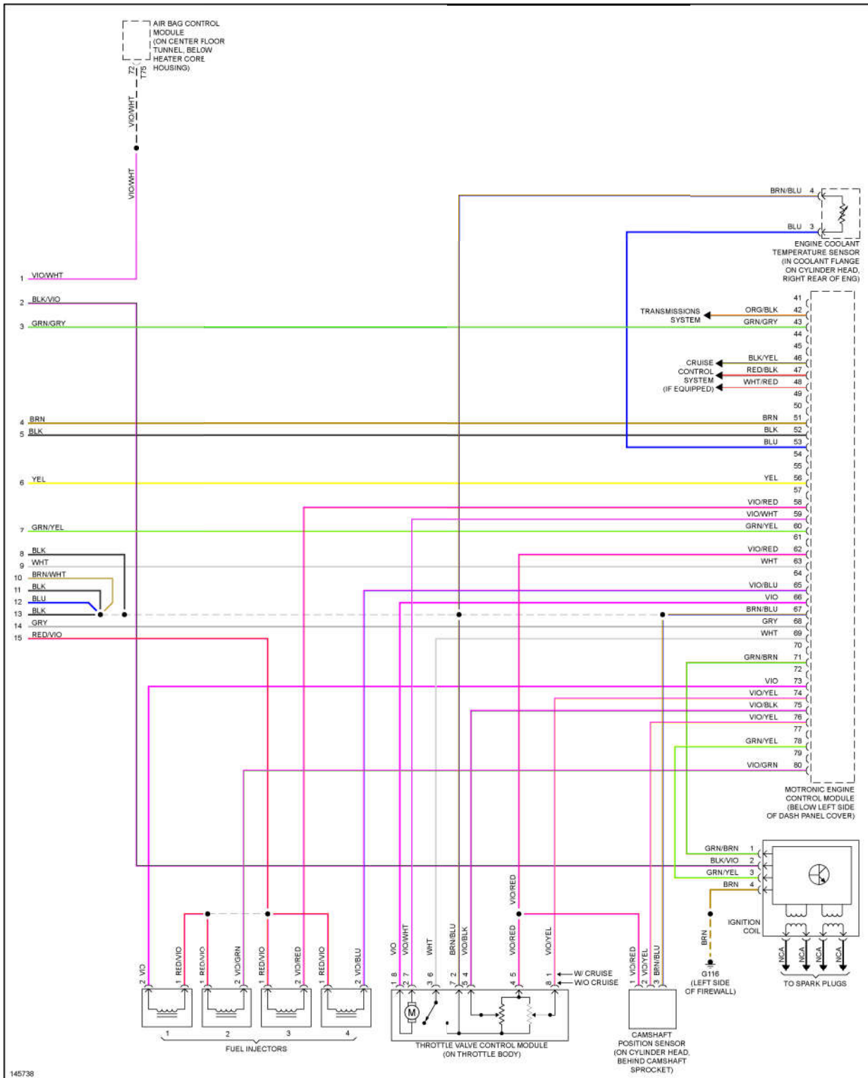
Fig. 30: 2.0L, Engine Performance Circuits, Early Production (3 of 3)
