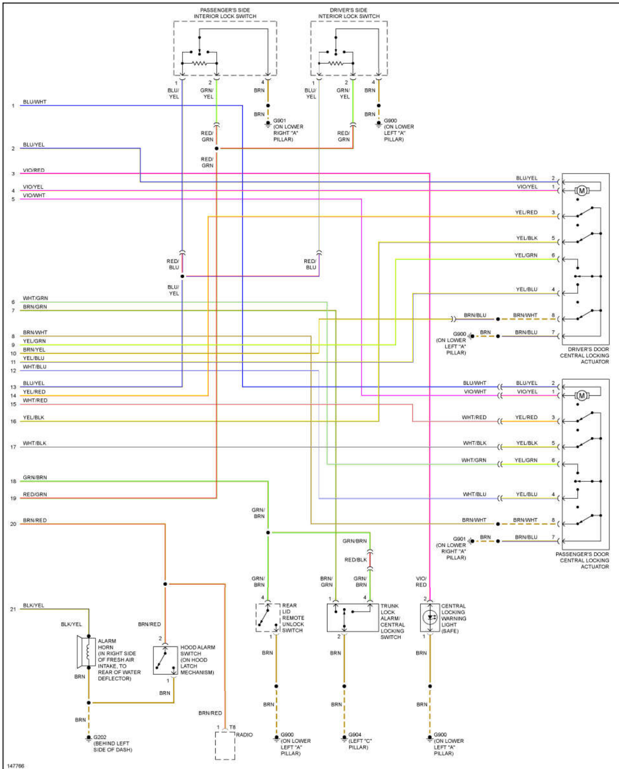
Fig. 10: Anti-theft Circuit, W/O Power Windows (2 of 2)
