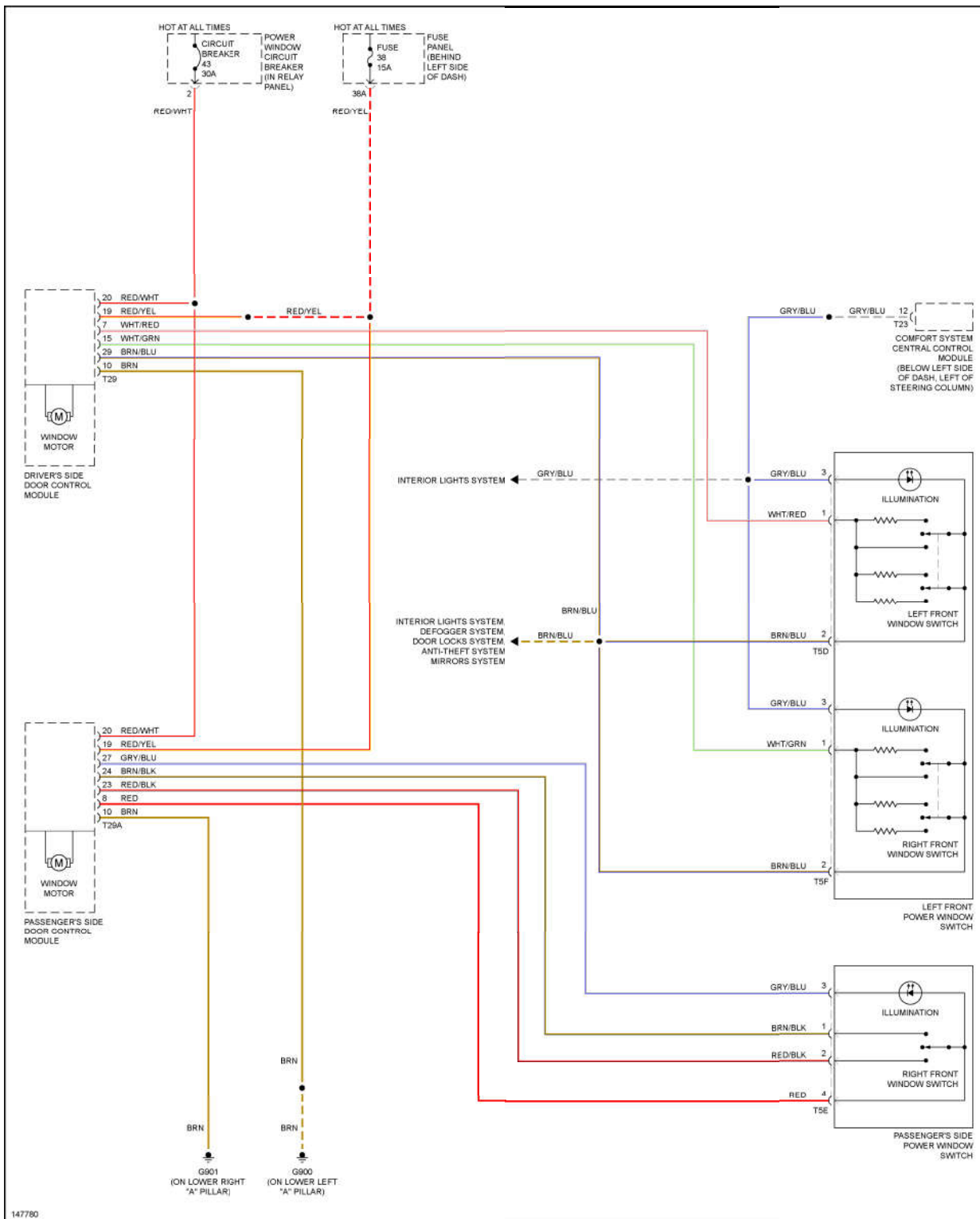
Fig. 60: Power Window Circuit
