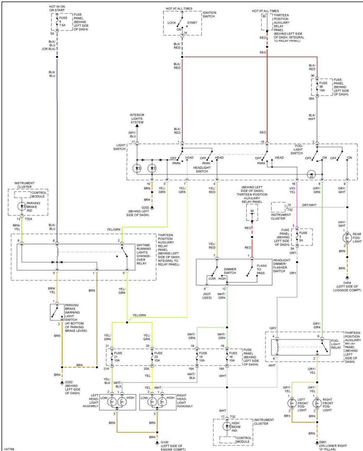
Fig. 40: Headlight Circuit
