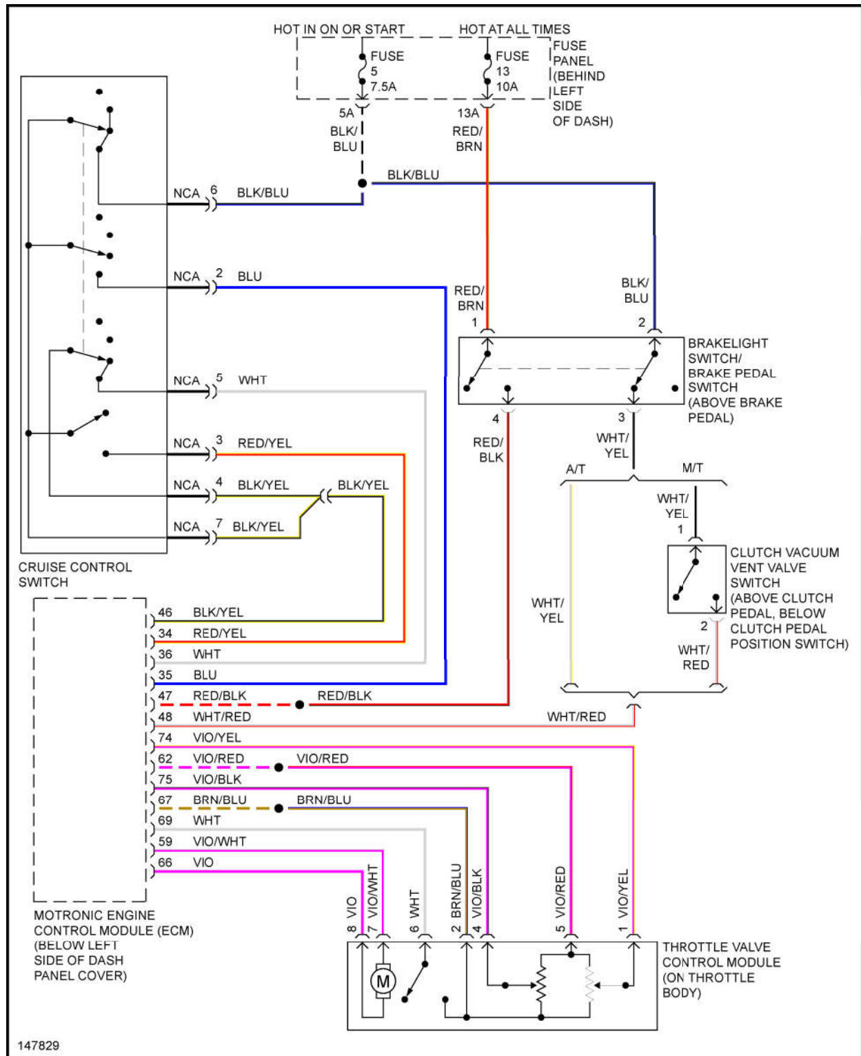
Fig. 18: 2.0L, Cruise Control Circuit, Early Production
