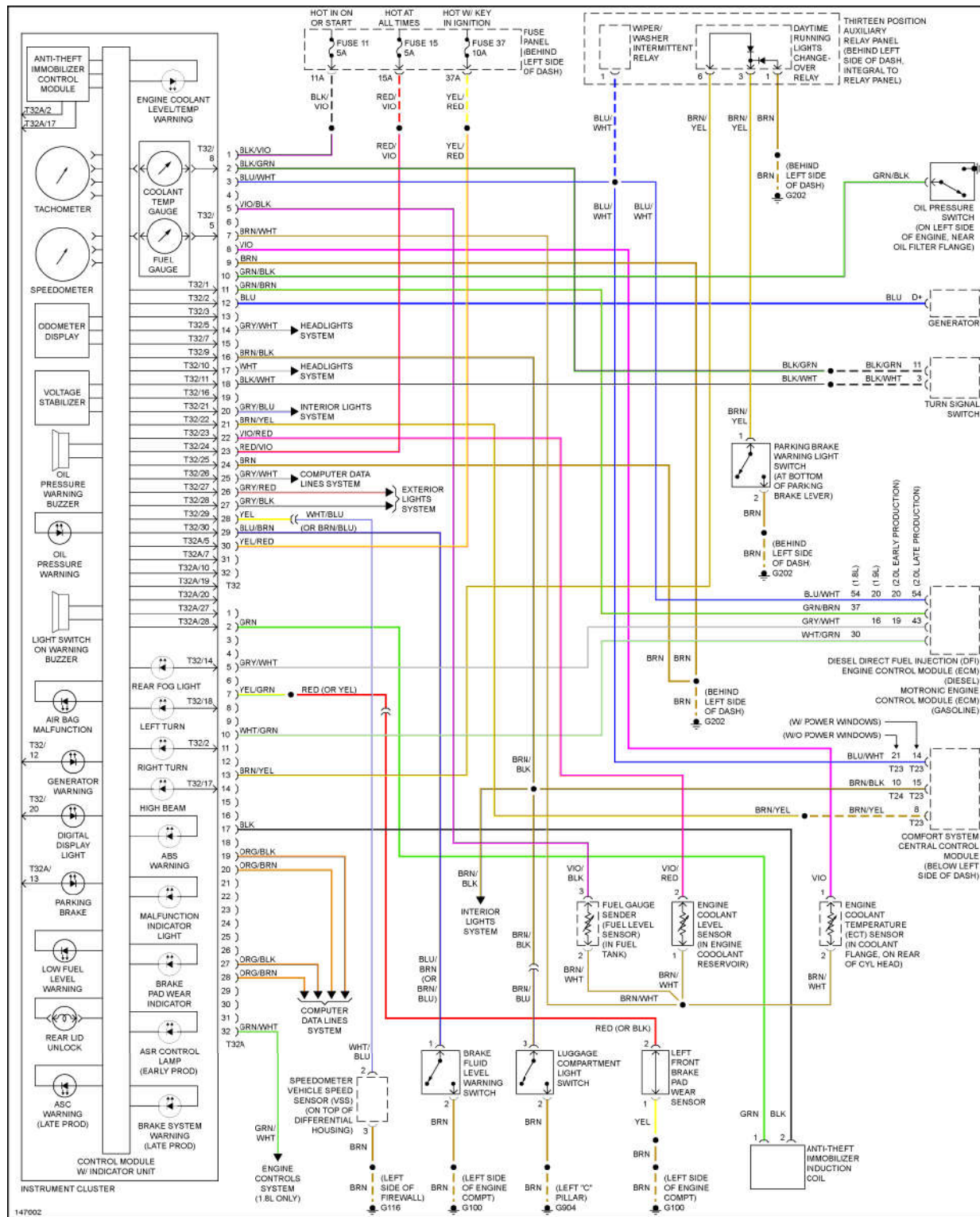
Fig. 43: Gauges And Indicators Circuit
