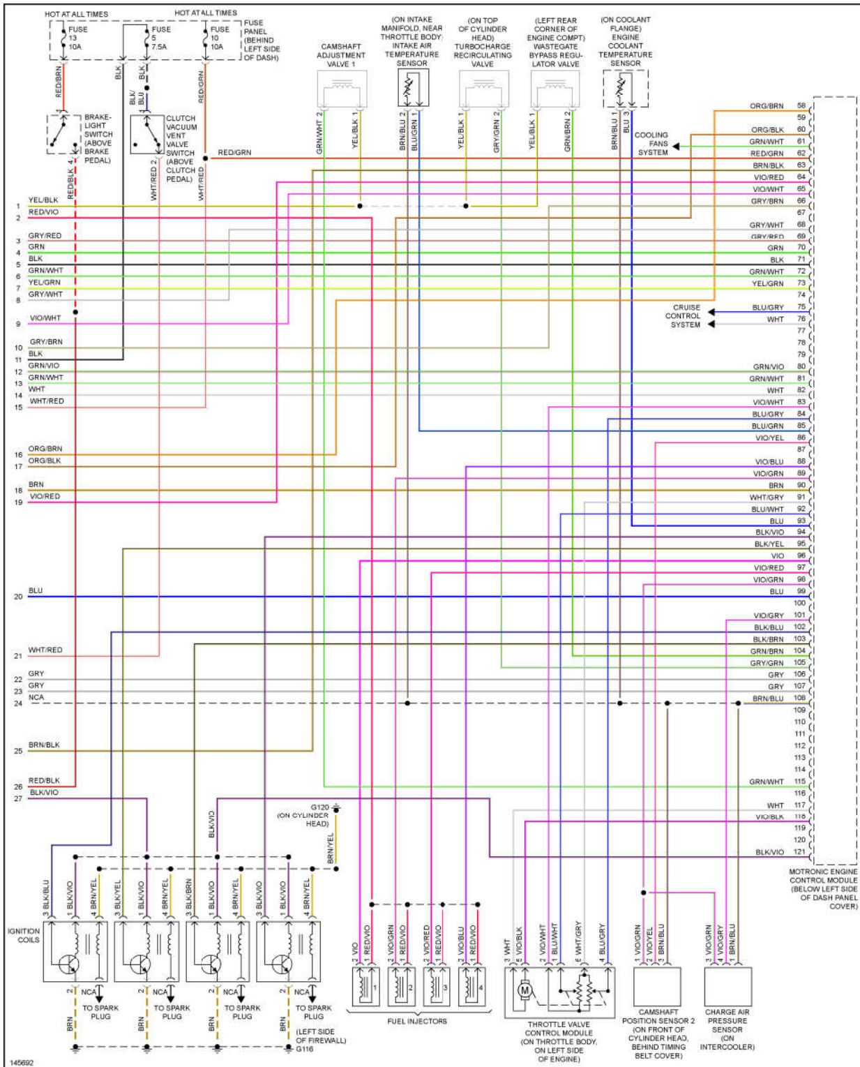
Fig. 24: 1.8L Turbo, Engine Performance Circuits (3 of 3)
