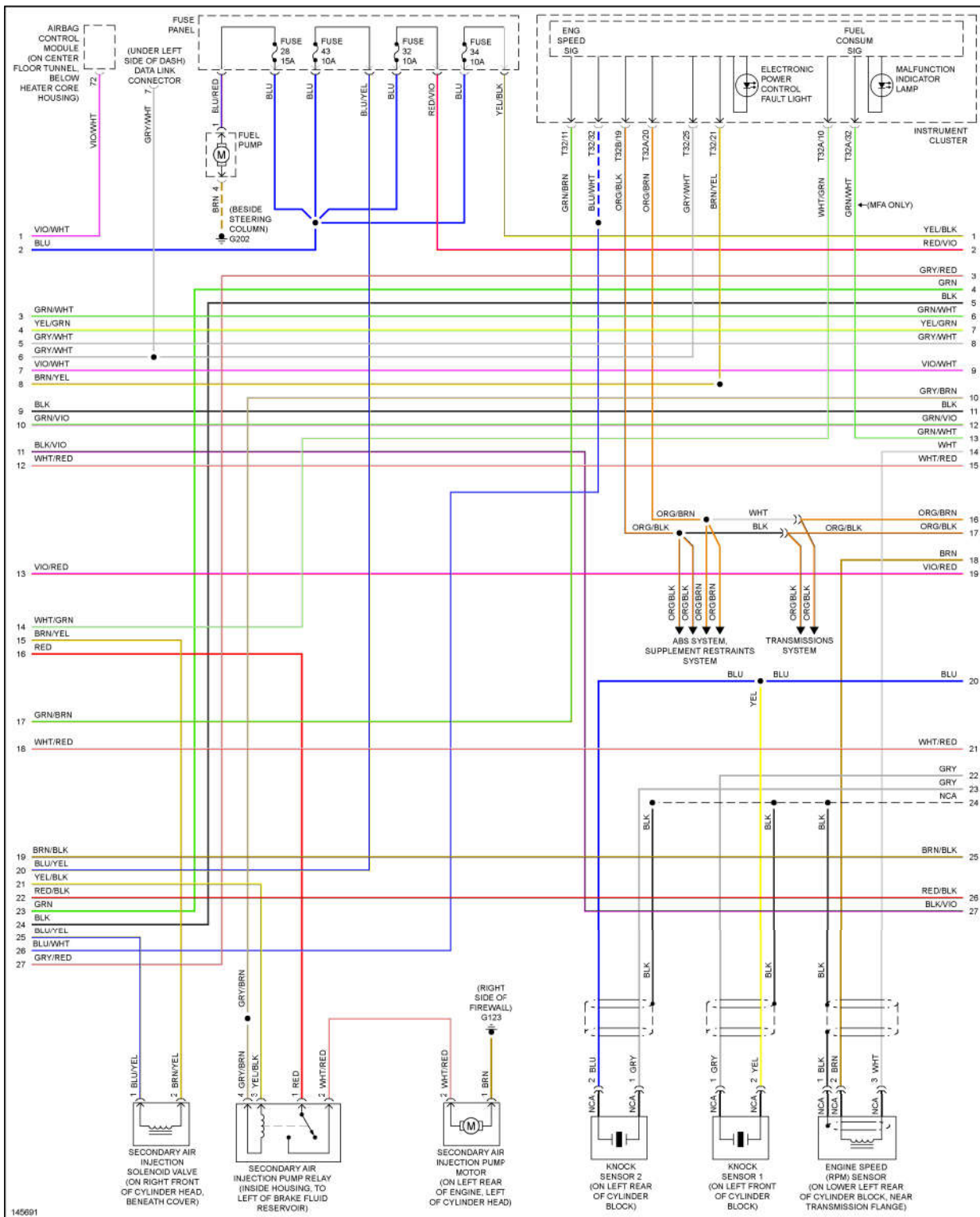
Fig. 23: 1.8L Turbo, Engine Performance Circuits (2 of 3)
