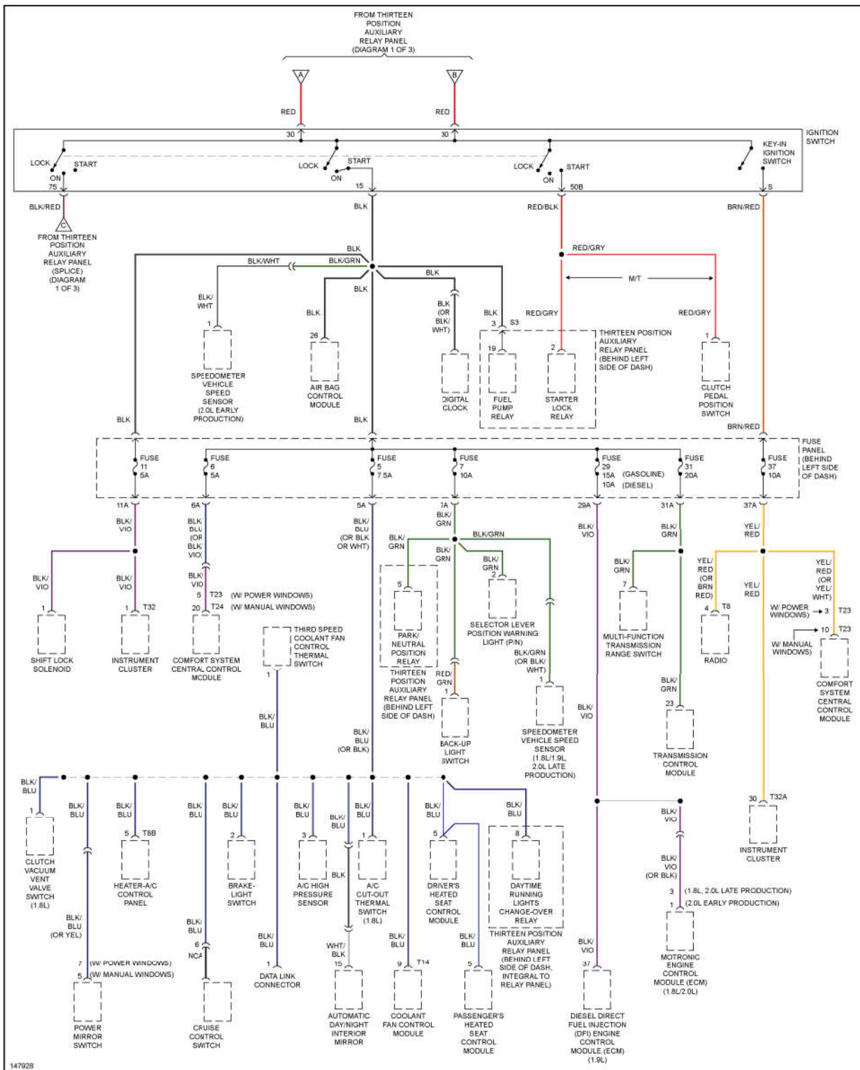
Fig. 49: Power Distribution Circuit (2 of 3)
