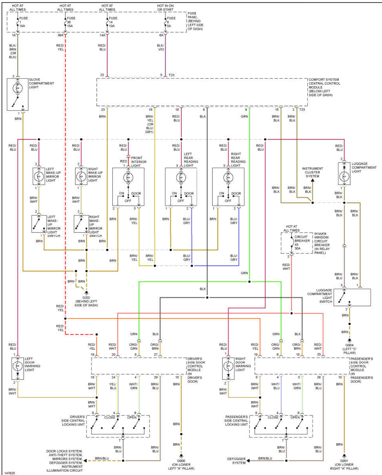
Fig. 44: Courtesy Lamps Circuit, W/ Power Windows
