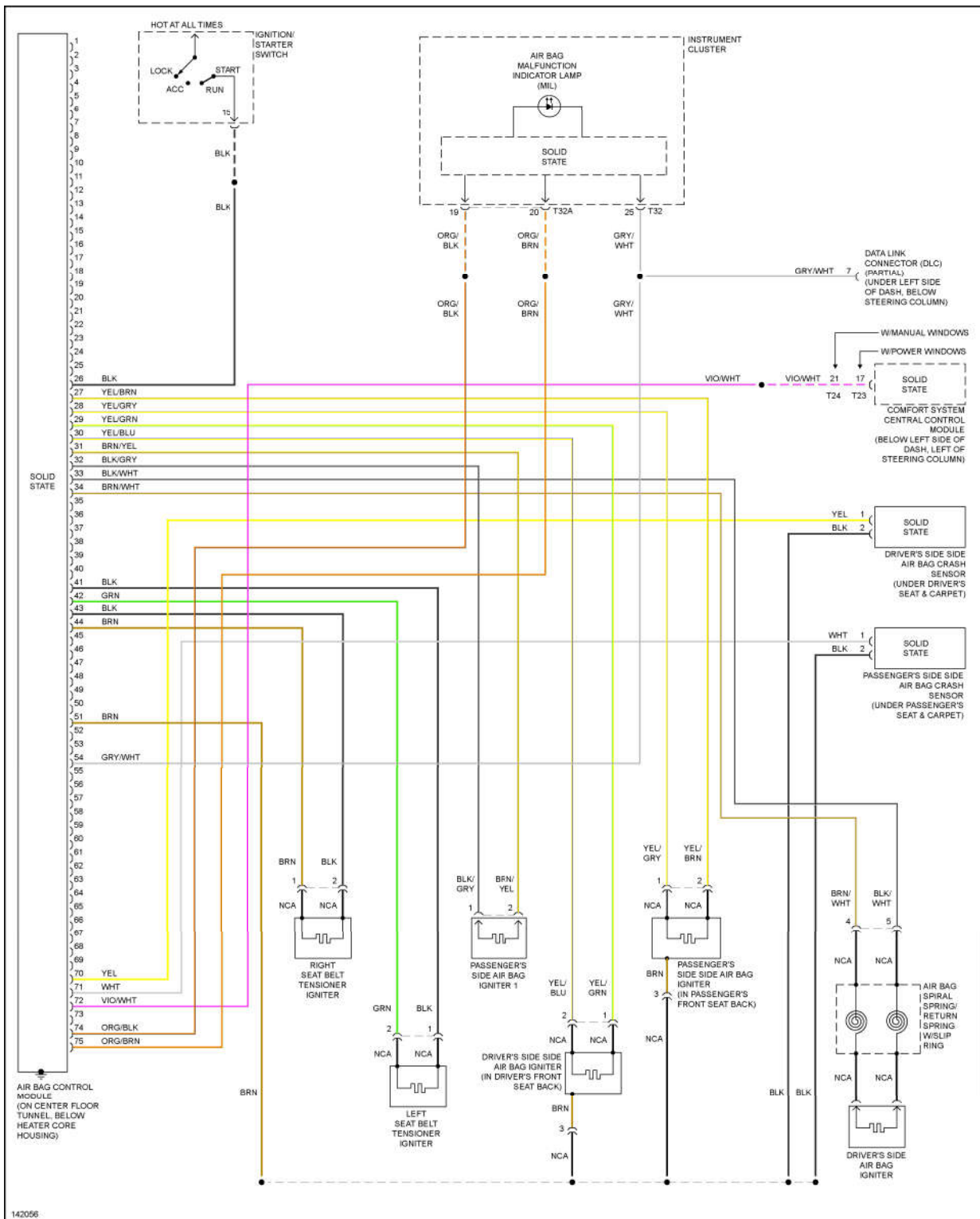
Fig. 67: Supplemental Restraint Circuit, Early Production
