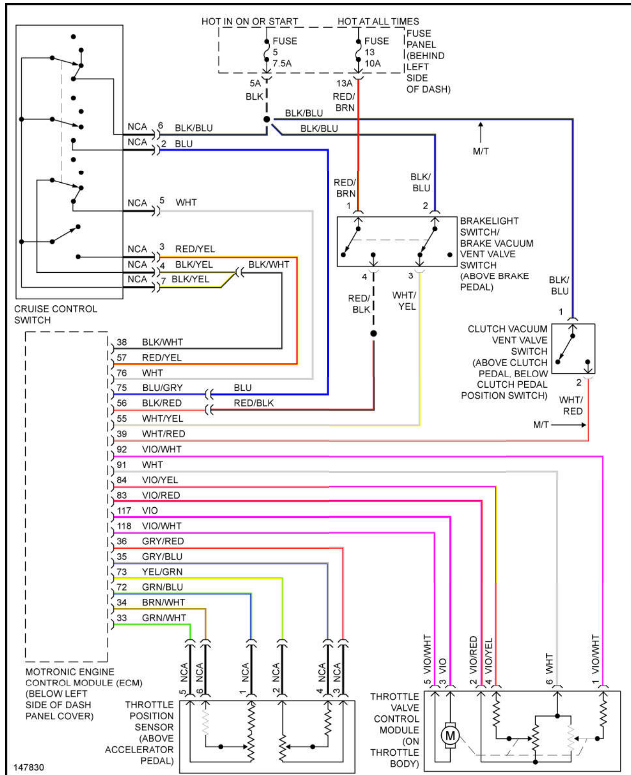
Fig. 19: 2.0L, Cruise Control Circuit, Late Production
