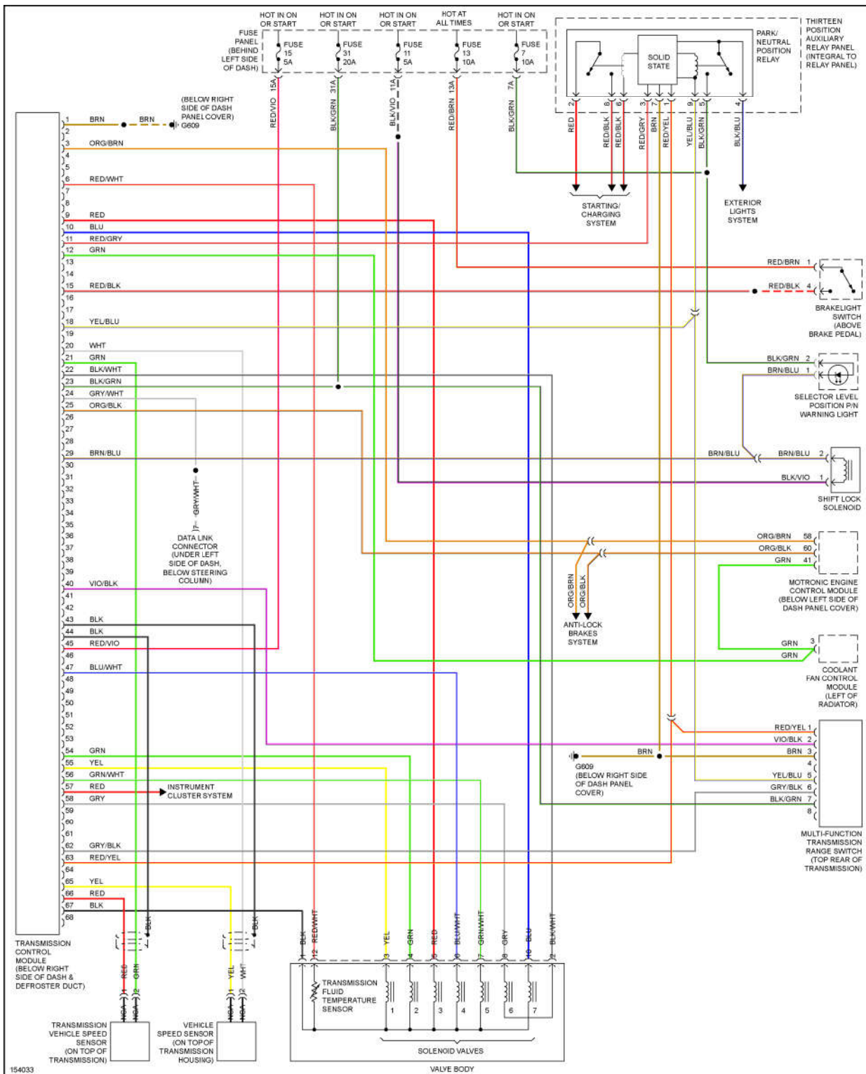
Fig. 73: 2.0L, A/T Circuit, Late Production
