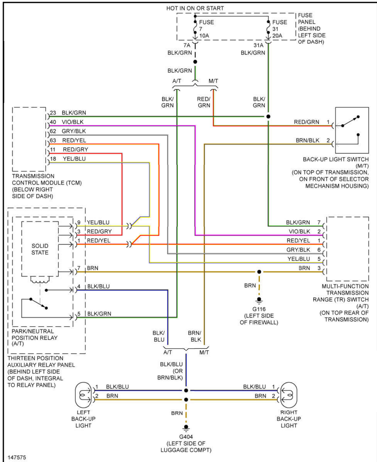
Fig. 34: Back-up Lamps Circuit
