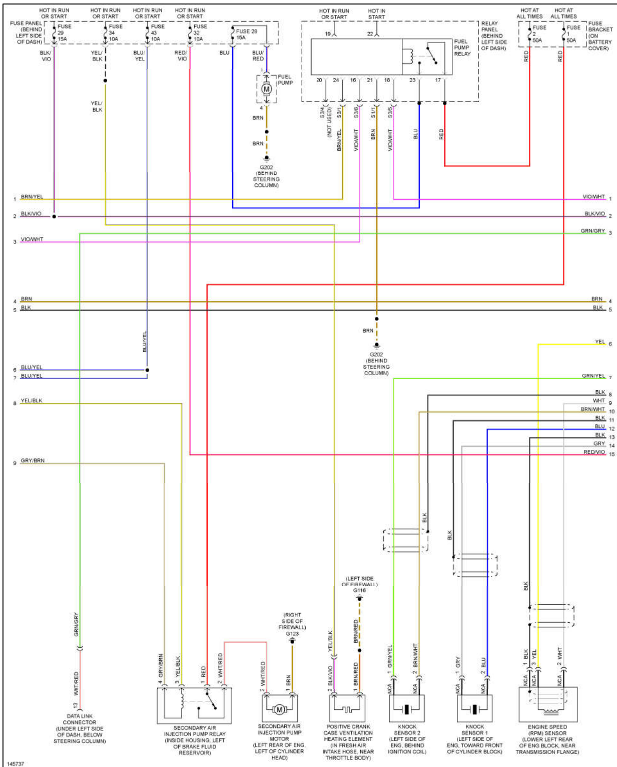
Fig. 29: 2.0L, Engine Performance Circuits, Early Production (2 of 3)
