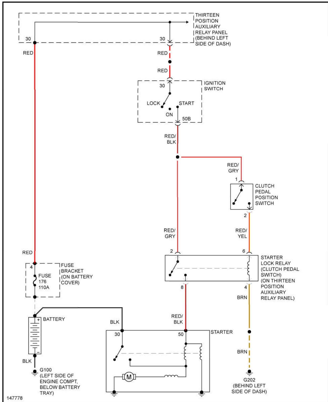
Fig. 66: Starting Circuit, M/T
