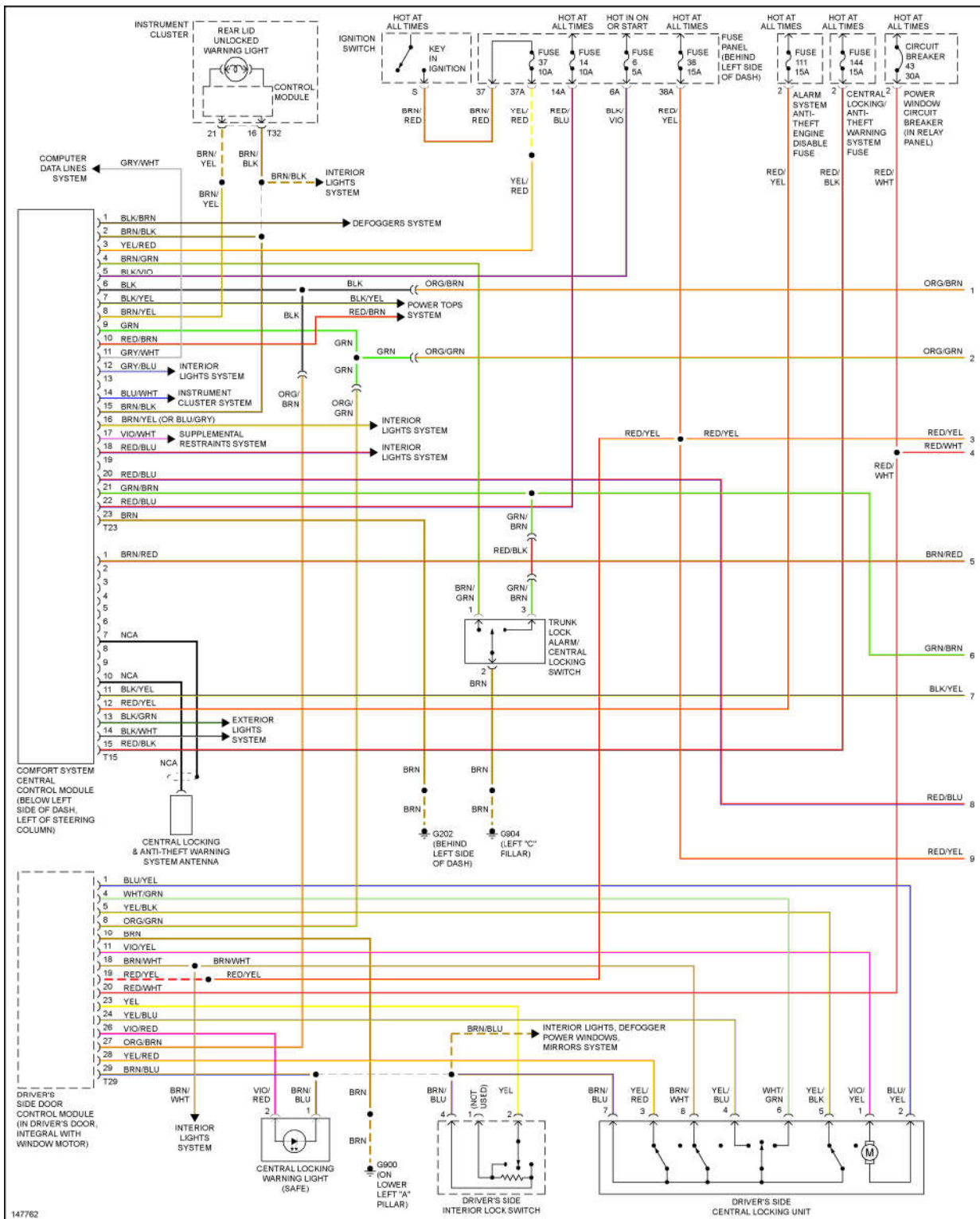
Fig. 7: Anti-theft Circuit, W/ Power Windows (1 of 2)
