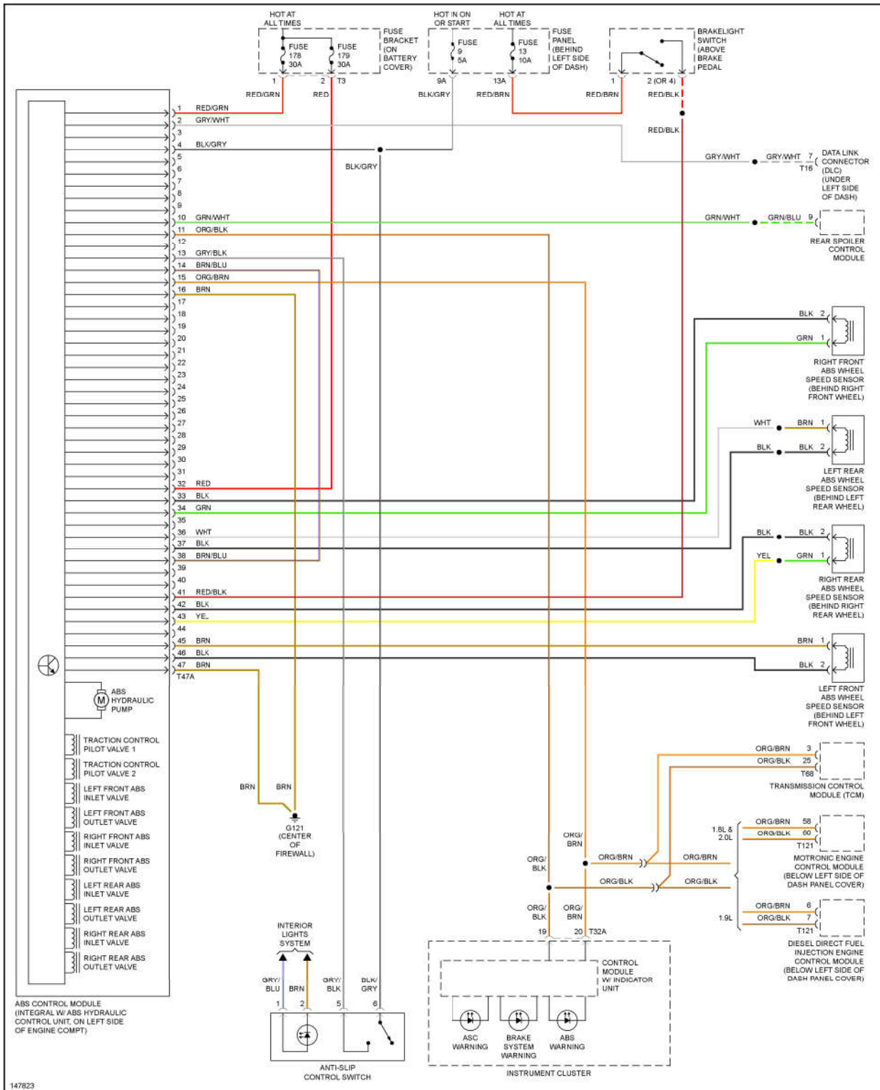
Fig. 6: Anti-lock Brake Circuits, Late Production
