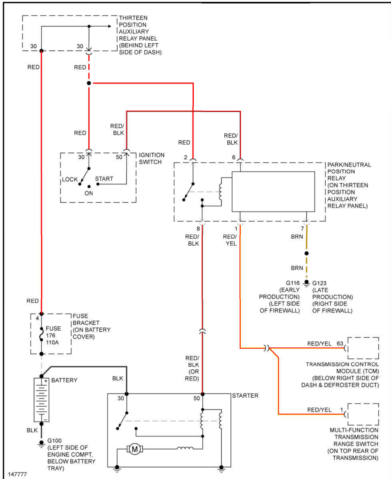
Fig. 65: Starting Circuit, A/T
