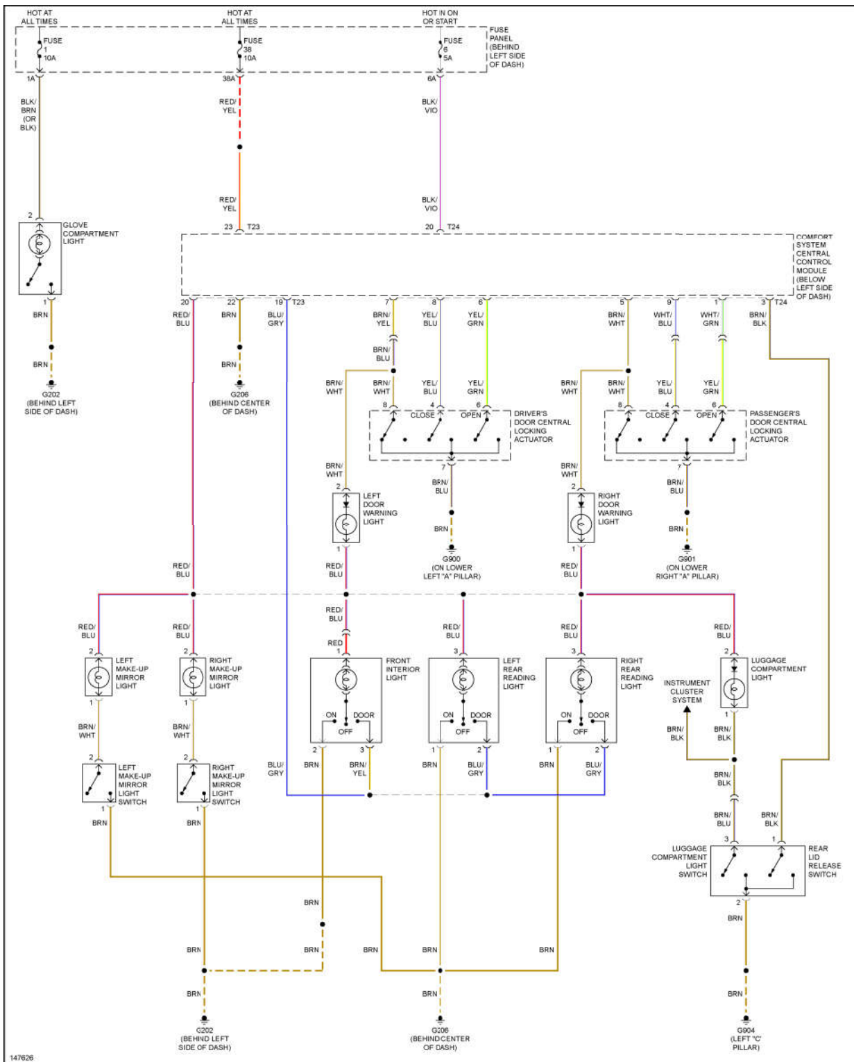
Fig. 45: Courtesy Lamps Circuit, W/O Power Windows
