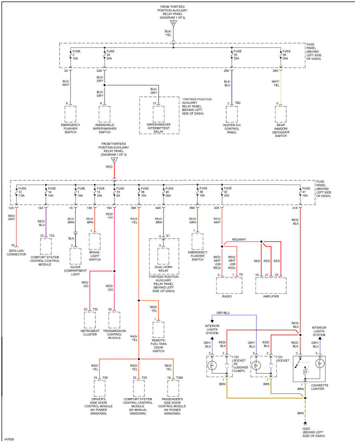
Fig. 50: Power Distribution Circuit (3 of 3)
