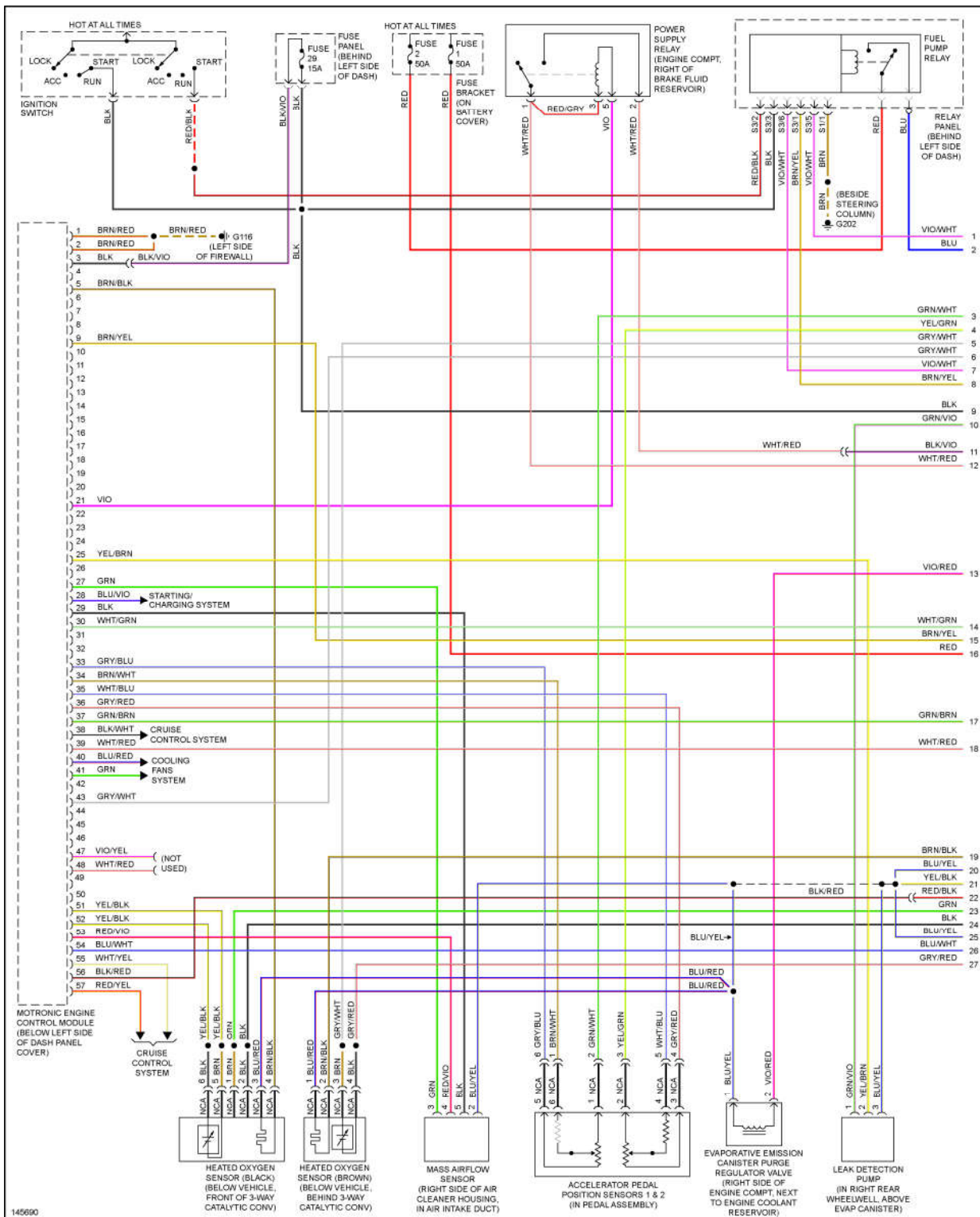
Fig. 22: 1.8L Turbo, Engine Performance Circuits (1 of 3)
