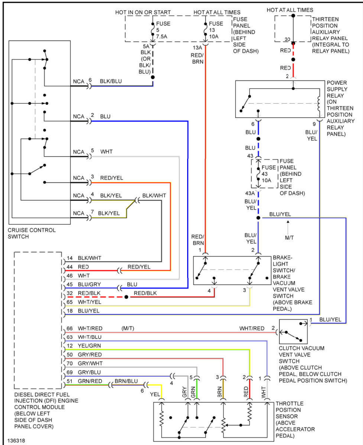
Fig. 17: 1.9L Turbo Diesel, Cruise Control Circuit
