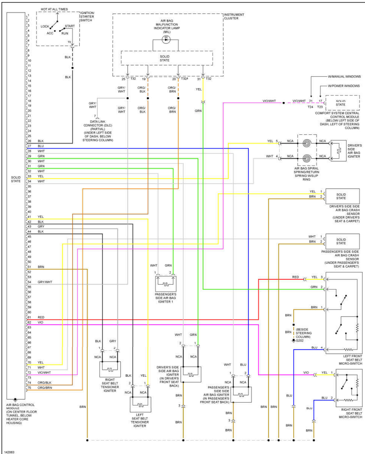
Fig. 68: Supplemental Restraint Circuit, Late Production
