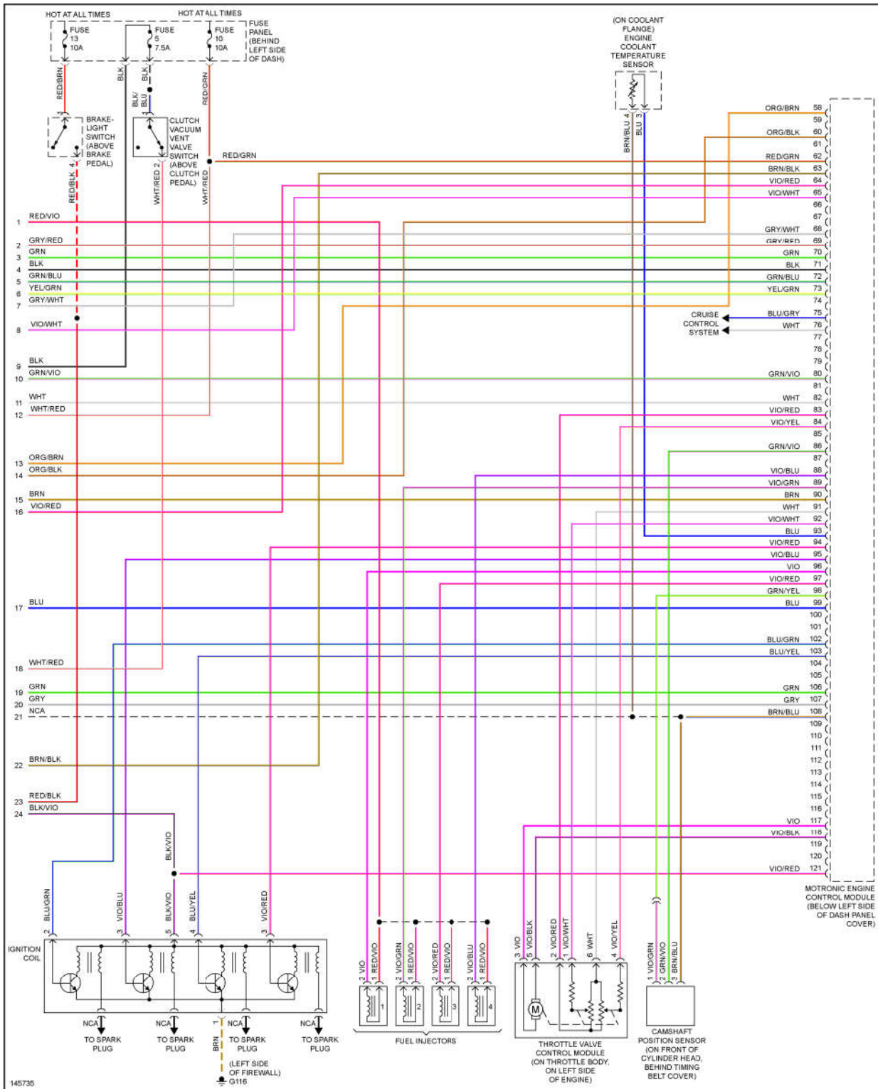
Fig. 33: 2.0L, Engine Performance Circuits, Late Production (3 of 3)
