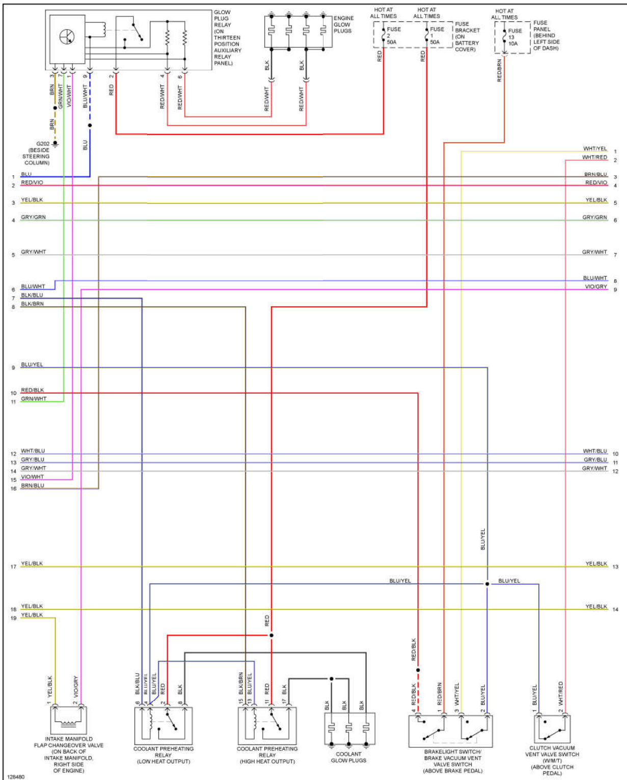
Fig. 26: 1.9L Turbo Diesel, Engine Performance Circuits (2 of 3)
