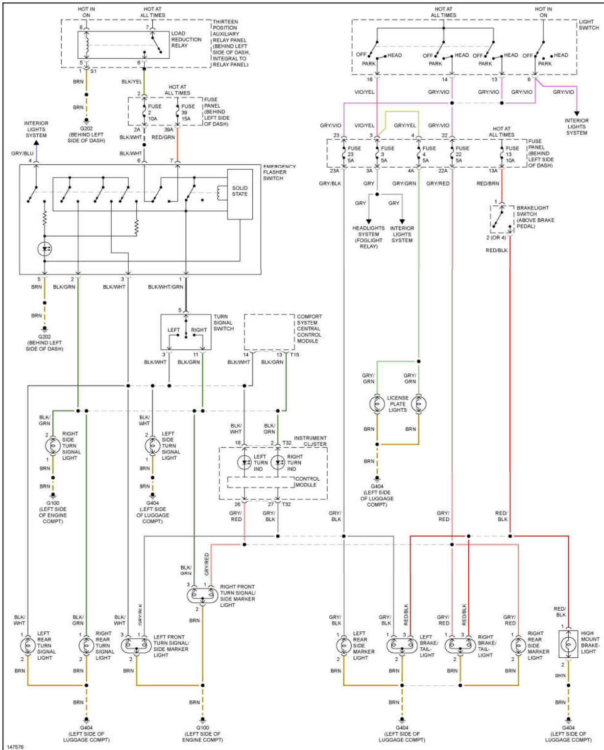
Fig. 35: Exterior Lamps Circuit
