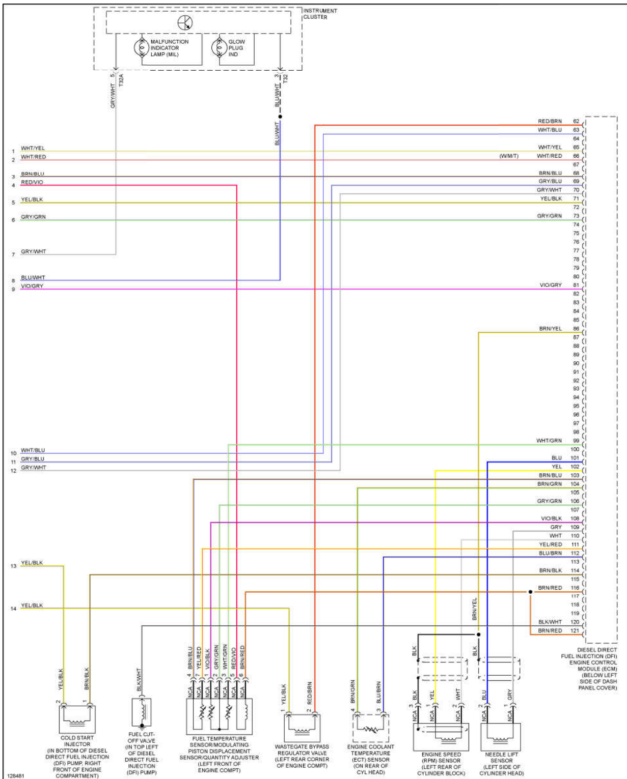
Fig. 27: 1.9L Turbo Diesel, Engine Performance Circuits (3 of 3)
