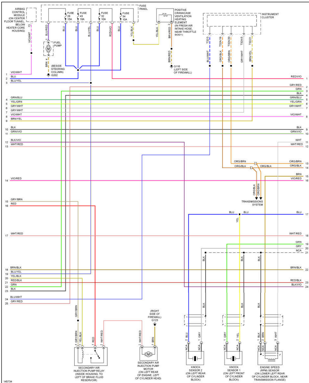
Fig. 32: 2.0L, Engine Performance Circuits, Late Production (2 of 3)
