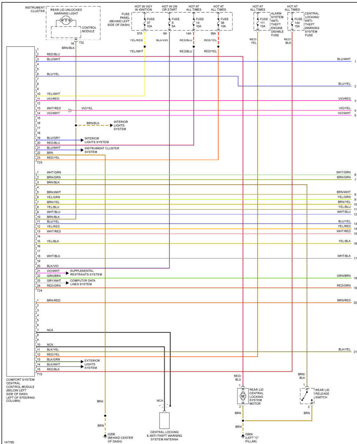
Fig. 9: Anti-theft Circuit, W/O Power Windows (1 of 2)
