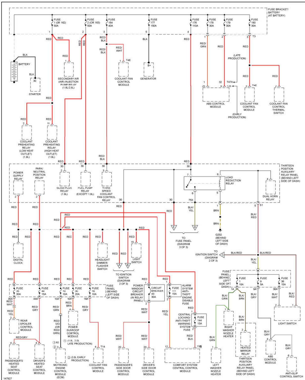
Fig. 48: Power Distribution Circuit (1 of 3)
