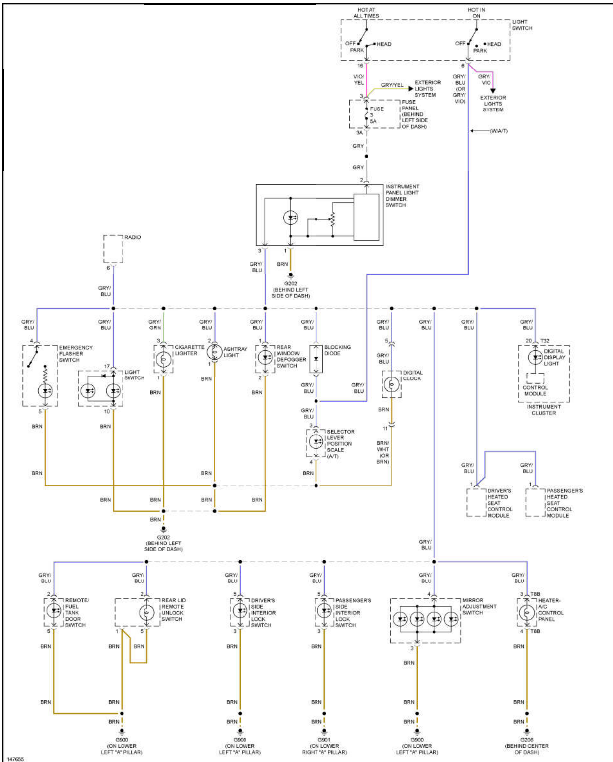
Fig. 47: Instrument Illumination Circuit, W/O Power Windows
