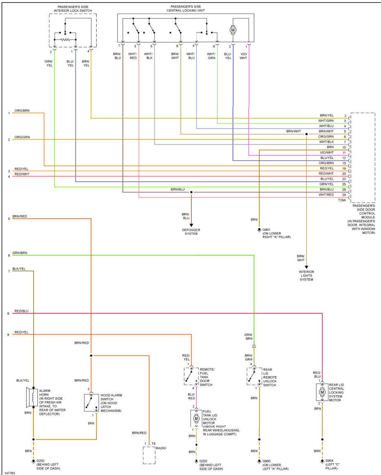
Fig. 52: Power Door Lock Circuit, W/ Power Windows (2 of 2)
