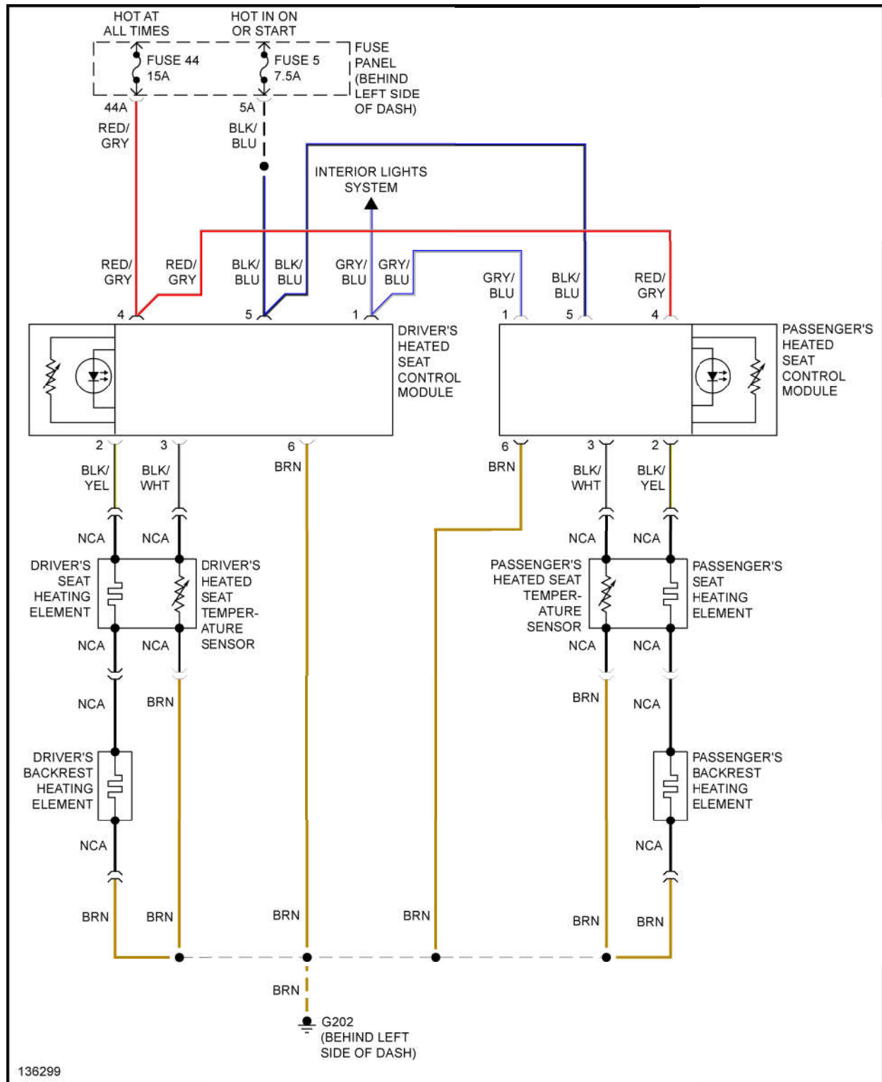
Fig. 58: Heated Seats Circuit
