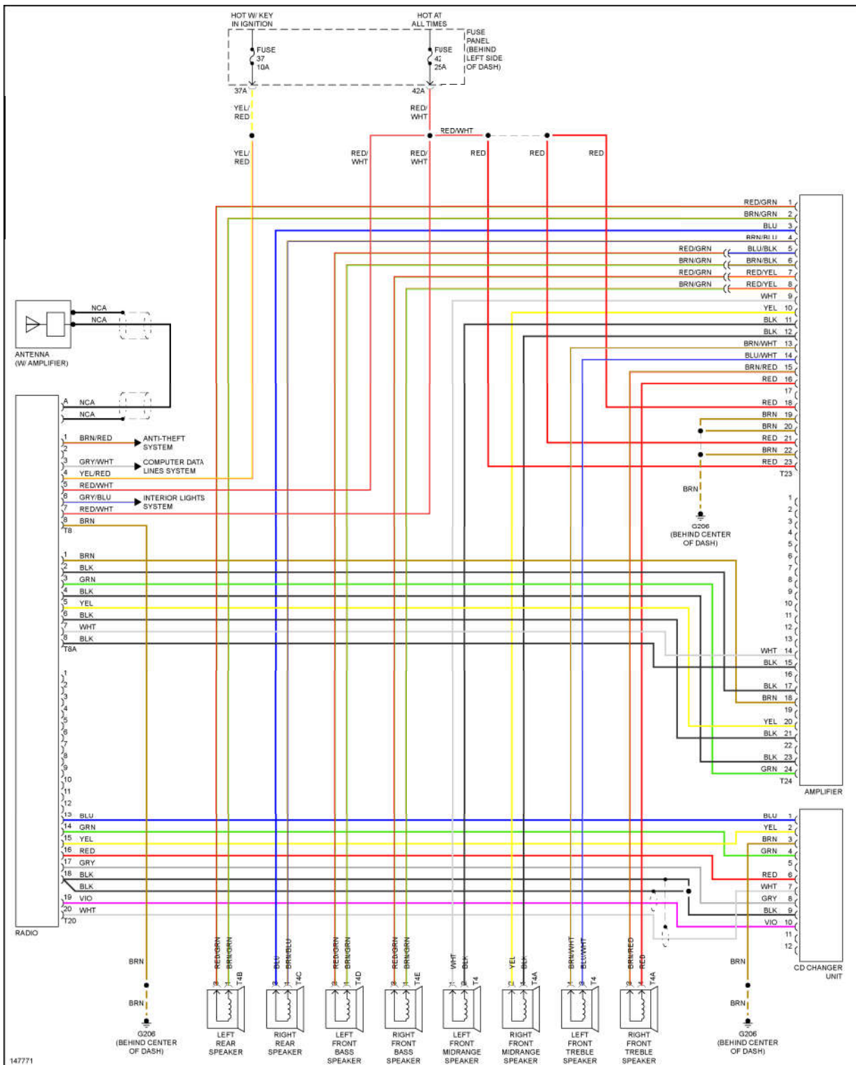
Fig. 62: Radio Circuits, Premium Radio
