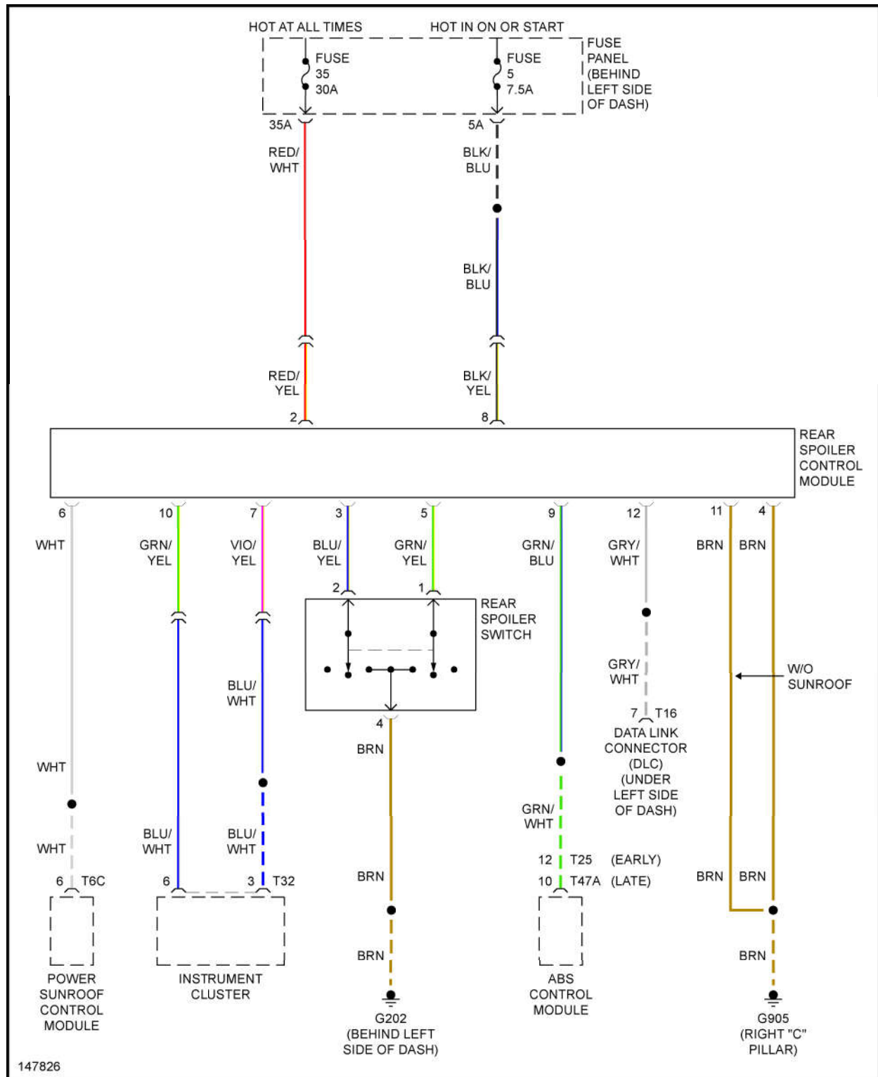
Fig. 1: Active Aerodynamic Circuit
