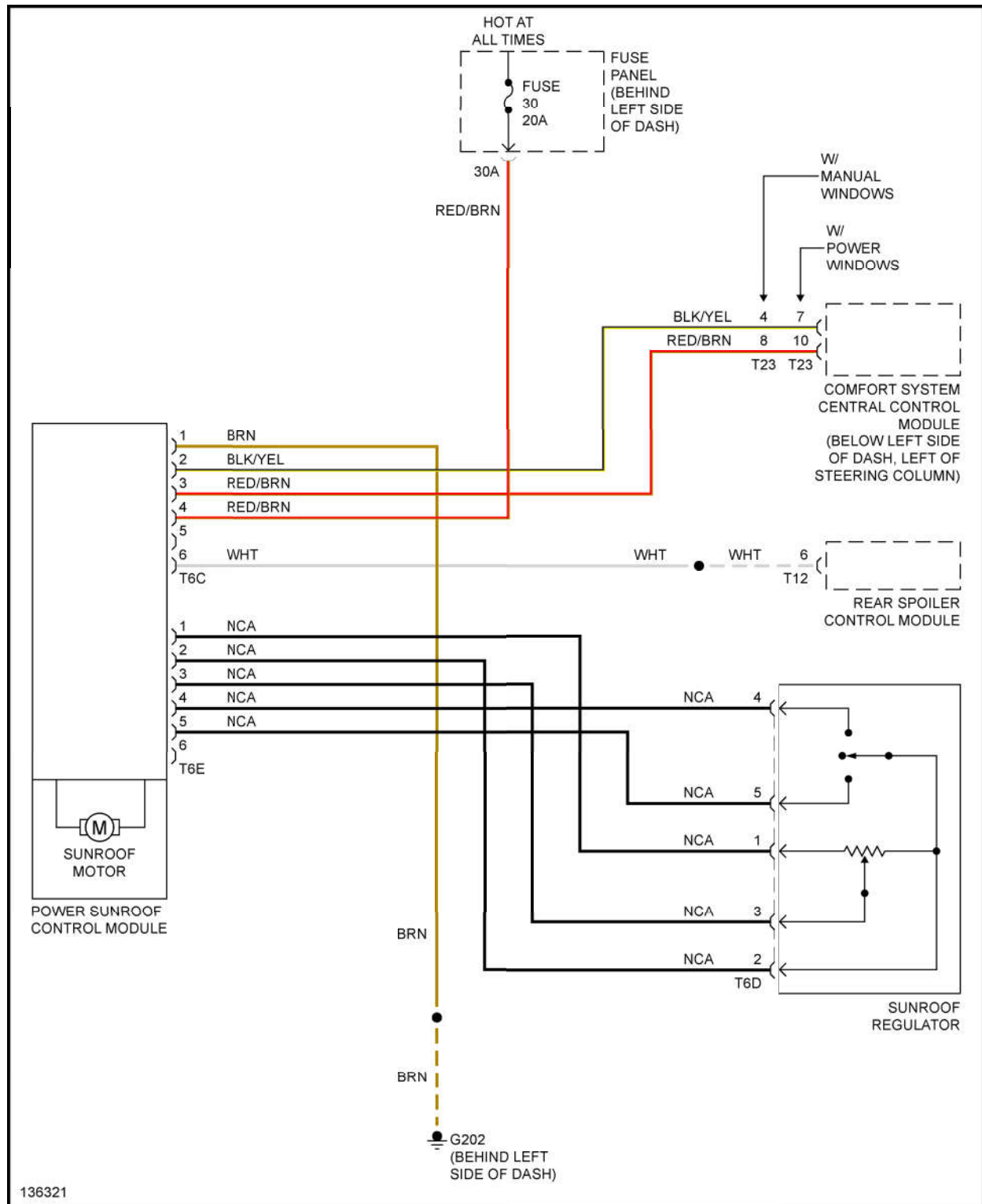
Fig. 59: Sunroof Circuit
