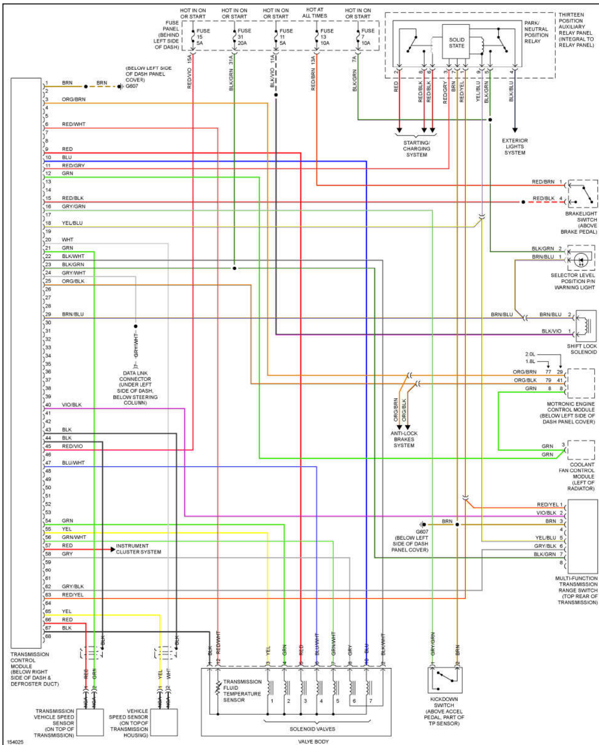
Fig. 72: 2.0L, A/T Circuit, Early Production
