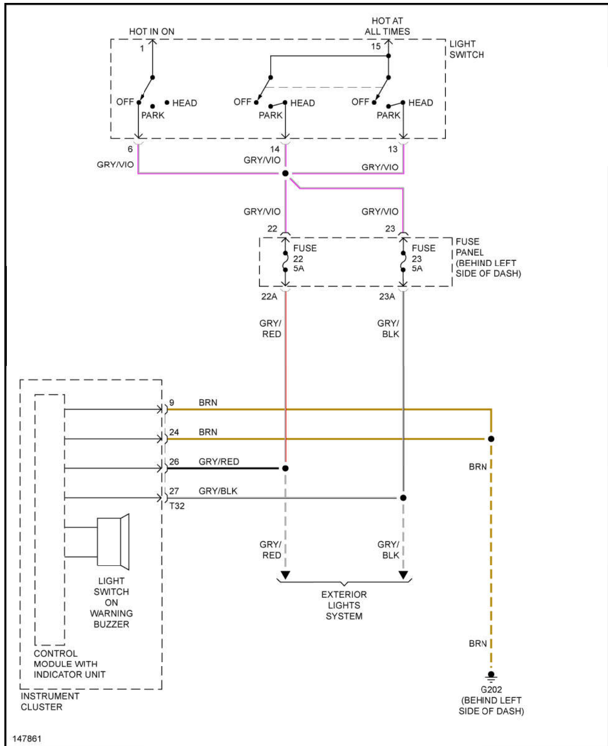
Fig. 76: Buzzer Circuit
