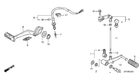
C-20 Pedal
