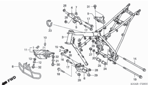
C-28 Chasis (CTX200, 9, A, B, C, D)
