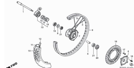
F-10 Front Wheel (CTX200, 9, A, B, C, D)
