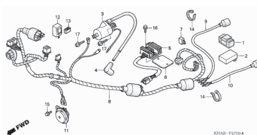
C-28.1 Chasis (CTX200E)
