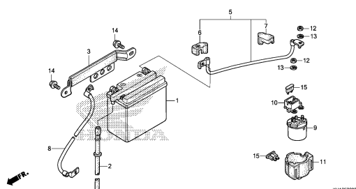
C-28 Chasis (CTX200, 9, A, B, C, D)
