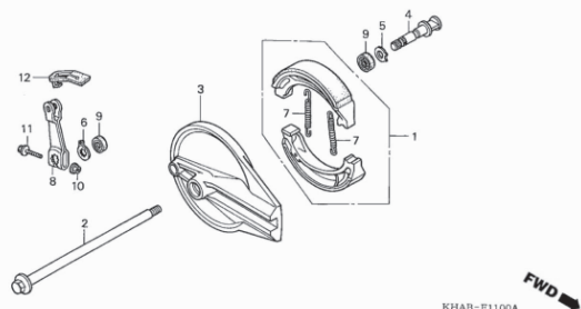
F-12.1 Rear Wheel (CTX200E)
