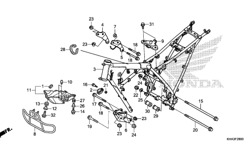
C-28.1 Chasis (CTX200E)
