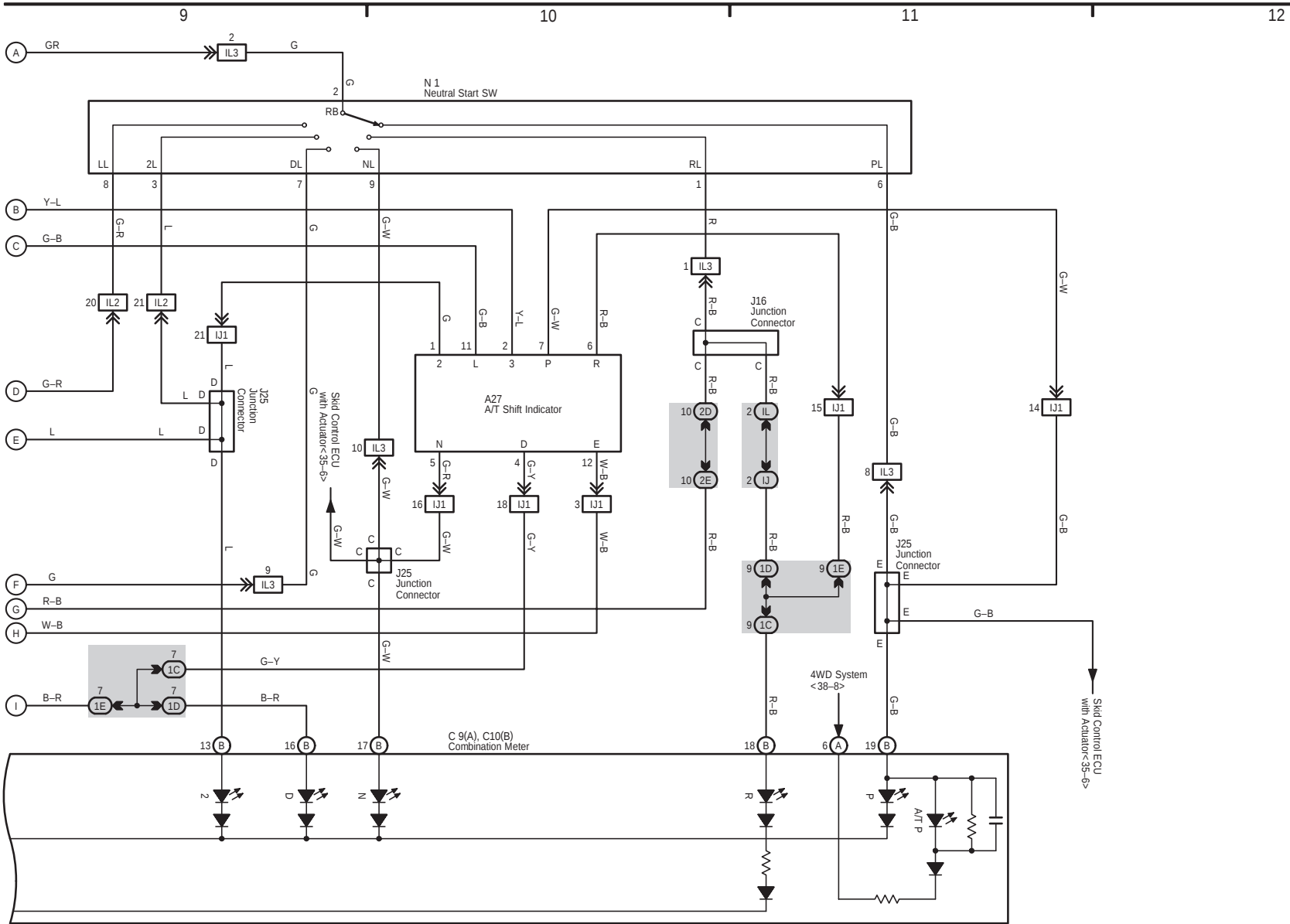
ECT and A/T Indicator (2TR-FE)
