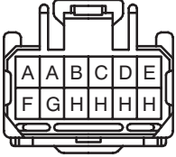
J37 Gray
