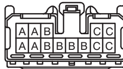
J10 (1KD-FTV, 5L-E)
