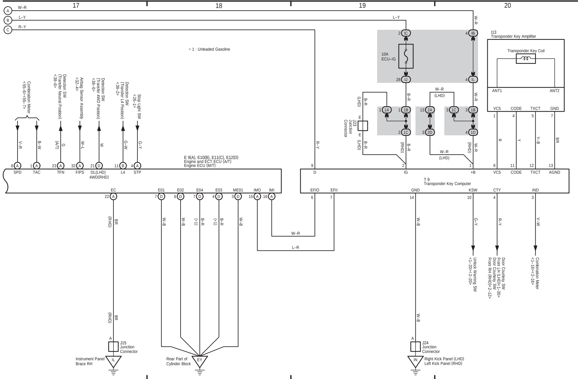
Engine Control (2TR-FE)
