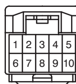
R 7 (Automatic A/C)
