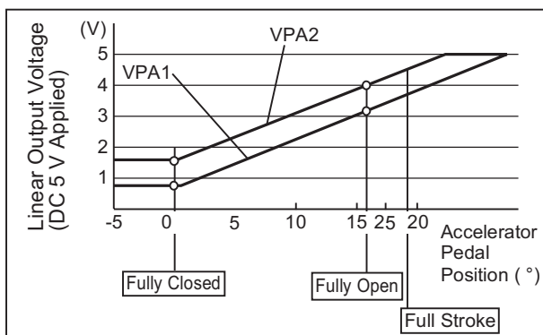
&lt; Linear Output Characteristics Graph &gt;
