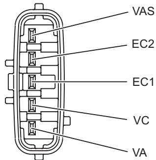
< Connector Pin Layout >
