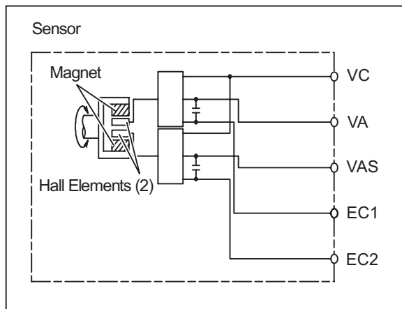
< Wiring Diagram >
