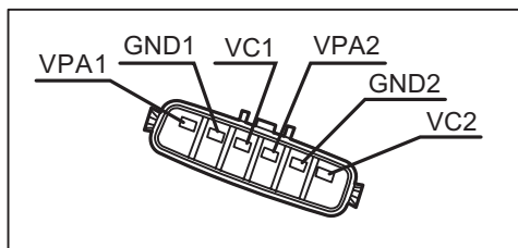
&lt; Connector Pin Layout &gt;
