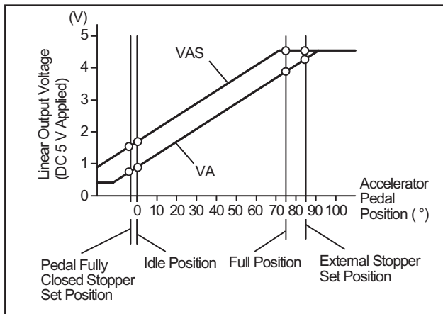
< Linear Output Characteristics Graph >
