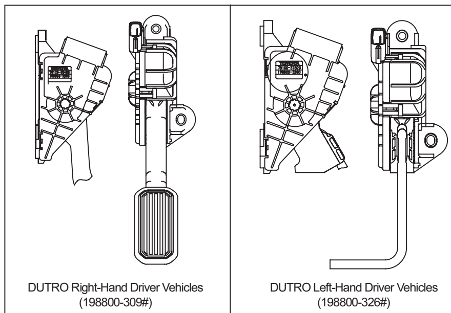
&lt; External View &gt;
