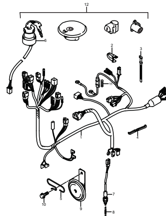
FIG.24 (D-9) WIRING HARNESS
