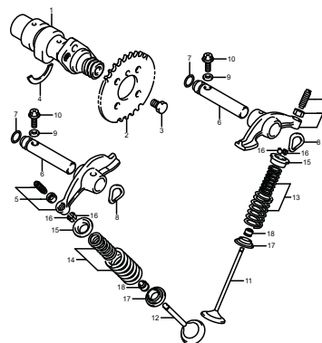
FIG.7 (B-8) CAMSHAFT / VALVE
