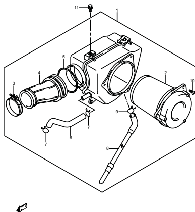
FIG.10 (B-11) AIR CLEANER
