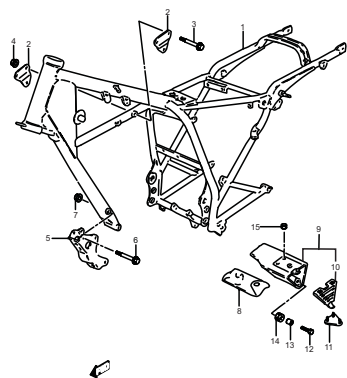
FIG.25 (E-2) FRAME
