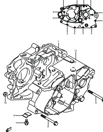
FIG.3 (B-4) CRANKCASE
