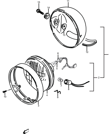
FIG.21 (D-6) HEADLAMP
