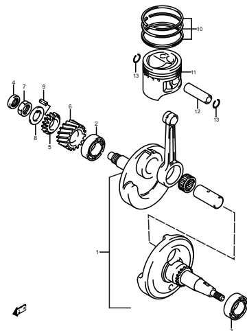
FIG.5 (B-6) CRANKSHAFT
