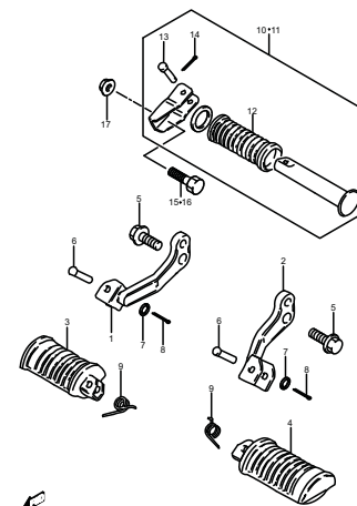
FIG.28 (E-5) FOOTREST
