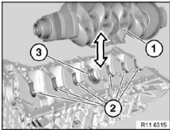
Fig. 97: Bearing Shells
