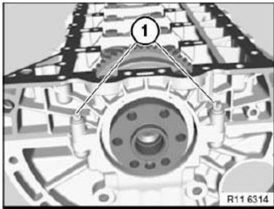
Fig. 96: Bedplate Screws
