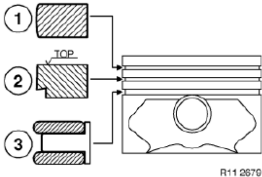
Fig. 191: Piston Rings Installation Position
