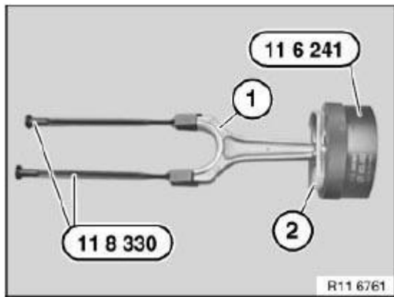
Fig. 182: Connecting Rod, Piston And Special Tools (11 8 330) And (11 6 241) Courtesy of BMW OF NORTH AMERICA, INC.
