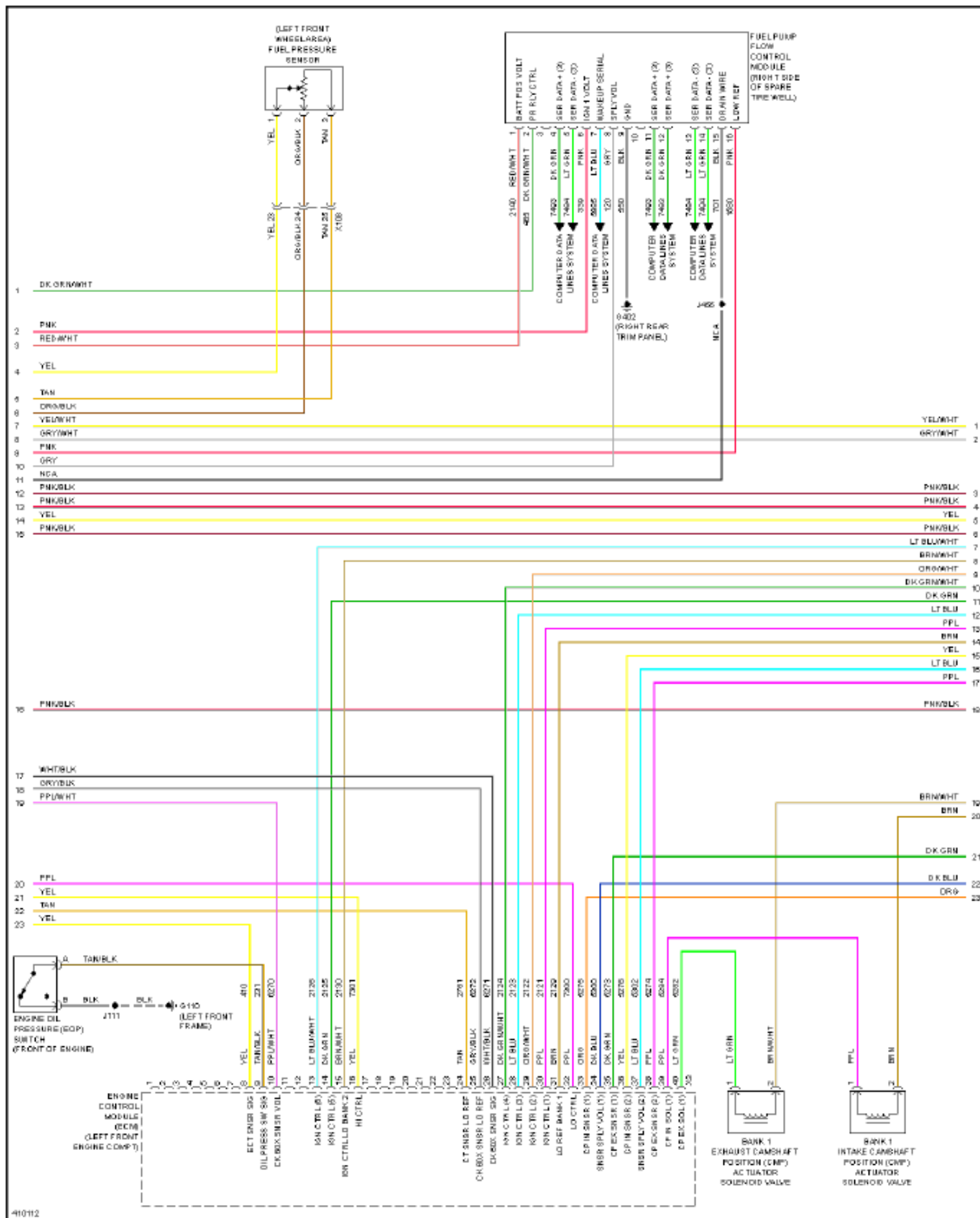
Fig. 26: 3.0L VIN 5, Engine Performance Circuit (3 of 6)
