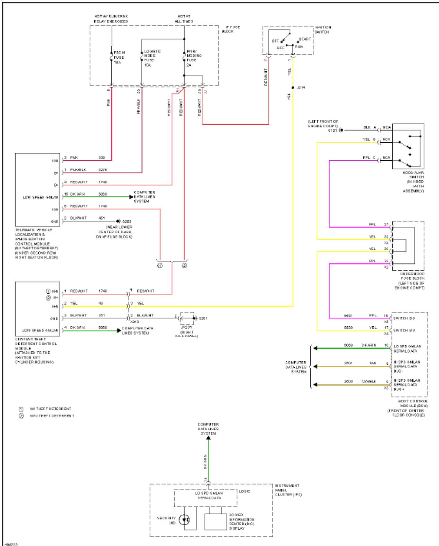
Fig. 9: Passlock Circuit
