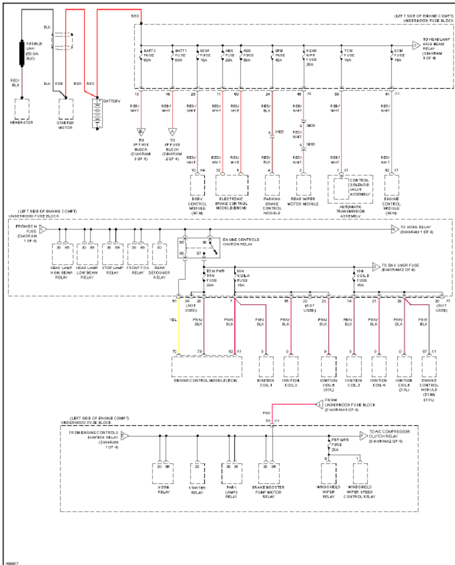
SYSTEM WIRING DIAGRAMS Fig. 45: Power Distribution Circuit (1 of 4)
