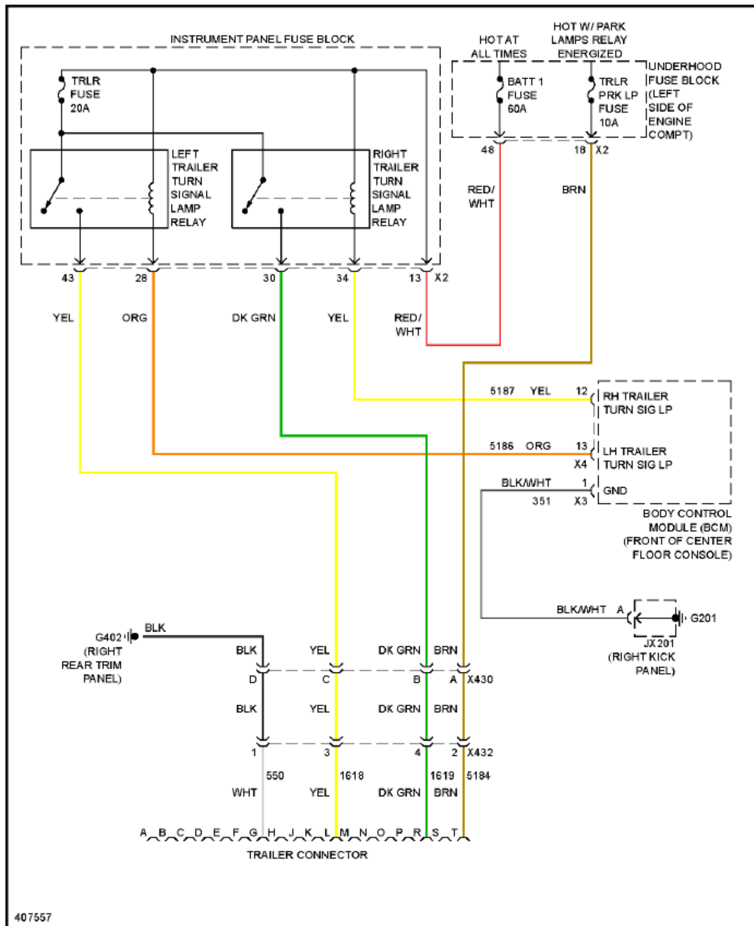
Fig. 33: Trailer Tow Circuit
