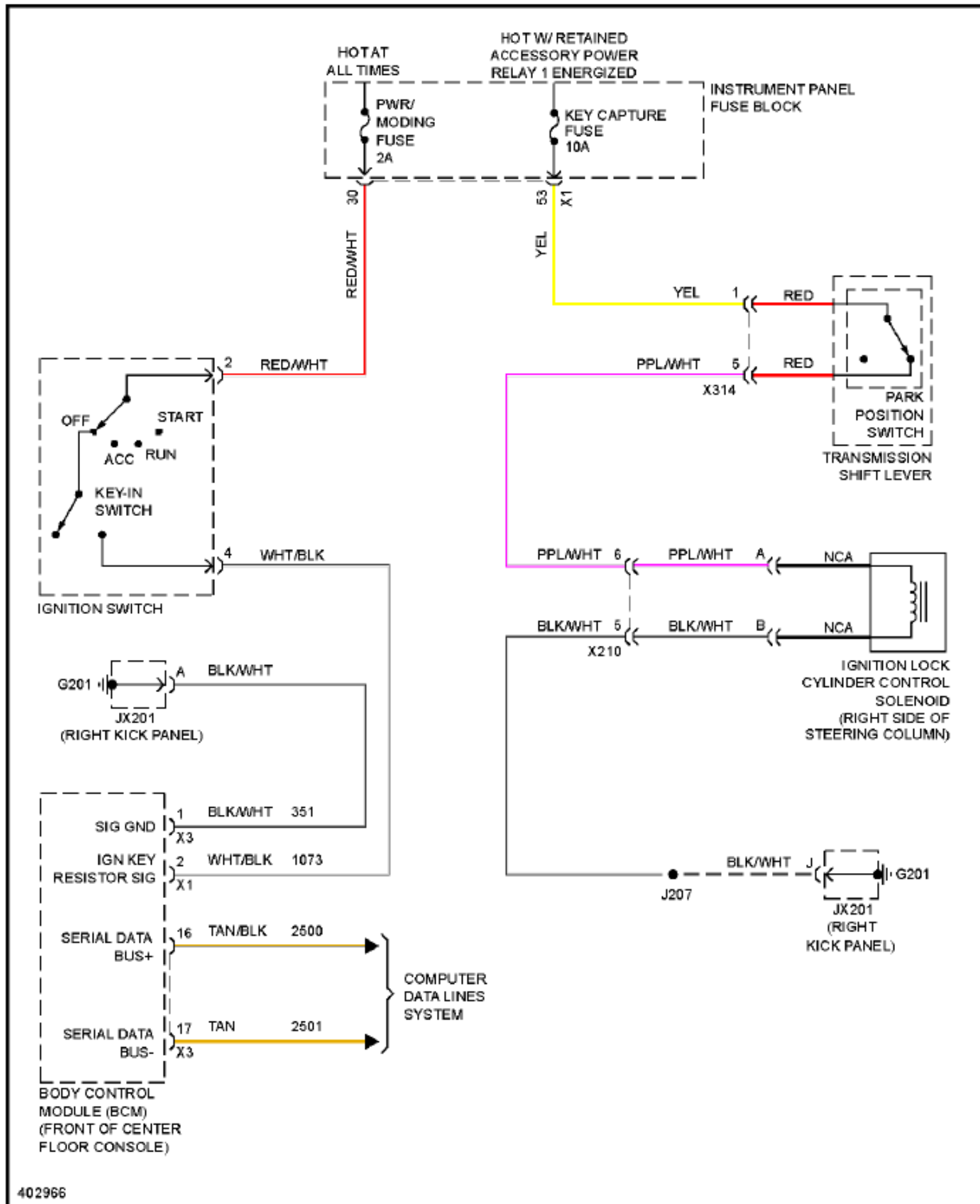
Fig. 61: Ignition Lock Solenoid Circuit
