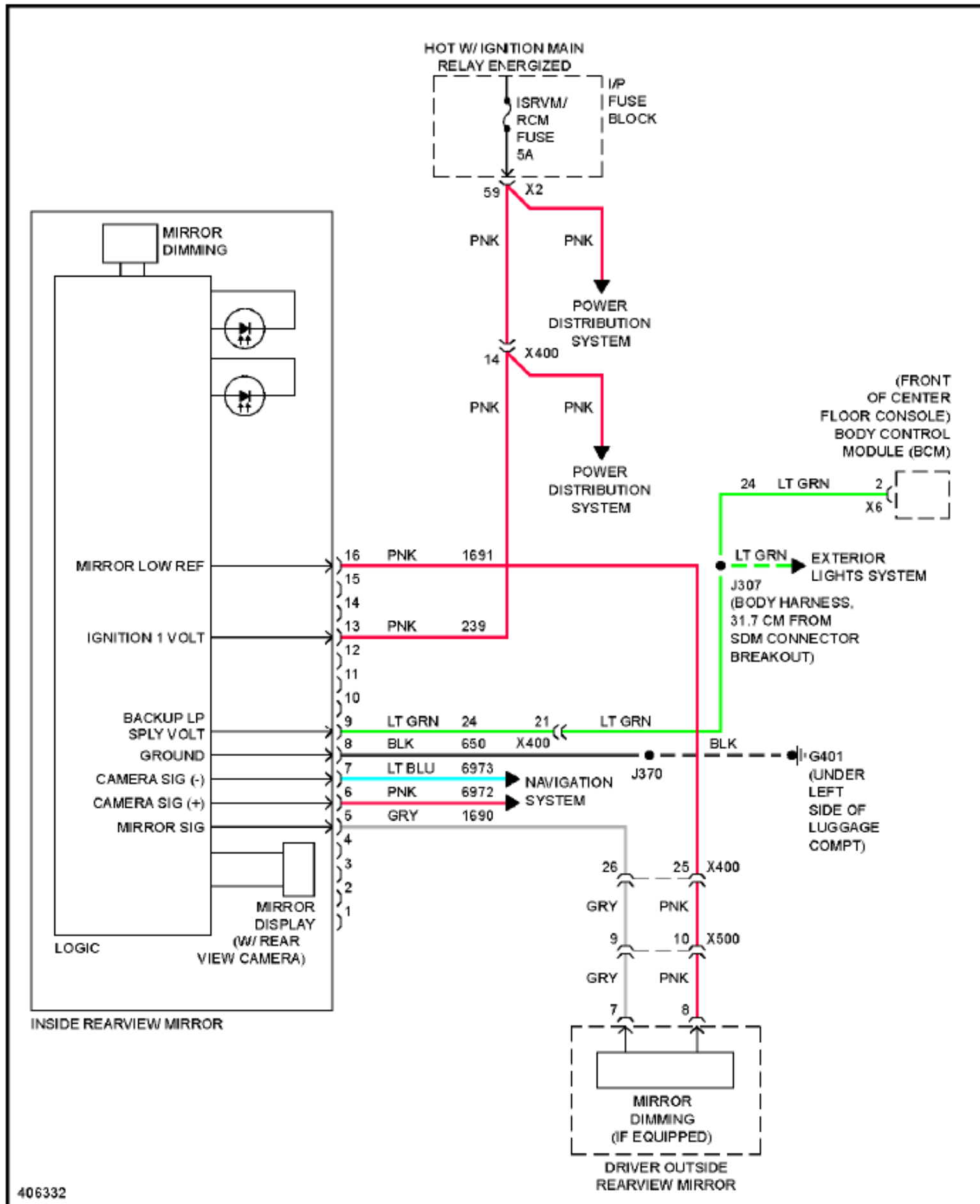
Fig. 51: Electrochromic Mirror Circuit
