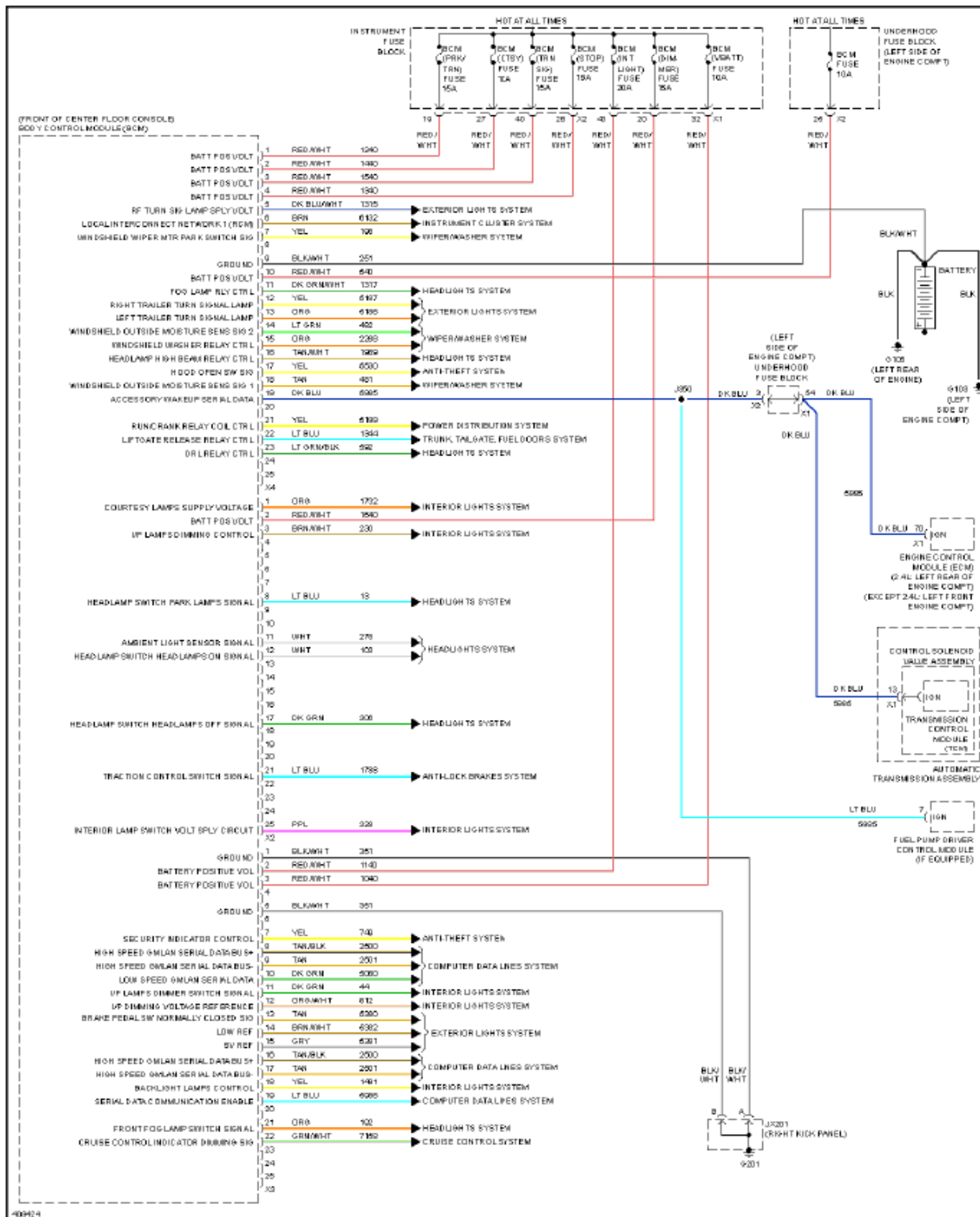
Fig. 10: Body Control Modules Circuit (1 of 2)
