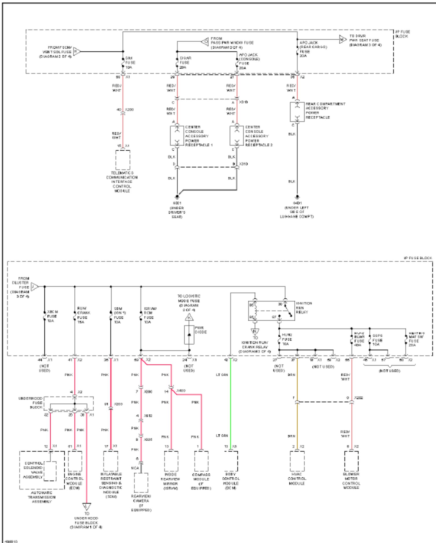
SYSTEM WIRING DIAGRAMS Fig. 48: Power Distribution Circuit (4 of 4)
