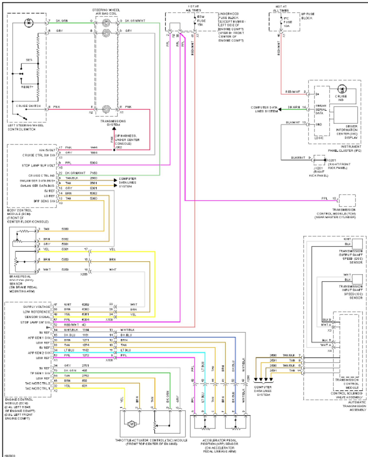
Fig. 16: Cruise Control Circuit
