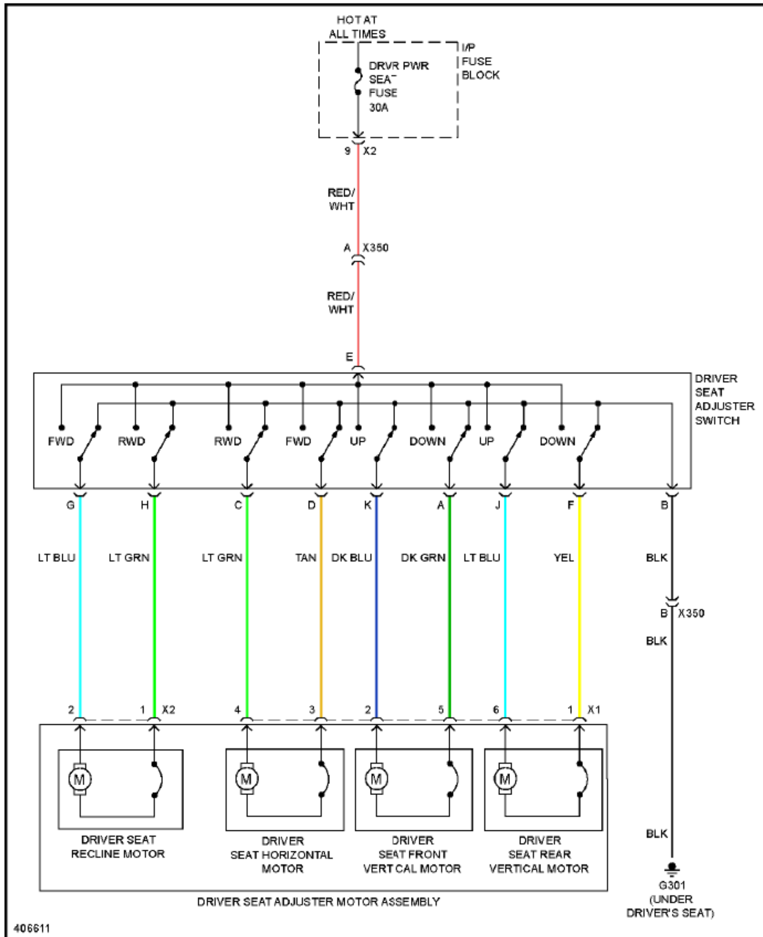
Fig. 53: Driver Seat Circuit
