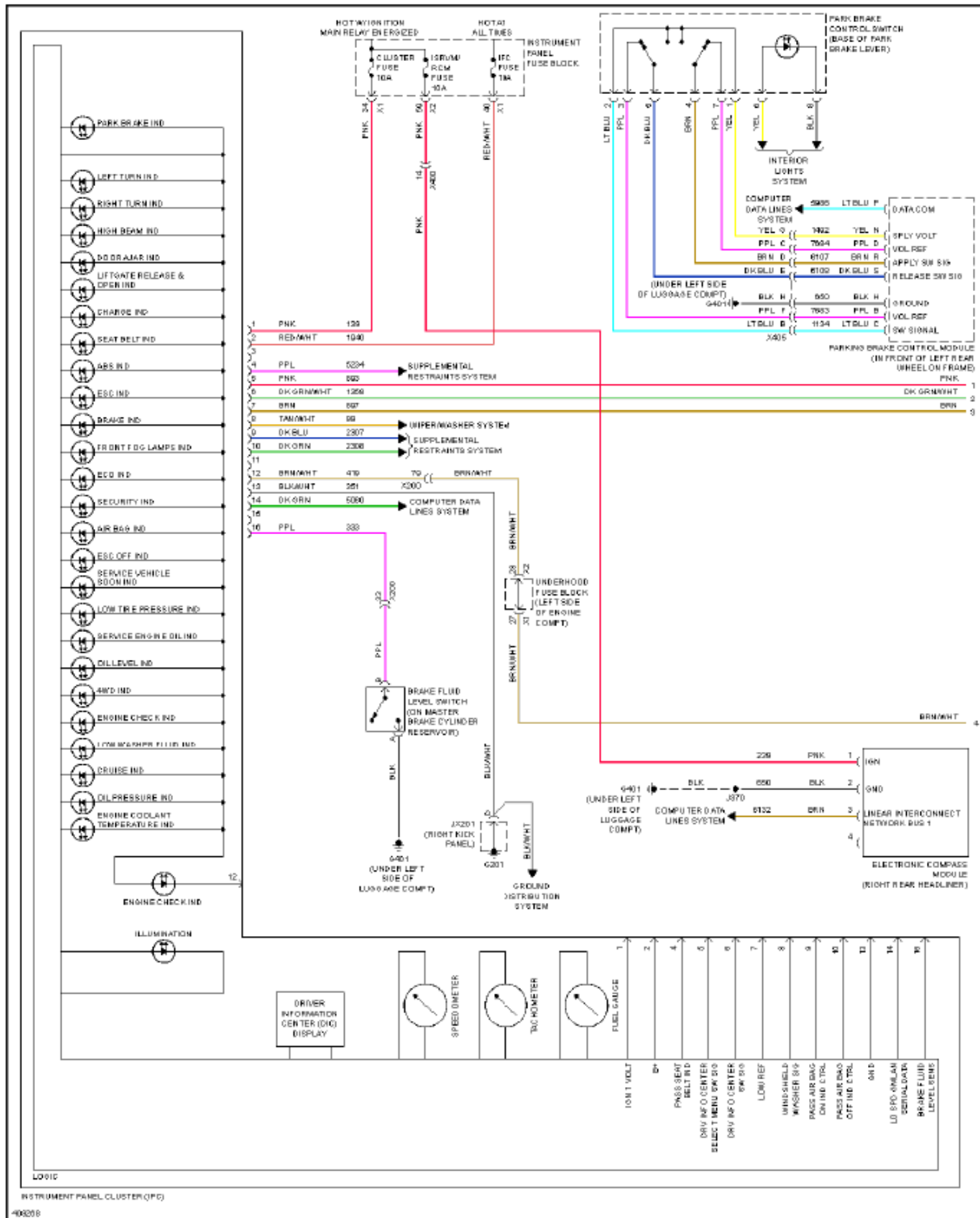
Fig. 39: Instrument Cluster Circuit (1 of 2)
