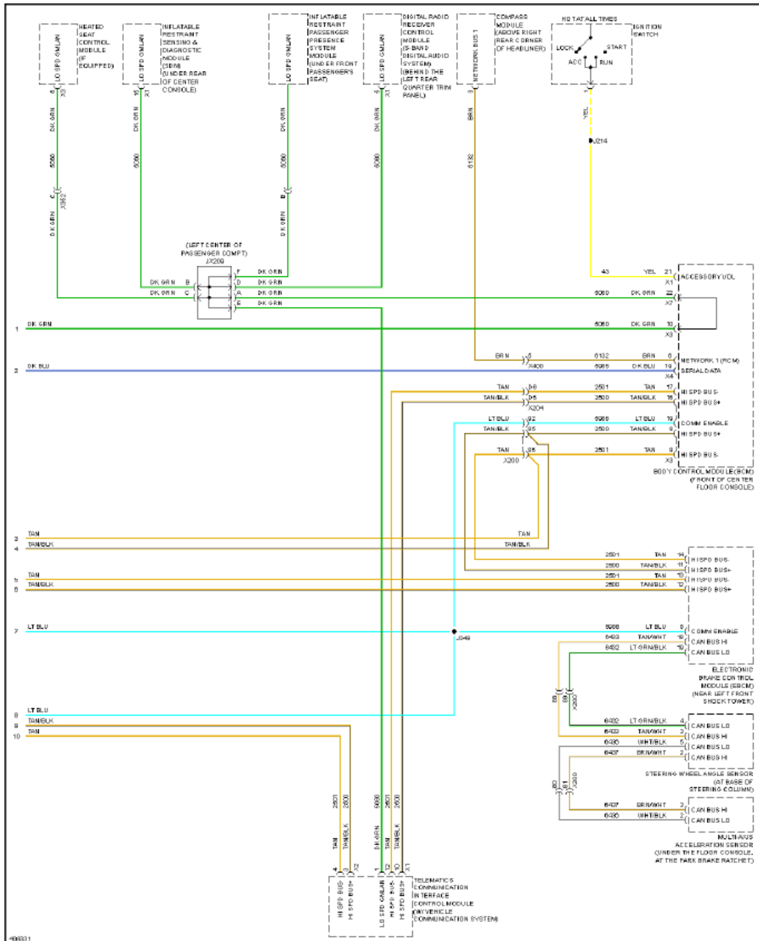
Fig. 13: Computer Data Lines Circuit (2 of 2)
