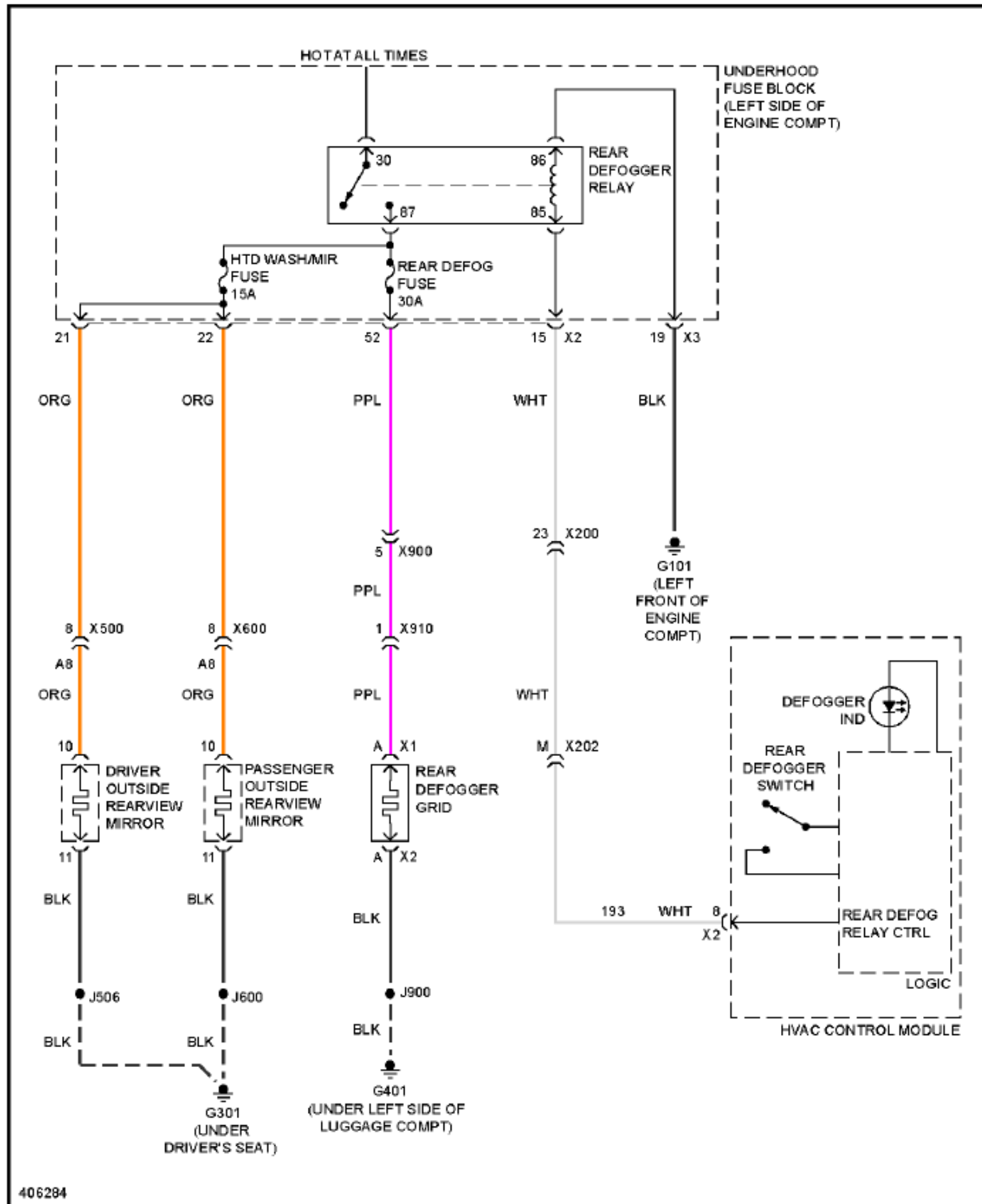
Fig. 17: Defoggers Circuit
