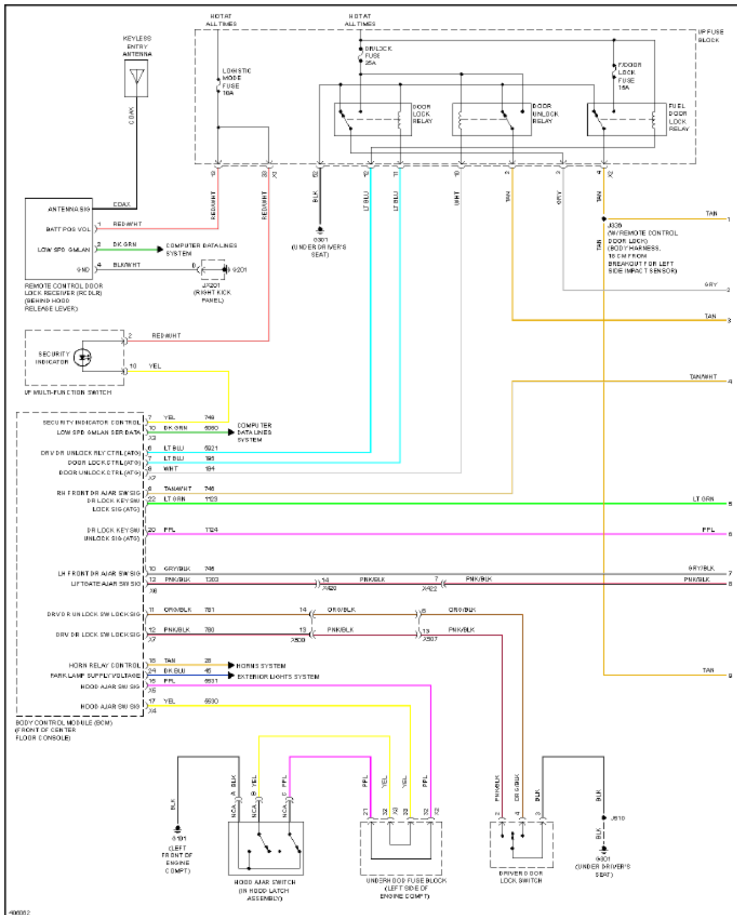
Fig. 49: Power Door Locks Circuit (1 of 2)
