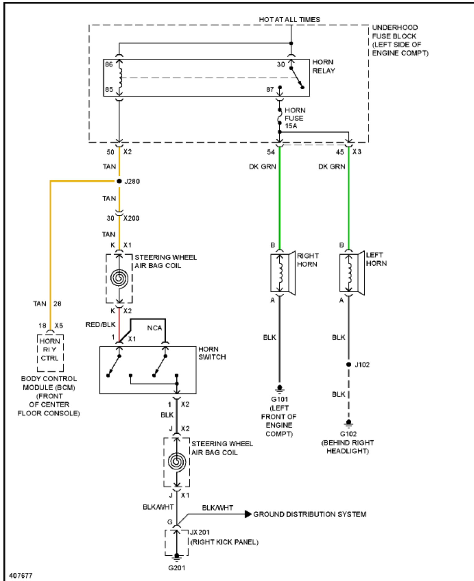
Fig. 38: Horn Circuit
