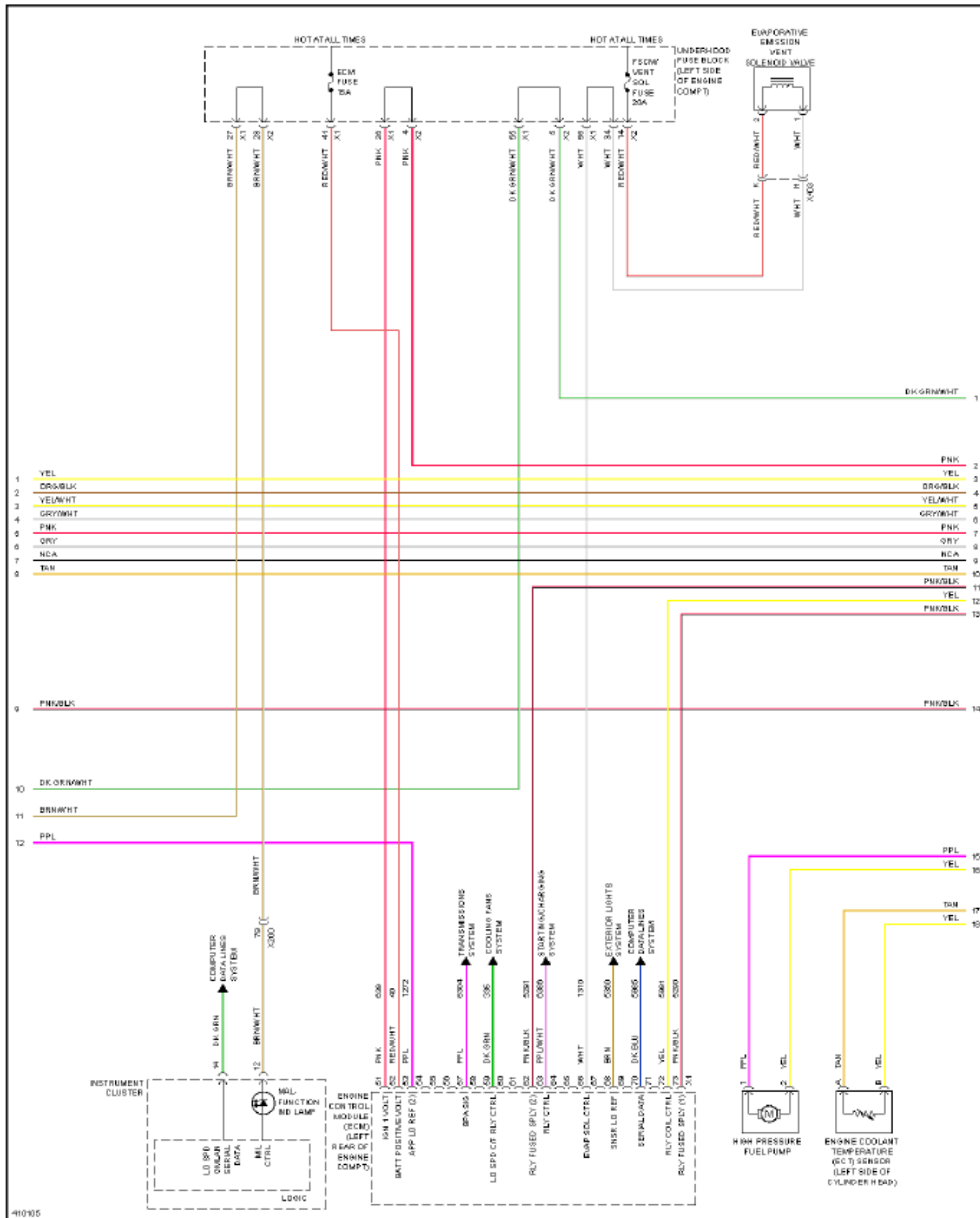
Fig. 19: 2.4L VIN K, Engine Performance Circuit (2 of 6)
