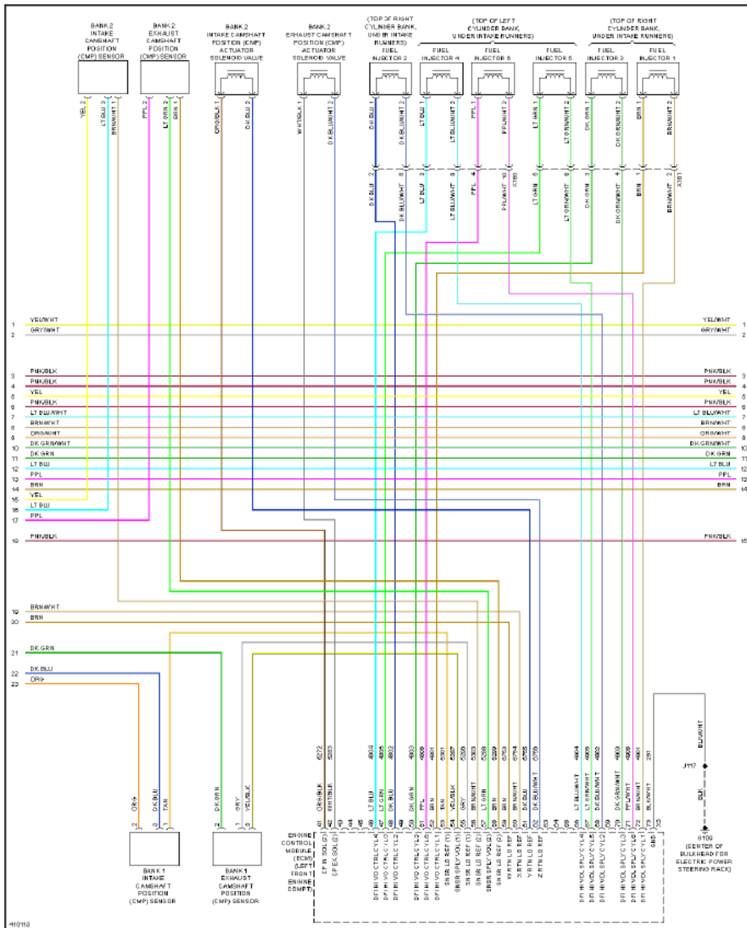
Fig. 27: 3.0L VIN 5, Engine Performance Circuit (4 of 6)
