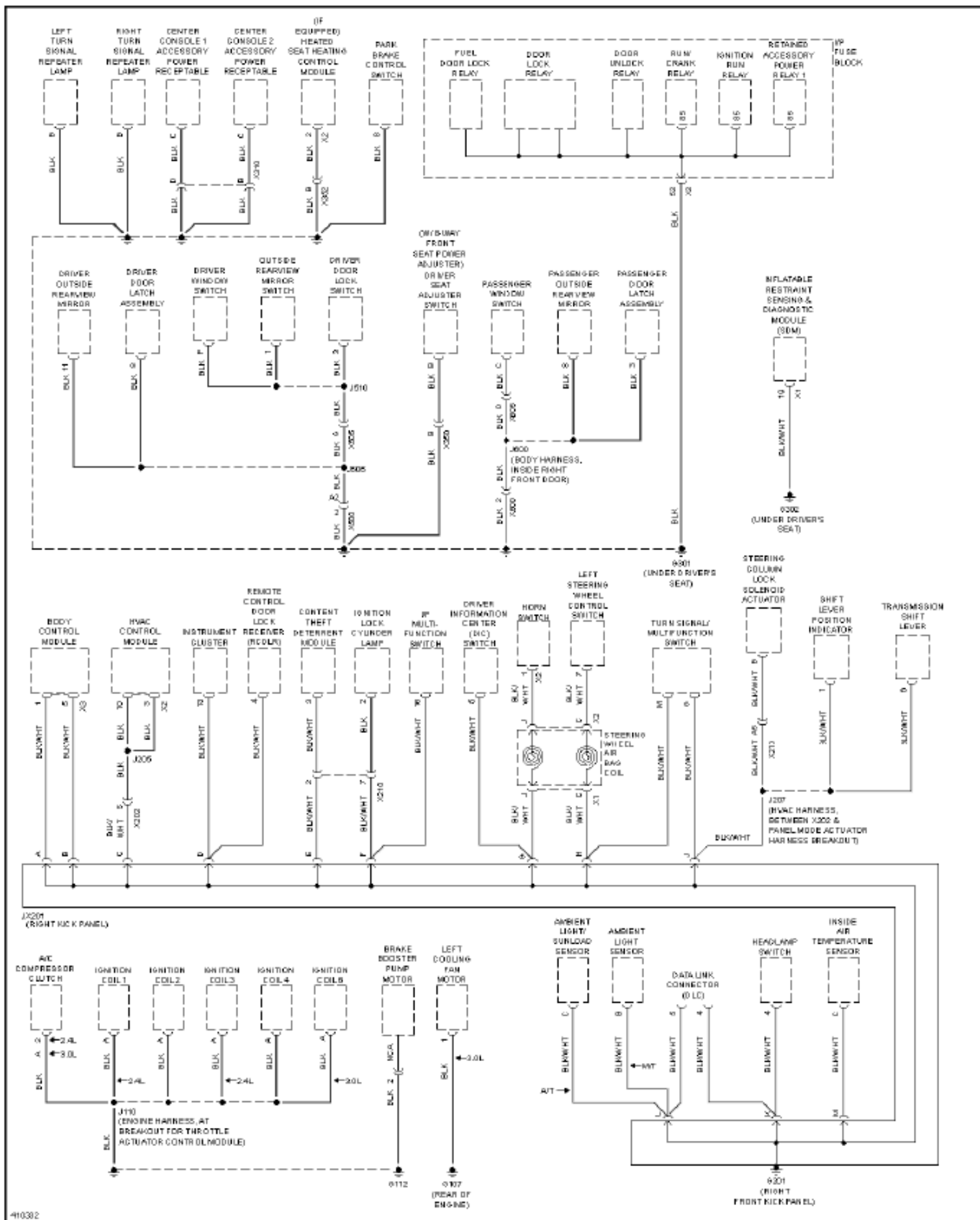
Fig. 35: Ground Distribution Circuit (2 of 3)
