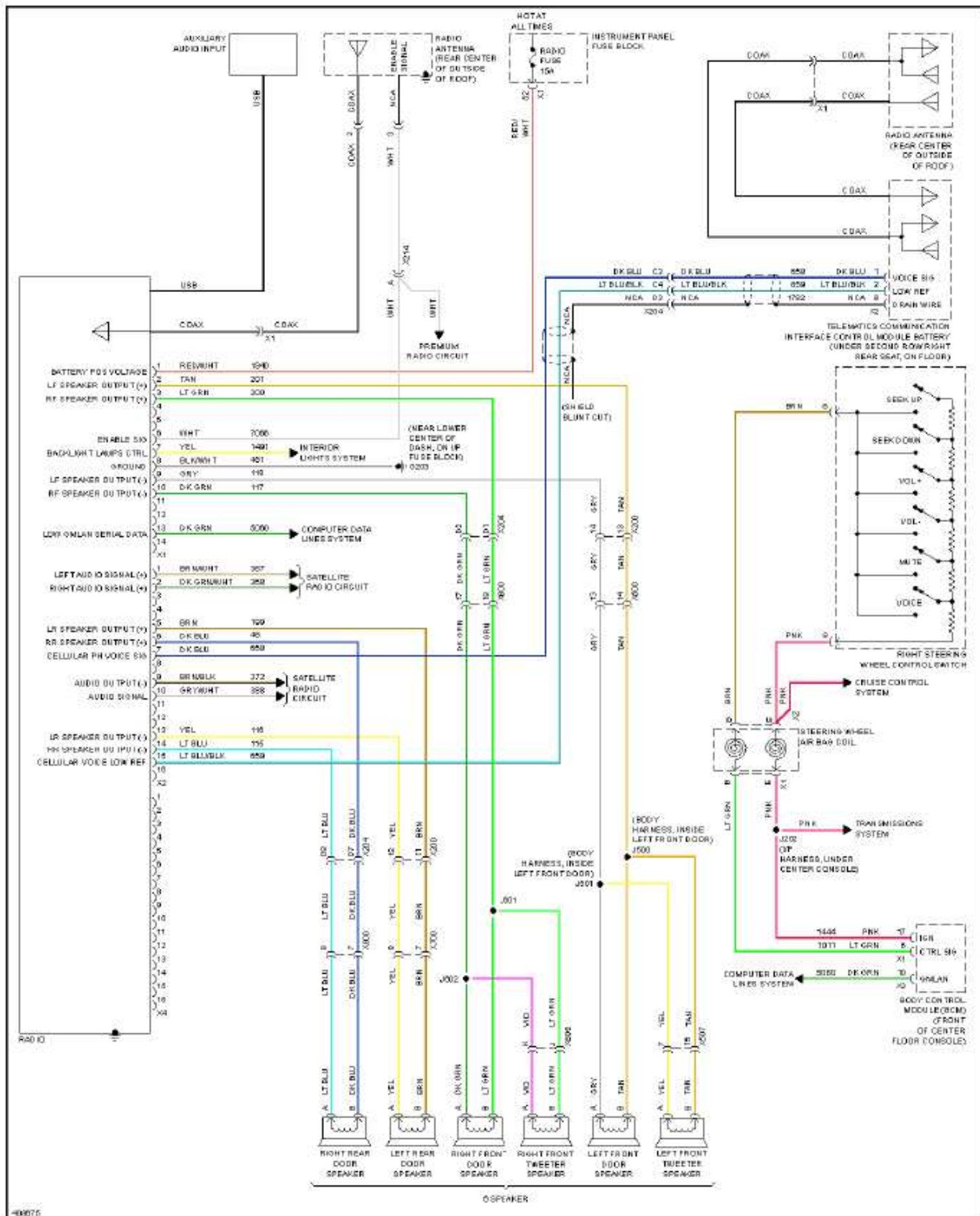
Fig. 57: Base Radio Circuit
