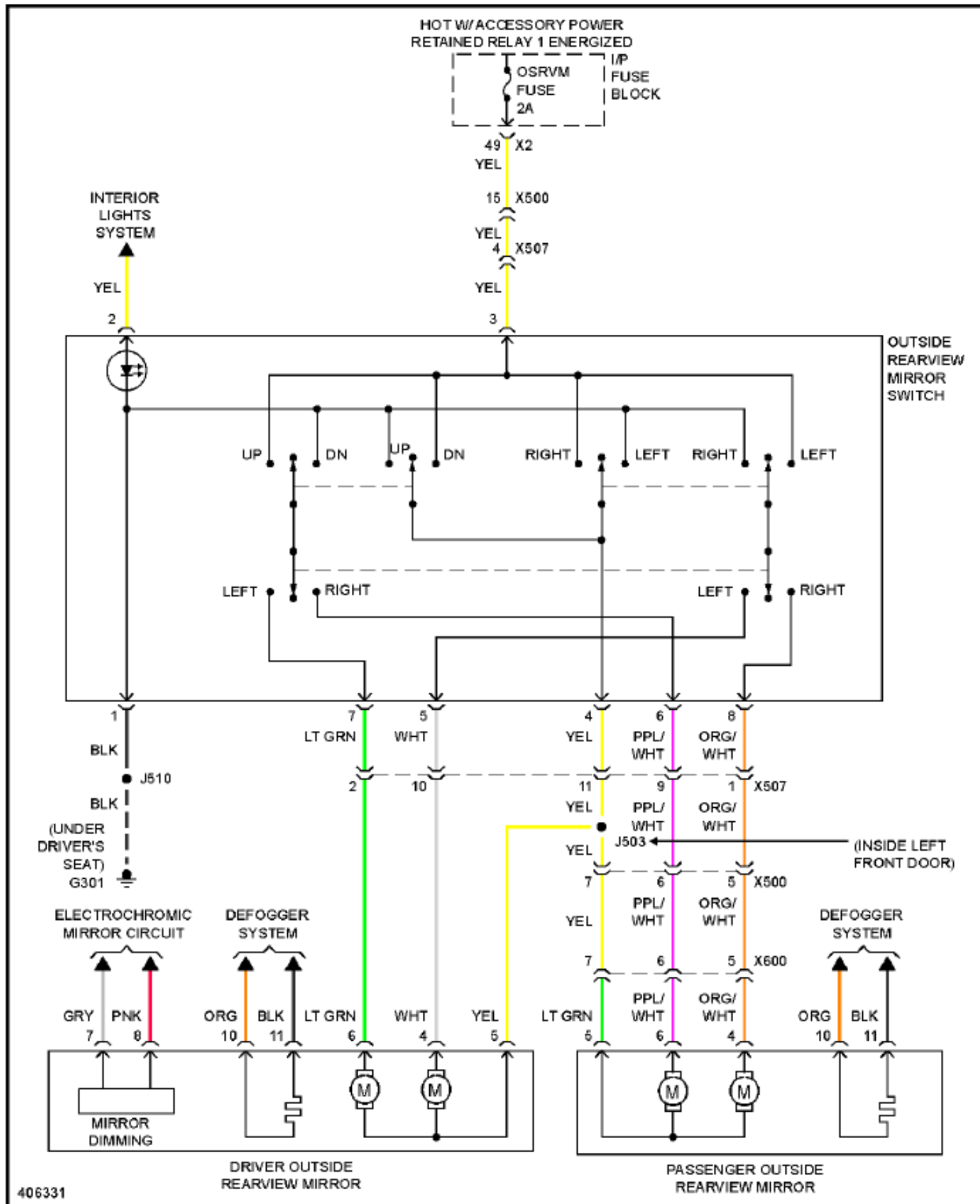
Fig. 52: Power Mirrors Circuit
