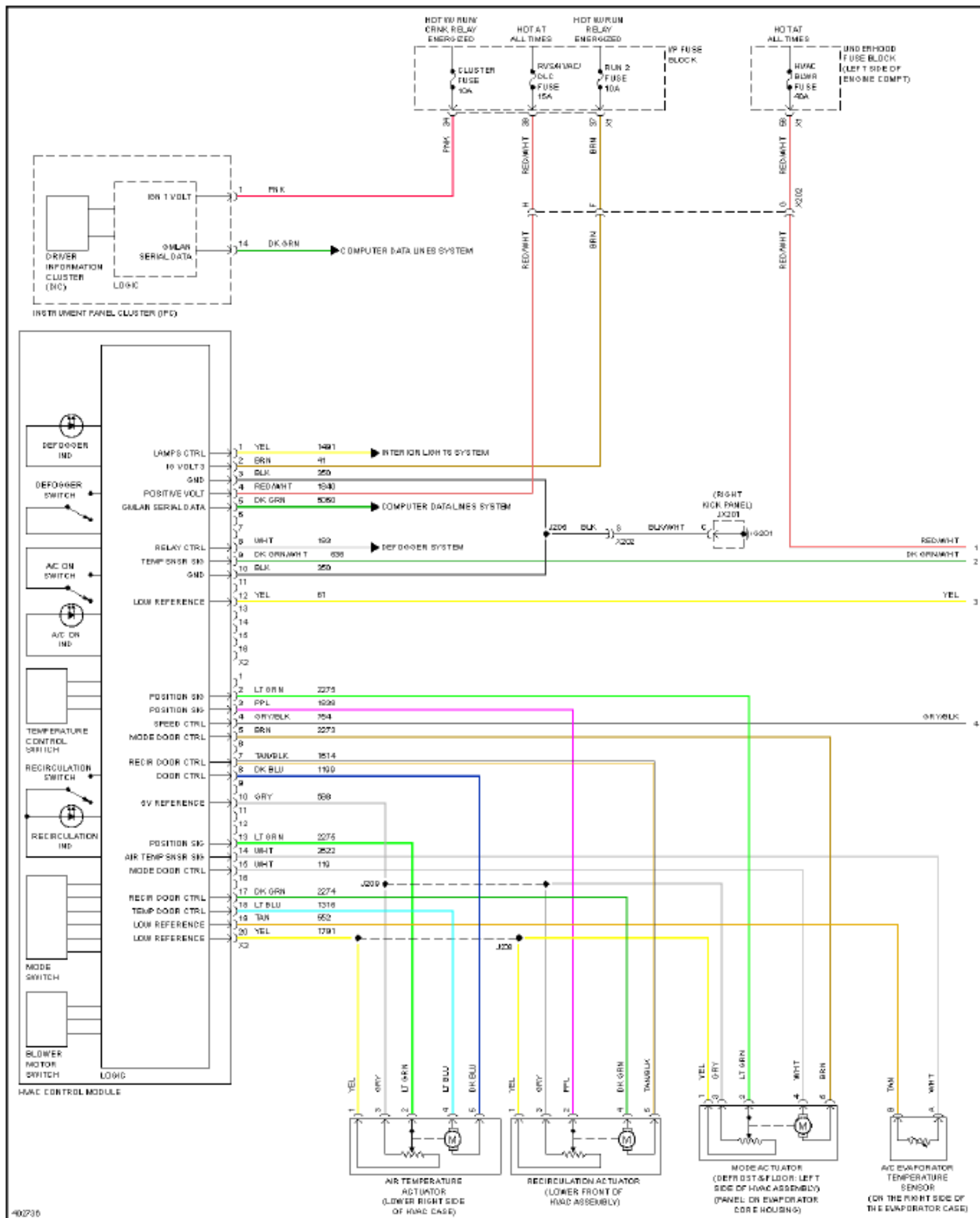
SYSTEM WIRING DIAGRAMS Fig. 3: Manual A/C Circuit (1 of 2)
