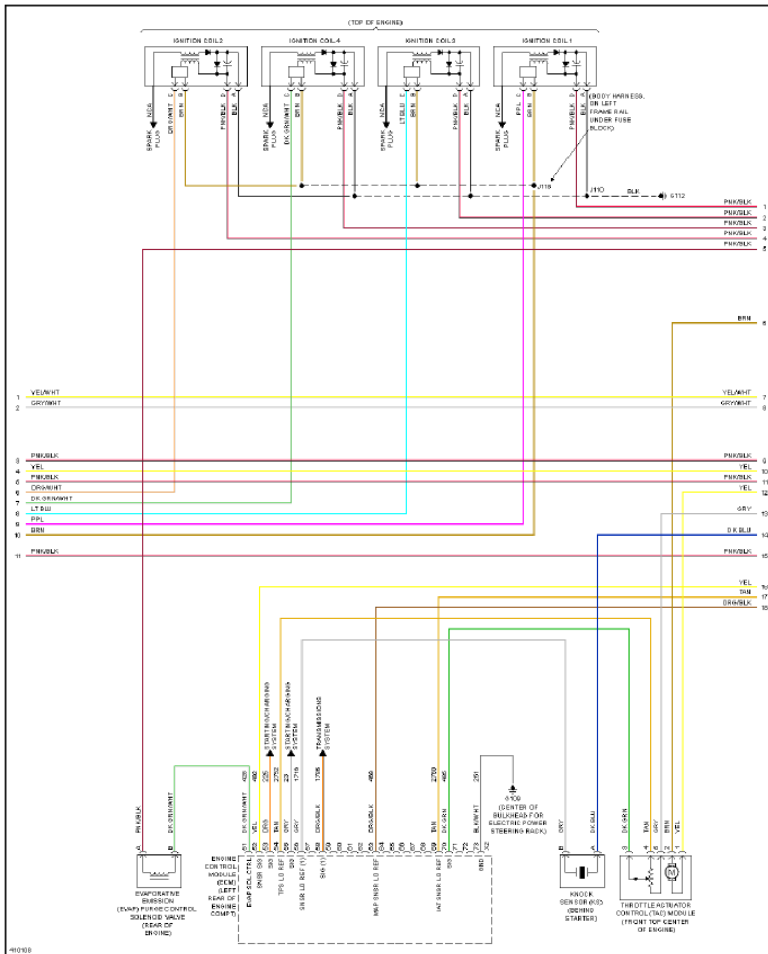
Fig. 22: 2.4L VIN K, Engine Performance Circuit (5 of 6)
