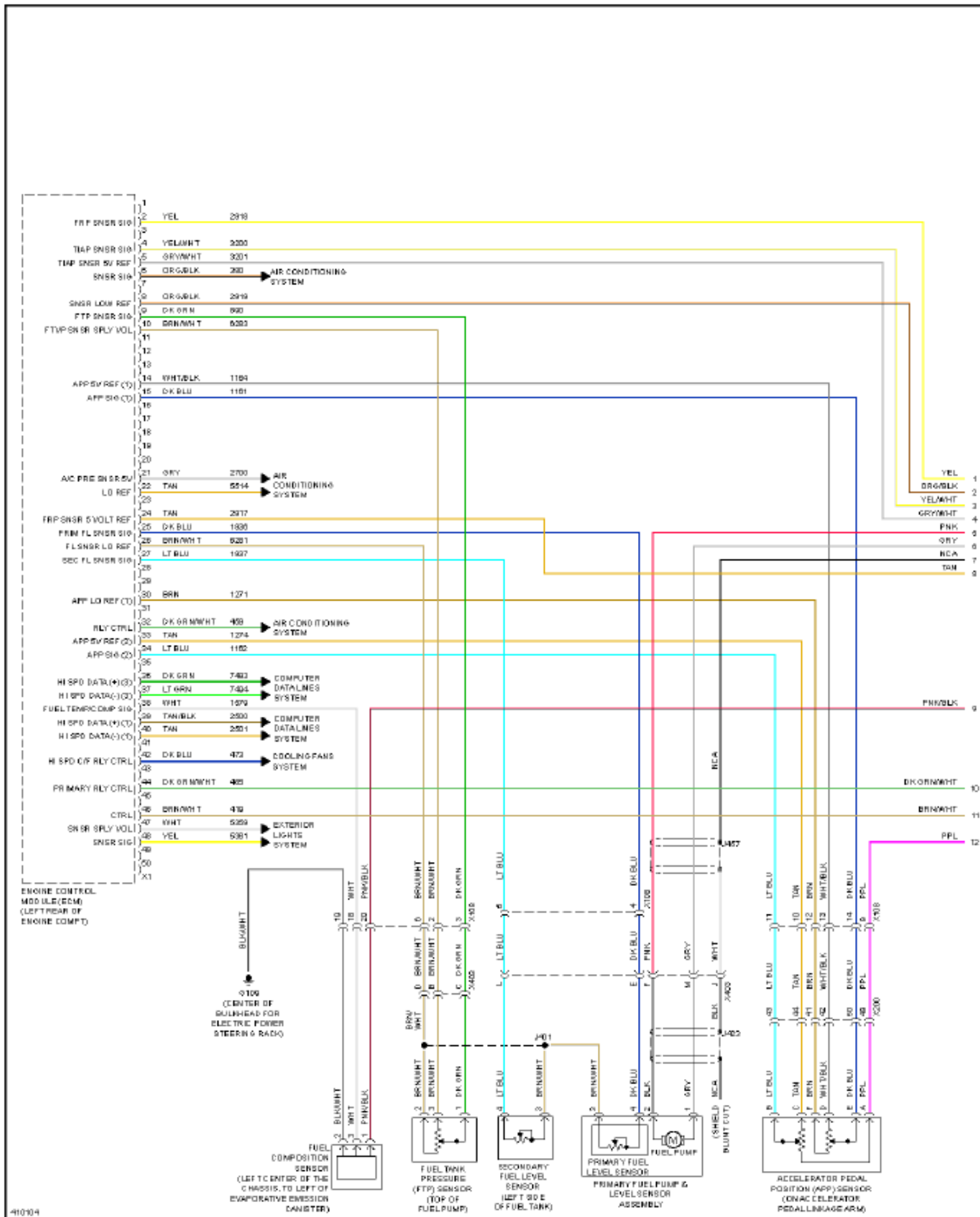
Fig. 18: 2.4L VIN K, Engine Performance Circuit (1 of 6)
