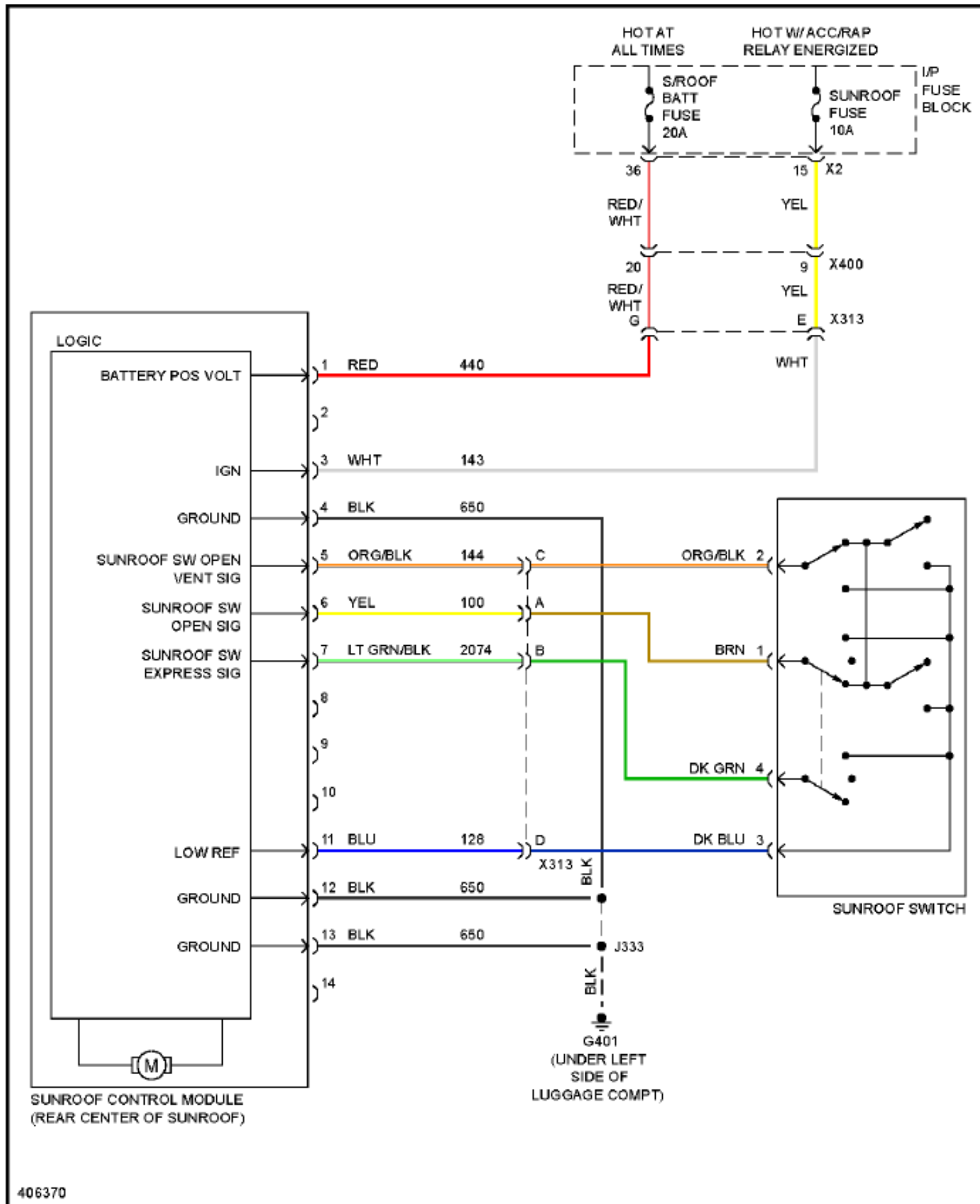
Fig. 55: Power Top/Sunroof Circuit
