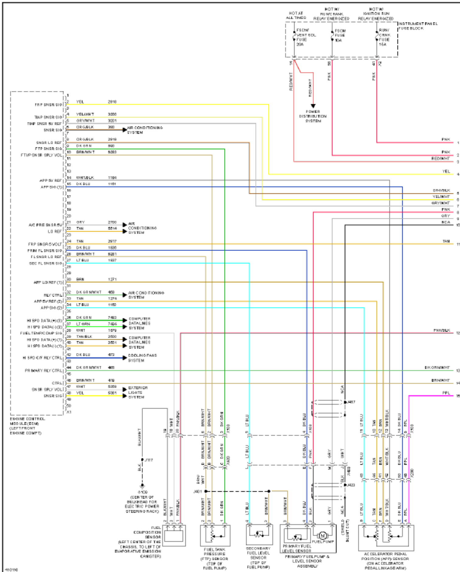
Fig. 24: 3.0L VIN 5, Engine Performance Circuit (1 of 6)
