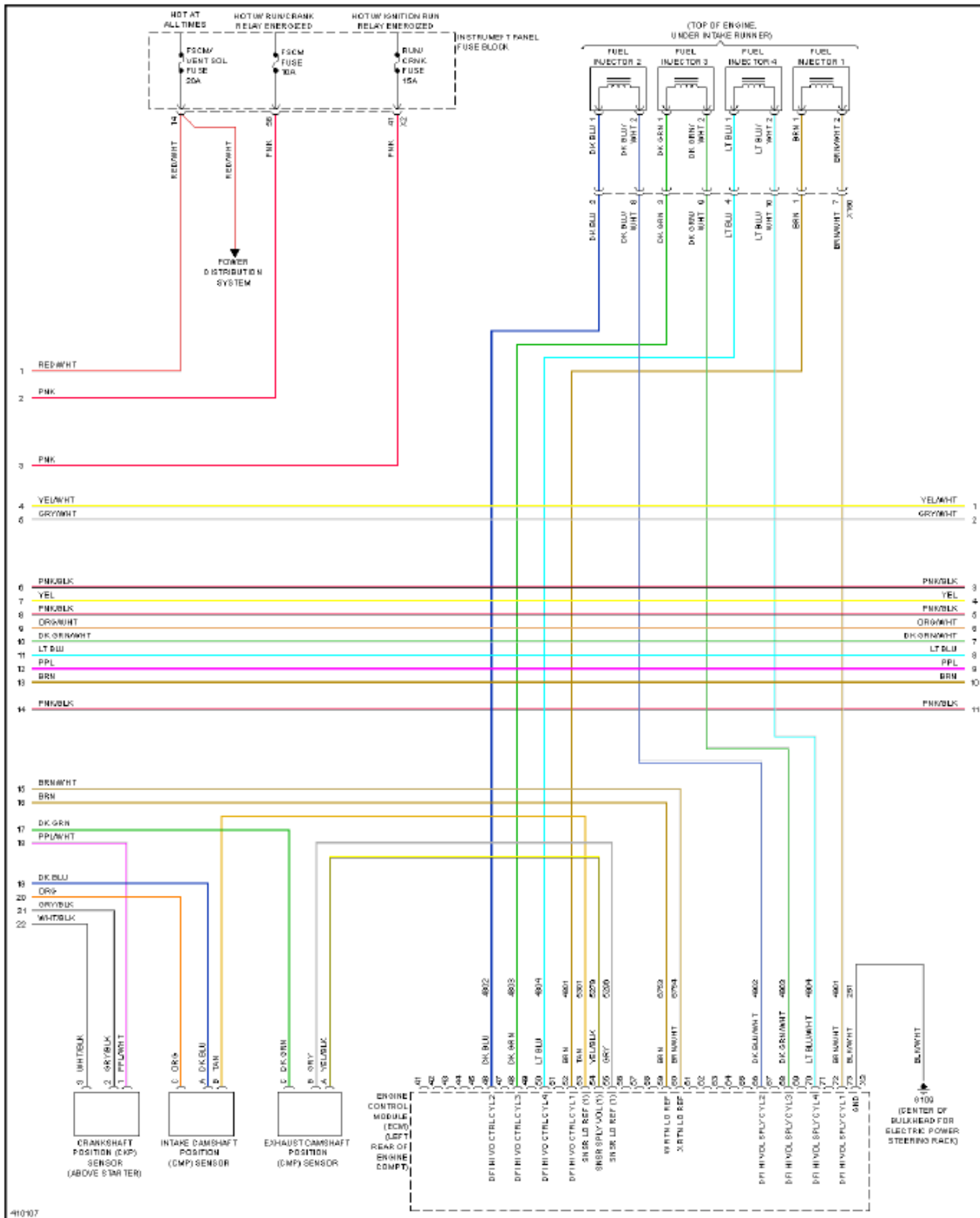
Fig. 21: 2.4L VIN K, Engine Performance Circuit (4 of 6)
