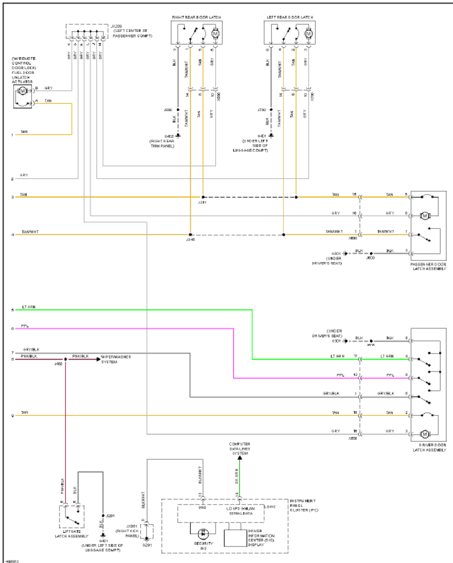
Fig. 50: Power Door Locks Circuit (2 of 2)
