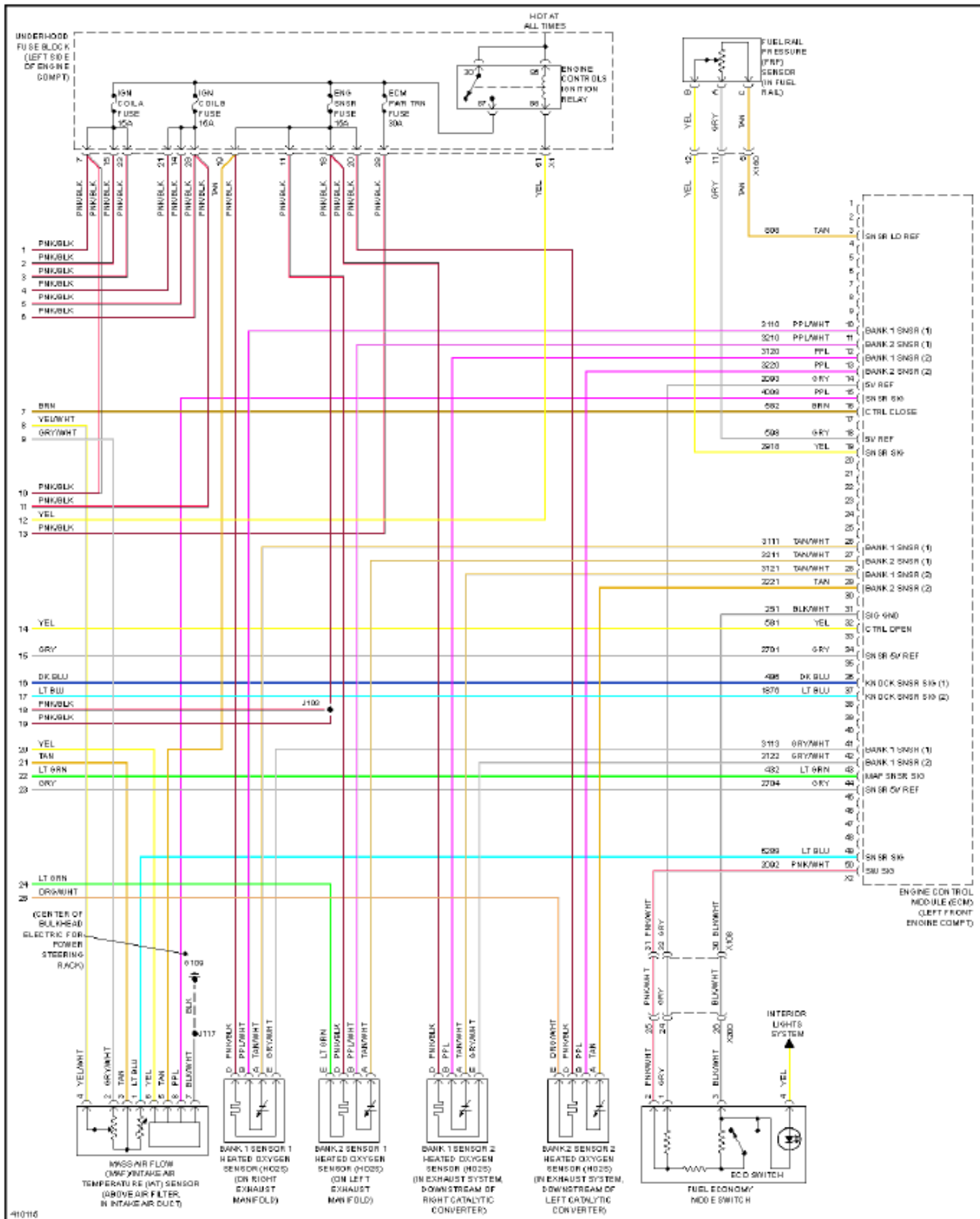
Fig. 29: 3.0L VIN 5, Engine Performance Circuit (6 of 6)
