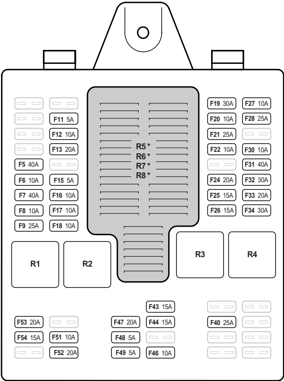
FRONT POWER DISTRIBUTION FUSE BOX * NON-SERVICEABLE PCB RELAYS
