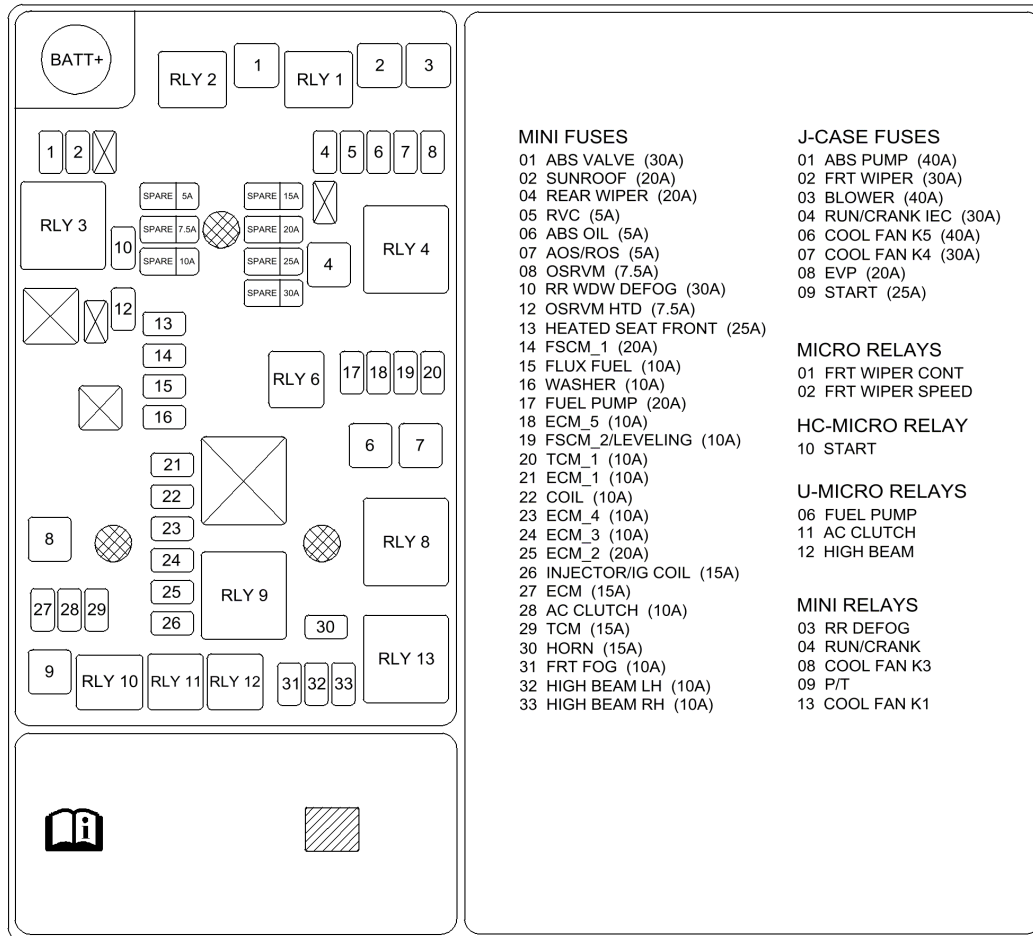
Fig. 2: X50A Fuse Block - Fuse And Relay Underhood Label (LUW) Courtesy of GENERAL MOTORS COMPANY
