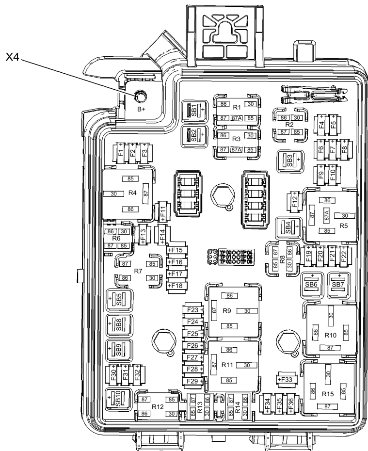
Fig. 5: X50A Fuse Block - Underhood, Top View (LWE)
