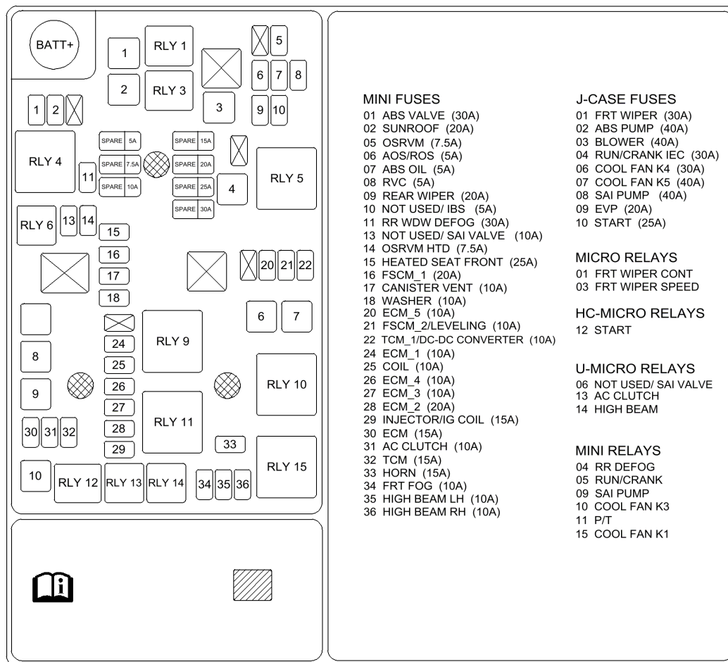
Fig. 3: X50A Fuse Block - Fuse And Relay Underhood Label (LWE) Courtesy of GENERAL MOTORS COMPANY
