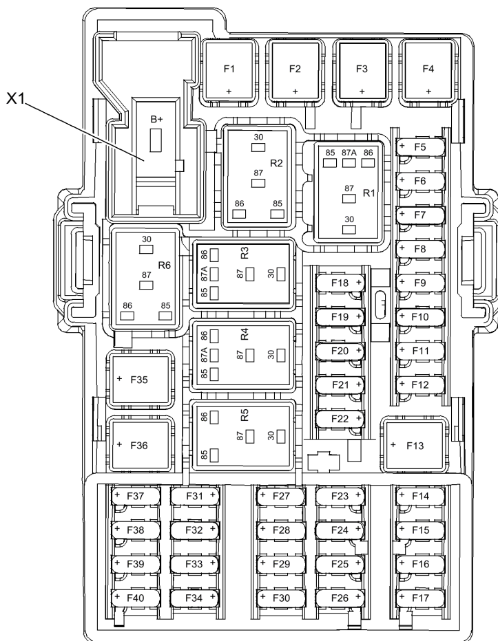
Fig. 9: X51A Fuse Block -- Instrument Panel, Top View Courtesy of GENERAL MOTORS COMPANY
