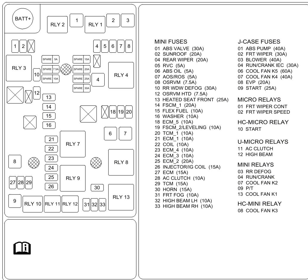
Fig. 1: X50A Fuse Block - Fuse And Relay Underhood Label (LUV) Courtesy of GENERAL MOTORS COMPANY
