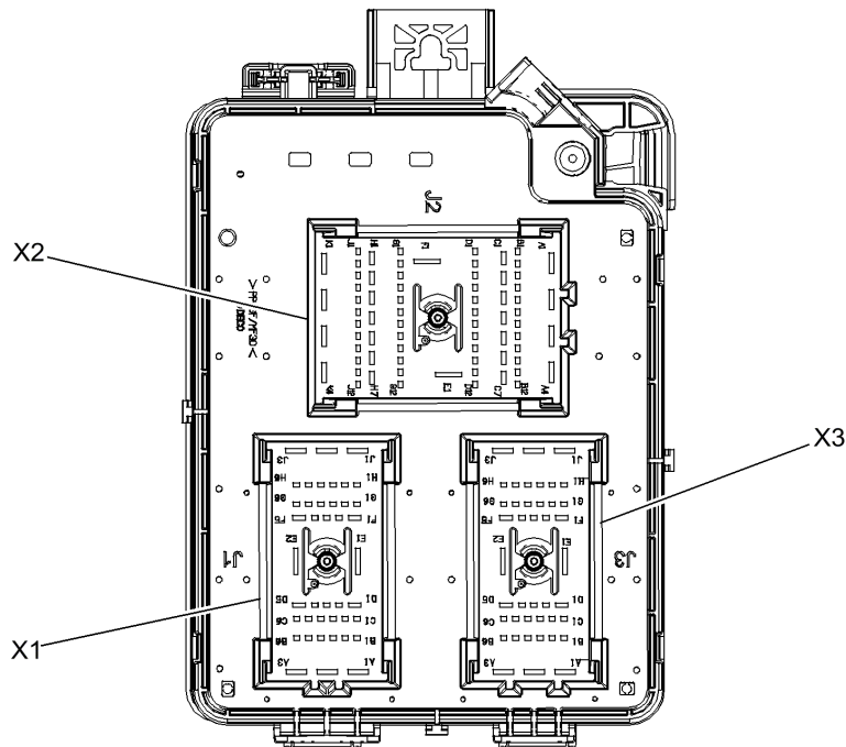
Fig. 6: X50A Fuse Block -- Underhood, Bottom View Courtesy of GENERAL MOTORS COMPANY
