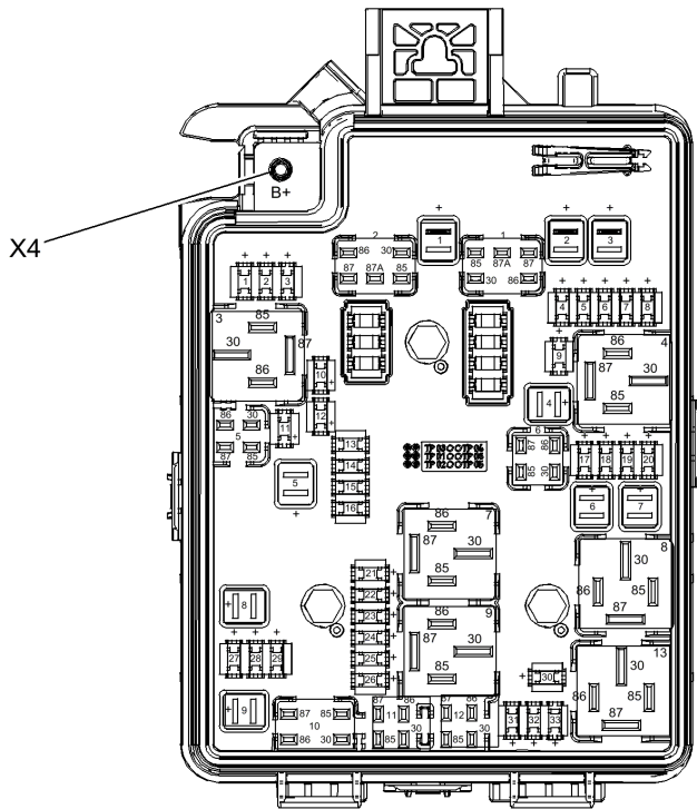
Fig. 4: X50A Fuse Block - Underhood, Top View (LUV or LUW) Courtesy of GENERAL MOTORS COMPANY
