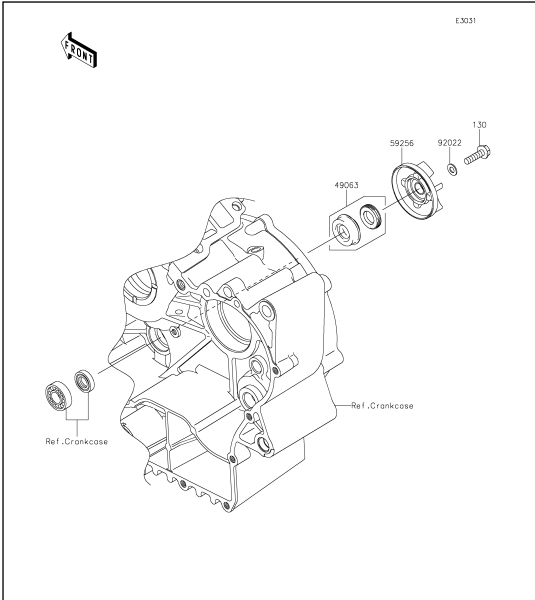
25 Water Pump
