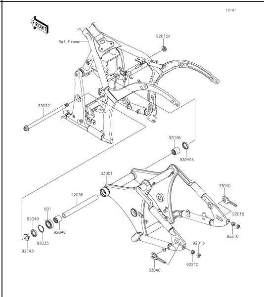
31 Swingarm
