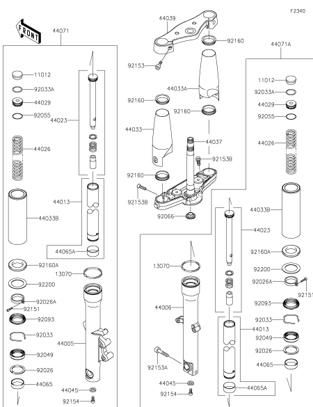
45 Front Fork
