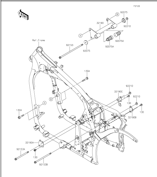
29 Engine Mount
