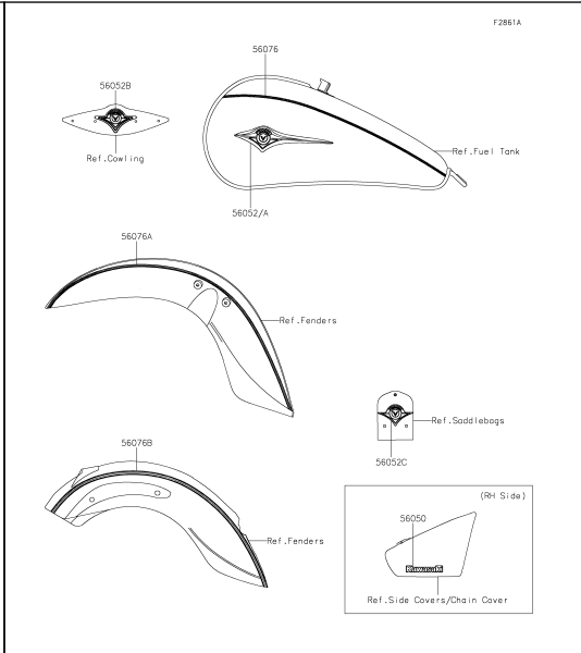
59 Decals(DPFNN/DPFNL)
