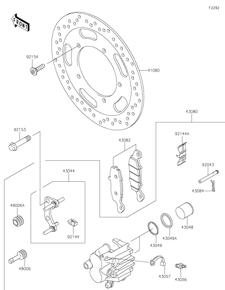
41 Front Brake
