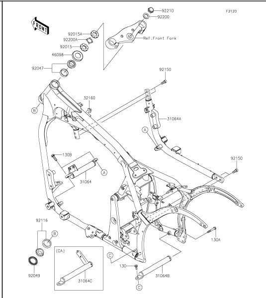
28 Frame
