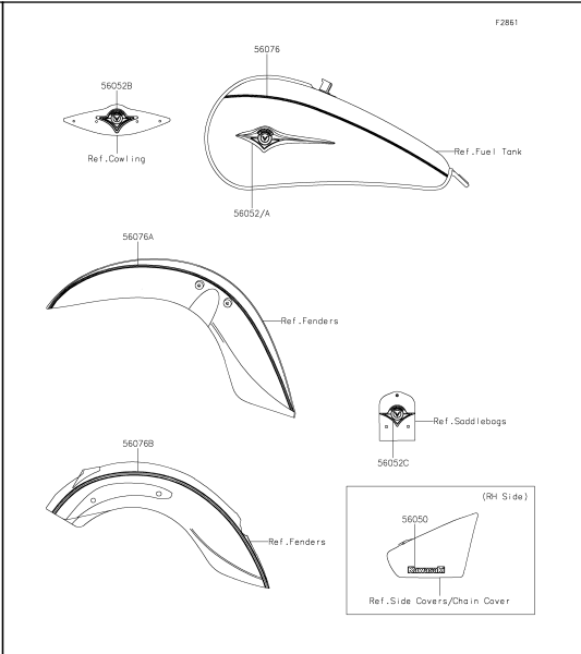
58 Decals(DNFNN/DNFNL)
