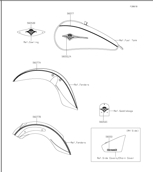
60 Decals(DRFNN/DRFNL)
