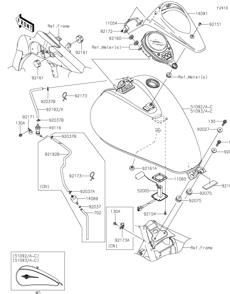
46 Fuel Tank
