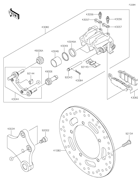
43 Rear Brake
