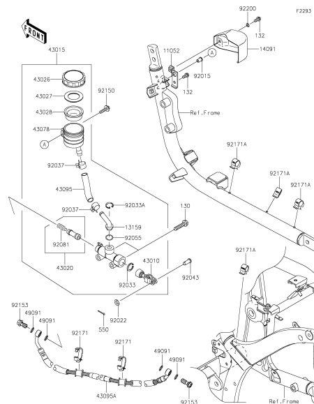
42 Rear Master Cylinder
