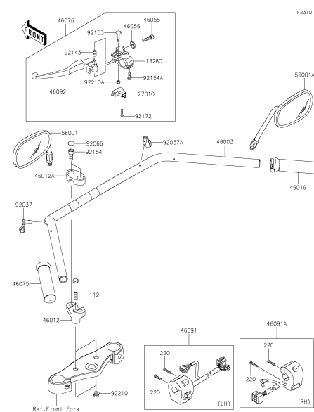
44 Handlebar
