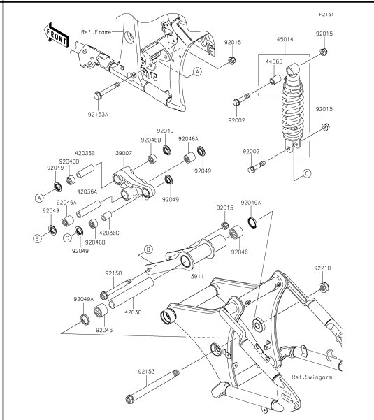
32 Suspension/Shock Absorber
