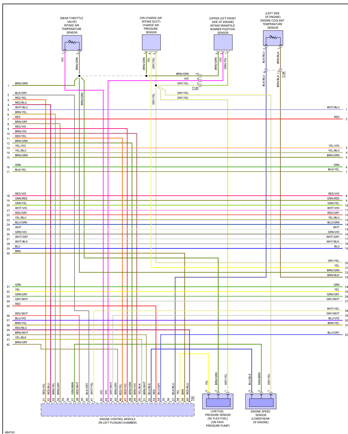
Fig 6: 2.0L Turbo, Engine Performance Circuit (6 of 7)
