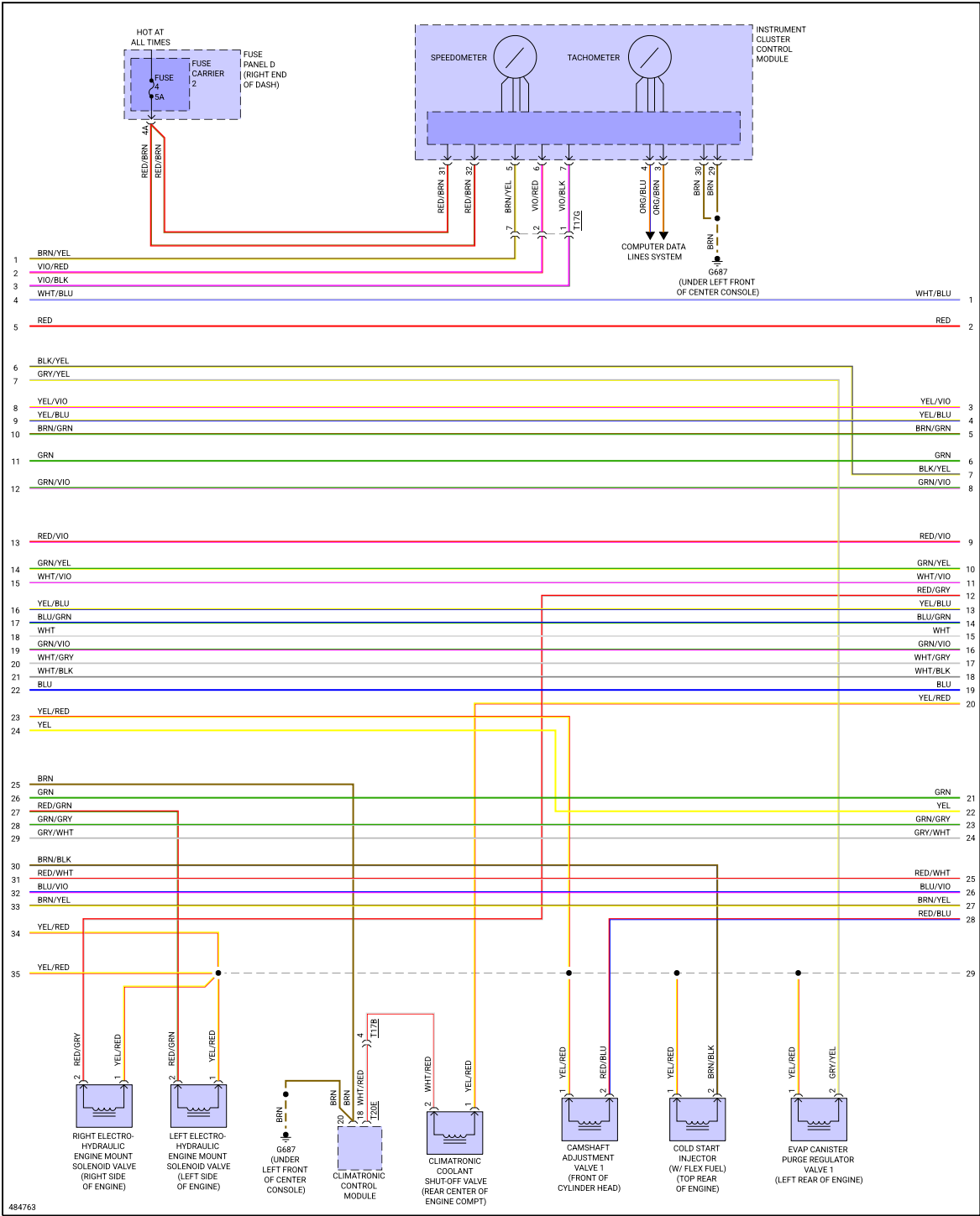
Fig 4: 2.0L Turbo, Engine Performance Circuit (4 of 7)
