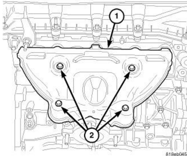
Fig. 372: Exhaust Manifold Heat Shield & Bolts Courtesy of CHRYSLER GROUP, LLC
