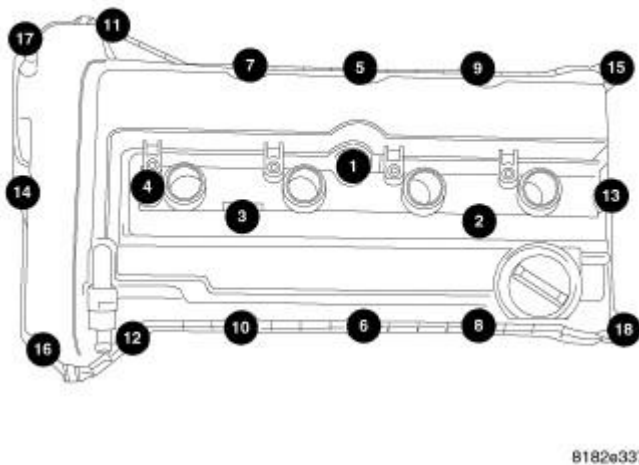
Fig. 167: Removing/Installing Cylinder Head Cover Bolts In Sequence Courtesy of CHRYSLER GROUP, LLC
