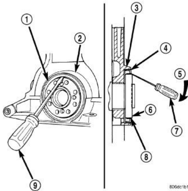
Fig. 266: Removing Rear Crankshaft Oil Seal Courtesy of CHRYSLER GROUP, LLC
