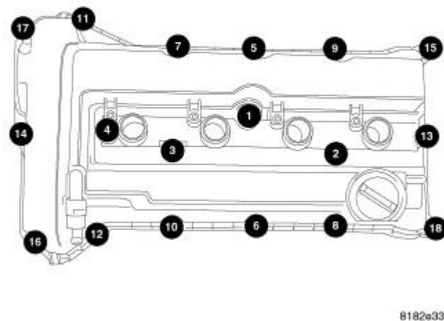
Fig. 80: Removing/Installing Cylinder Head Cover Bolts In Sequence Courtesy of CHRYSLER GROUP, LLC
