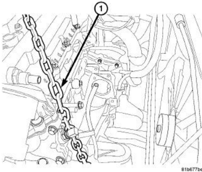
Fig. 232: Lift Chain
