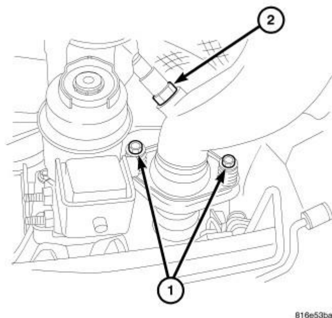
Fig. 41: Exhaust To Manifevter Bolts & Downstream Oxygen Sensor Courtesy of CHRYSLER GROUP, LLC
