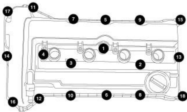
Fig. 440: Removing/Installing Cylinder Head Cover Bolts In Sequence Courtesy of CHRYSLER GROUP, LLC
