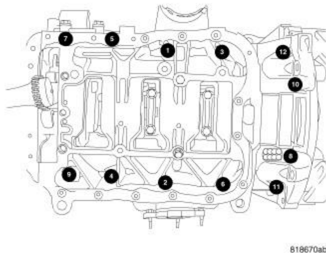
Fig. 241: Ladder Frame Bolts Tightening Sequence Courtesy of CHRYSLER GROUP, LLC
