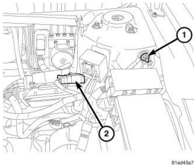
Fig. 375: Battery Cables
