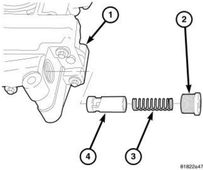
Fig. 329: Oil Pressure Relief Valve Courtesy of CHRYSLER GROUP, LLC
