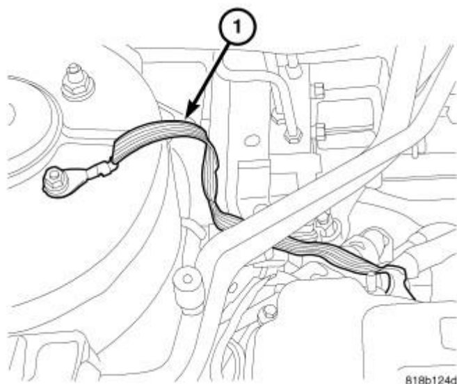
Fig. 100: Ground Strap
