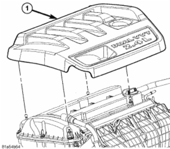
Fig. 329: Engine Cover Courtesy of CHRYSLER LLC
