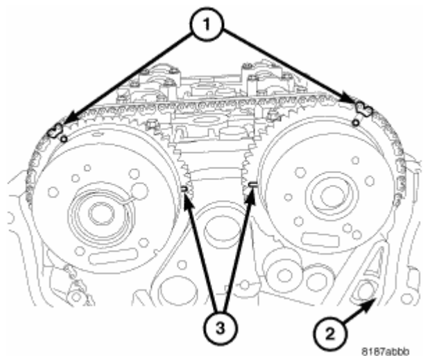
Fig. 128: Timing Chain Timing Marks
