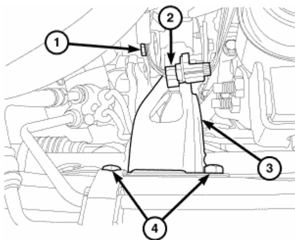
Fig. 190: Rear Mount
