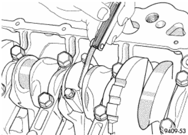
Fig. 237: Connecting Rod Side Clearance Courtesy of CHRYSLER LLC
