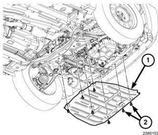
Fig. 314: Removal/Installation Front Skid Plate And Bolts Courtesy of CHRYSLER LLC
