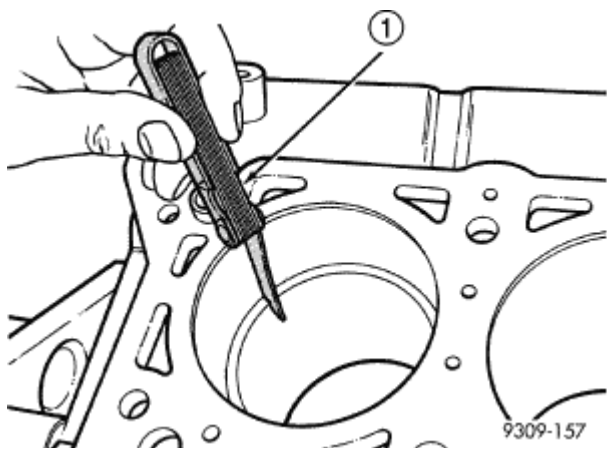
Fig. 244: Checking Ring Gap Courtesy of CHRYSLER LLC
