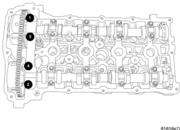
Fig. 134: Front CAM Cap Removal Sequence Courtesy of CHRYSLER LLC
