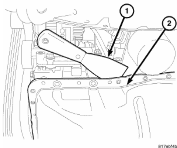
Fig. 200: Oil Pan Removal Courtesy of CHRYSLER LLC
