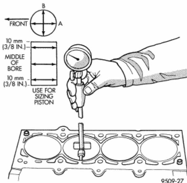
Fig. 193: Checking Cylinder Bore Size Courtesy of CHRYSLER LLC
