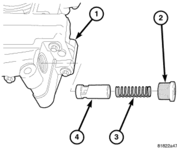
Fig. 293: View Of Pressure Regulating Valve Courtesy of CHRYSLER LLC
