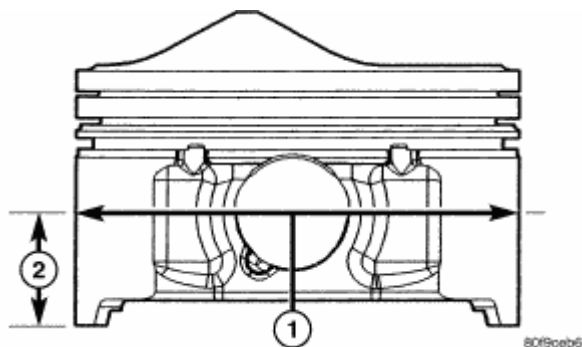
Fig. 228: Piston Measurement
