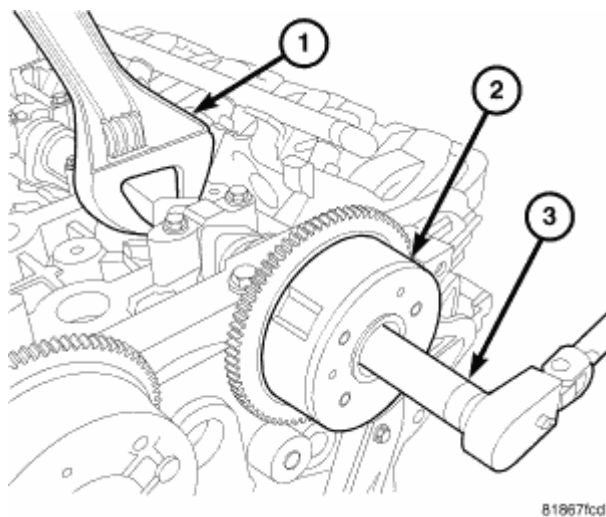
Fig. 173: CAMSHAFT PHASER Courtesy of CHRYSLER LLC
