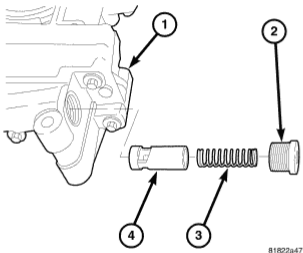
Fig. 292: View Of Pressure Regulating Valve Courtesy of CHRYSLER LLC
