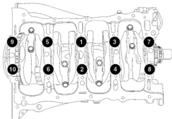
Fig. 204: Main Bearing Cap Torque Sequence Courtesy of CHRYSLER LLC
