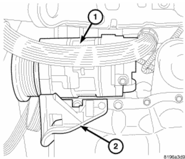
Fig. 42: A/C Compressor Courtesy of CHRYSLER LLC
