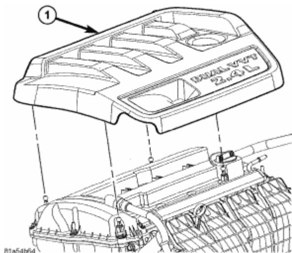
Fig. 359: Engine Cover Courtesy of CHRYSLER LLC
