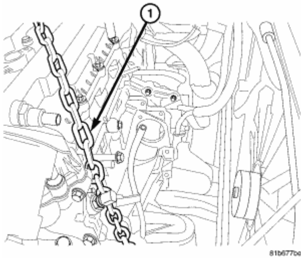
Fig. 196: Lift Chain Courtesy of CHRYSLER LLC
