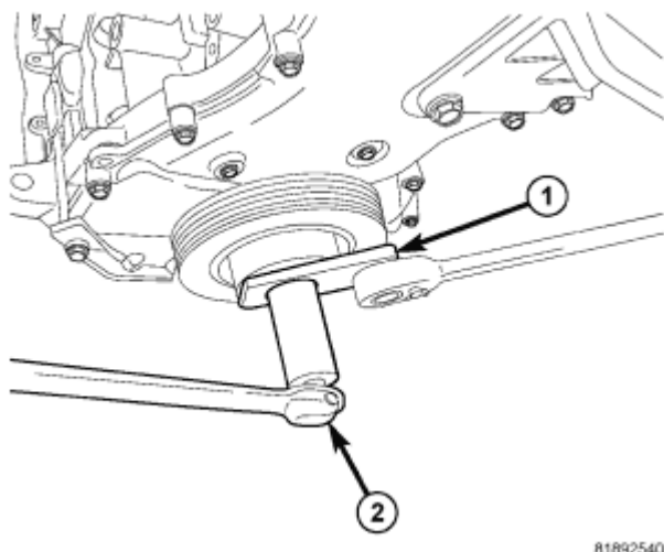
Fig. 250: Removing/Installing Damper Courtesy of CHRYSLER LLC
