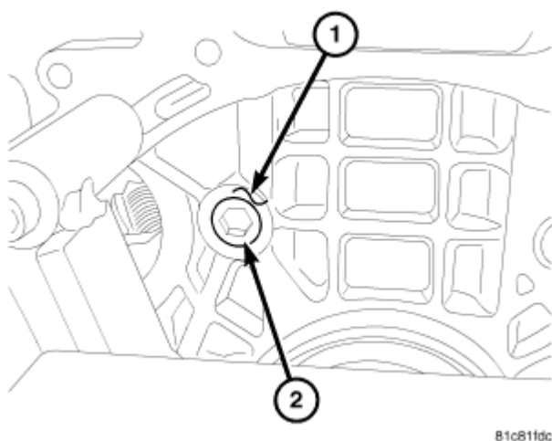
Fig. 3: Gallery Plug
