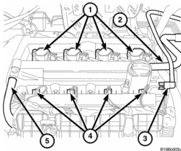
Fig. 397: Coil Connector Courtesy of CHRYSLER LLC
