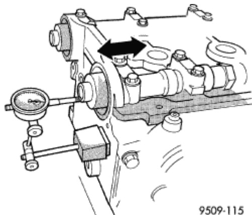
Fig. 123: Measuring Camshaft End Play
