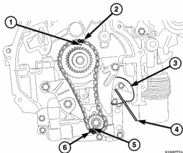
Fig. 302: Timing Chain Mark & Tensioner Pin Courtesy of CHRYSLER LLC
