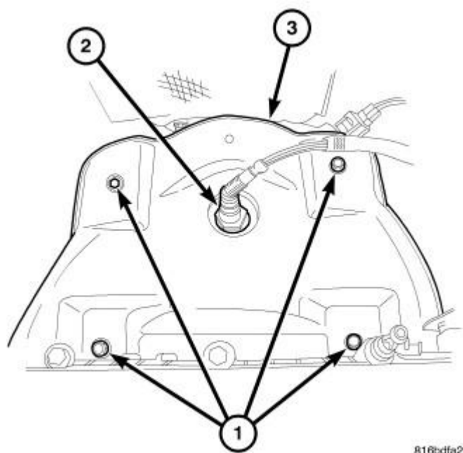
Fig. 313: Maniverter Heat Shield And Bolts Courtesy of CHRYSLER LLC
