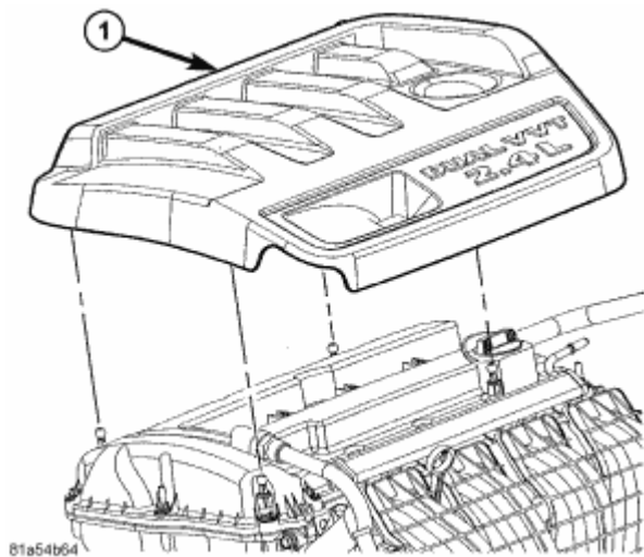
Fig. 7: Engine Cover
