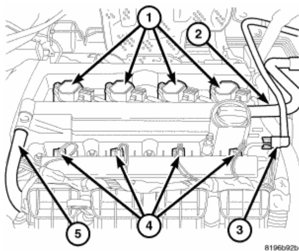
Fig. 8: Coil Connector
