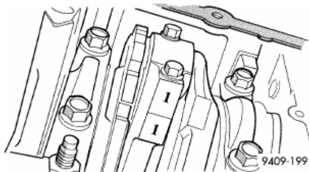
Fig. 233: Identify Connecting Rod to Cylinder-Typical
