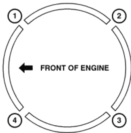
Fig. 234: Piston Ring End Gap Position Courtesy of CHRYSLER LLC
