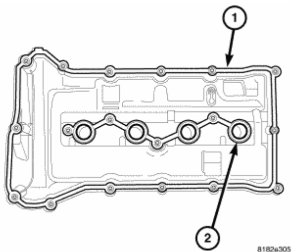
Fig. 154: Gasket Location
