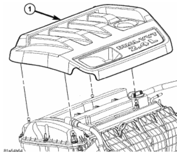
Fig. 358: Engine Cover Courtesy of CHRYSLER LLC
