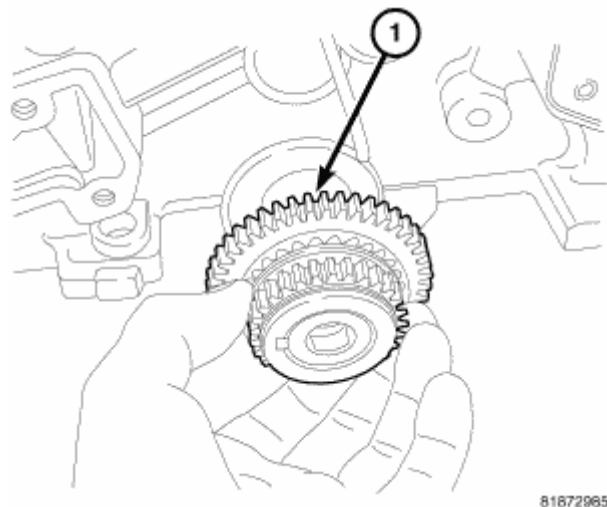
Fig. 201: Crankshaft Sprocket Courtesy of CHRYSLER LLC
