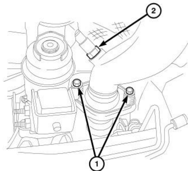
Fig. 347: Exhaust To Maniverter Bolts Courtesy of CHRYSLER LLC
