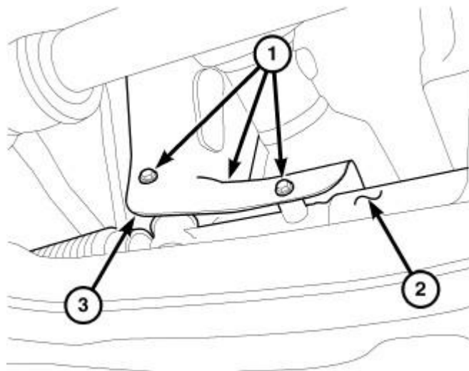
Fig. 346: Removing/Installing Bolts Securing Steering Gear Heat Shield Courtesy of CHRYSLER LLC
