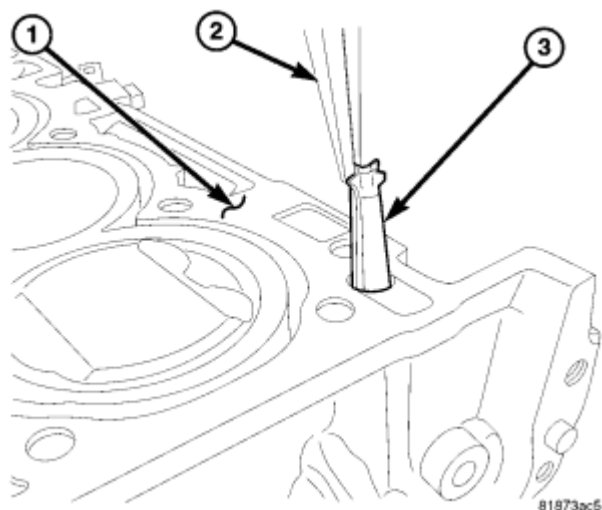
Fig. 104: VVT Filter
