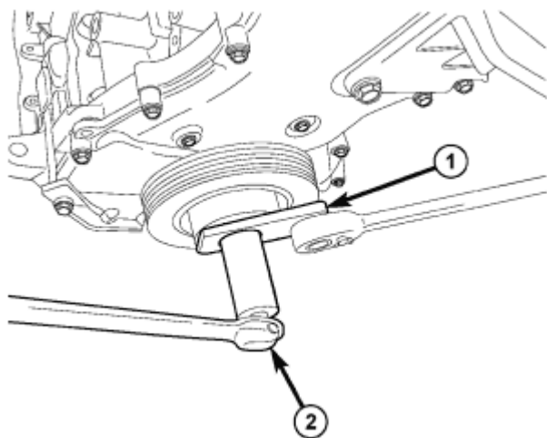
Fig. 249: Removing/Installing Damper Courtesy of CHRYSLER LLC
