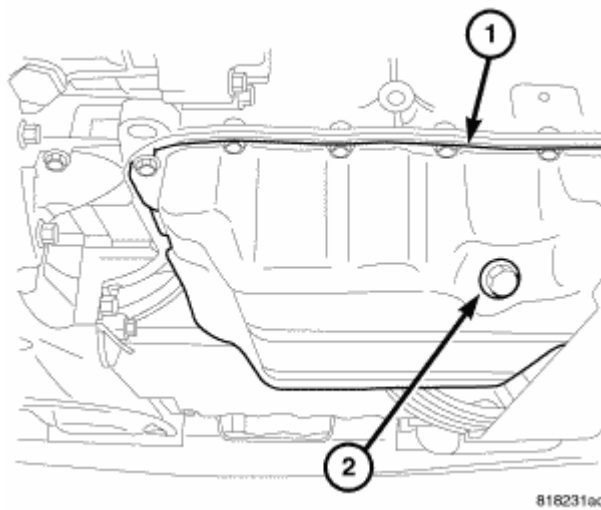
Fig. 197: Oil Drain Plug Courtesy of CHRYSLER LLC
