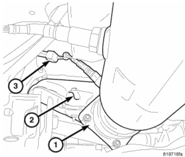
Fig. 41: Cat At Exhaust Manifold Courtesy of CHRYSLER LLC
