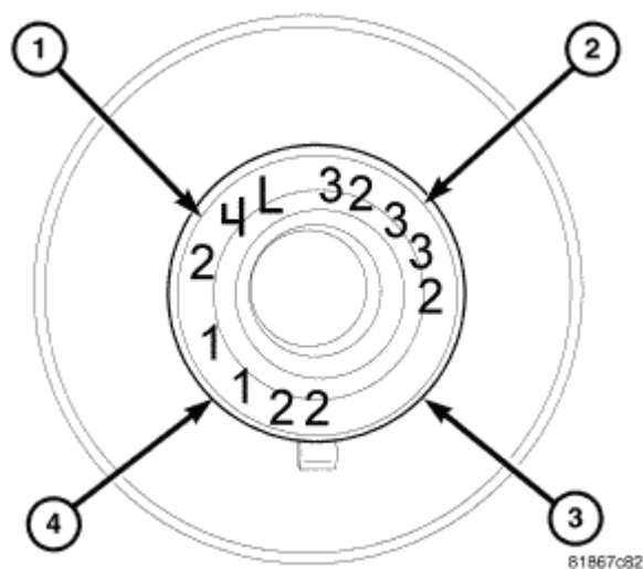
Fig. 241: Connecting Rod Bearing Identification Courtesy of CHRYSLER LLC
