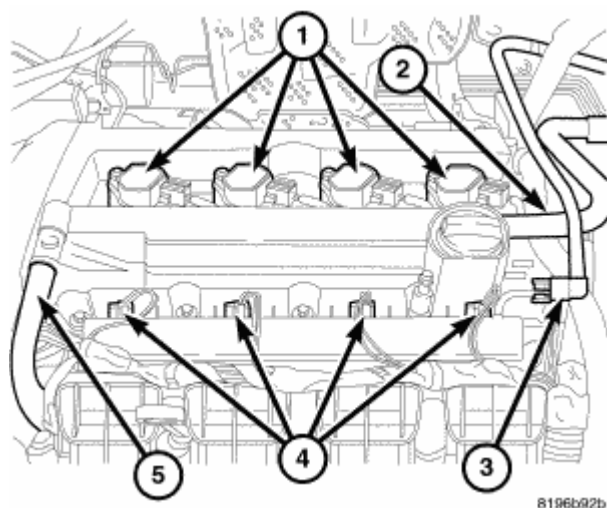
Fig. 376: Coil Connector
