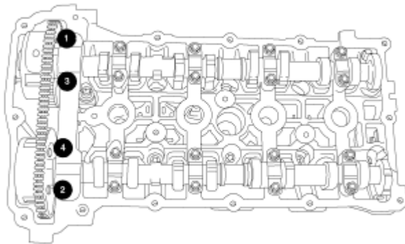
Fig. 145: Front Cam Cap Torque Sequence Courtesy of CHRYSLER LLC
