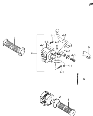
Fig. 33 HANDLE SWITCH (P01-S340-0007)
