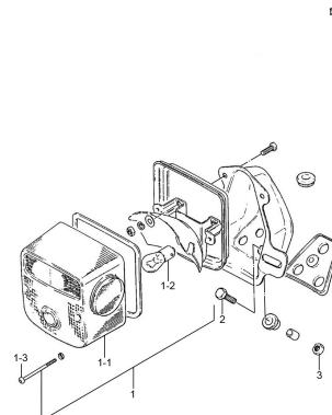
Fig. 23 REAR COMBINATION LAMP (P01-S240-0005)
