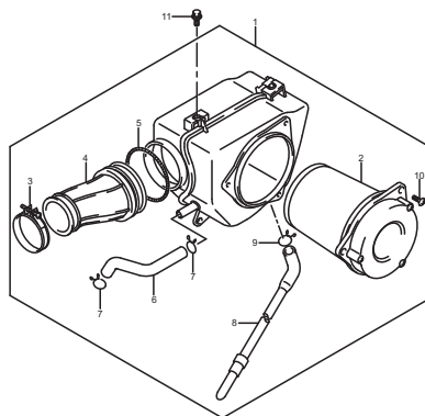
FIG.10 (B-11) AIR CLEANER
