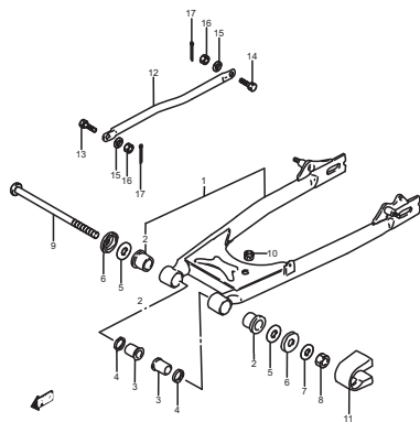
FIG.41 (G-4) REAR SWINGING ARM
