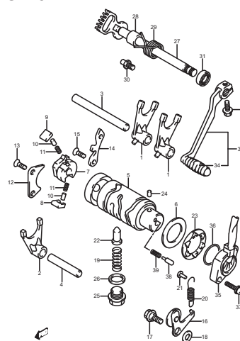
FIG.15 (C-4) GEAR SHIFTING
