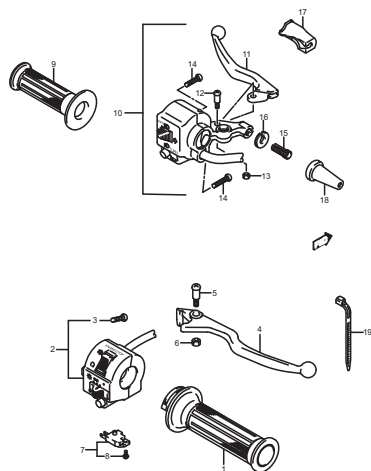
FIG.37 (F-7) HANDLE SWITCH
