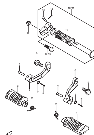
FIG.28 (E-5) FOOTREST
