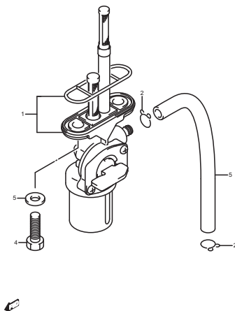
FIG.30 (E-7) FUEL COCK
