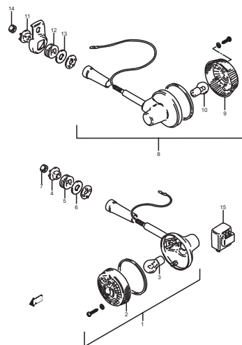
FIG.22 (D-7) TURN SIGNAL LAMP
