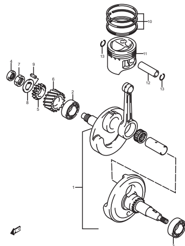
FIG.5 (B-6) CRANKSHAFT
