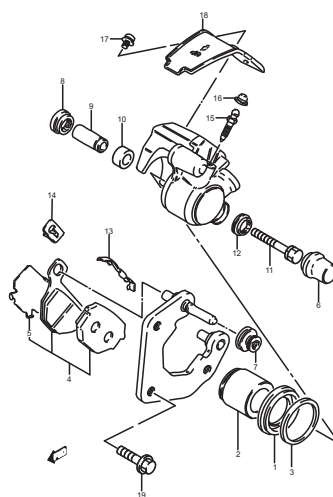
FIG.38 (F-8) FRONT CALIPER
