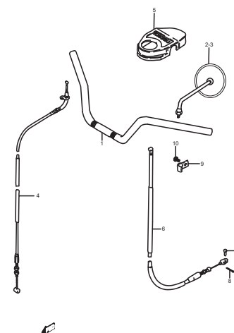
FIG.36 (F-6) HANDLE BAR CONTROL CABLE
