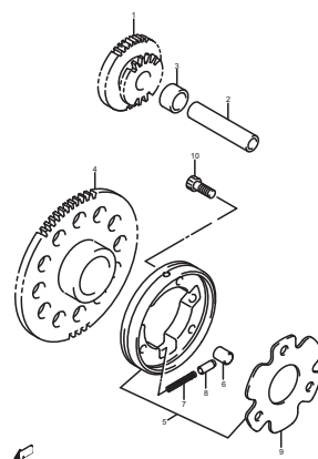
FIG.6 (B-7) STARTER CLUTCH
