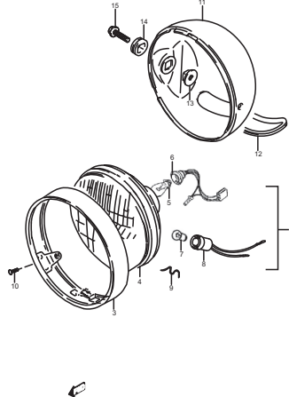
FIG.21 (D-6) HEADLAMP
