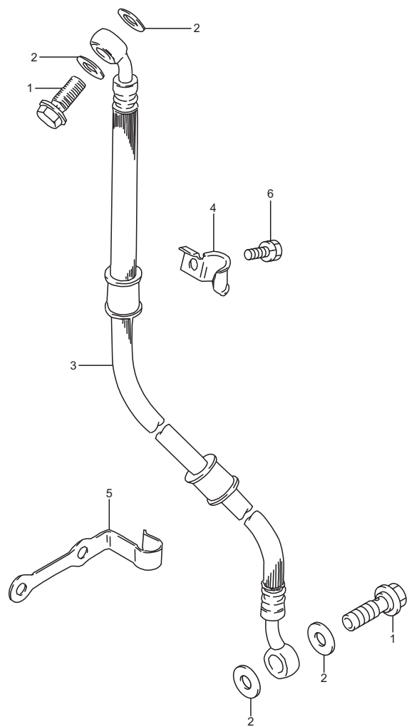
GN125K7_039 FRONT BRAKE HOSE
