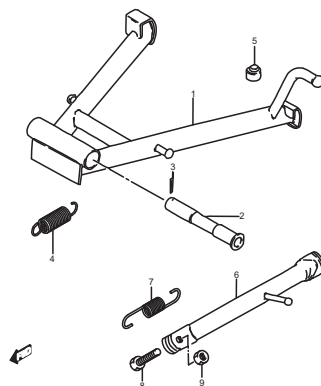
FIG.26 (E-3) CENTER STAND
