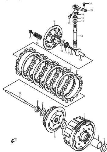
FIG.13 (C-2) CLUTCH
