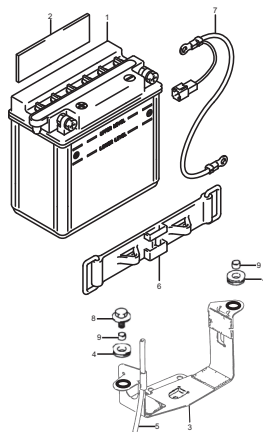
FIG.18 (D-3) BATTERY
