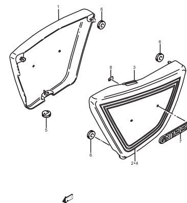
FIG.32 (E-9) FRAME COVER
