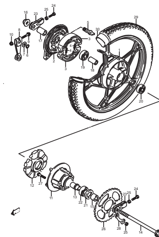
FIG.44 (G-7) REAR WHEEL
