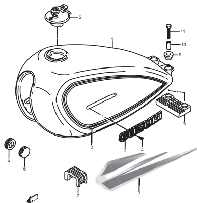
FIG.29 (E-6) FUEL TANK
