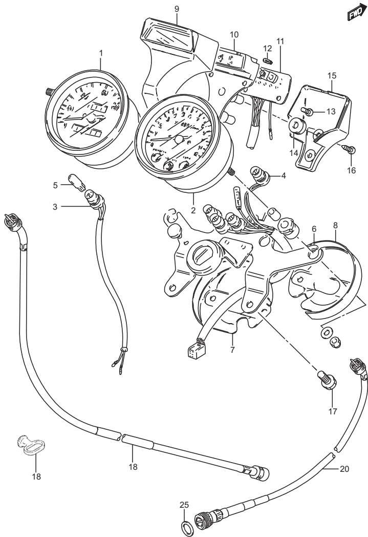
GN125K7_020 SPEEDOMETER
