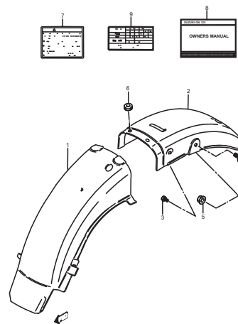
FIG.43 (G-6) REAR FENDER
