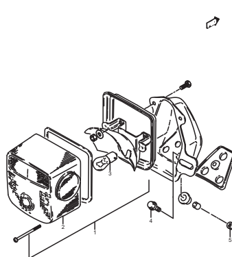
FIG.23 (D-8) REAR COMBINATION LAMP
