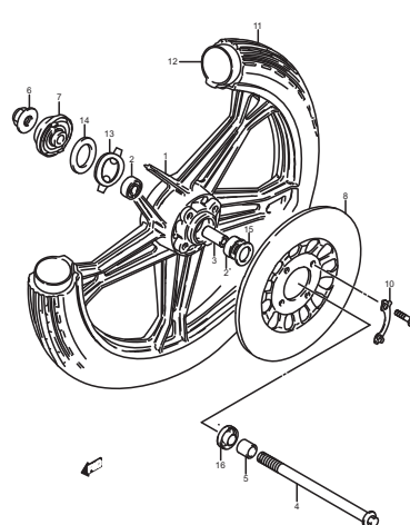
FIG.35 (F-5) FRONT WHEEL
