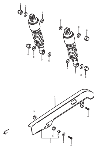
FIG.42 (G-5) CHAIN CASE REAR SHOCK ABSORBER
