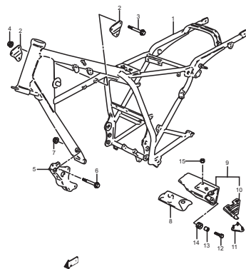
FIG.25 (E-2) FRAME
