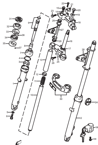
FIG.33 (F-3) FRONT FORK
