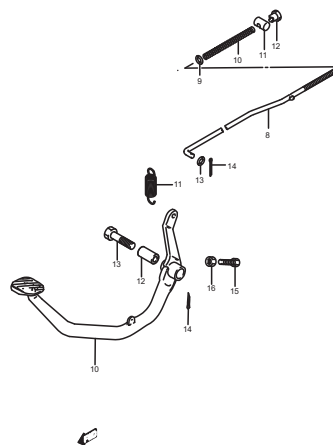
FIG.27 (E-4) REAR BRAKE PEDAL
