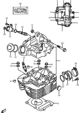
FIG.1 (B-2) CYLINDER HEAD
