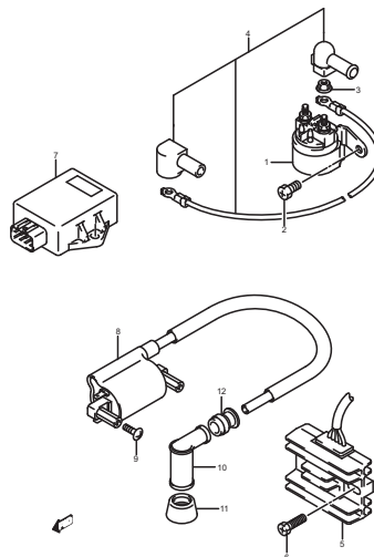
FIG.19 (D-4) ELECTRICAL
