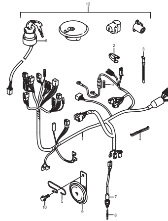
FIG.24 (D-9) WIRING HARNESS
