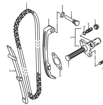
FIG.8 (B-9) CAM CHAIN
