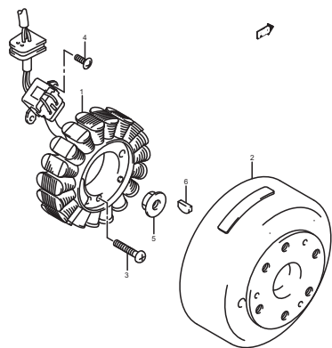
FIG.17 (D-2) MAGNETO
