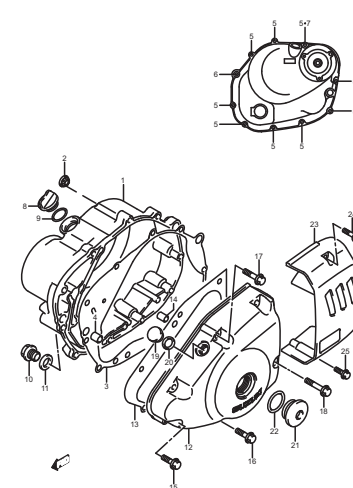
FIG.4 (B-5) CRANKCASE COVER
