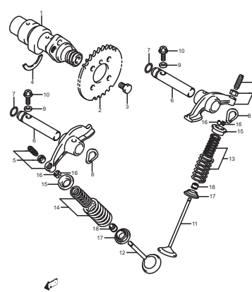
FIG.7 (B-8) CAMSHAFT / VALVE
