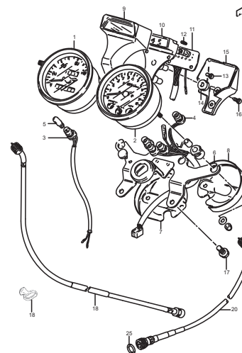
FIG.20 (D-5) SPEEDOMETER / TACHOMETER
