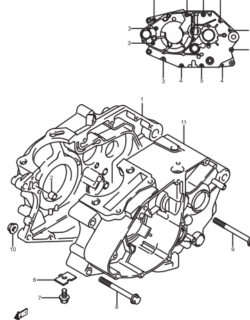
FIG.3 (B-4) CRANKCASE
