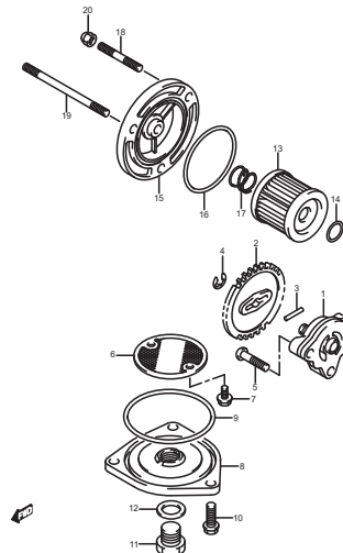
FIG.12 (B-13) OIL PUMP
