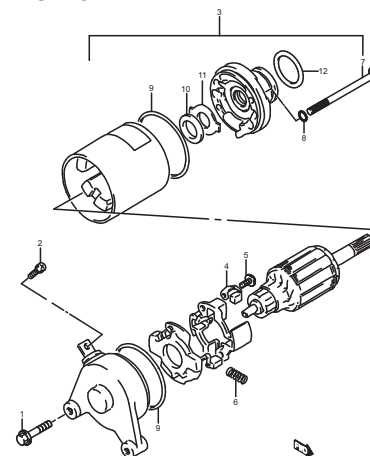
FIG.16 (C-5) STARTING MOTOR
