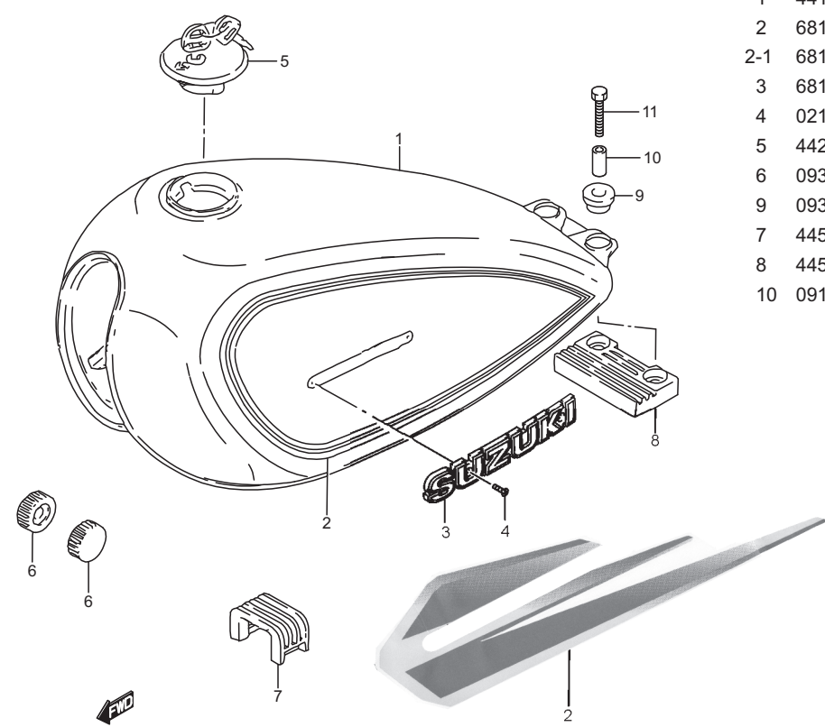
FIG.29 (E-6) FUEL TANK
