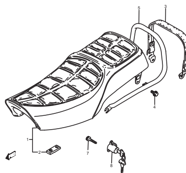
FIG.31 (E-8) SEAT
