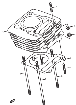
FIG.2 (B-3) CYLINDER
