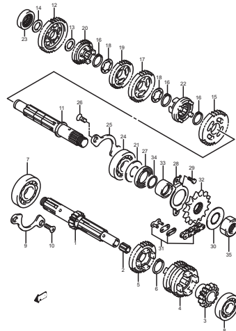
FIG.14 (C-3) TRANSMISSION
