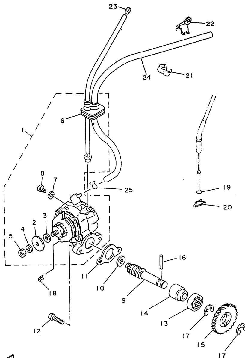
FIG. 3 OIL PUMP
