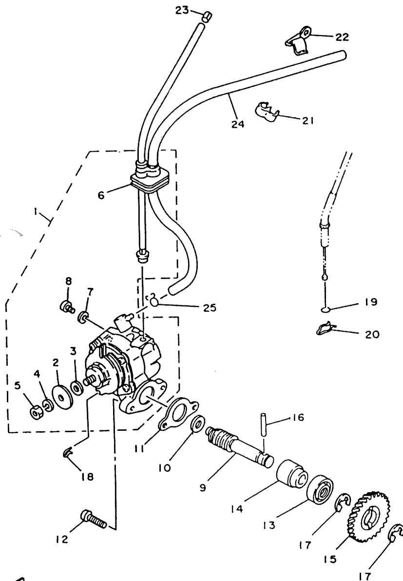
FIG. 3 OIL PUMP
