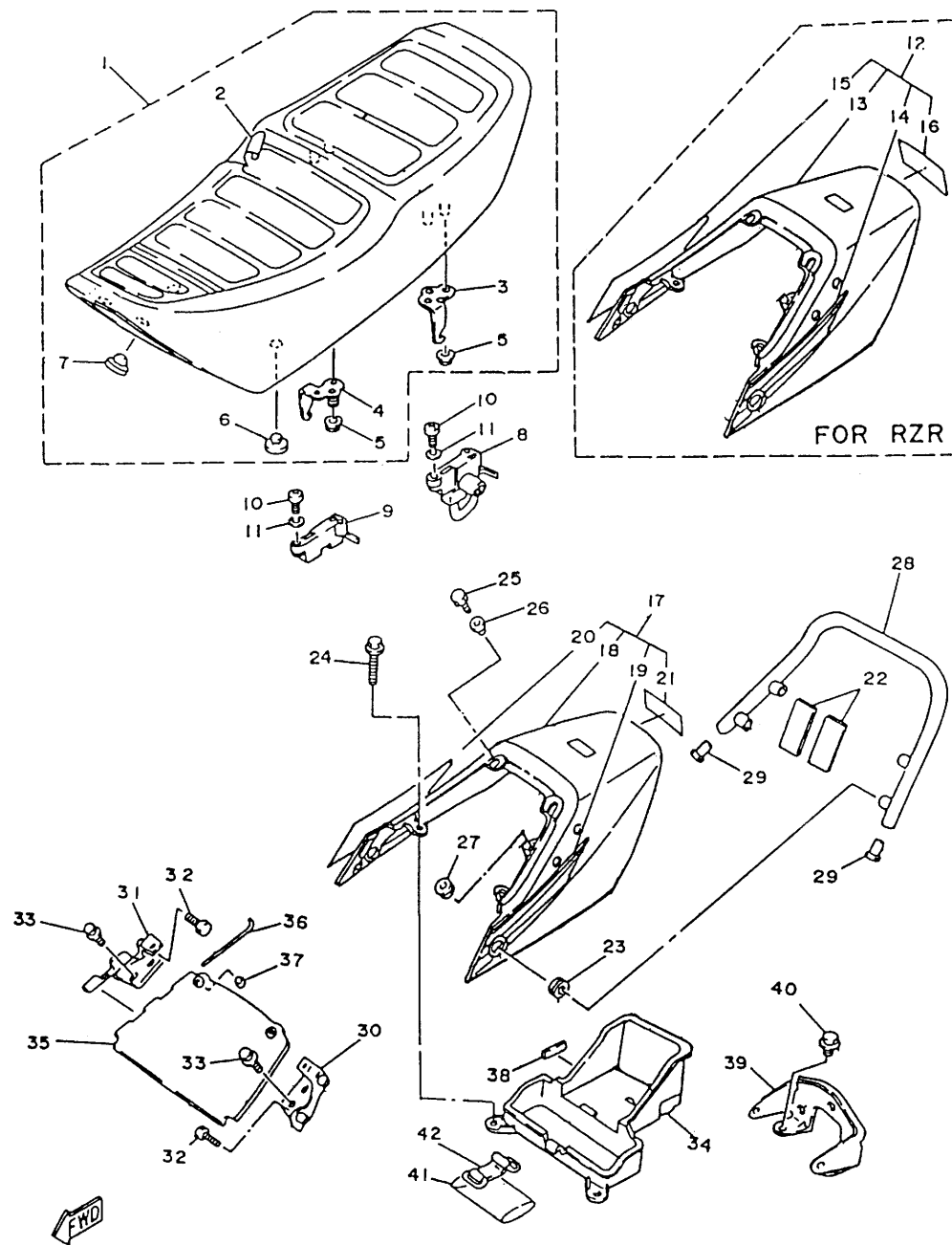
FIG. 23 SEAT
