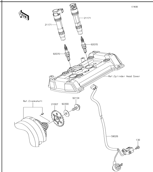
24 Ignition System
