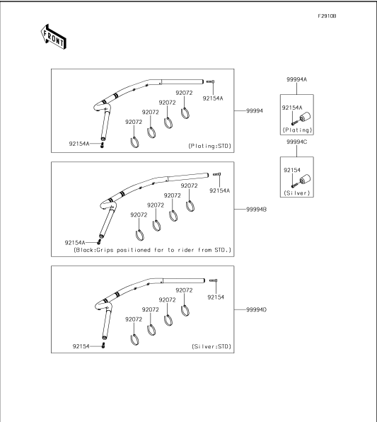
68 Accessory(Handlebar)
