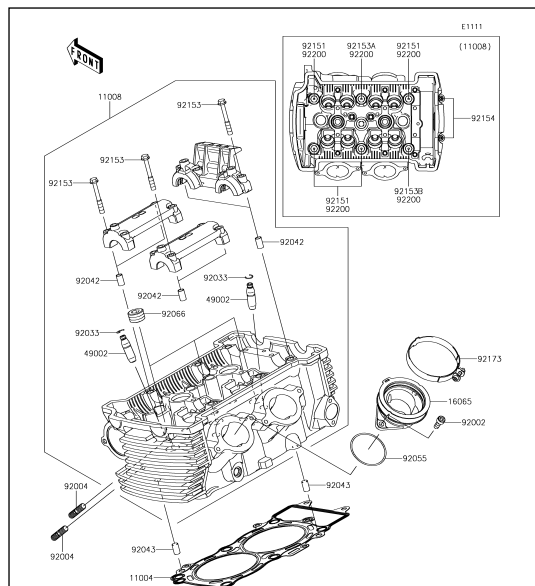
1 Cylinder Head
