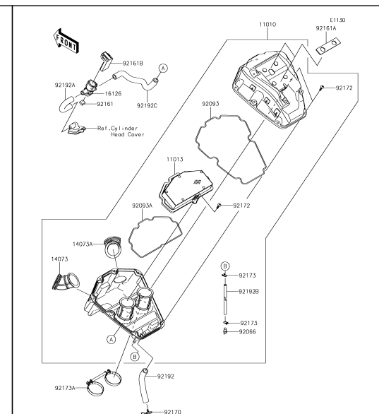
4 Air Cleaner
