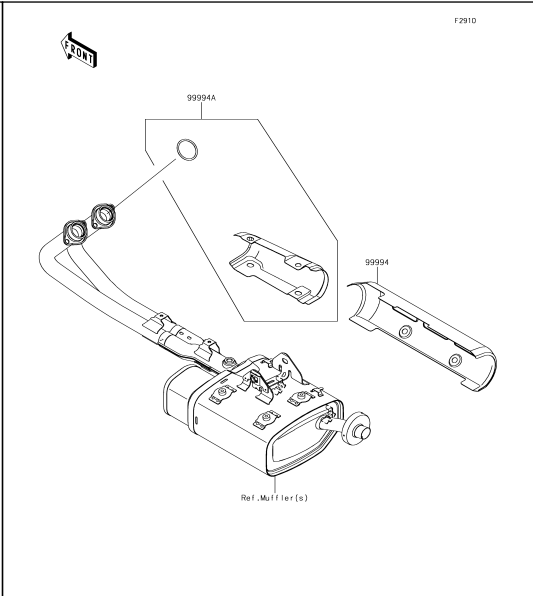
66 Accessory(Muffler Cover)
