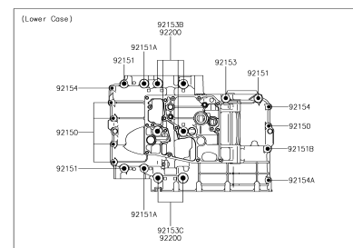
15 Crankcase Bolt Pattern
