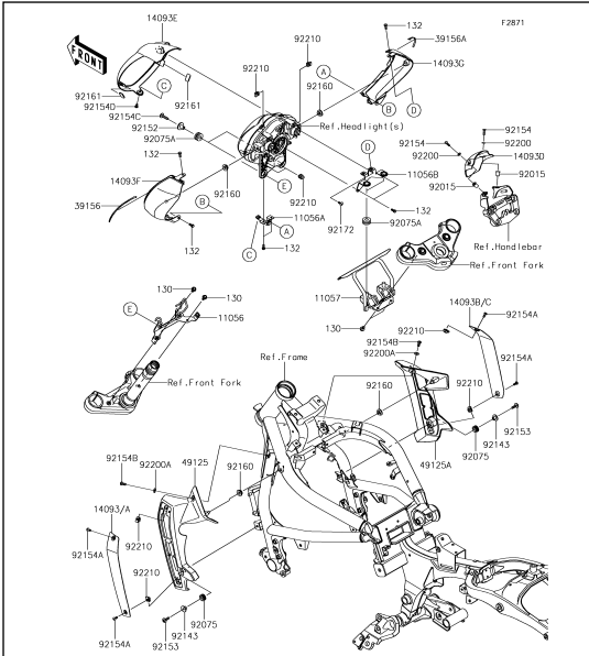
65 Cowling
