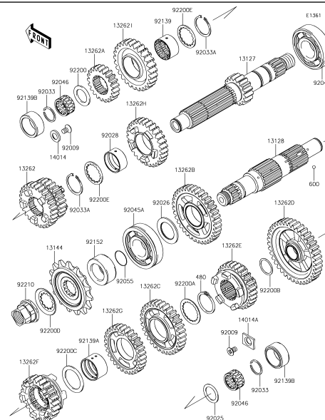
11 Transmission
