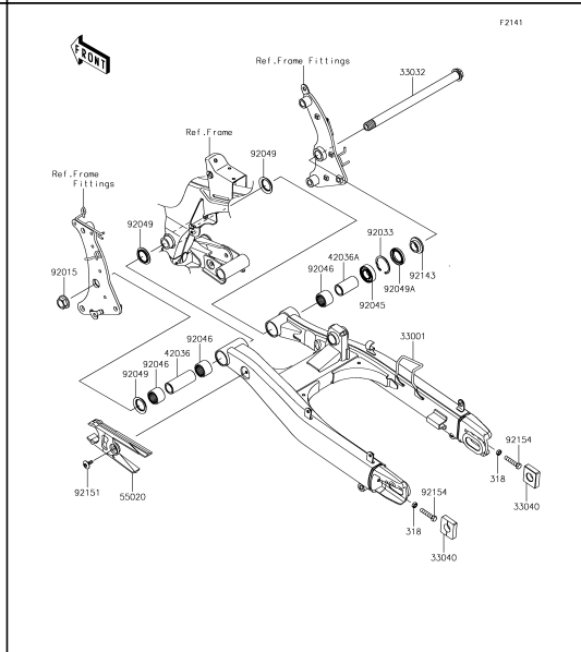
32 Swingarm
