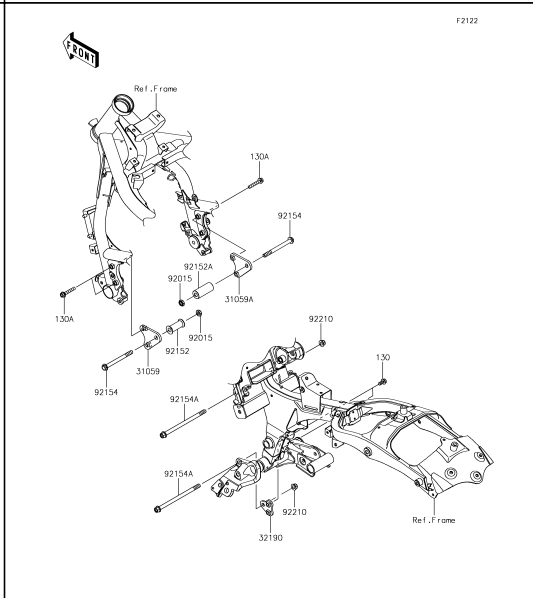
30 Engine Mount
