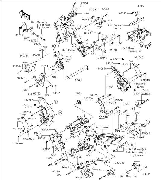
31 Frame Fittings
