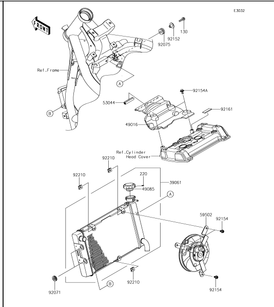
27 Radiator
