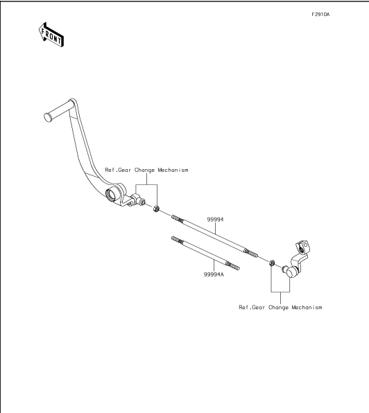
67 Accessory(Tie Rod)
