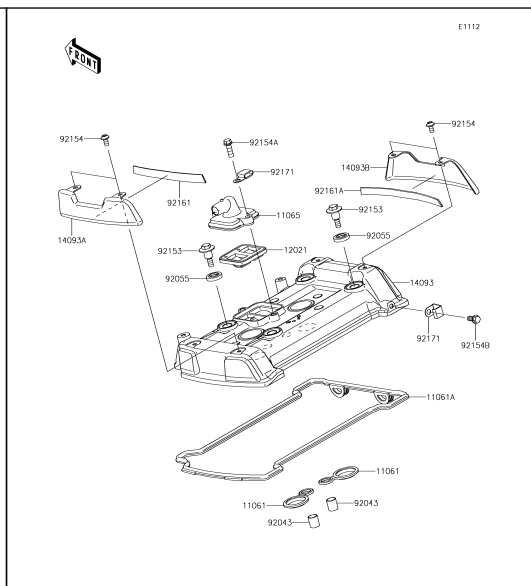
2 Cylinder Head Cover
