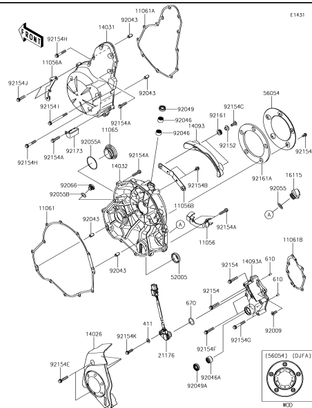
16 Engine Cover(s)
