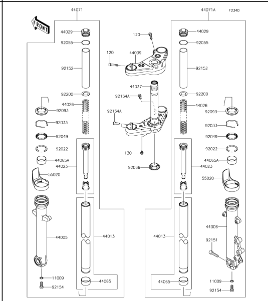
48 Front Fork
