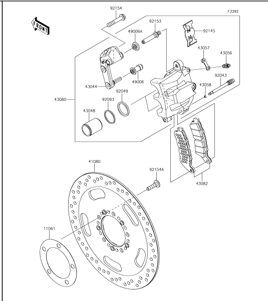
44 Front Brake
