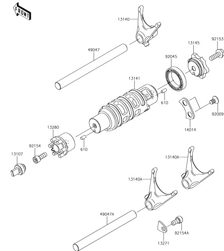
12 Gear Change Drum/Shift Fork(s)
