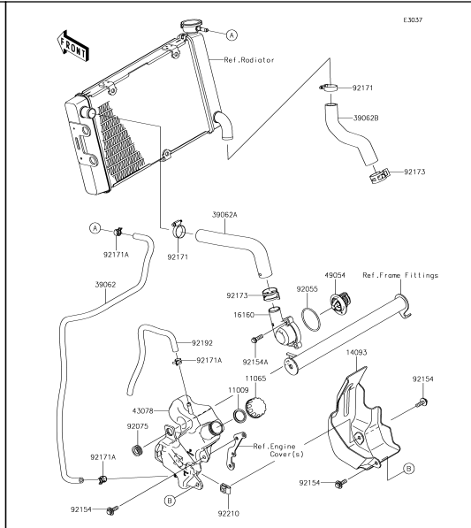
28 Water Pipe
