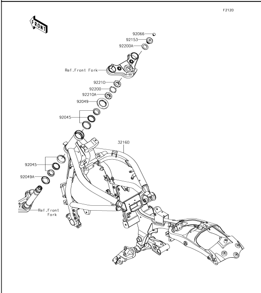
29 Frame
