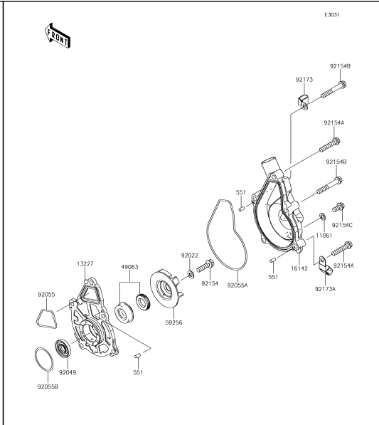
26 Water Pump
