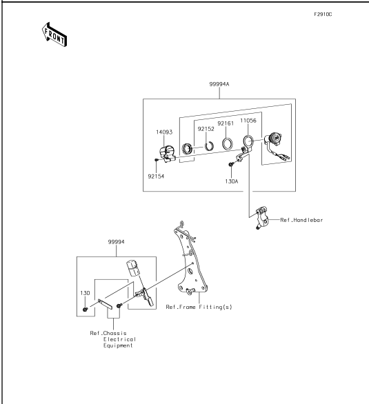
69 Accessory(DC Socket etc.)
