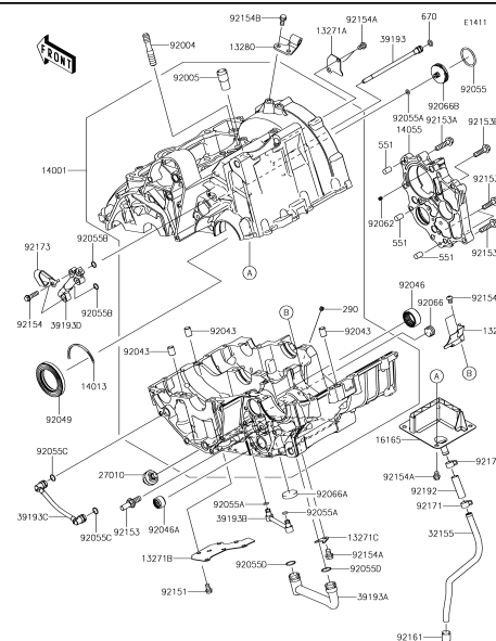
14 Crankcase
