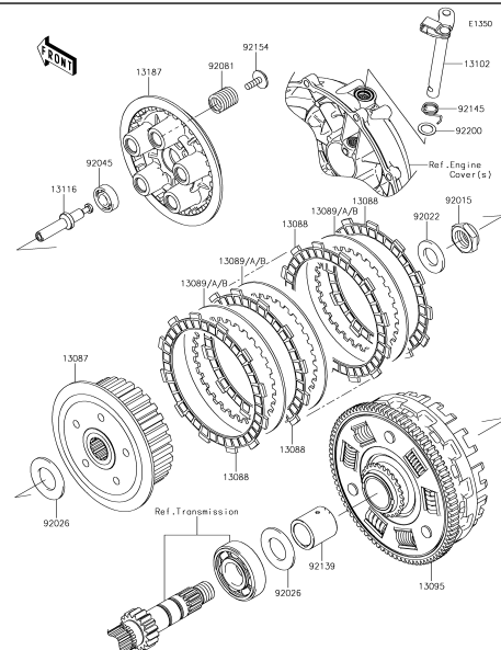
10 | Clutch
