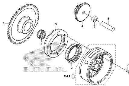
STARTING CLUTCH
