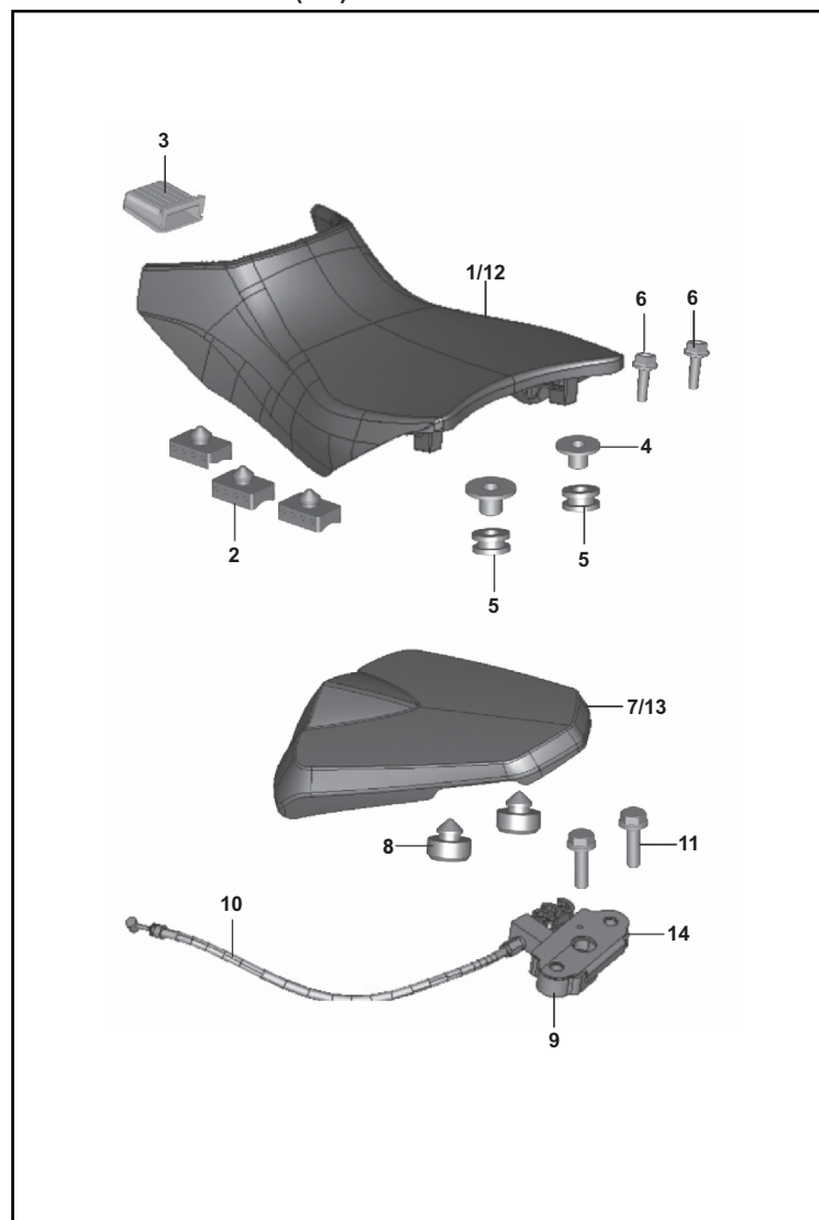
FIGURA N° 24: SILLÍN (1/2)
