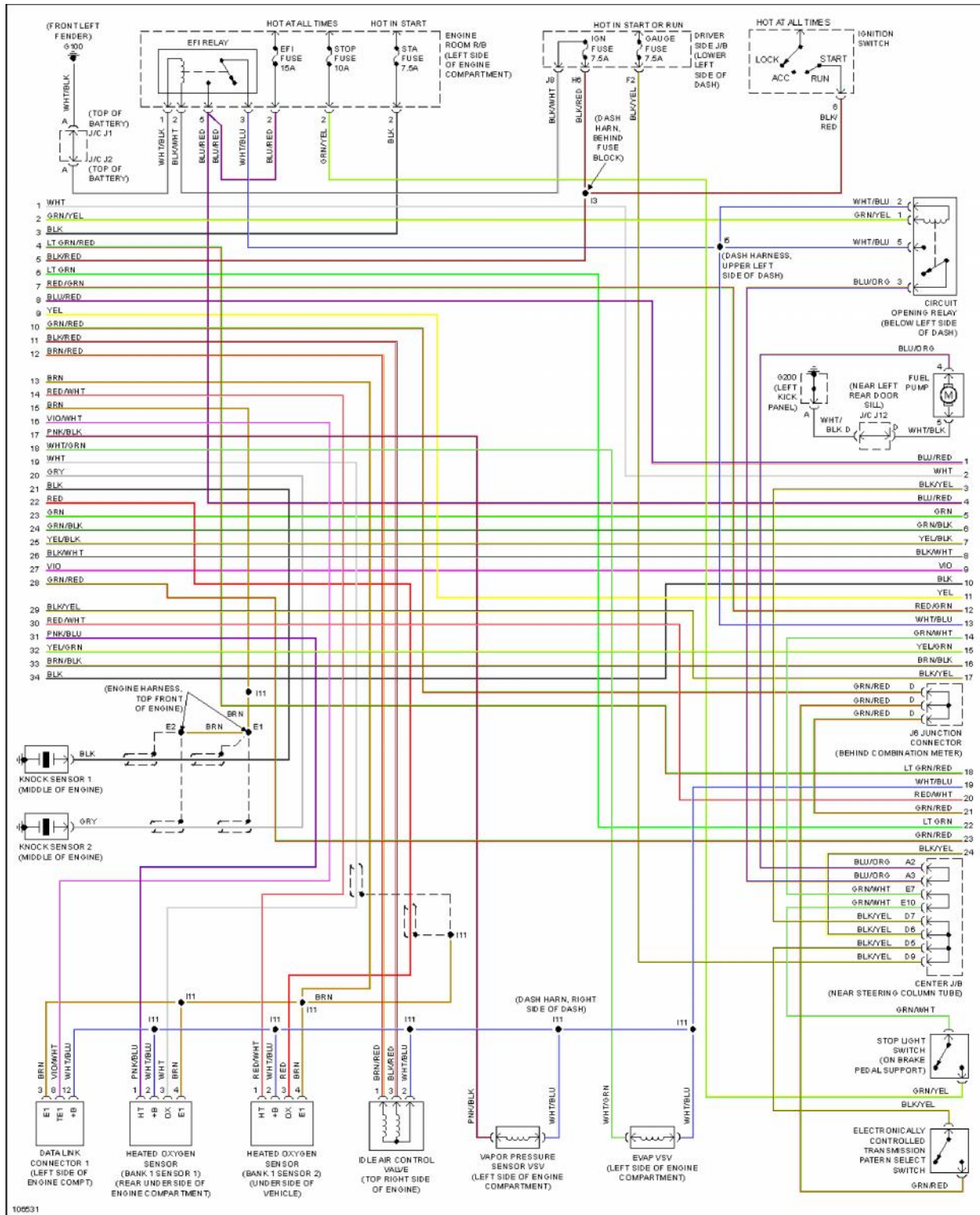
Fig. 13: 3.4L, Engine Performance Circuits (2 of 3)
