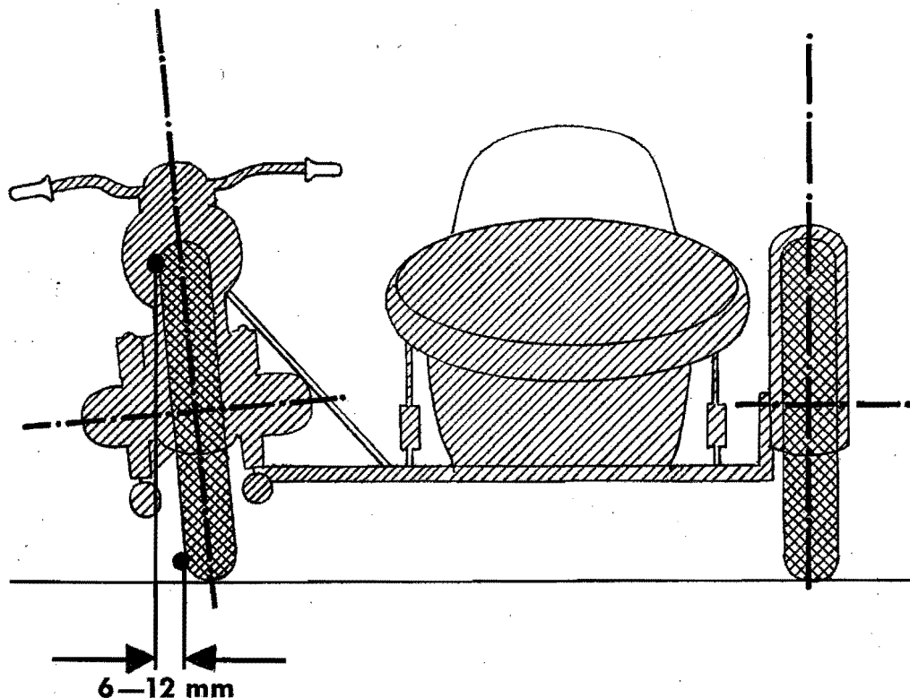
Adjusting Camber when connecting a Side Car.
