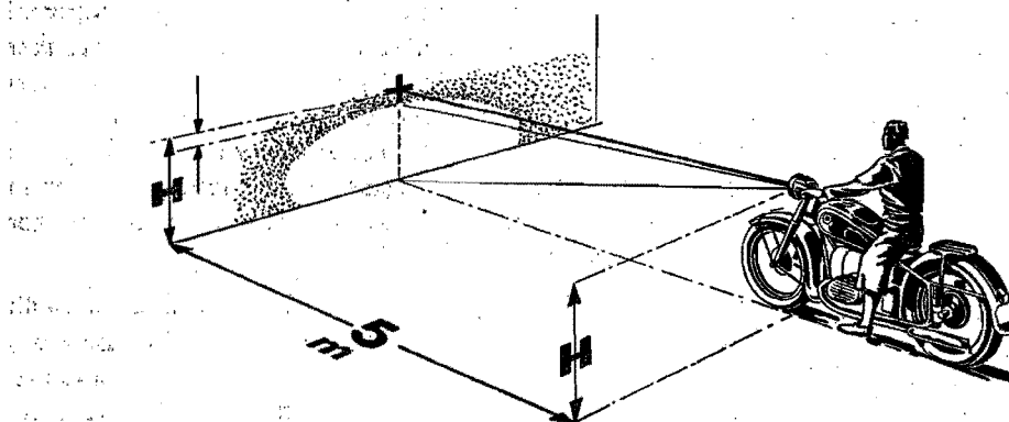
Headlamp adjustment (correctly focussed dipped beam)
