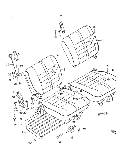
FIG.134 REAR SEAT
