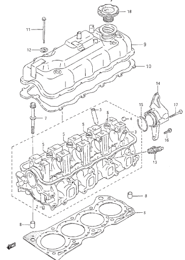
FIG.5 CYLINDER HEAD (GASOLINE CARBURETOR)
