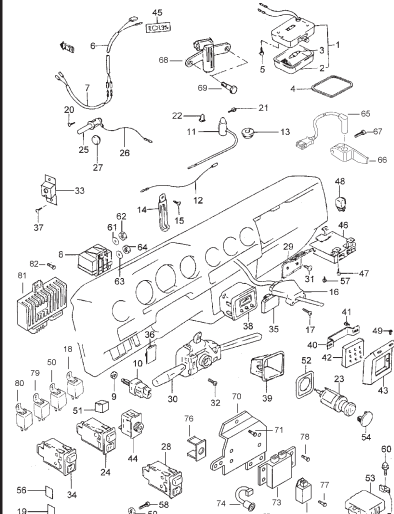
FIG.73 ELECTRICAL CONTROL
