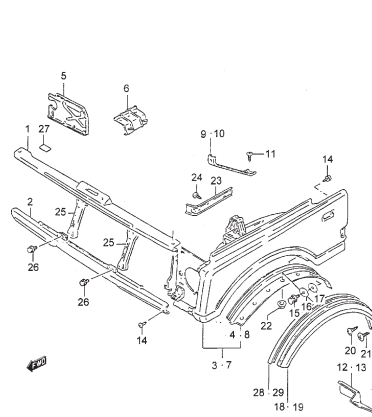
FIG.97 FRONT BODY
