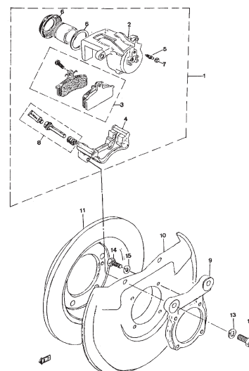
FIG.92 FRONT WHEEL BRACKE
