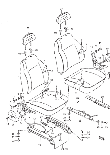
FIG.133 FRONT SEAT
