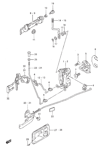
FIG.126 FRONT DOOR LOCK
