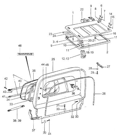
FIG.123 RESIN TOP (PICK UP)
