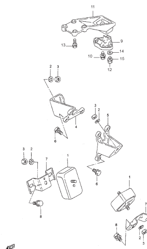
FIG.12 ENGINE MOUNTING
