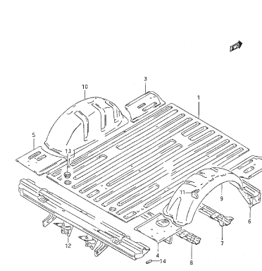
FIG.102 REAR BODY (LONG)
