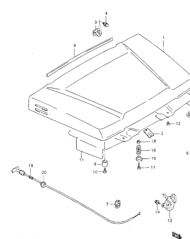
FIG.98 FRONT HOOD
