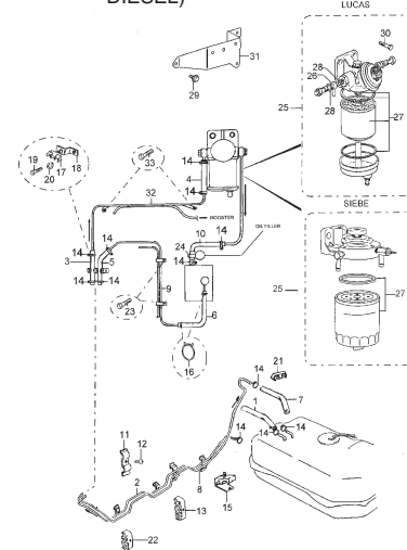
FIG.36 FUEL FEED CIRCUIT (TURBO DIESEL)
