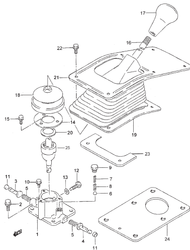
FIG.51 GEAR SHIFTING CONTROL
