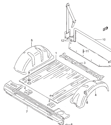
FIG.101 REAR BODY (SHORT)
