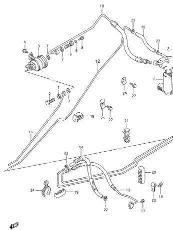
FIG.35 FUEL PUMP (GASOLINE: FUEL INJECTION)
