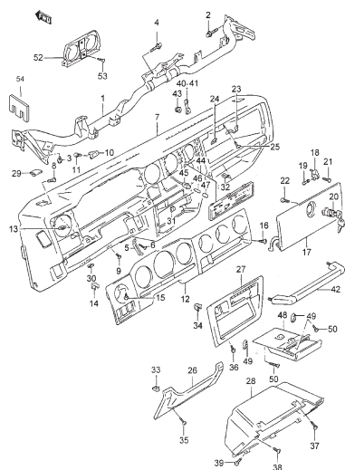
FIG.115 INTERIOR TRIM
