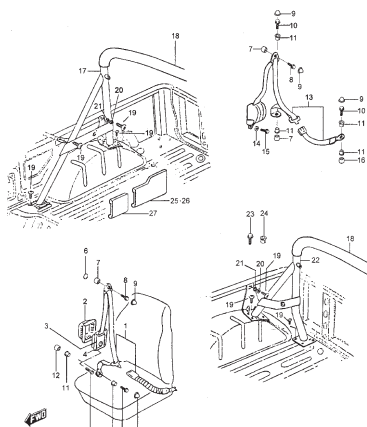
FIG.135 SEAT BELTS
