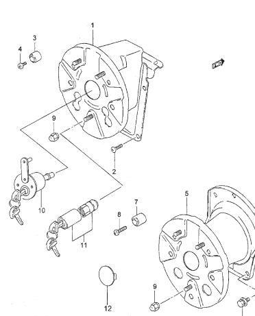
FIG.117 TIRE CARRIER
