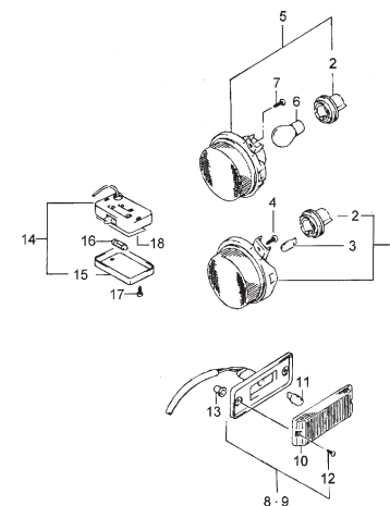
FIG.70 FRONT LAMP AND ROOM LAMP
