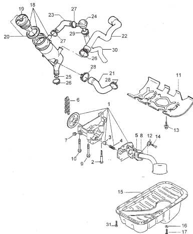
FIG.11 OIL PUMP (TURBO DIESEL)
