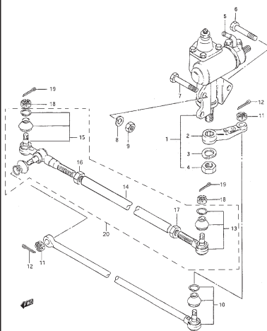
FIG.86 STEERING LINK (W/POWER STEERING)
