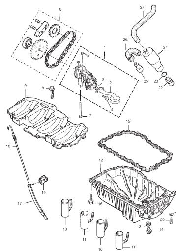
FIG.11A OIL PUMP (DIESEL EURO III)
