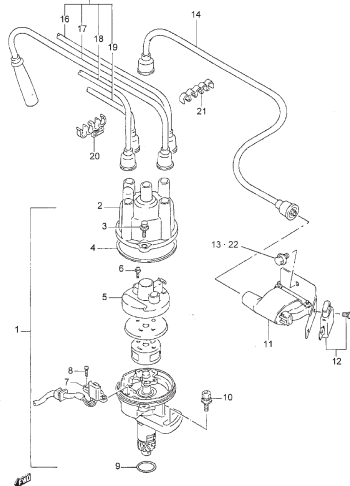
FIG.64 DISTRIBUTOR (W/FUEL INJECTION)
