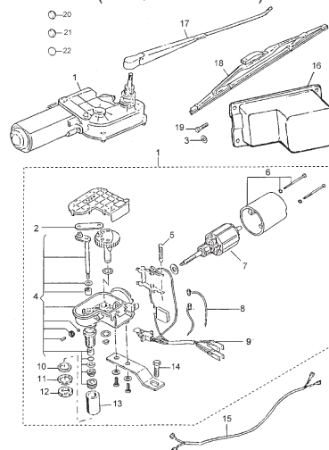
FIG.75A REAR WINDOW WIPER (V=W / REAR WIPER)
