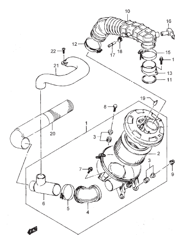
FIG.26 AIR CLEANER (GASOLINE: FUEL INJECTION)
