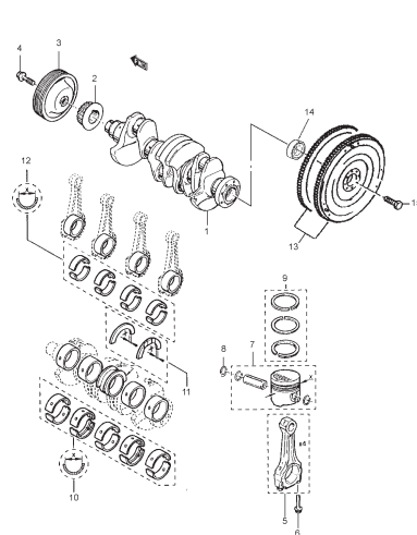
FIG.14A CRANKSHAFT(DIESEL EUROIII)
