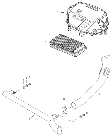
FIG.27A AIR CLEANER (DIESEL EUROIII)
