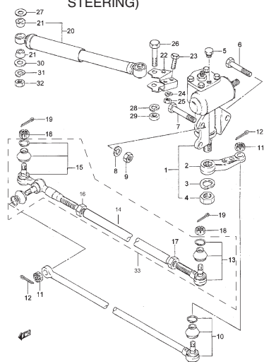
FIG.85 STEERING LINK (N/POWER STEERING)
