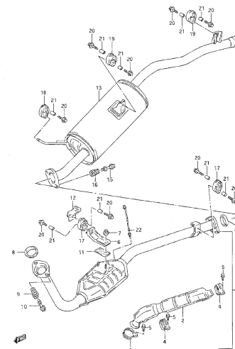
FIG.32 MUFFLER (GASOLINE: FUEL INJECTION)
