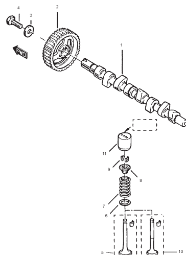
FIG.16A CAMSHAFT (DIESEL EURO III)
