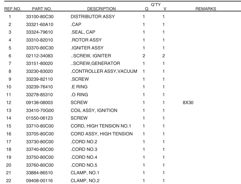
FIG.63 DISTRIBUTOR (W/CARBURETOR)
