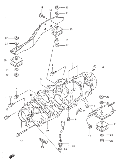
FIG.60 GENERATOR (GASOLINE)
