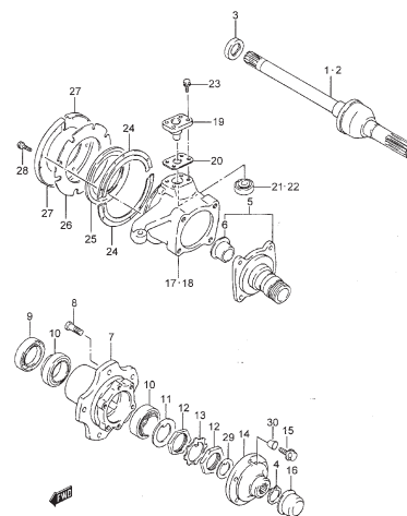
FIG.78 FRONT AXLE
