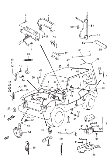
FIG.72 WIRING HARNESS
