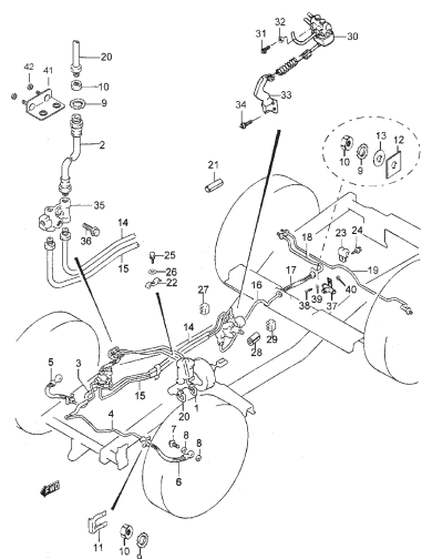
FIG.91A BRAKE PIPING (DIESEL)
