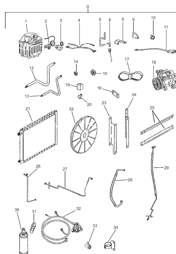
FIG.136 AIR CONDITIONER (GASOLINE)
