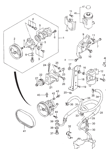
FIG.87 POWER STEERING PUMP
