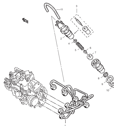
FIG.36C FUEL DELIVERY (DIESEL EURO III)
