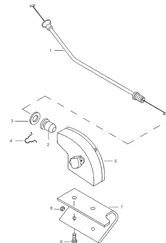
FIG.28A CONTROL CABLE (DIESEL EUROIII)
