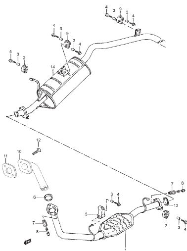
FIG.33 MUFFLER (DIESEL)
