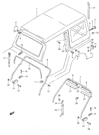
FIG.119 DECK TOP (CANVAS:SHORT)
