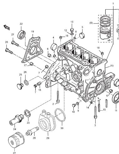
FIG.9A CYLINDER BLOCK (DIESEL EUROIII)
