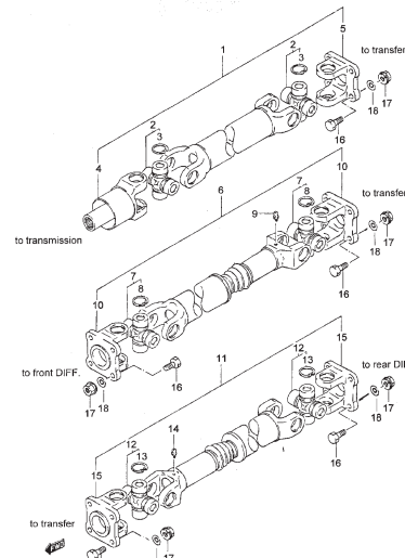
FIG.52 PROPELLER SHAFT
