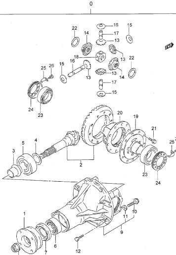
FIG.53 FRONT DIFF GEAR
