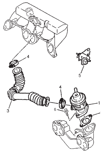
FIG.45 ENG. GAS RECIRCULATION (TURBO DIESEL)
