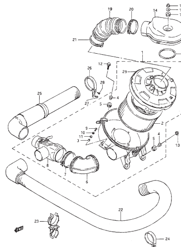
FIG.25 AIR CLEANER (GASOLINE: CARBURETOR)
