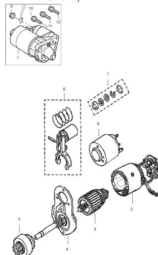
FIG.59A STARTING MOTOR (DIESEL EURO III)
