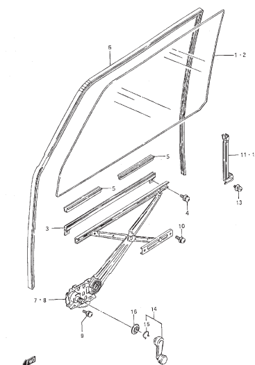
FIG.125 FR DR REGULATOR
