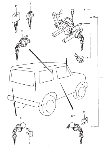
FIG.74 LOCK SET
