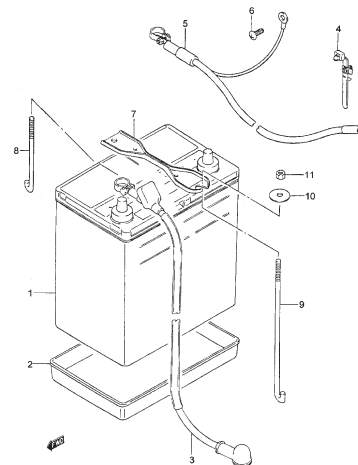
FIG.66 BATTERY
