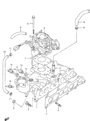
FIG.20 INTAKE MANIFOLD (GASOLINE: FUEL INJECTION)
