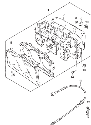
FIG.67 SPEEDOMETER ASSY (W/TACHOMETER) GASOLINE
