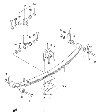
FIG.79 REAR SUSPENSION
