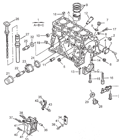
FIG.9 CYLINDER BLOCK (TURBO DIESEL)
