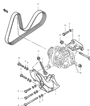
FIG.62A GENERATOR FITTING (DIESEL EURO III)
