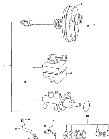
FIG.89 BRAKE MASTER CYLINDER (GASOLINE)
