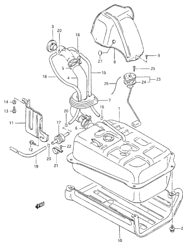
FIG.131 FUEL TANK (GASOLINE:CABURETOR, DIESEL)
