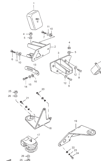
FIG.12A ENGINE MOUNTING
