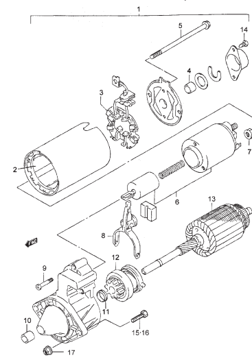
FIG.58 STARTING MOTOR (GASOLINE)
