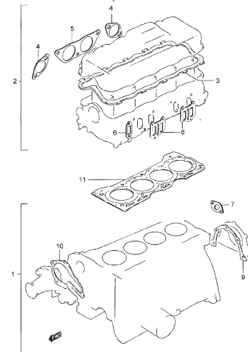
FIG.7A CYLINDER HEAD (DIESEL EURO III)
