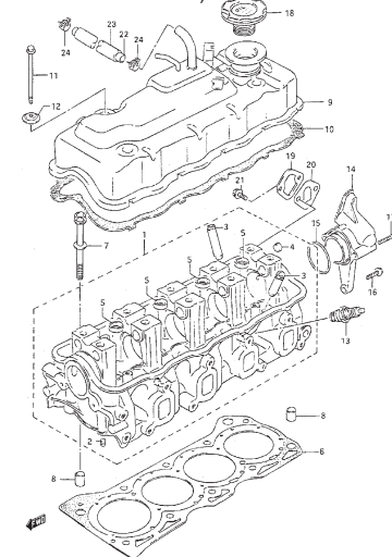
FIG.6 CYLINDER HEAD (GASOLINE INJECTION)
