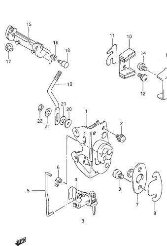
FIG.129 BACK DR LOCK (V)
