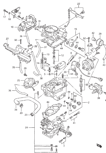
FIG.22 CARBURETOR (GASOLINE)
