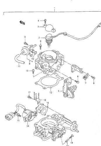
FIG.23 THROTTLE BODY (GASOLINE: FUEL INJECTION)
