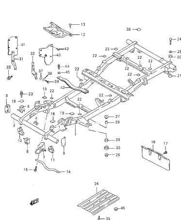
FIG.96 CHASSIS FRAME (LONG)
