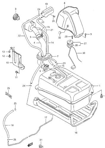
FIG.132 FUEL TANK (GASOLINE:FUEL INJECTION)
