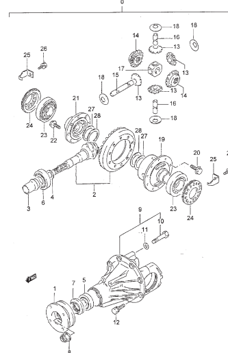
FIG.54 REAR DIFF GEAR
