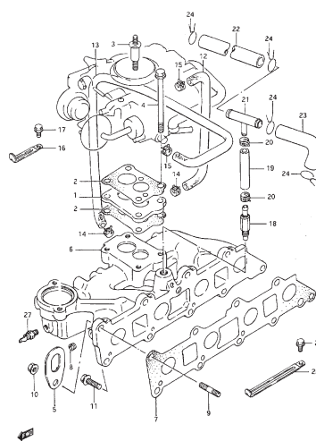
FIG.19 INTAKE MANIFOLD (GASOLINE: CARBURETOR)
