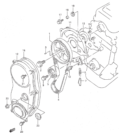
FIG.17 TIMING BELT (GASOLINE)
