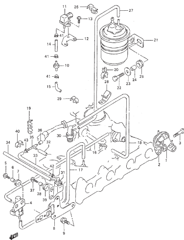
FIG.44 EMISSION CONTROL (GASOLINE: FUEL INJECTION)
