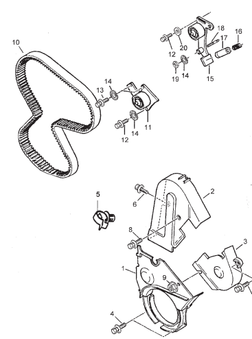
FIG.18 TIMING COVER (TURBO DIESEL)
