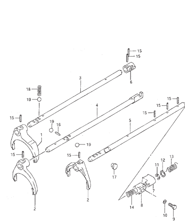
FIG.50 GEAR SHIFTING FORK
