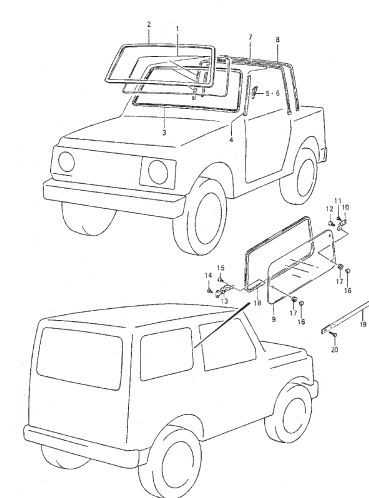
FIG.118 WINDOW GLASS
