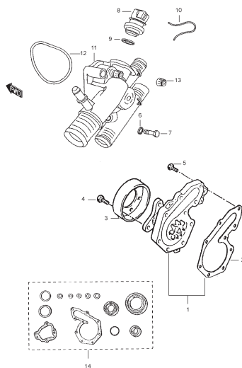
FIG.38A WATER PUMP (DIESEL EURO III)
