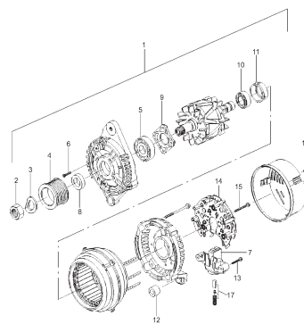
FIG.60 GENERATOR (GASOLINE)
