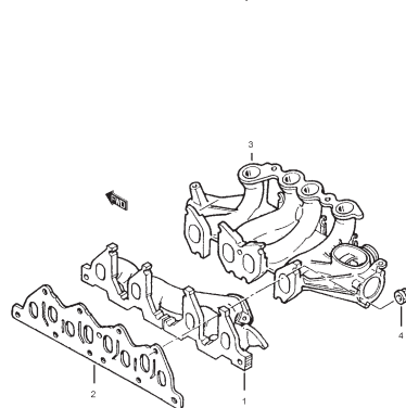
FIG. 21A INTAKE AND EXHAUST MANIFOLD (DIESEL EURO III)
