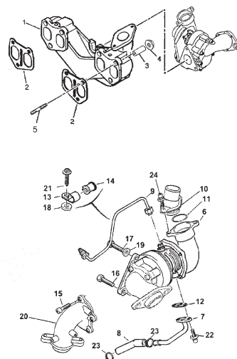
FIG.30 EXHAUST MANIFOLD AND TURBO CHARGE (TURBO DIESEL)
