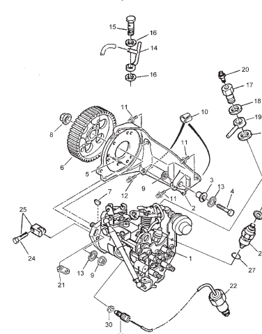
FIG.24 INJECTION PUMP (TURBO DIESEL)
