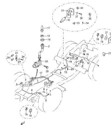
FIG.94 PARKING BRAKE
