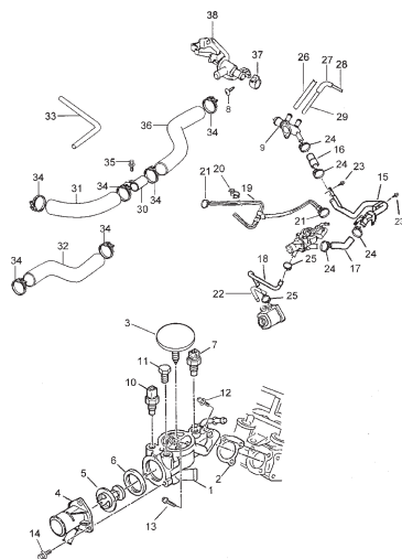
FIG.45 ENG. GAS RECIRCULATION (TURBO DIESEL)
