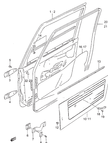
FIG.124 FR DR PANEL
