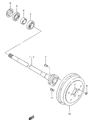
FIG.80 REAR AXLE
