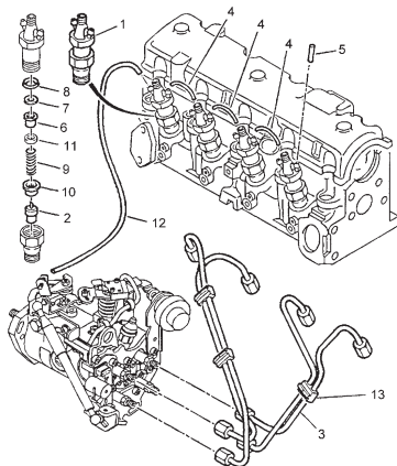
FIG.36A FUEL DELIVERY (TURBO DIESEL)
