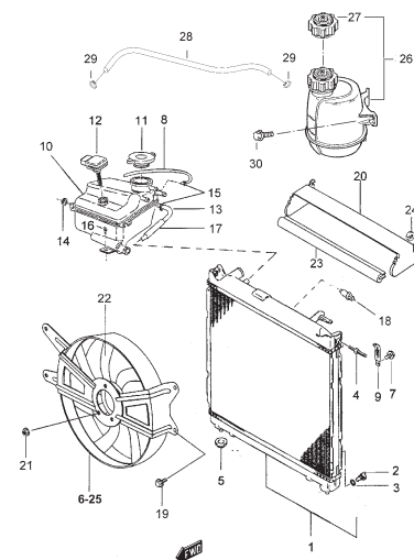
FIG.40 RADIATOR (DIESEL)
