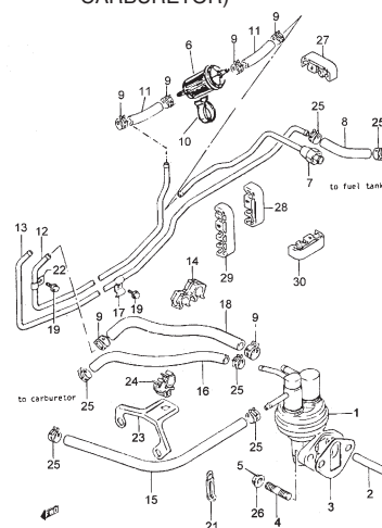
FIG.34 FUEL PUMP (GASOLINE: CARBURETOR)
