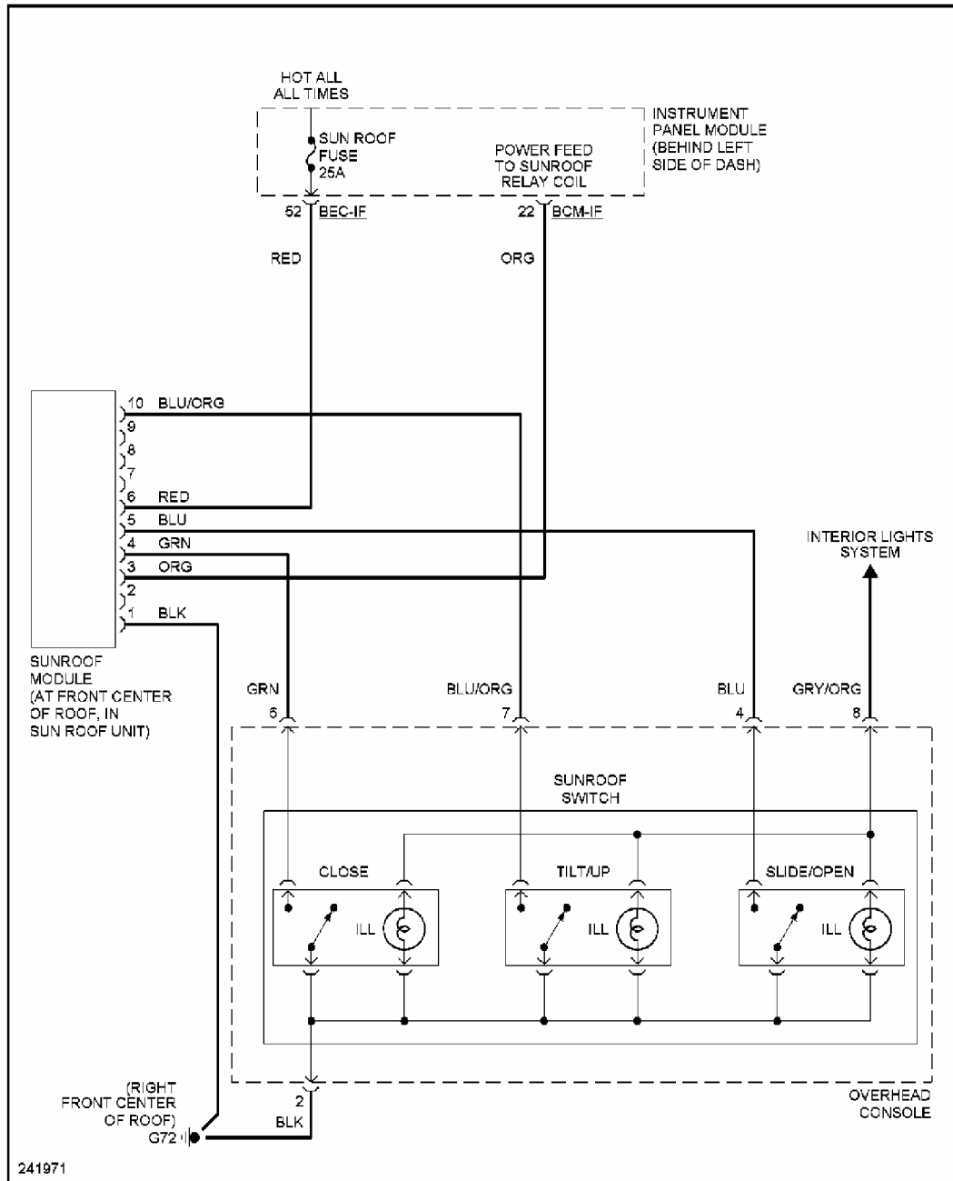
Fig. 62: Power Top/Sunroof Circuit
