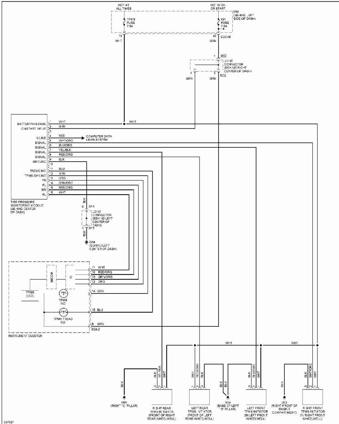
Fig. 78: Tire Pressure Monitoring Circuit
