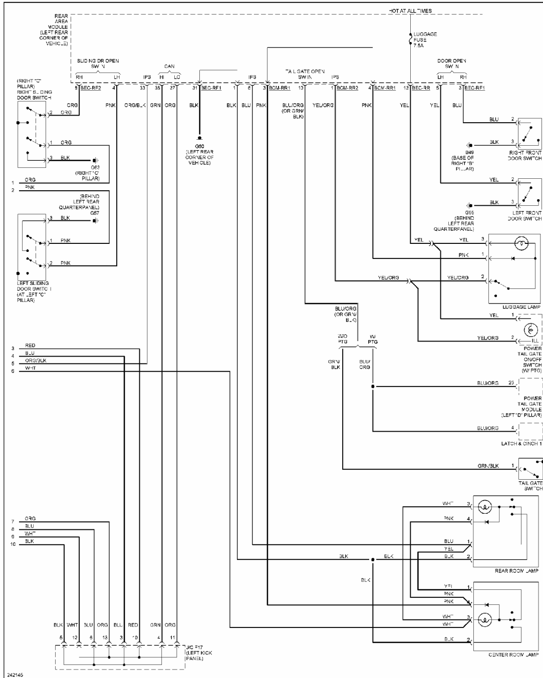
Fig. 43: Courtesy Lamps Circuit (2 of 2)
