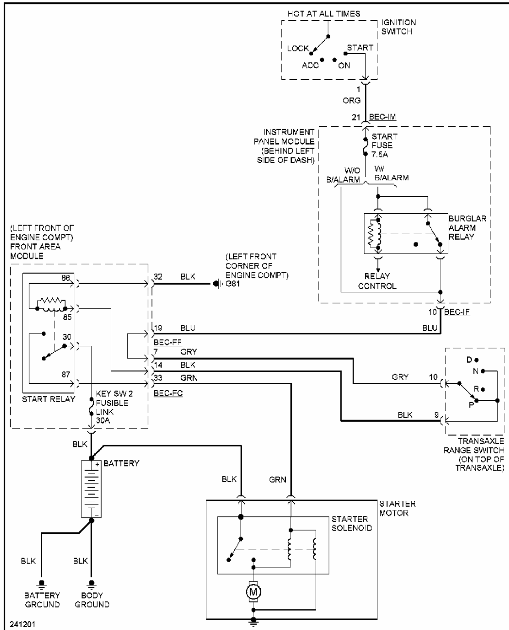
Fig. 70: Starting Circuit
