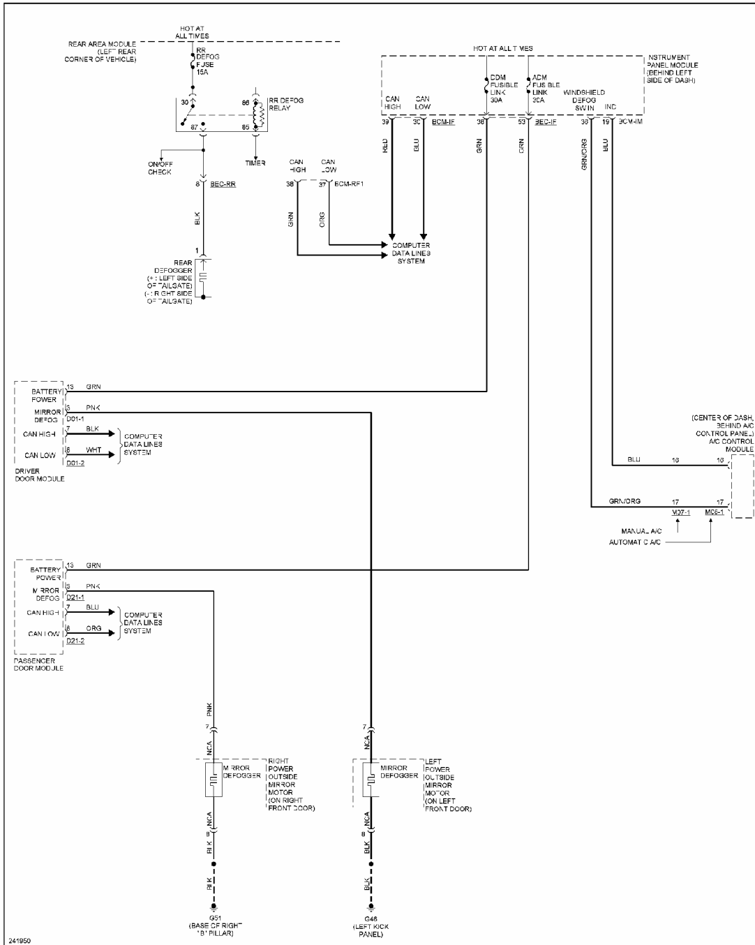
Fig. 23: Rear Defogger & Heated Mirrors Circuit
