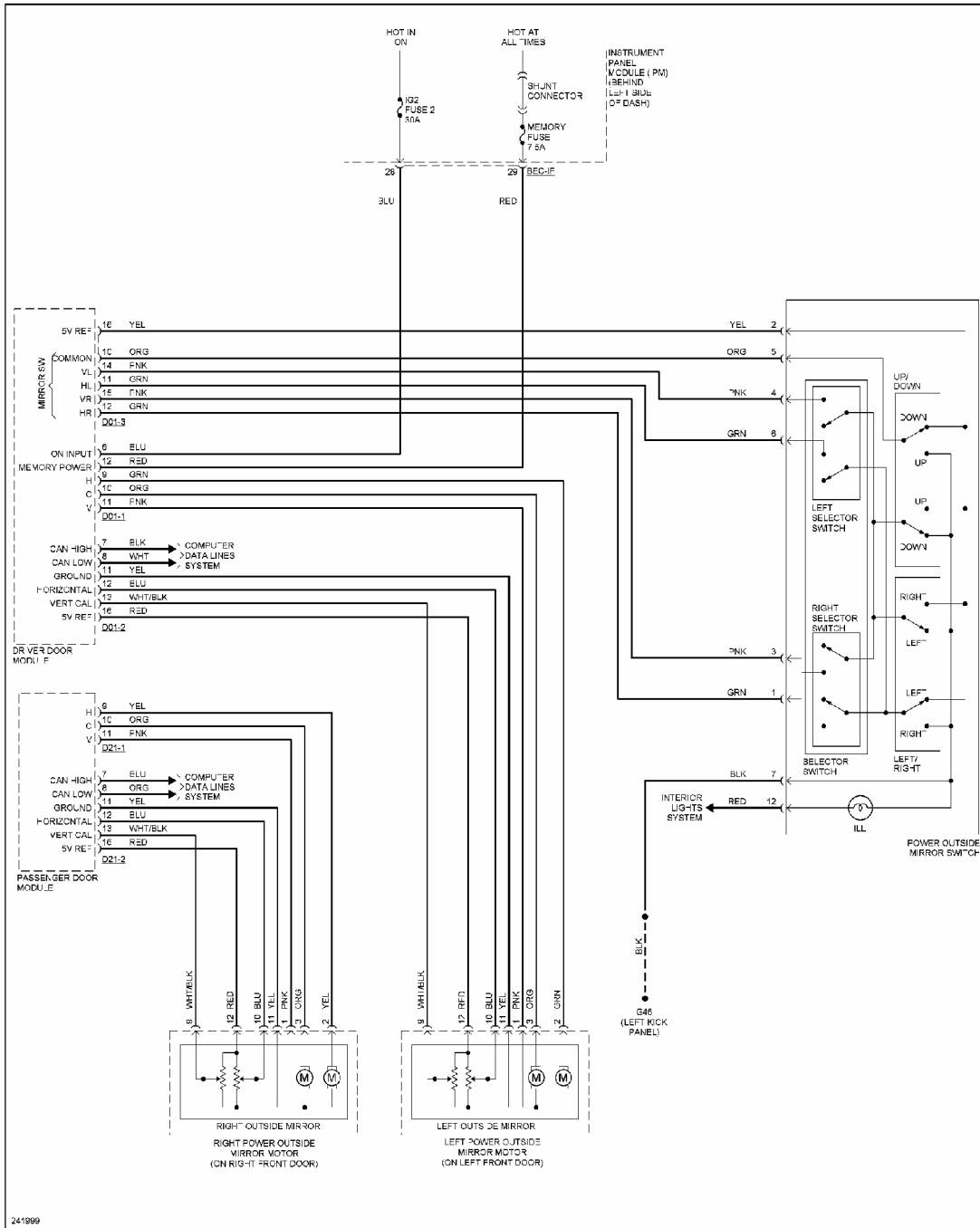
Fig. 48: Memory Mirrors Circuit
