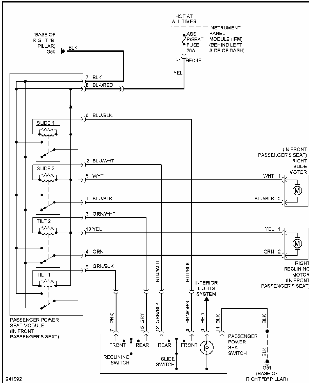
Fig. 61: Passenger Seat Circuit
