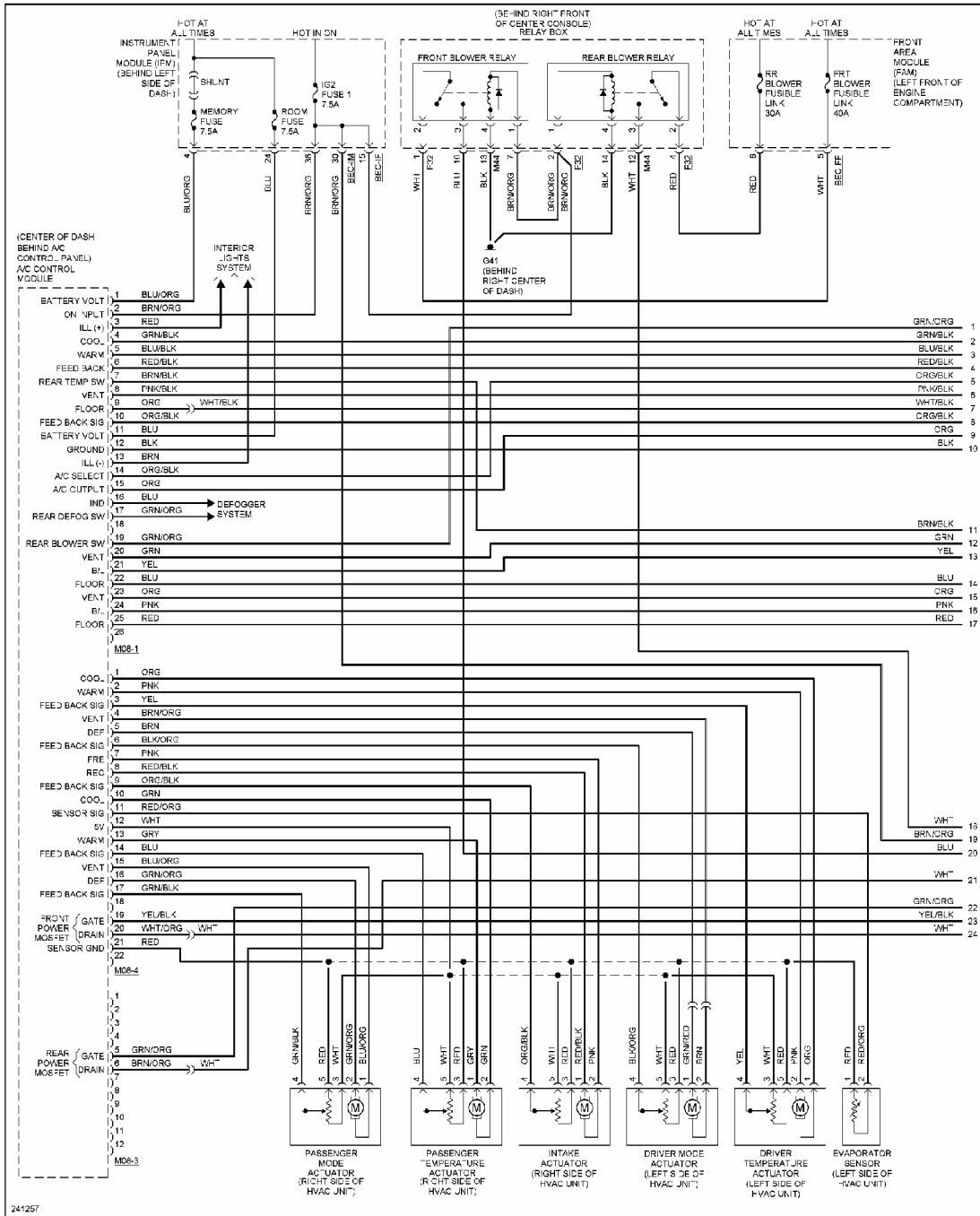
Fig. 1: Automatic A/C Circuit (1 of 3)
