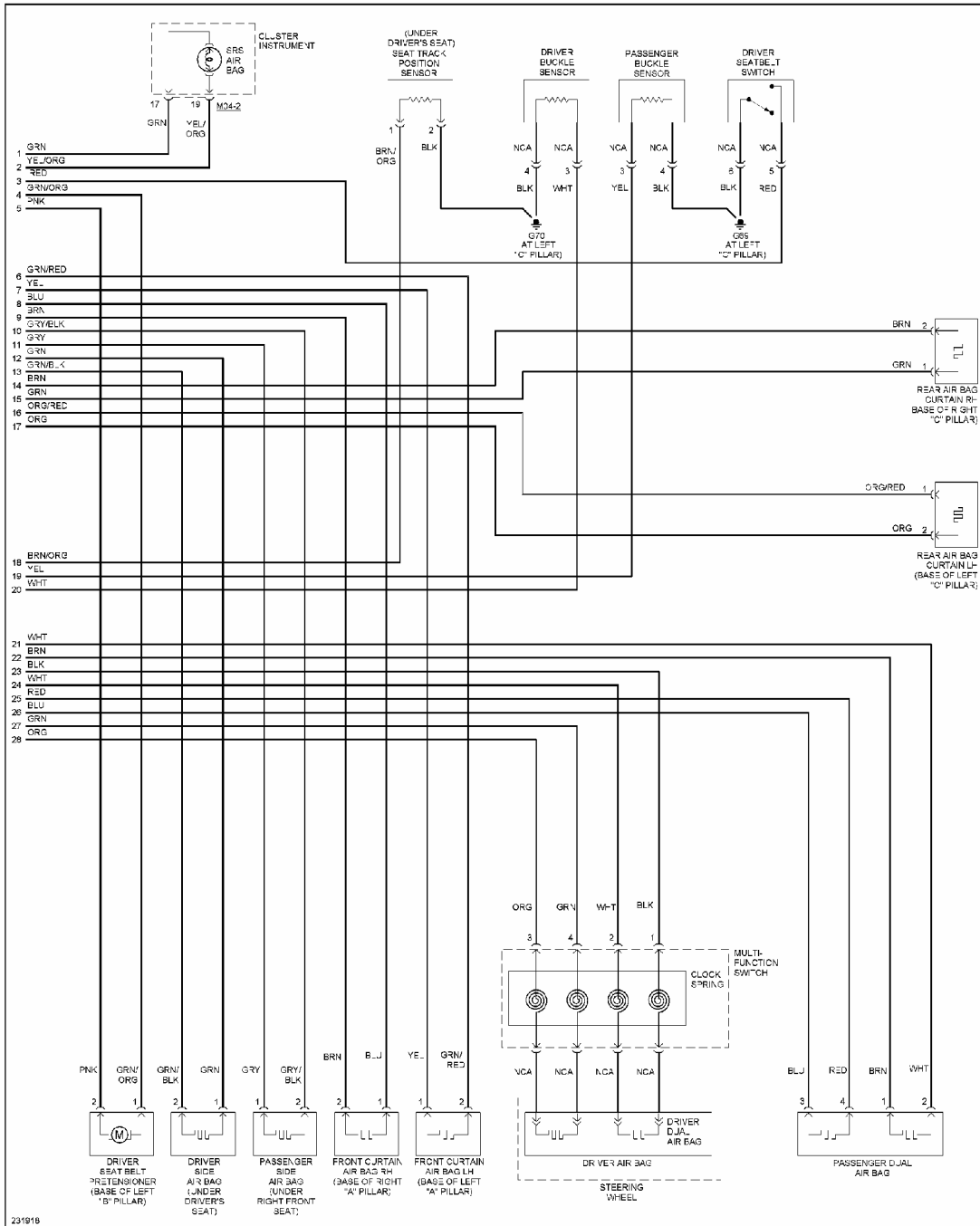
Fig. 72: Supplemental Restraints Circuit (2 of 2)
