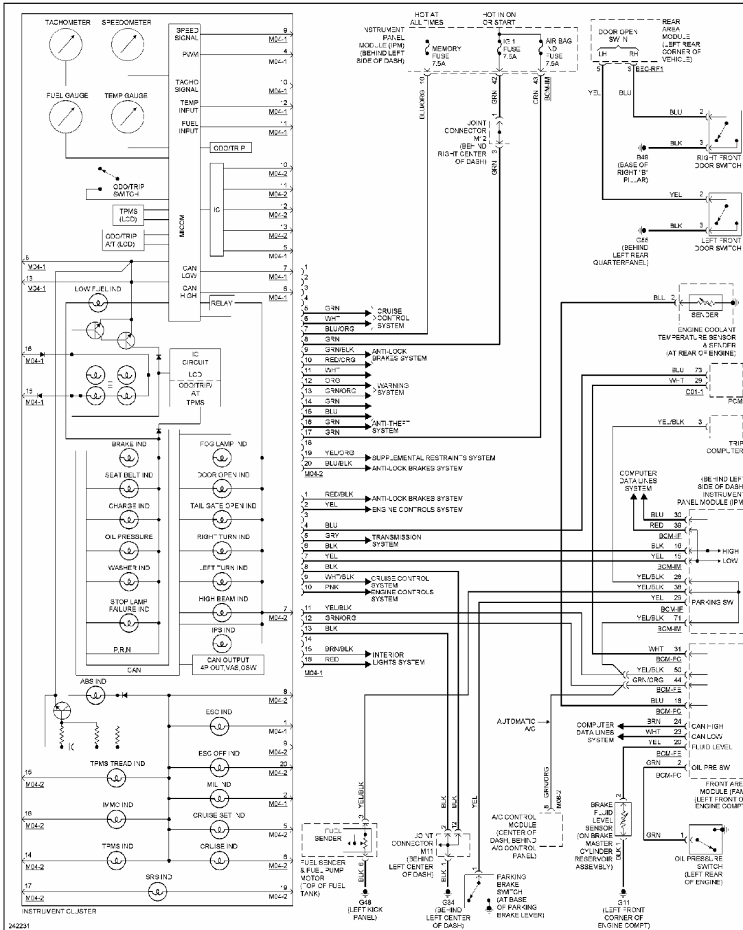
Fig. 40: Instrument Cluster Circuit, W/O Super Vision
