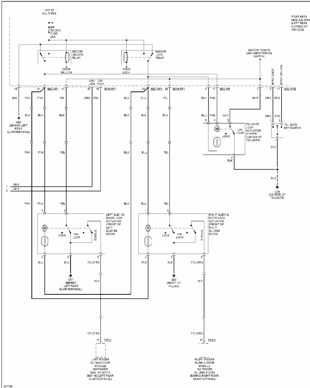
Fig. 55: Power Door Locks Circuit (2 of 2)
