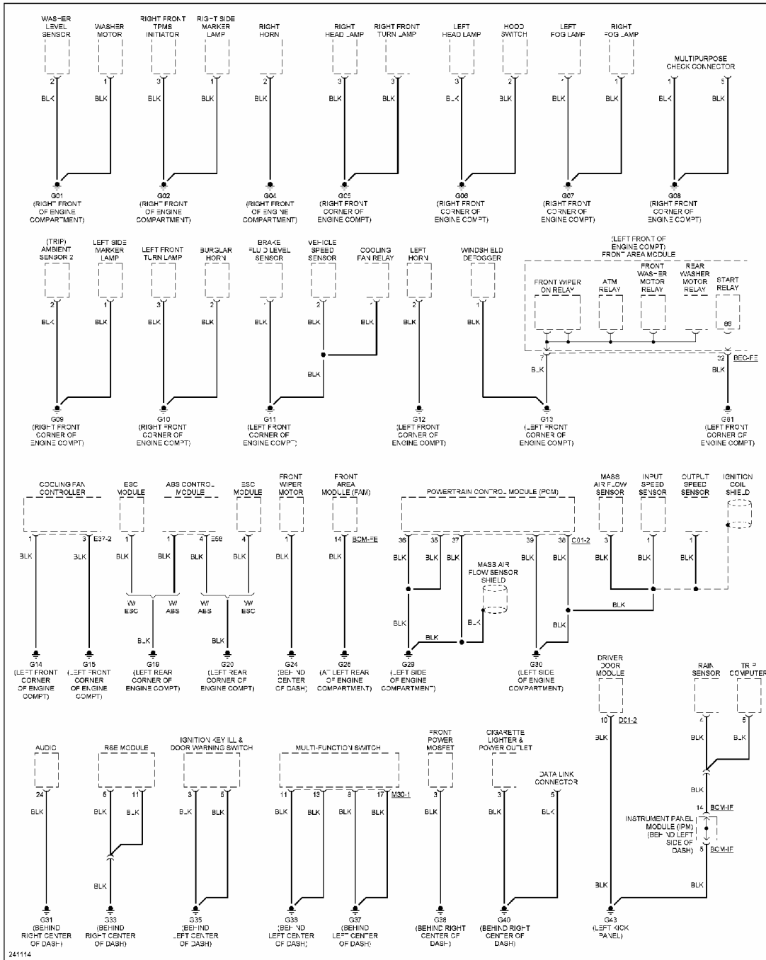
Fig. 32: Ground Distribution Circuit (1 of 4)
