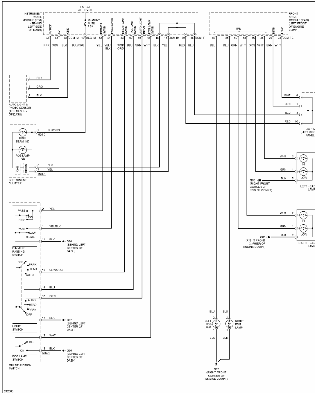
Fig. 36: Headlamps Circuit
