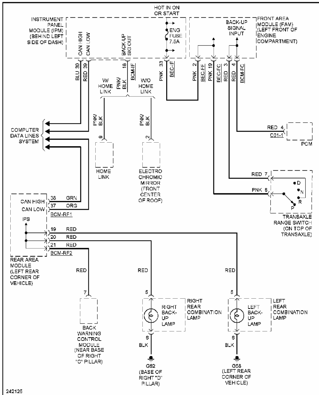
Fig. 29: Back-up Lamps Circuit
