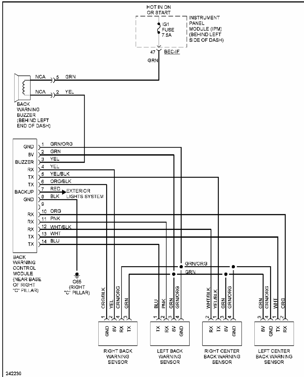
Fig. 49: Parking Assistant Circuit
