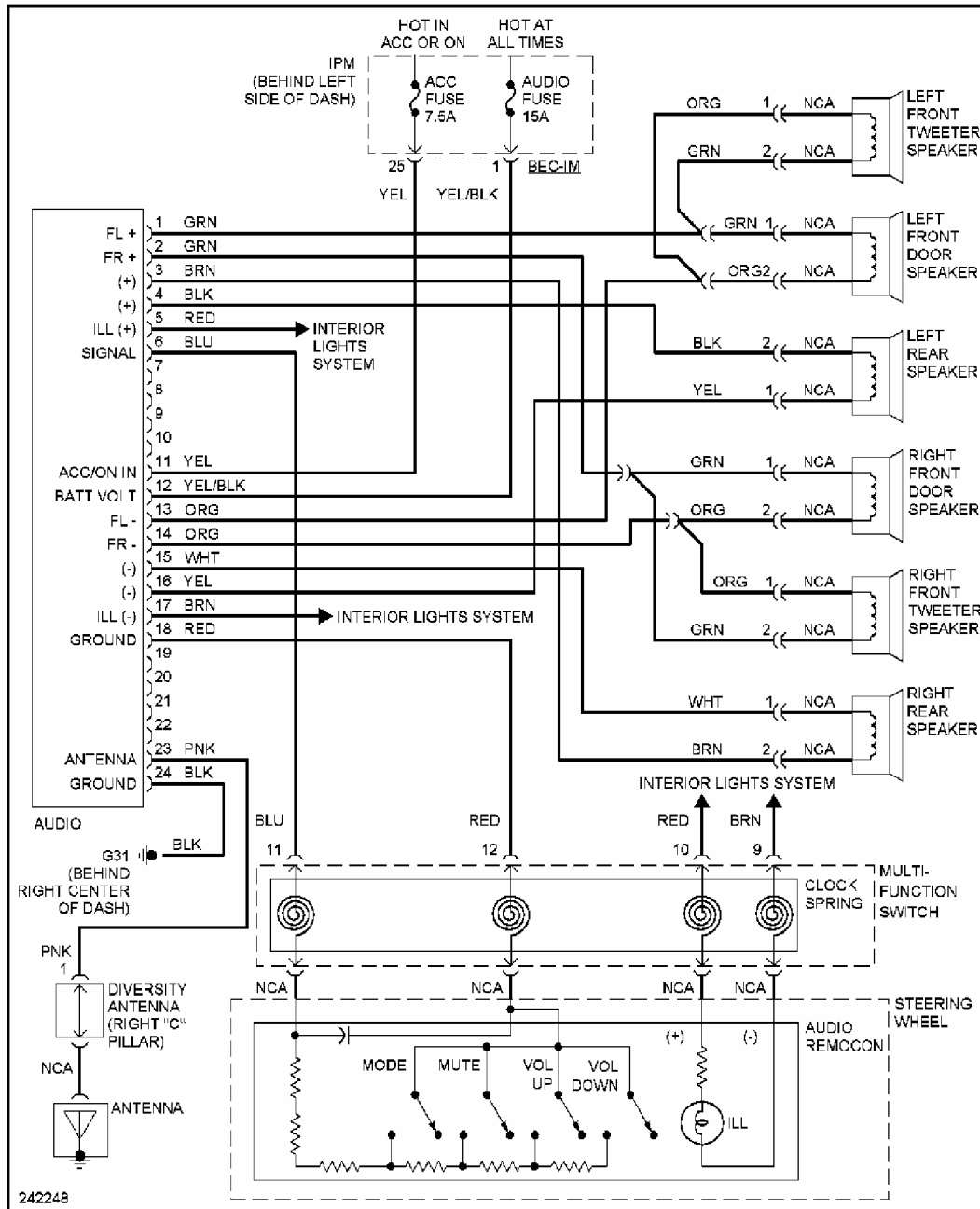
Fig. 65: Base Radio Circuit
