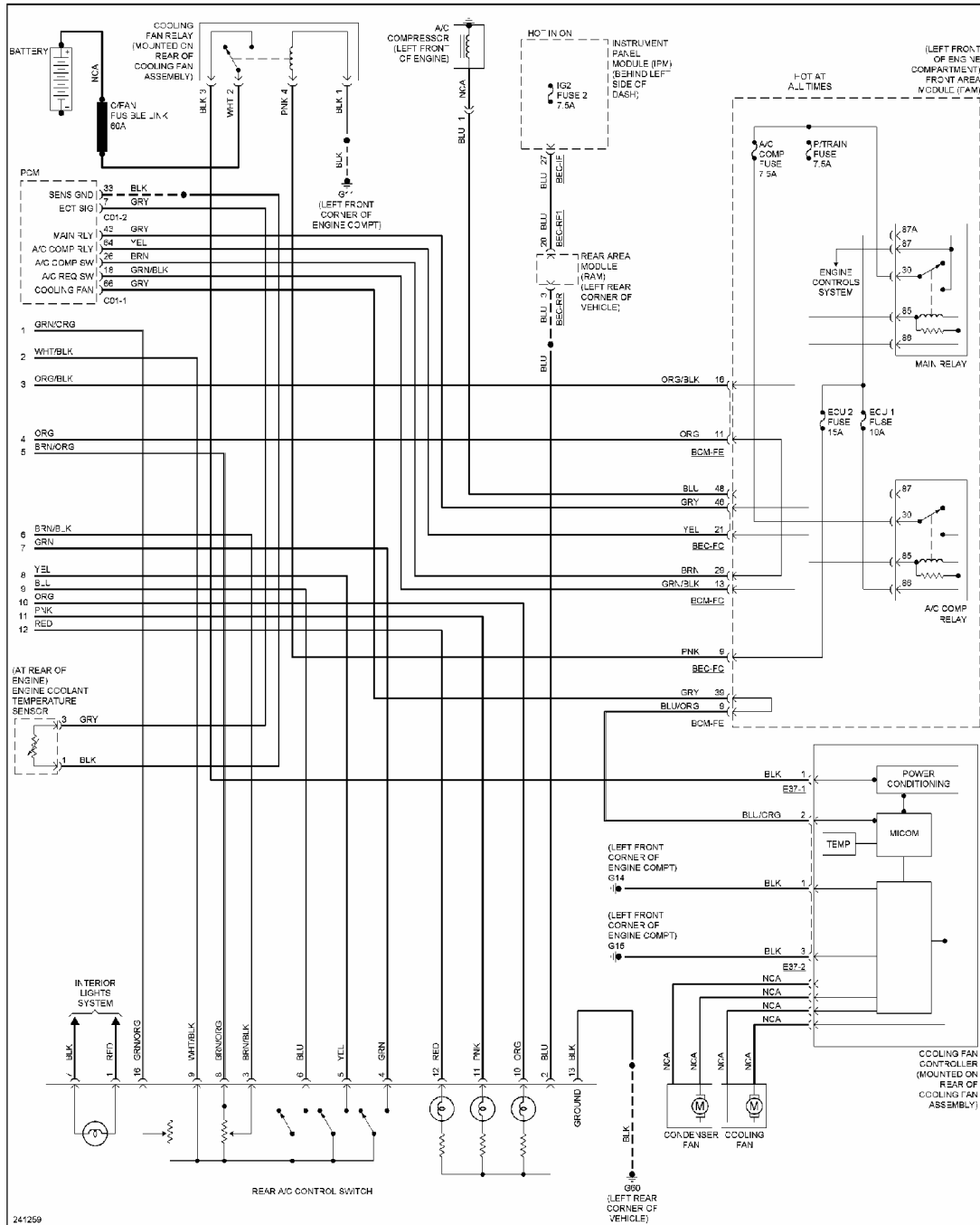
Fig. 3: Automatic A/C Circuit (3 of 3)
