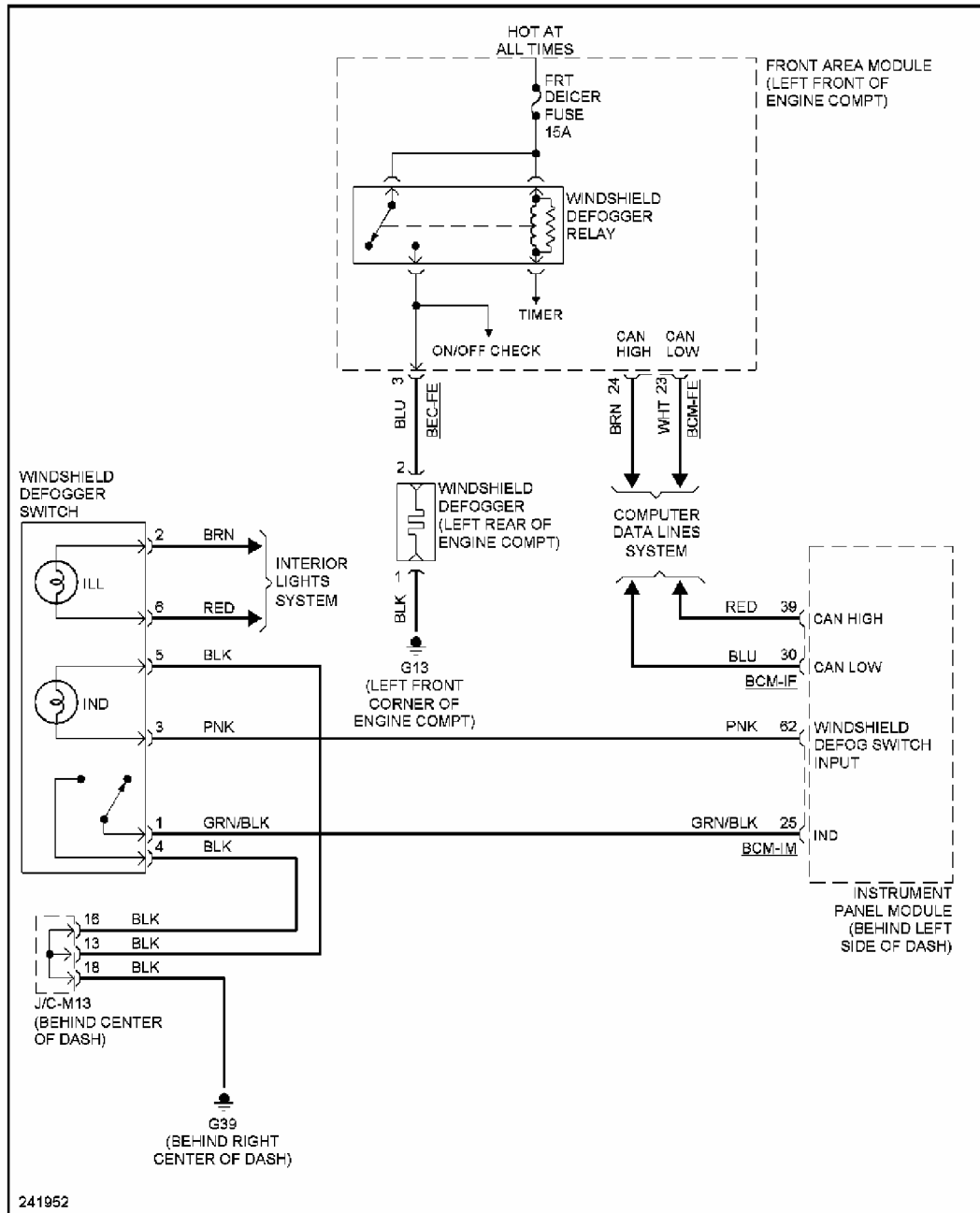
Fig. 22: Heated Windshield Circuit
