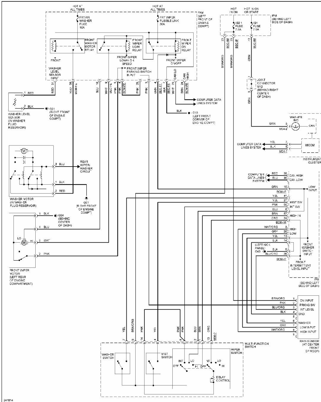
Fig. 80: Front Wiper/Washer Circuit
