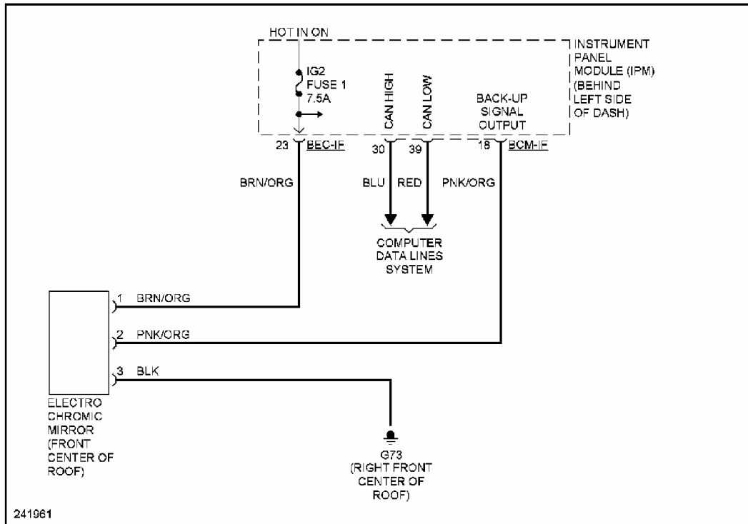
Fig. 56: Electrochromic Mirror Circuit
