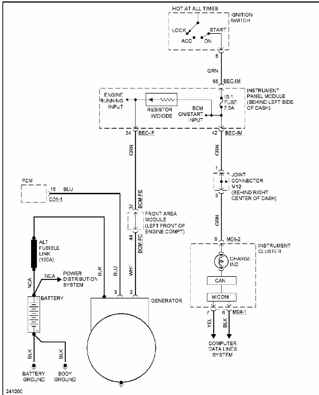
Fig. 69: Charging Circuit
