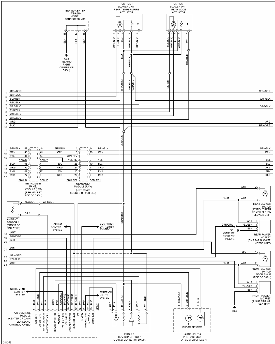
Fig. 2: Automatic A/C Circuit (2 of 3)
