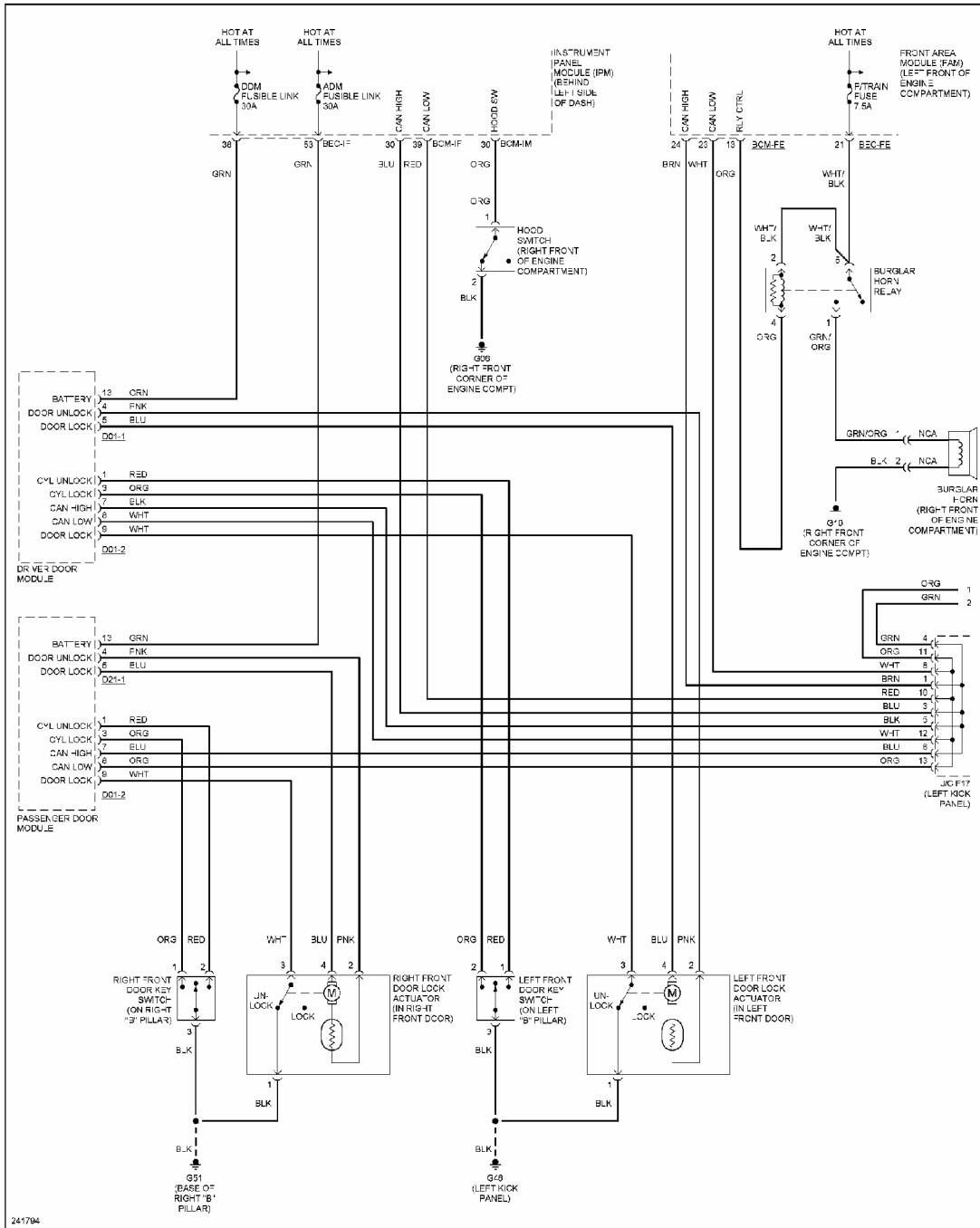
Fig. 9: Forced Entry Circuit (1 of 2)
