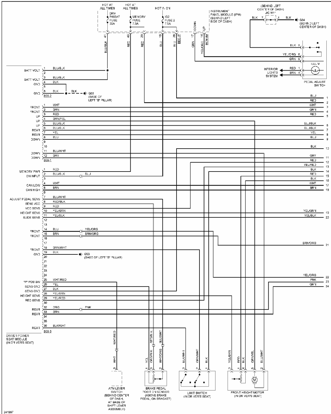
Fig. 46: Driver's Memory Seat Circuit (1 of 2)
