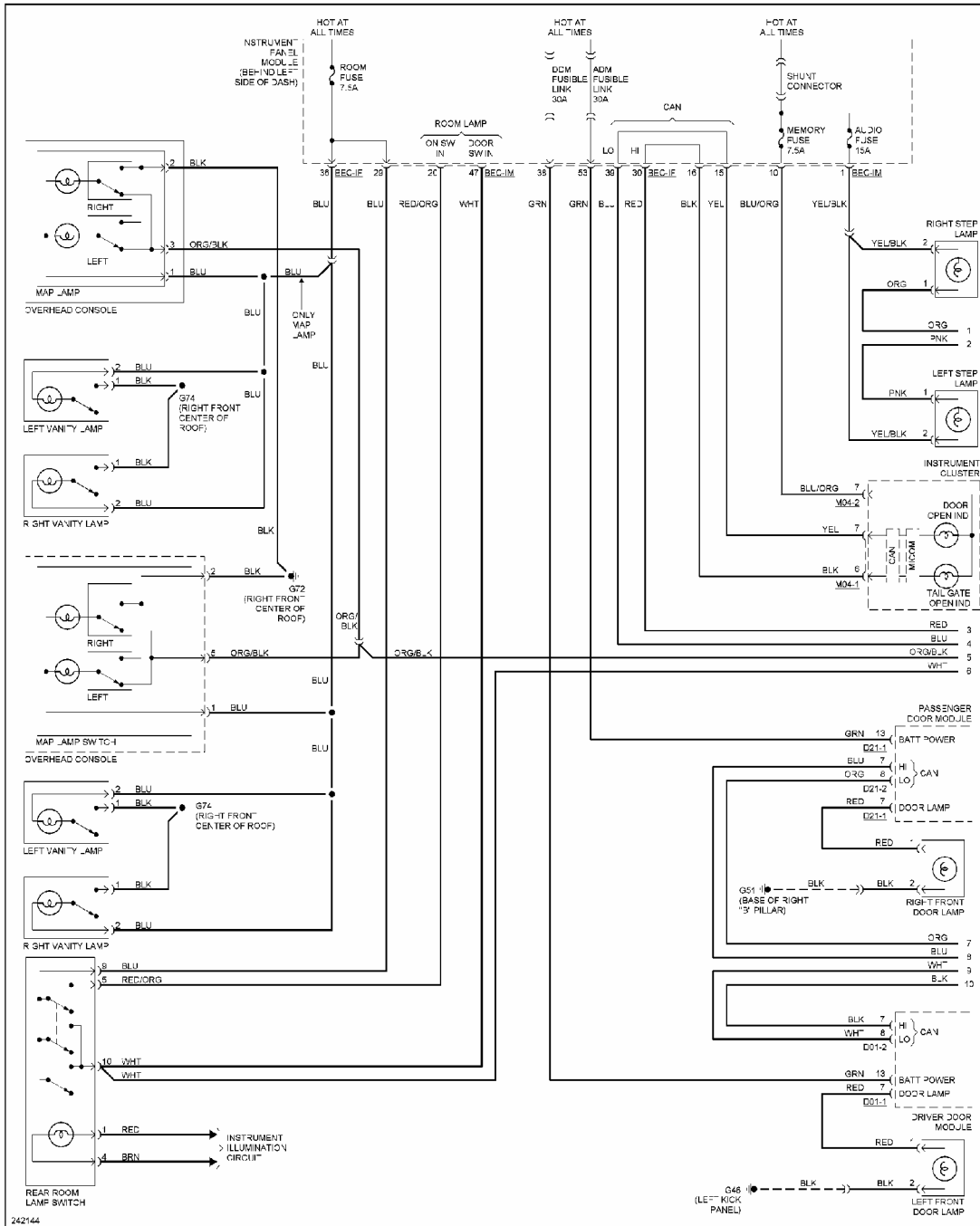
Fig. 42: Courtesy Lamps Circuit (1 of 2)
