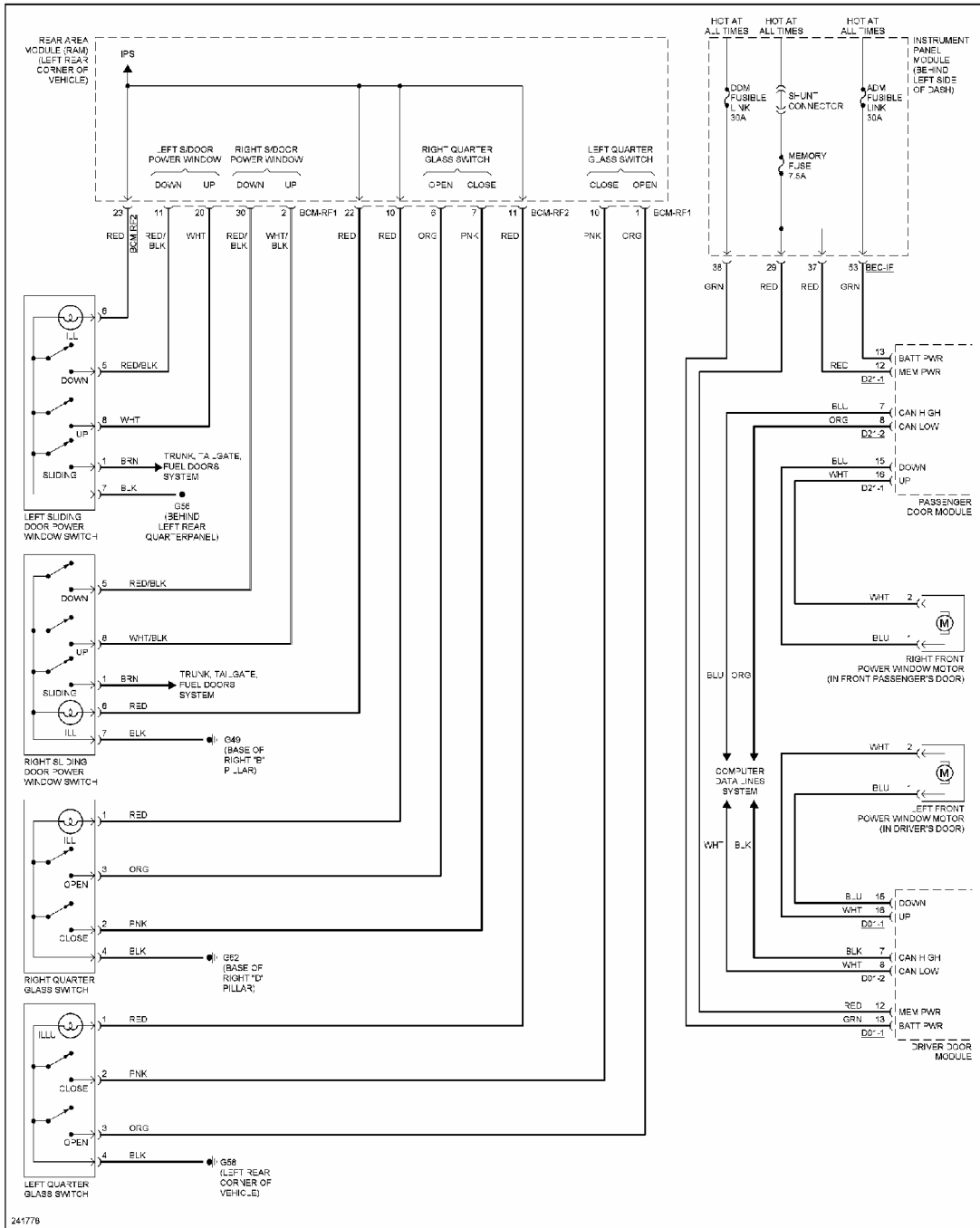
Fig. 64: Power Windows Circuit (2 of 2)
