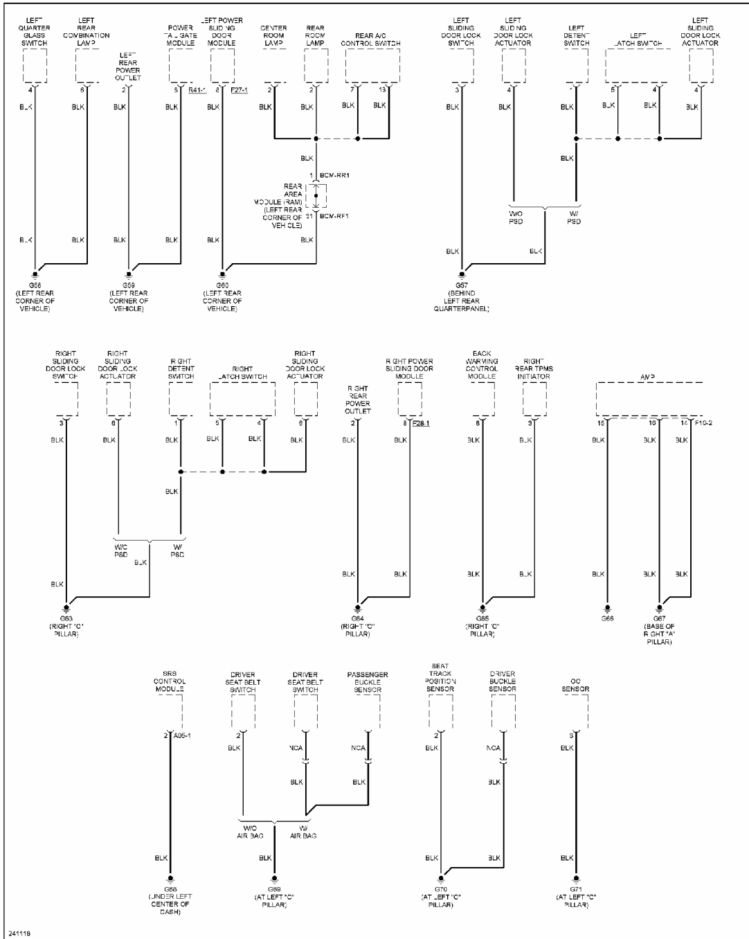
Fig. 35: Ground Distribution Circuit (4 of 4)
