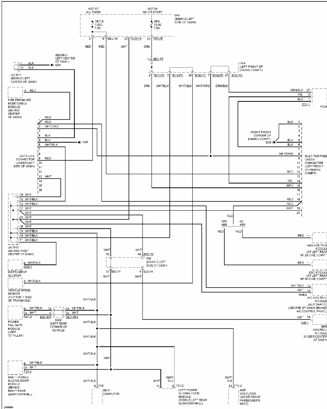
Fig. 18: Computer Data Lines Circuit
