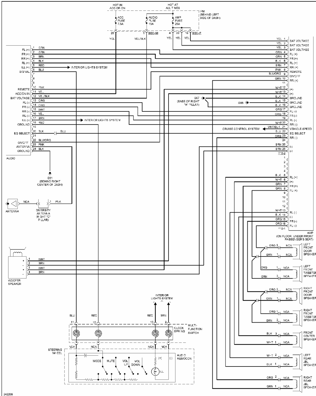
Fig. 67: Radio Circuit, W/O Rear Seat Entertainment
