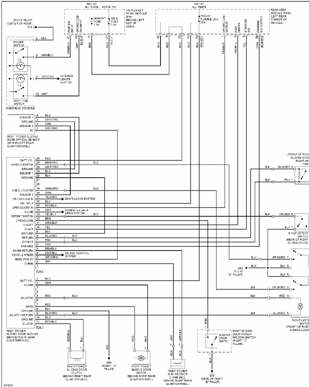
Fig. 76: Passenger Side Power Sliding Door Circuit
