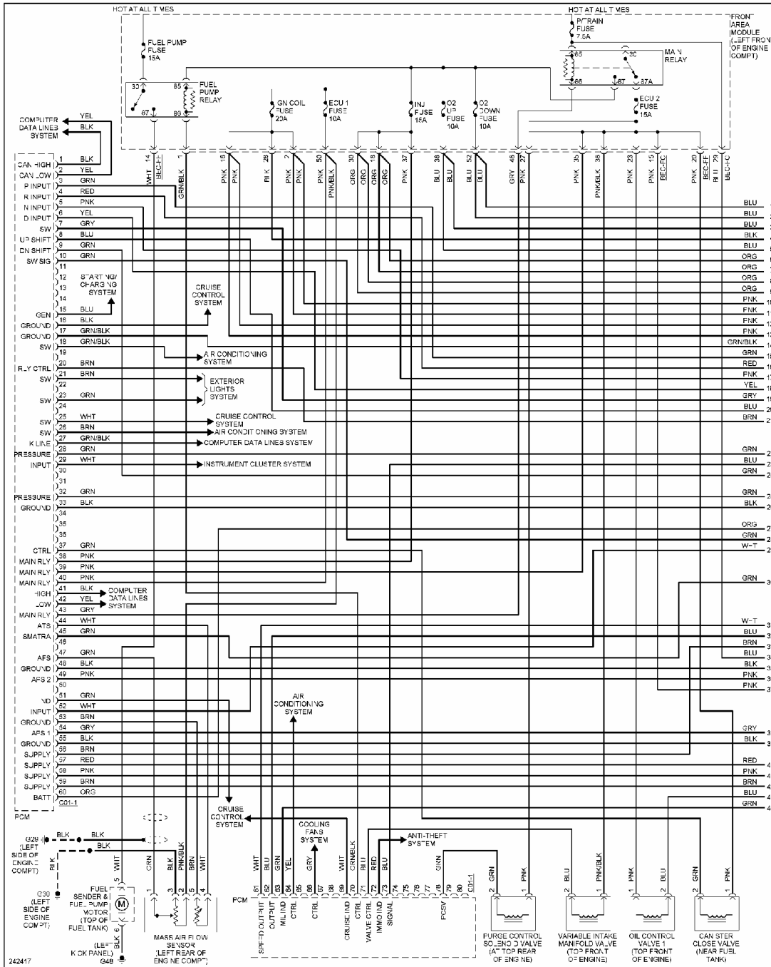
Fig. 24: 3.8L, Engine Performance Circuit (1 of 5)
