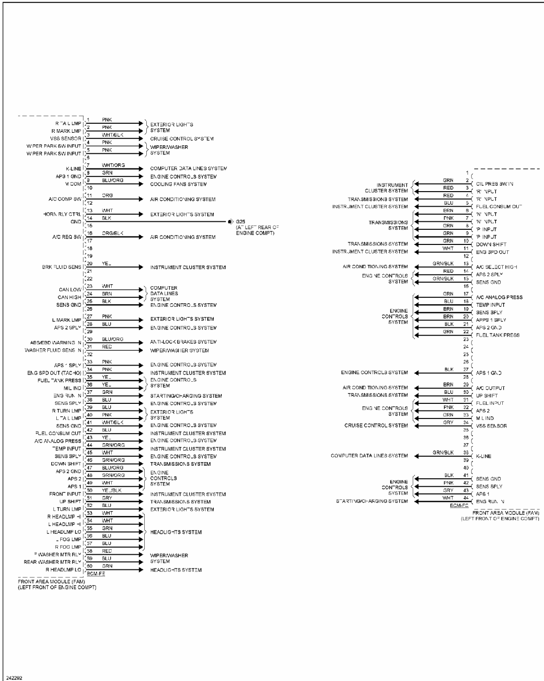
Fig. 13: Front Area Module Circuit (2 of 2)
