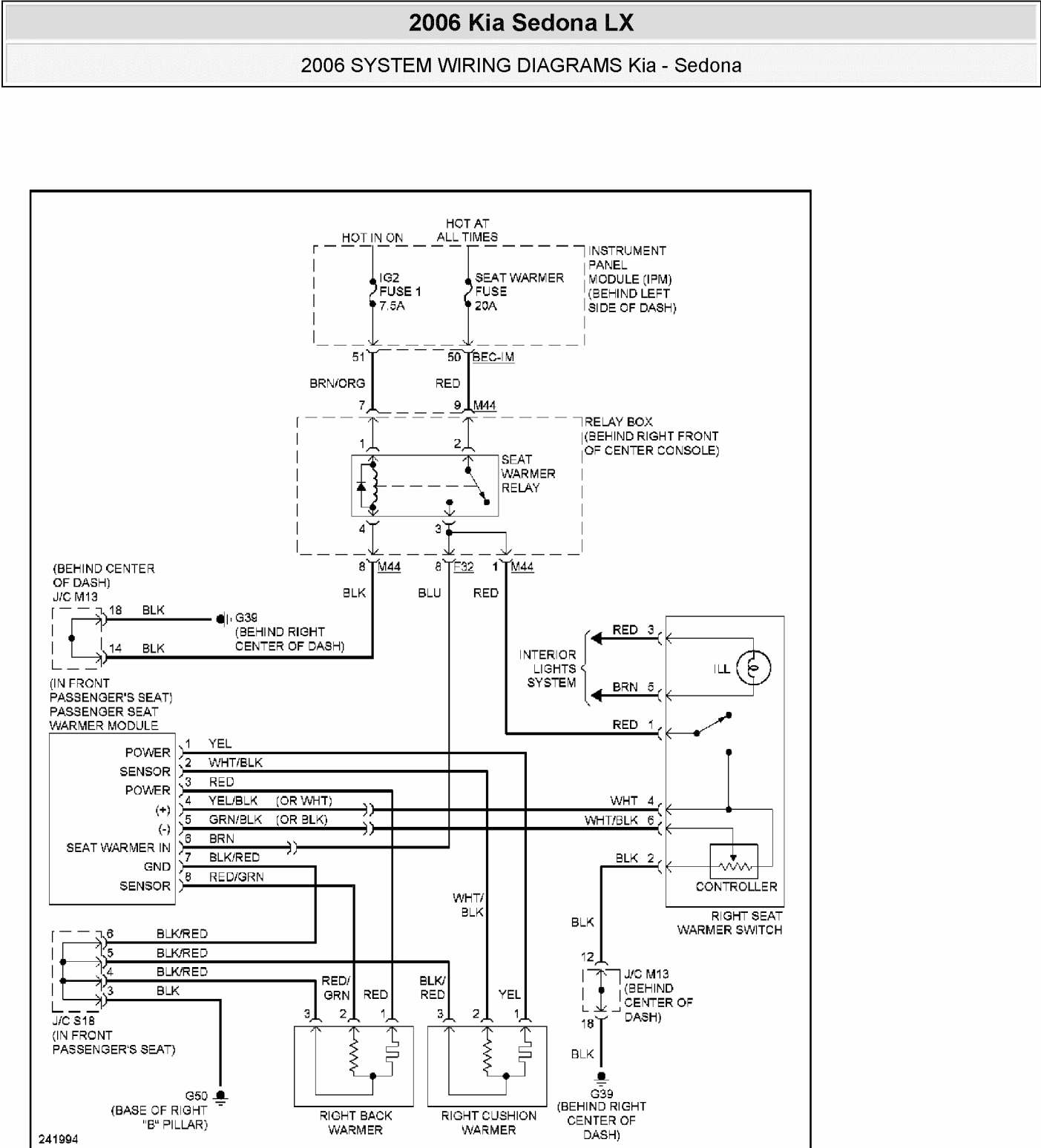
Fig. 60: Passenger Heated Seat Circuit
