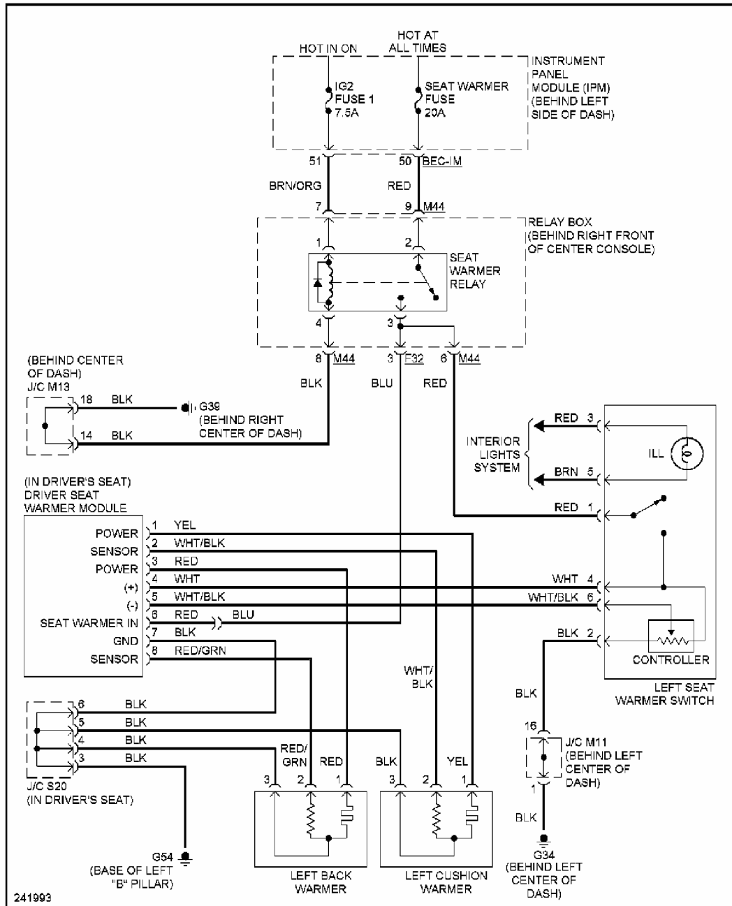
Fig. 58: Driver Heated Seat Circuit
