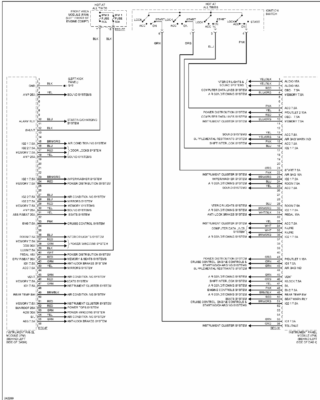
Fig. 14: Instrument Panel Module Circuit (1 of 2)
