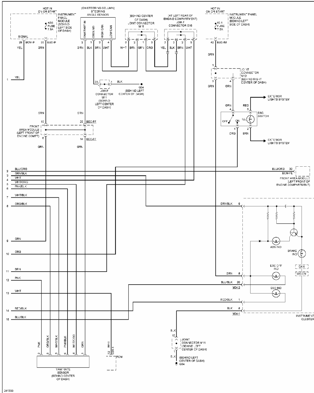
Fig. 7: Anti-lock Brakes Circuit, W/ ESC (2 of 2)
