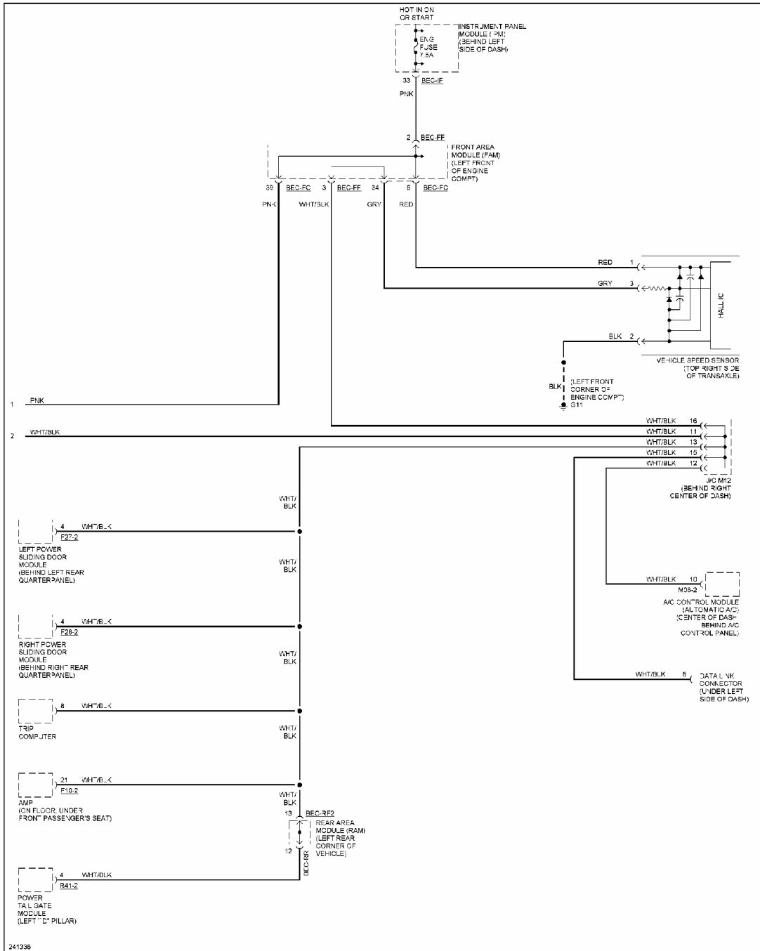
Fig. 21: Cruise Control Circuit (2 of 2)
