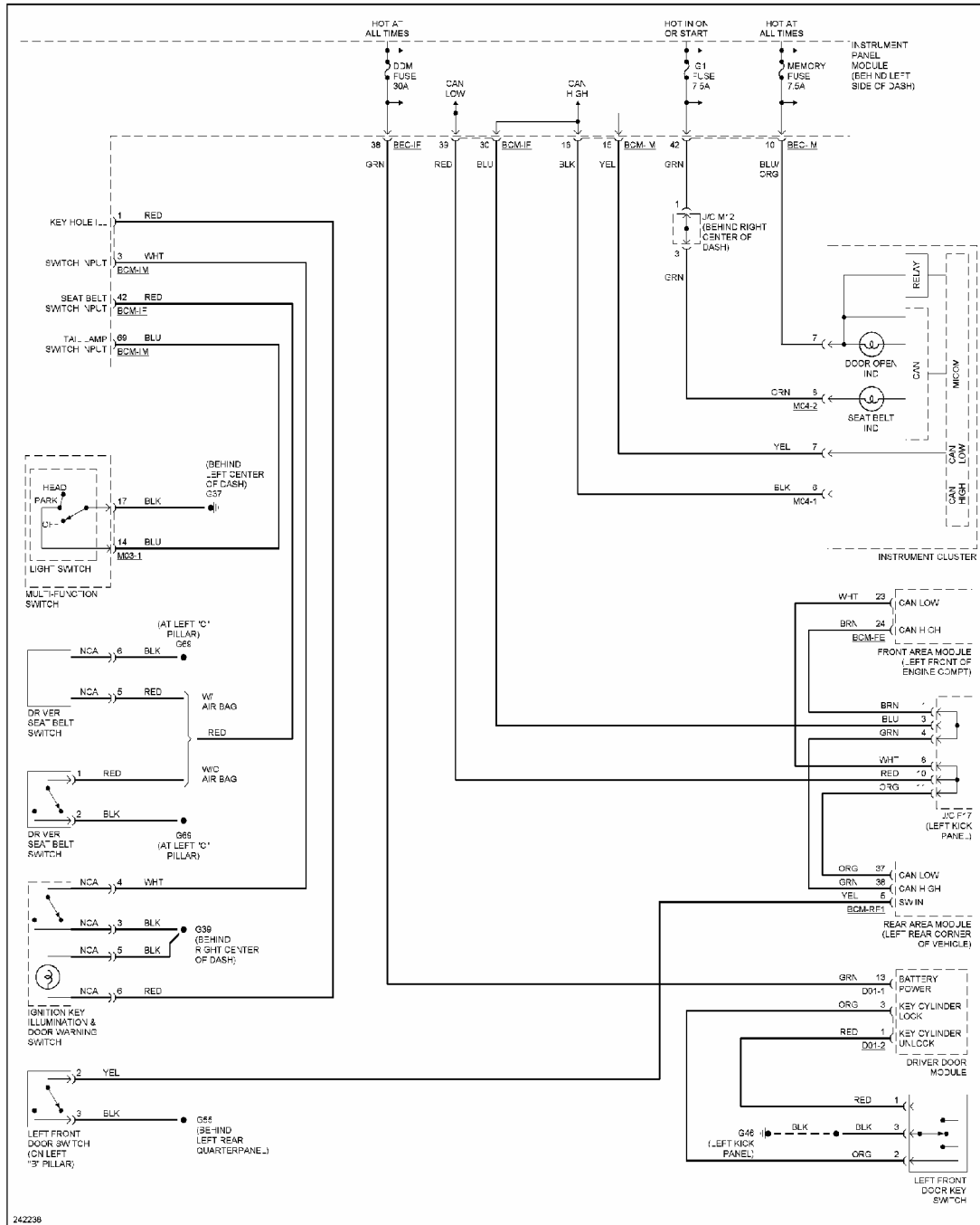
Fig. 79: Warning Systems Circuit
