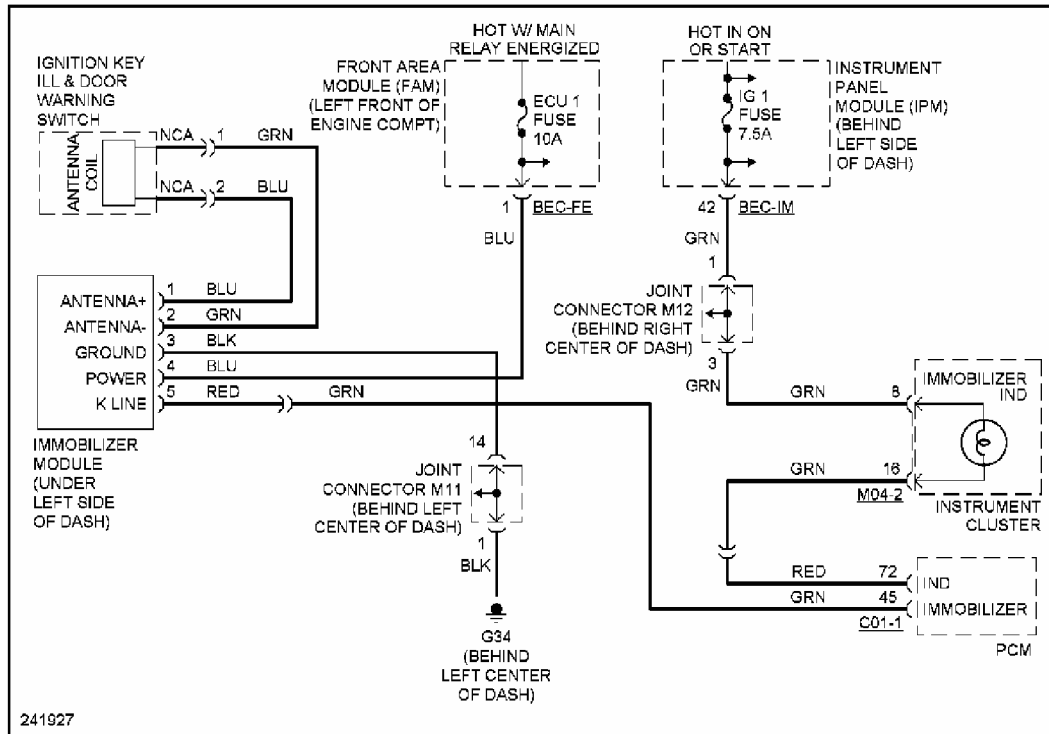
Fig. 11: Immobilizer Circuit
