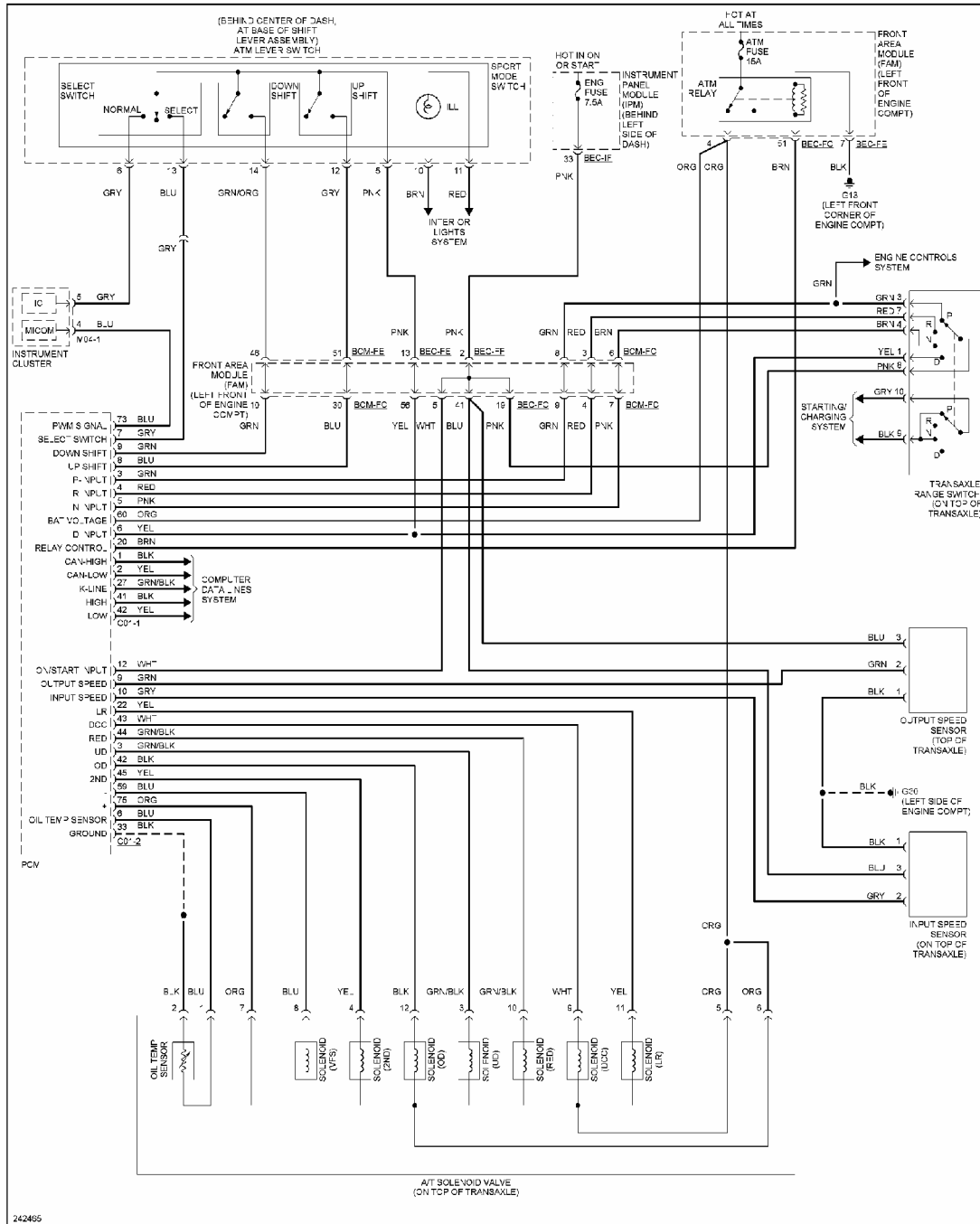
Fig. 73: Transmission Circuit
