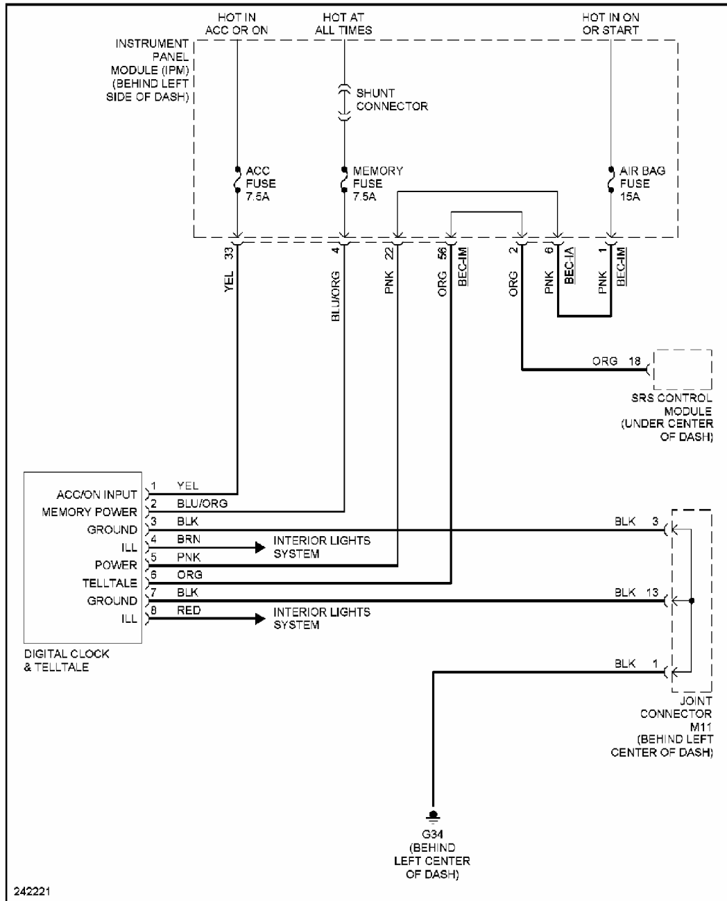
Fig. 38: Clock Circuit
