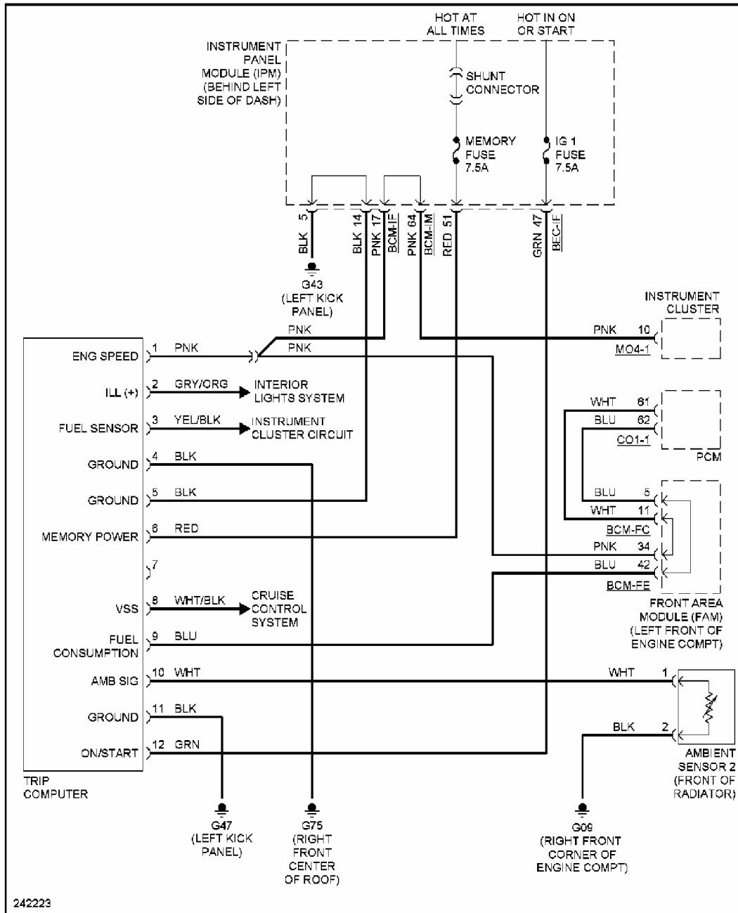
Fig. 41: Trip Computer Circuit
