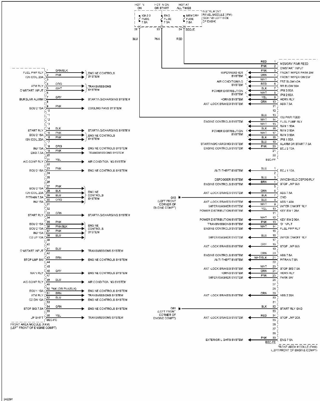
Fig. 12: Front Area Module Circuit (1 of 2)
