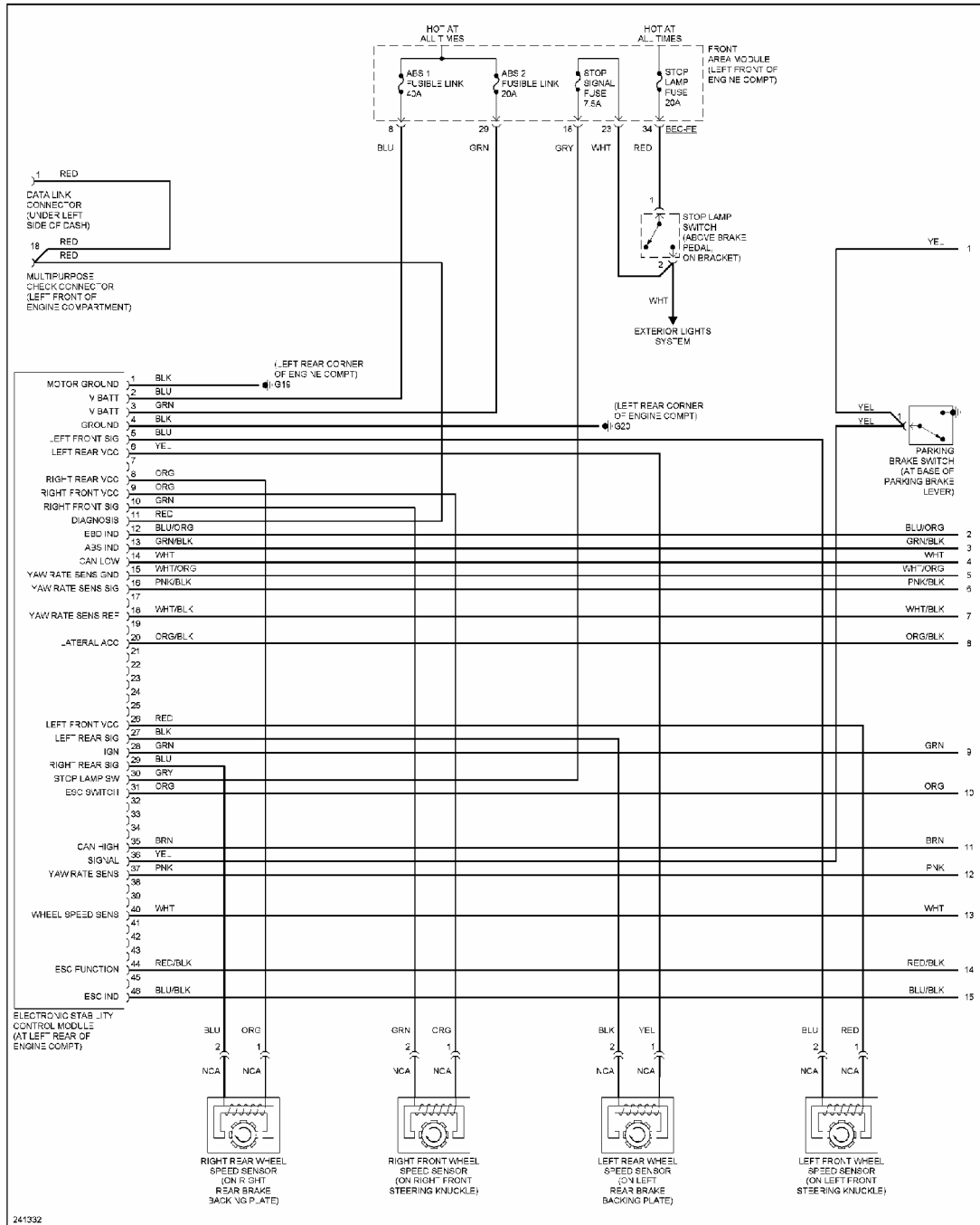
Fig. 6: Anti-lock Brakes Circuit, W/ ESC (1 of 2)
