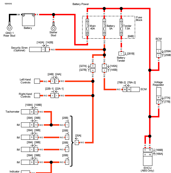
Battery Power Distribution
