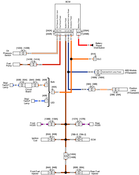
Ignition and Accessory Power Distribution
