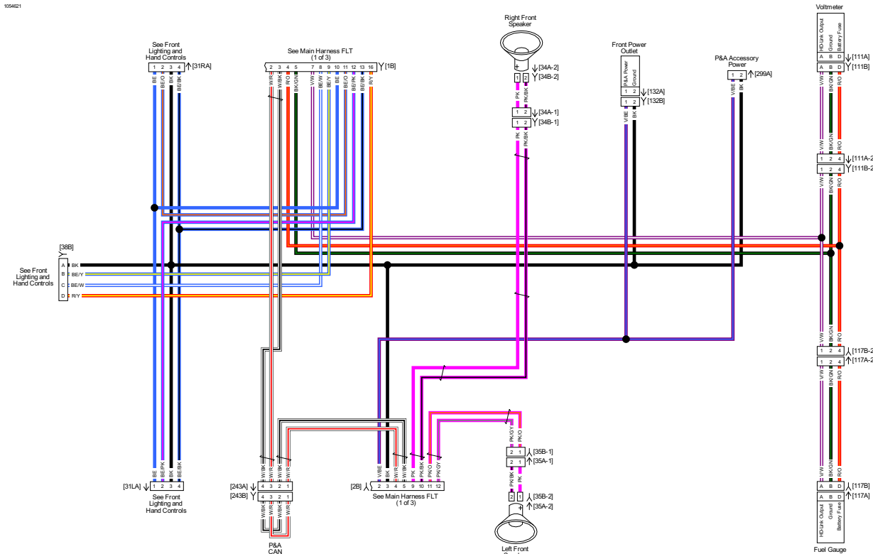
Fairing Harness FLT: 2018 Touring
