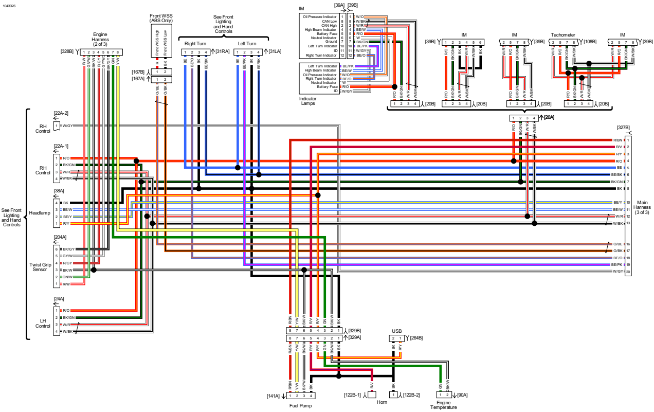
Backbone Harness 1 of 3: 2018 Softail
