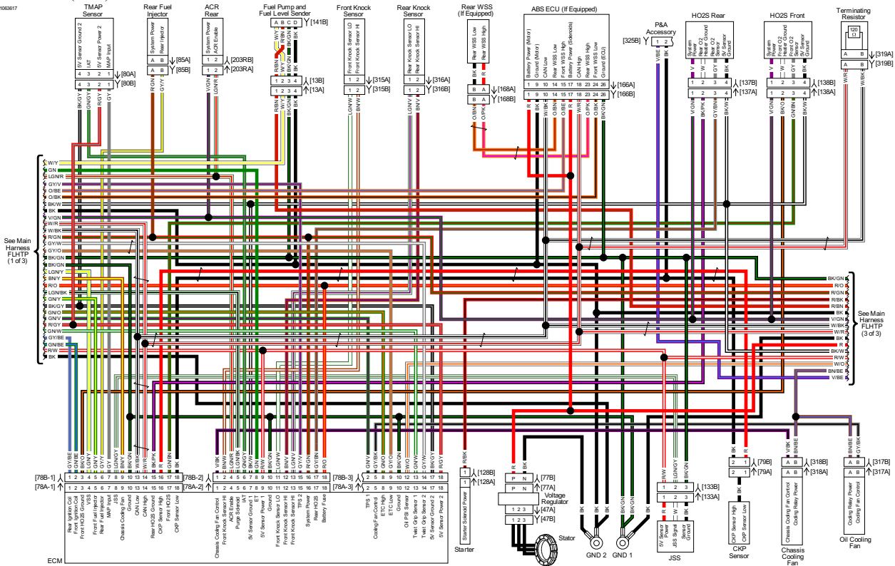
Main Harness (2 of 3): 2018 FLHTP
