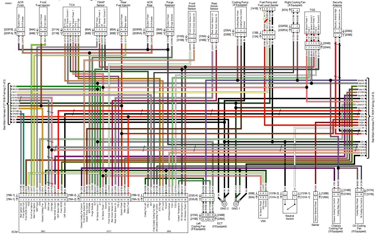
Main Harness FLT (2 of 3): 2018 Touring (with Fairing)
