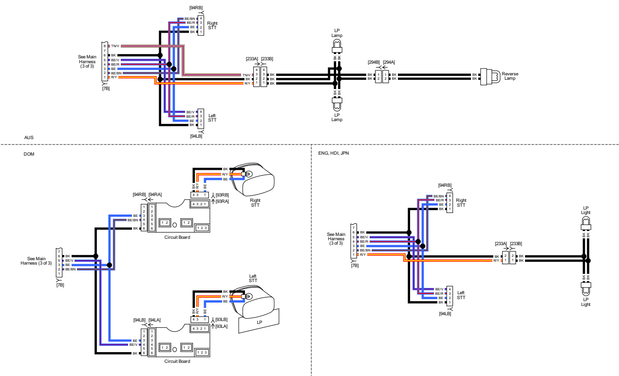
Rear Lighting: 2018 Trike Models (FLRT)
