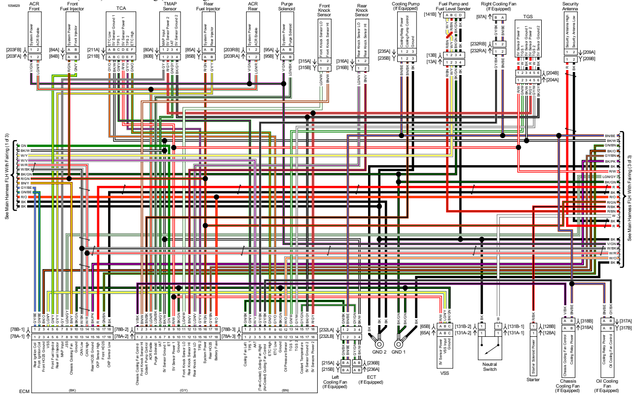
Main Harness FLH (2 of 3): 2018 Touring (with Fairing)
