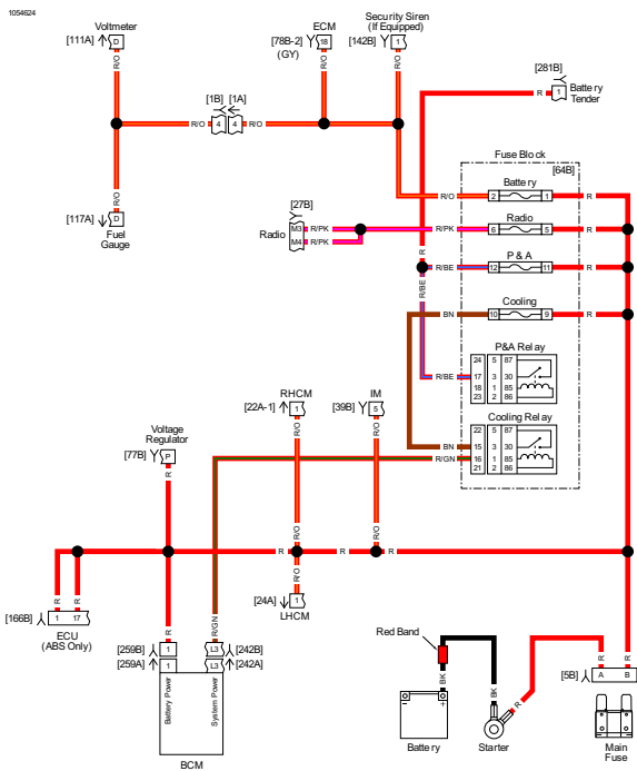
Battery Power Distribution: FLT
