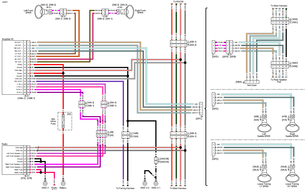
P&amp;A Radio with 1 Amp: 2018 Touring
