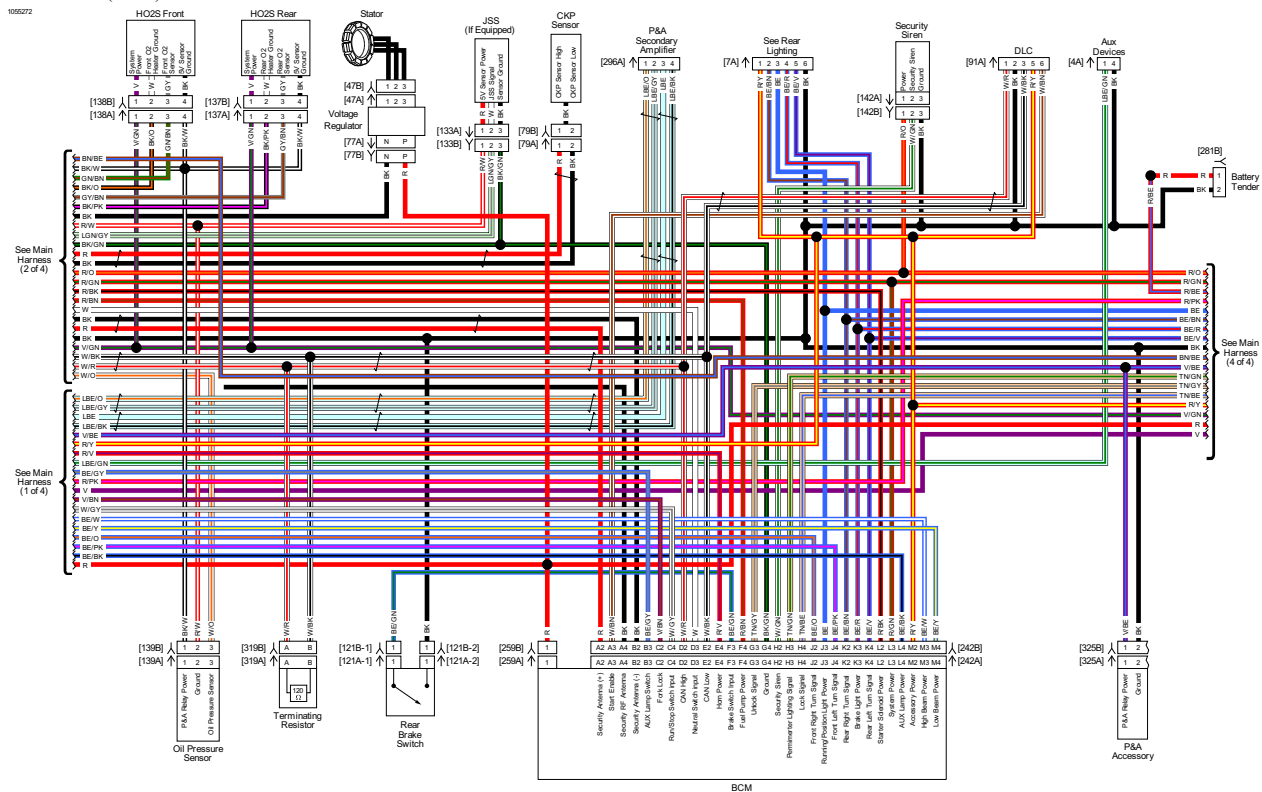
Main Harness (3 of 4): 2018 FLHTKSE
