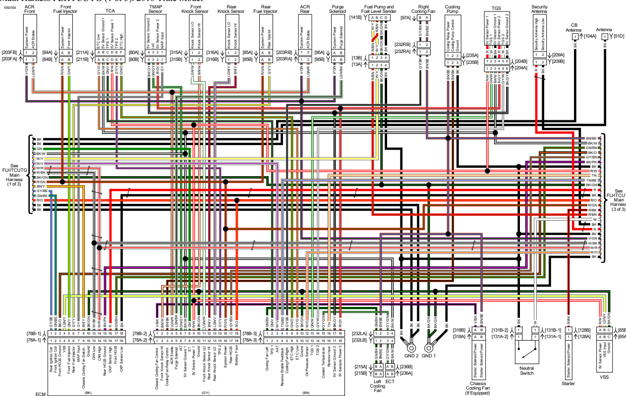
Main Harness FLHTCUTG (2 of 3): 2018 Trike Model
