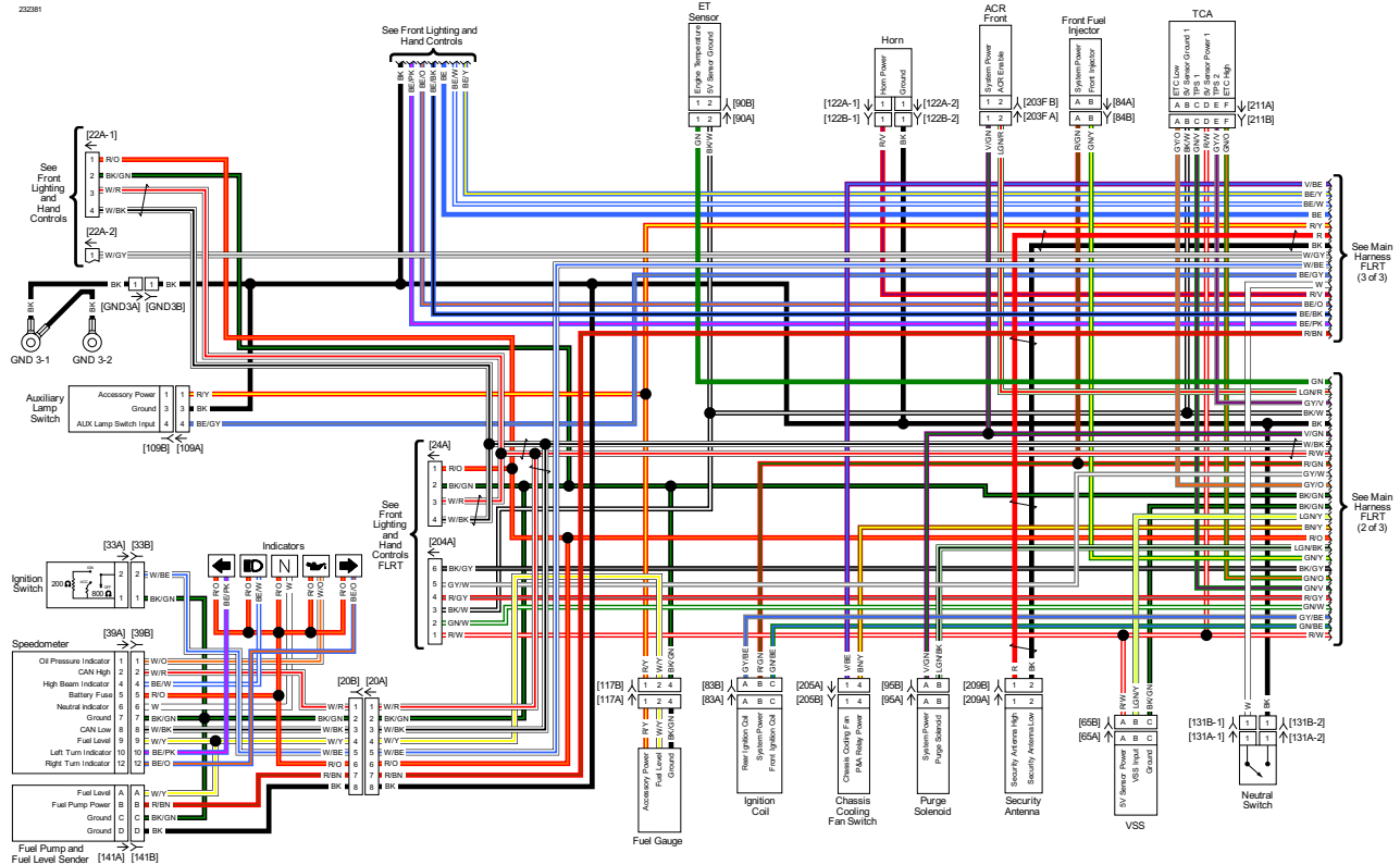
Main Harness FLRT (1 of 3): 2018 Trike Model
