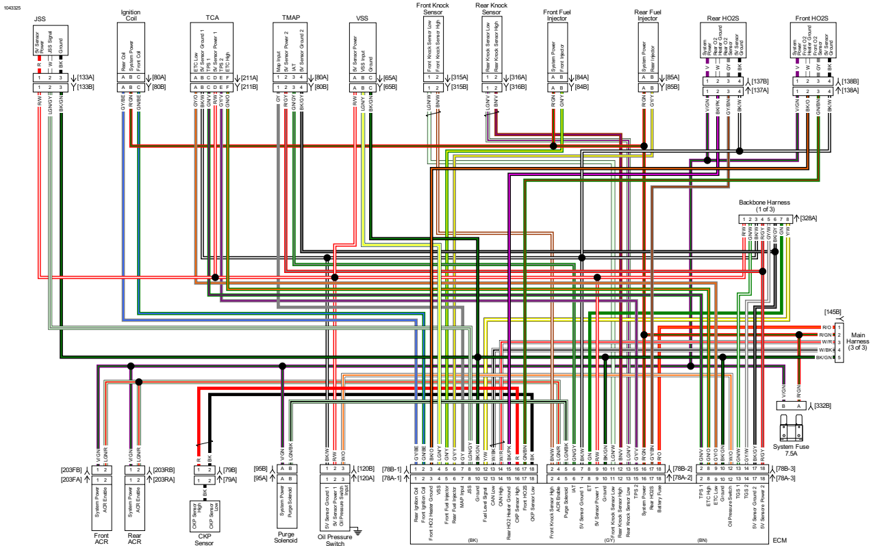
Engine Harness 2 of 3: 2018 Softail
