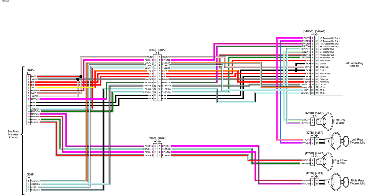
Radio (1 of 2): 2018 FLTRXSE
