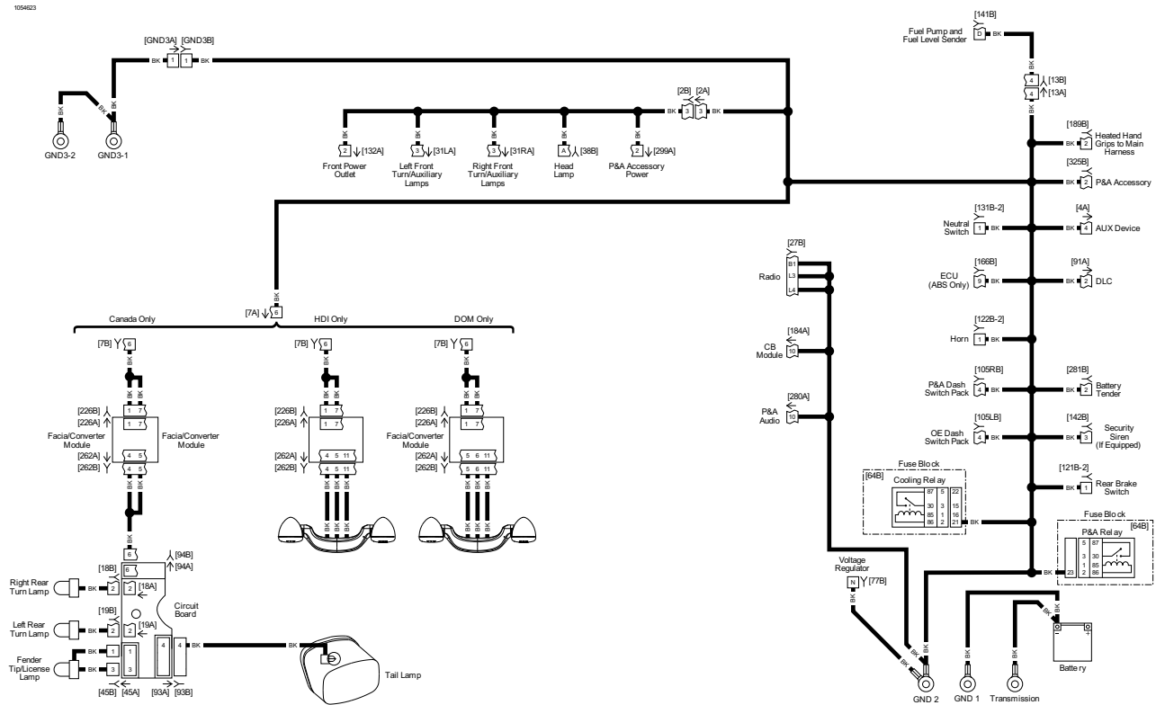
Ground Circuit FLT: 2018 Touring
