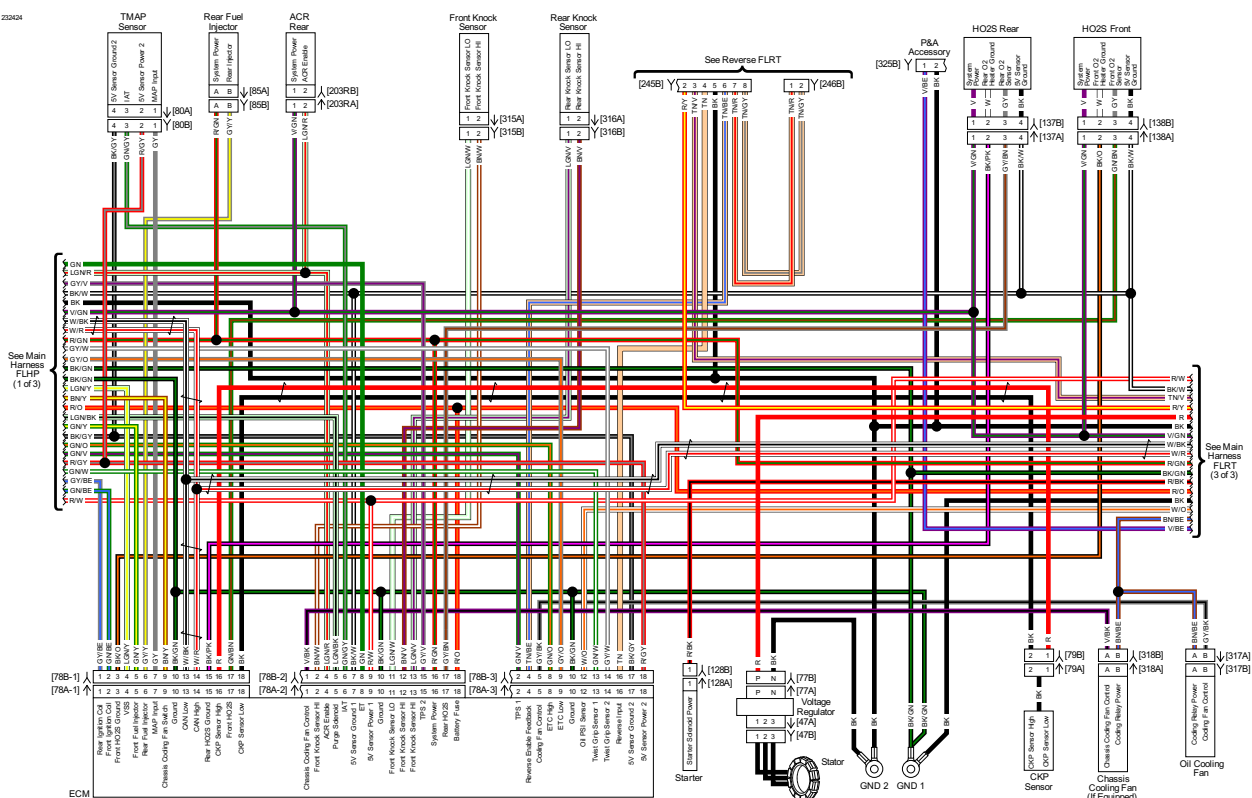
Main Harness FLRT (2 of 3): 2018 Trike Model
