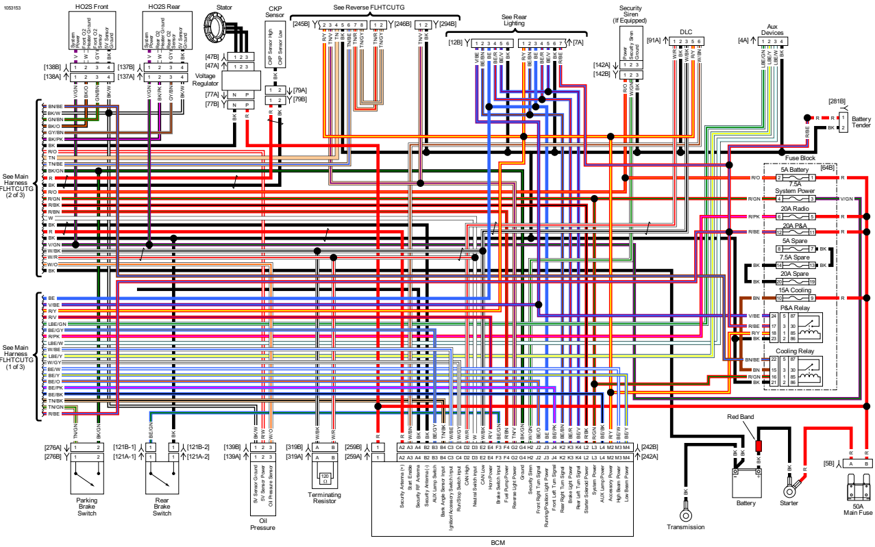
Main Harness FLHTCUTG (3 of 3): 2018 Trike Model
