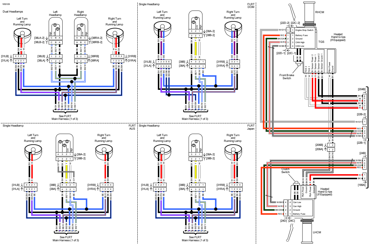
Front Lighting and Hand Controls: 2018 Trike Models (FLRT)
