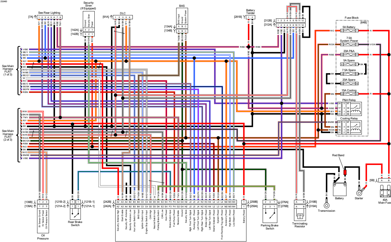
Main Harness FLRT (3 of 3): 2018 Trike Model
