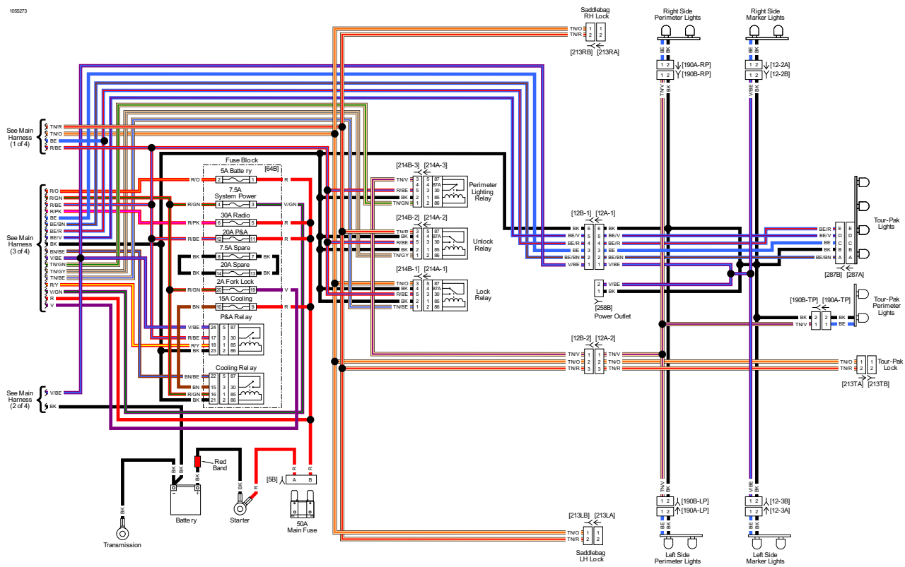
Main Harness (4 of 4): 2018 FLHTKSE
