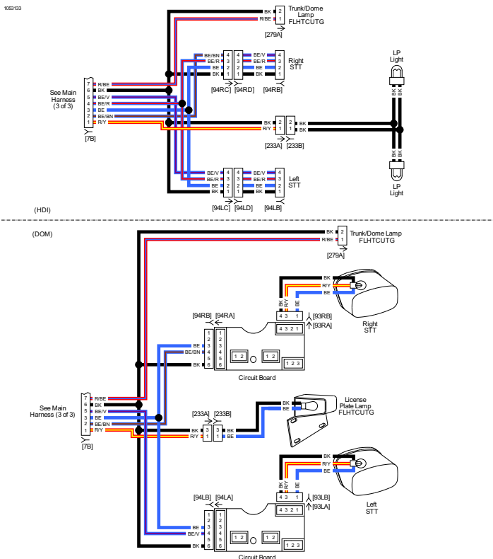
Rear Lighting: 2018 Trike Models (FLHTCUTG)
