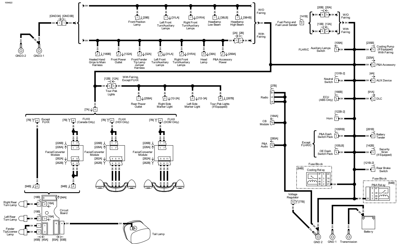
Ground Circuit FLH: 2018 Touring
