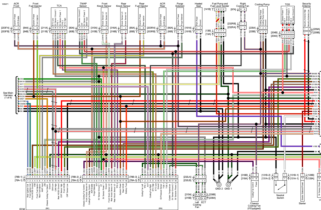
Main Harness (2 of 4): 2018 FLHTKSE
