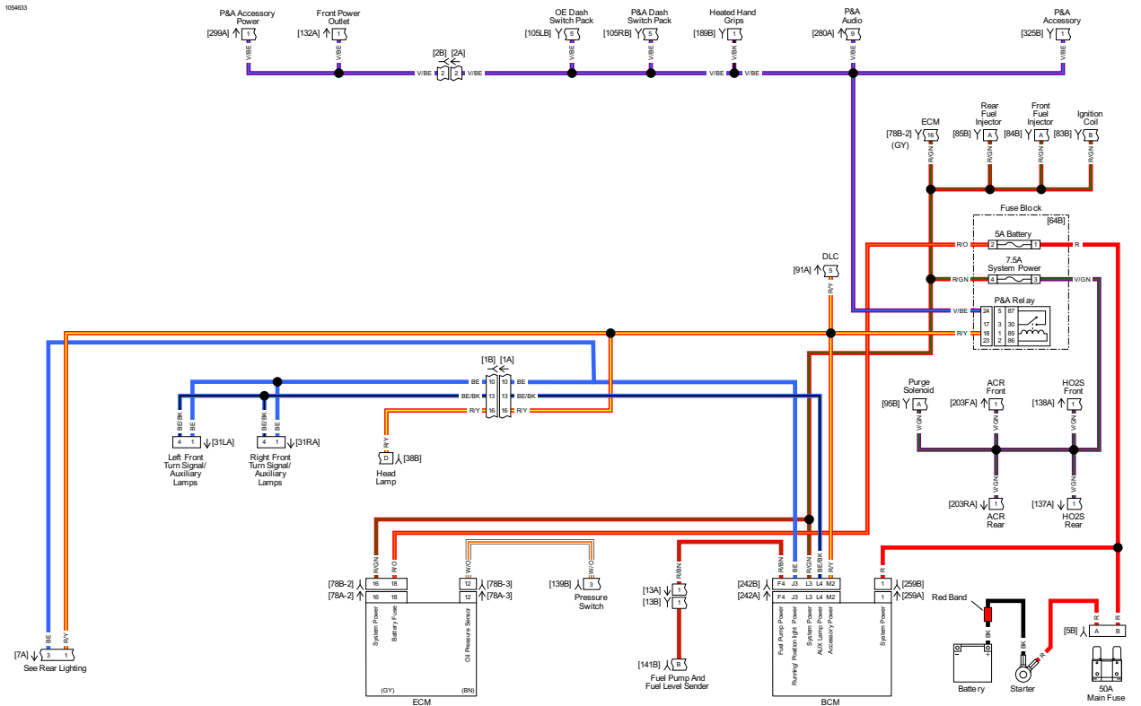
Ignition and ACC FLT: 2018 Touring
