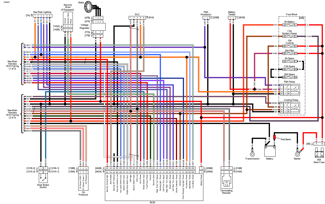
Main Harness (3 of 3): 2018 Touring (without Fairing)
