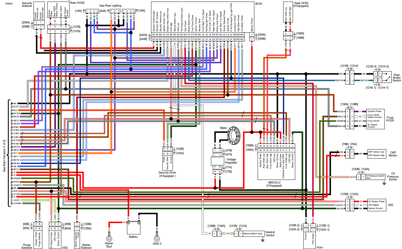
Main Harness 2 of 2: 2018 Sportster
