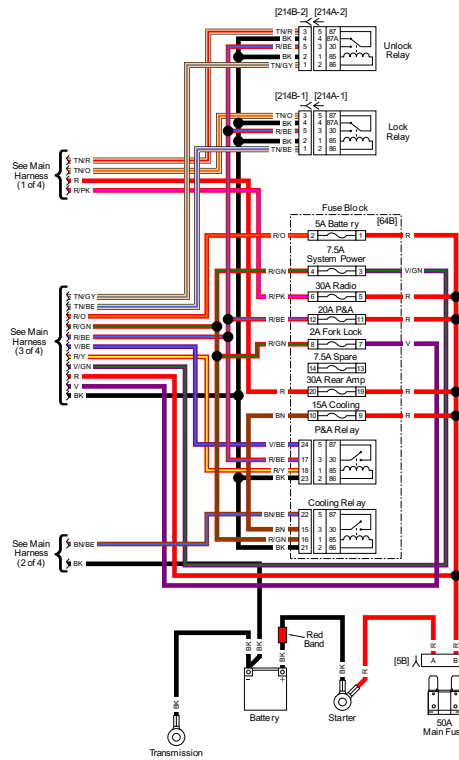
Main Harness (4 of 4): 2018 FLTRXSE
