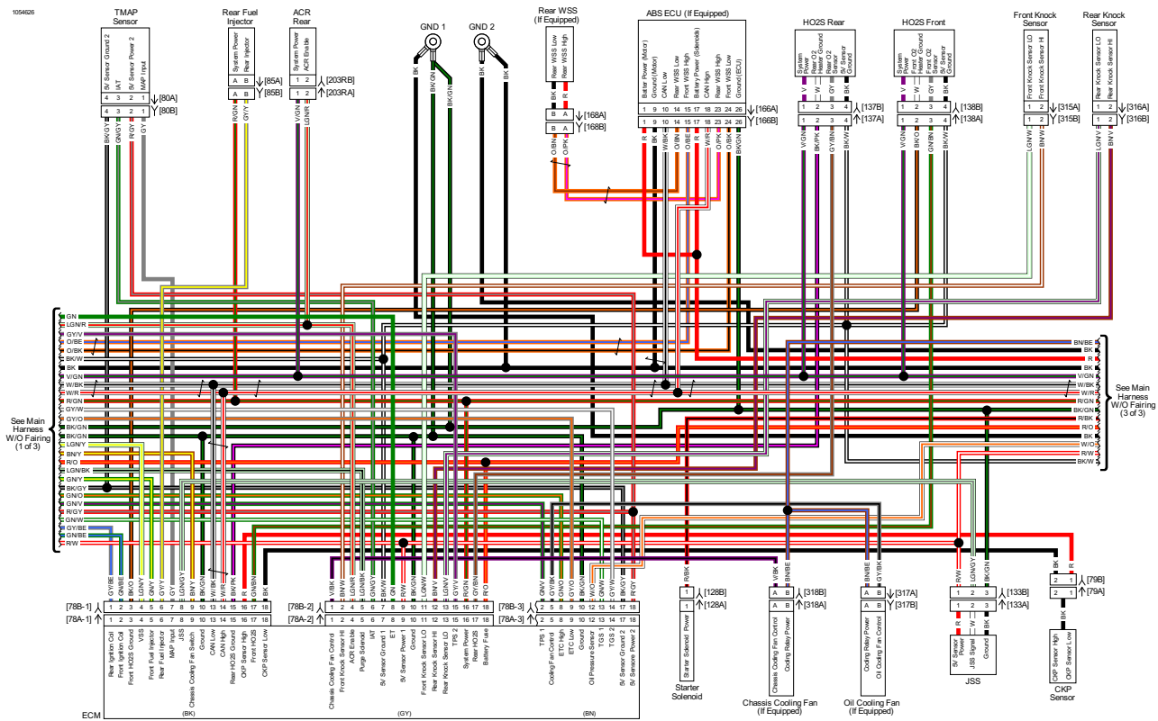
Main Harness (2 of 3): 2018 Touring (without Fairing)
