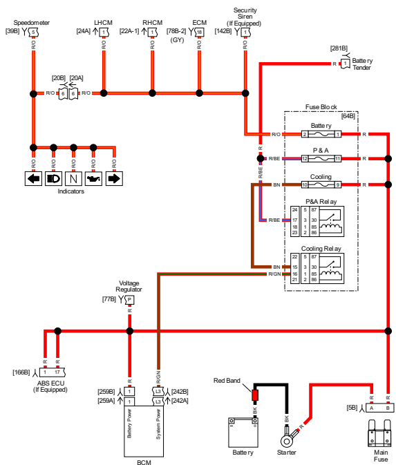
Battery Power Distribution without Fairing
