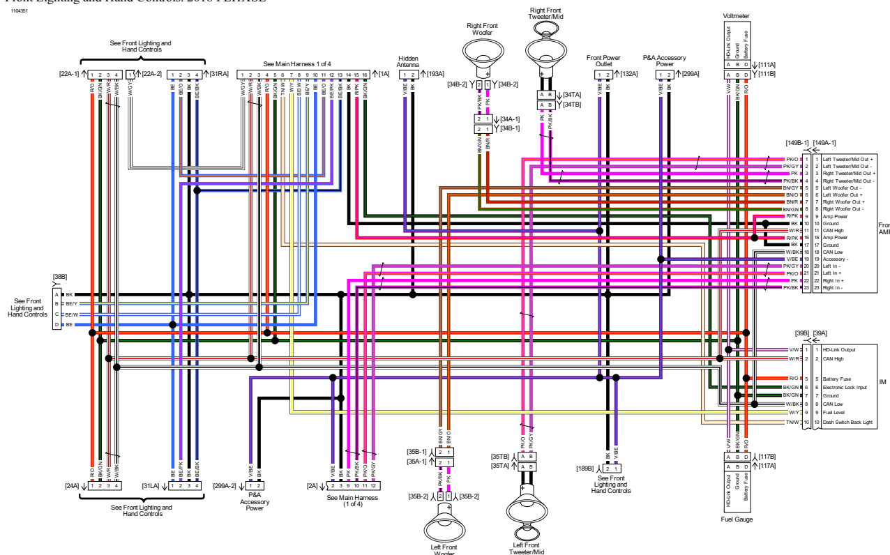
Fairing Harness: 2018 FLHXSE
