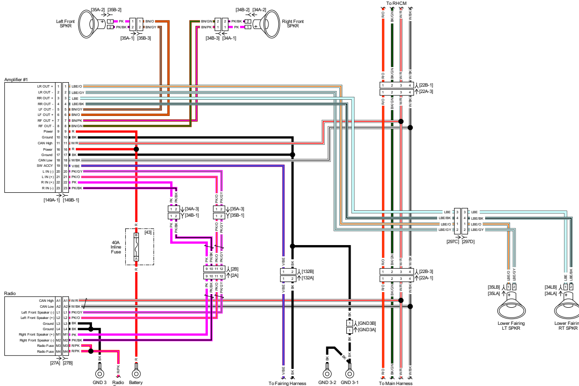
P&amp;A Radio with 2 Amps (1 of 2): 2018 Touring
