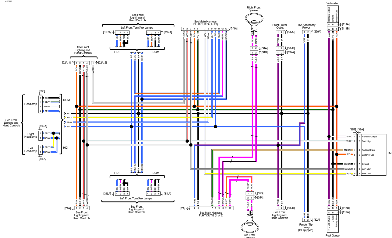
Fairing Harness FLHTCUTG: 2018 Trike Model
