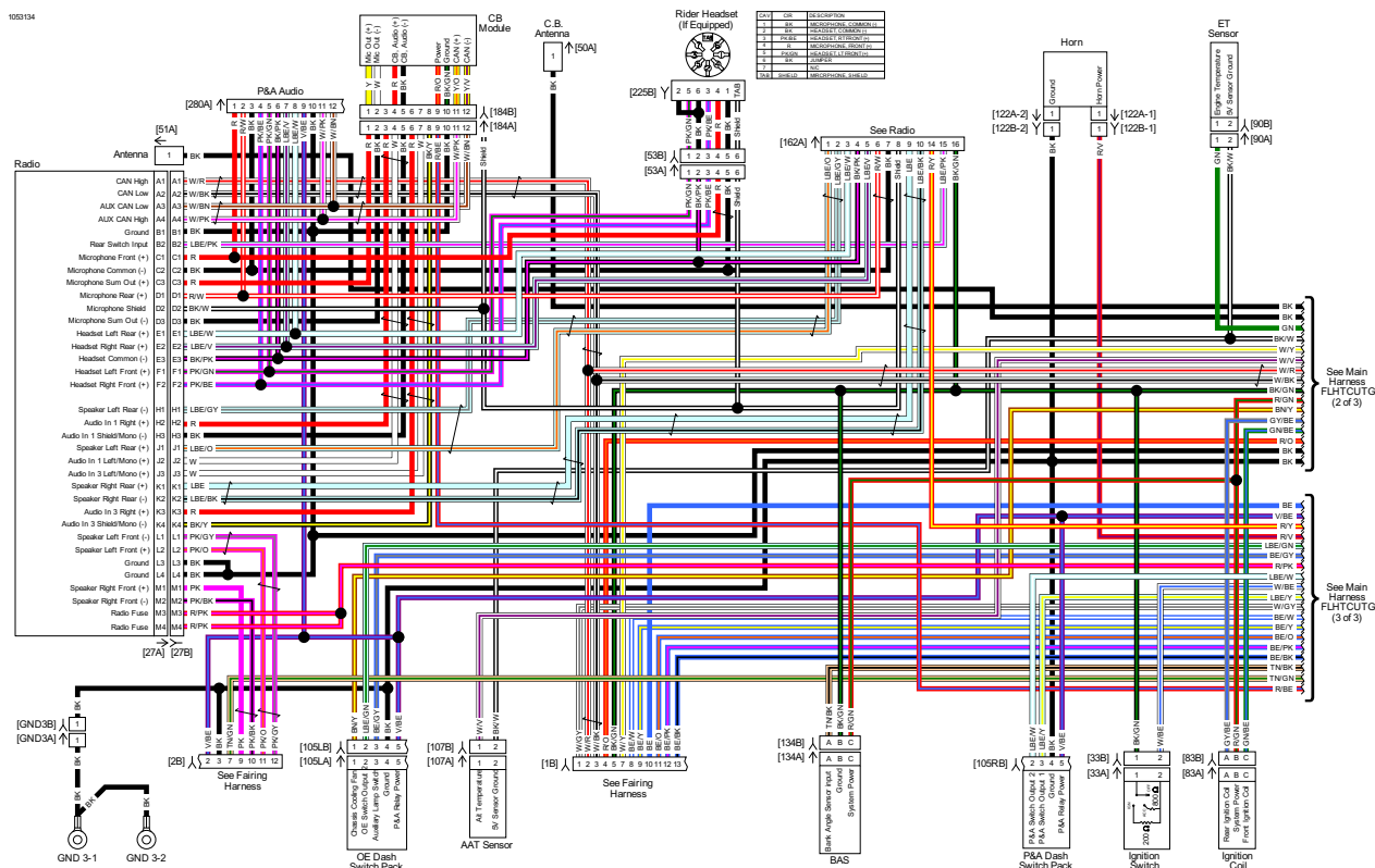
Main Harness FLHTCUTG (1 of 3): 2018 Trike Model
