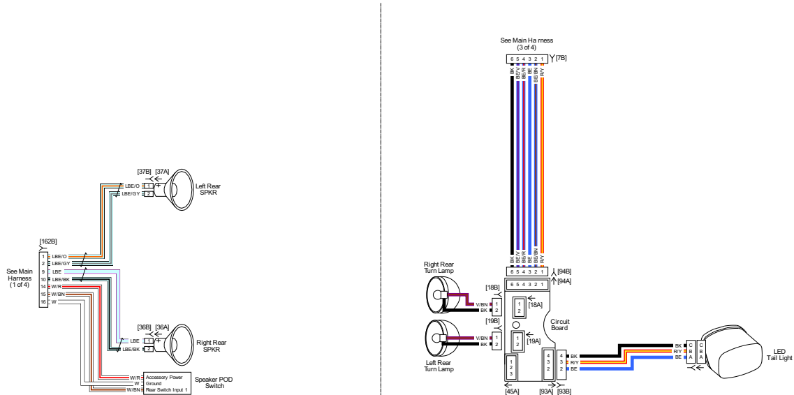
Main Harness (4 of 4): 2018 FLHTKSE
