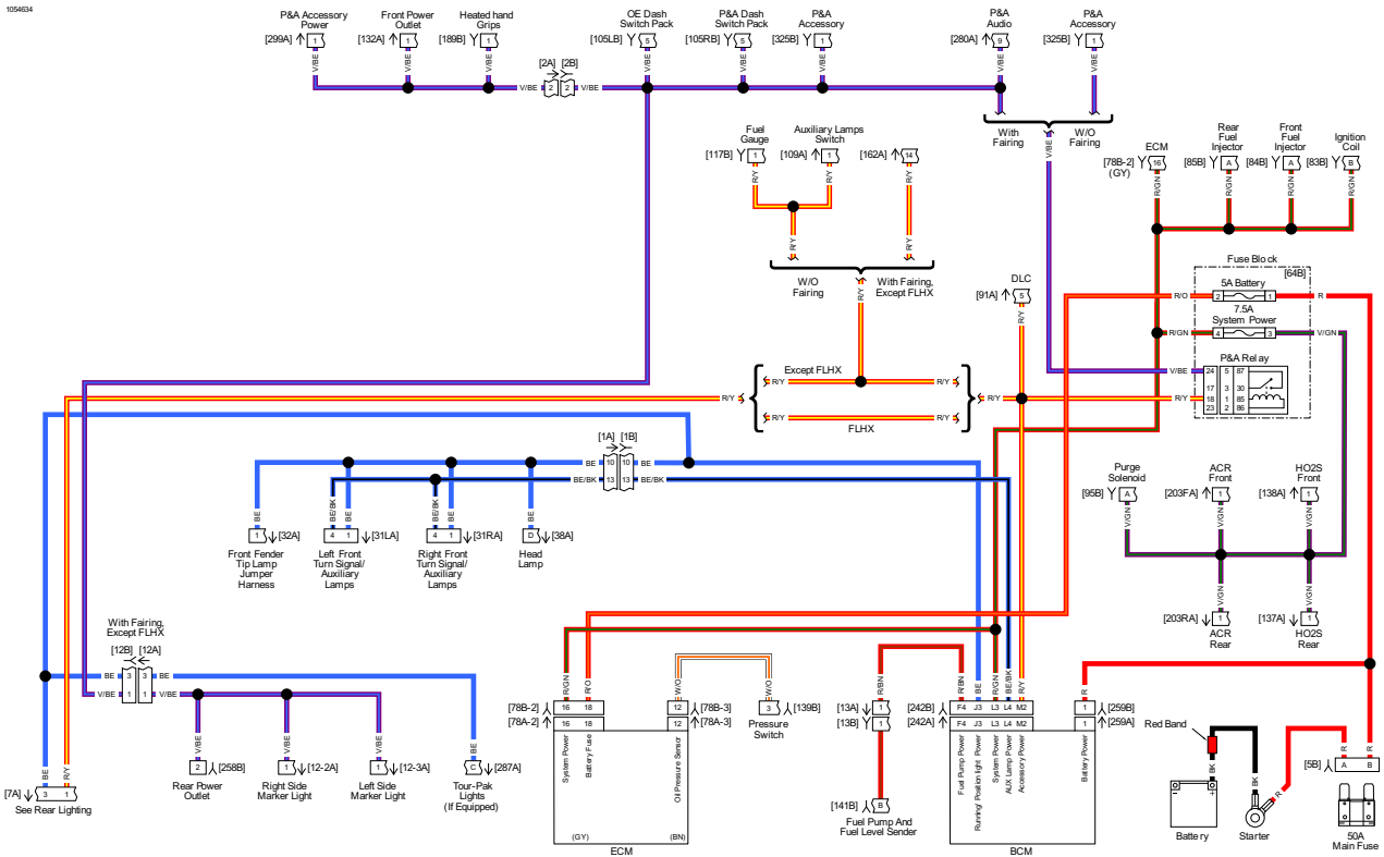
Ignition and ACC FLH: 2018 Touring
