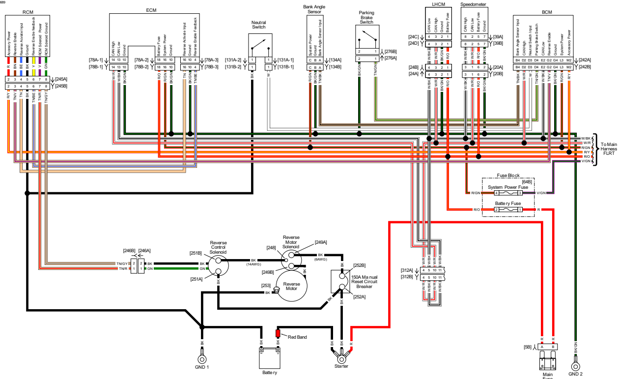
Reverse FLRT: 2018 Trike Model
