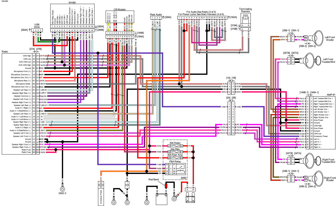
Radio (1 of 2): 2018 FLTRXSE
