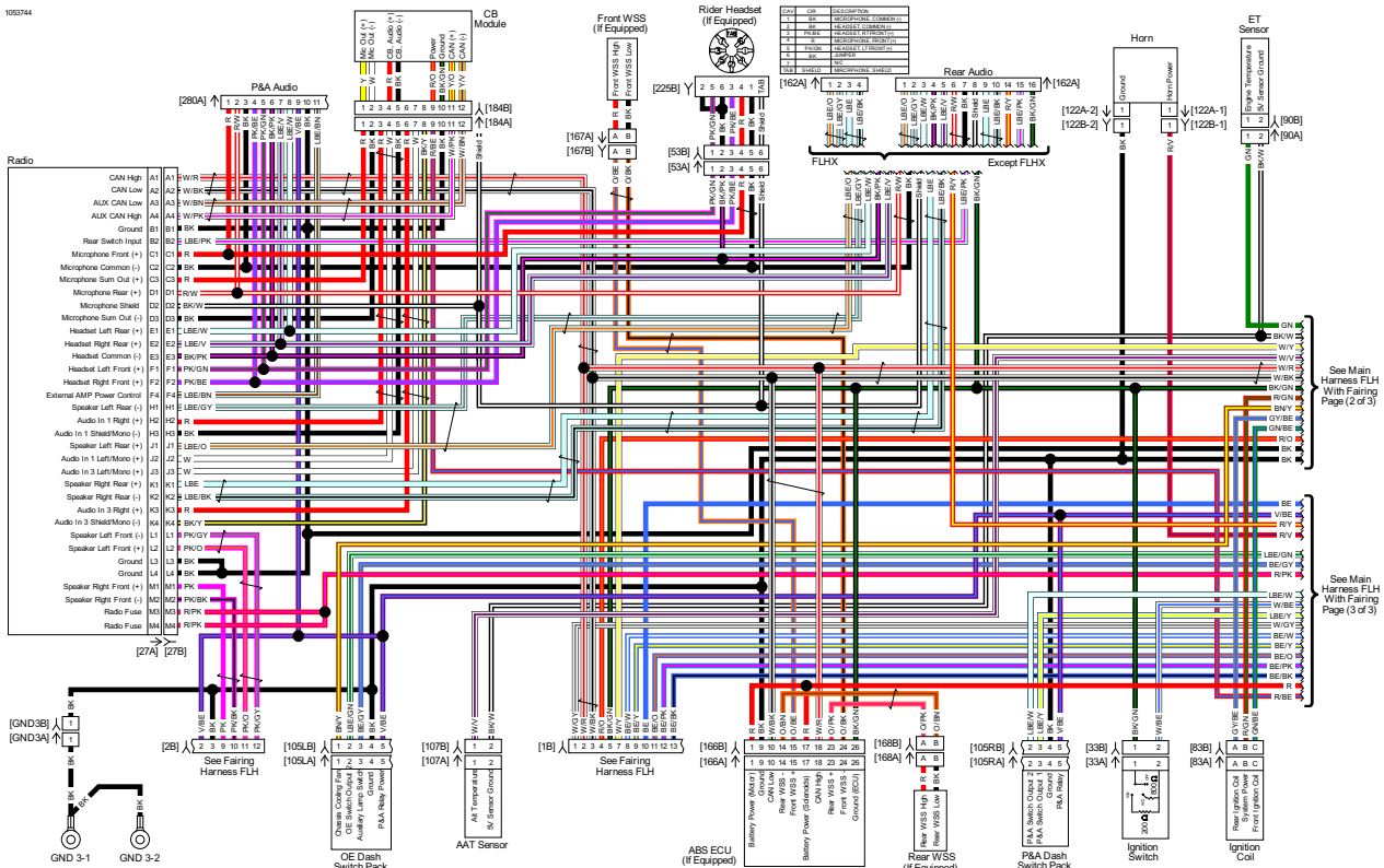
Main Harness FLH (1 of 3): 2018 Touring (with Fairing)
