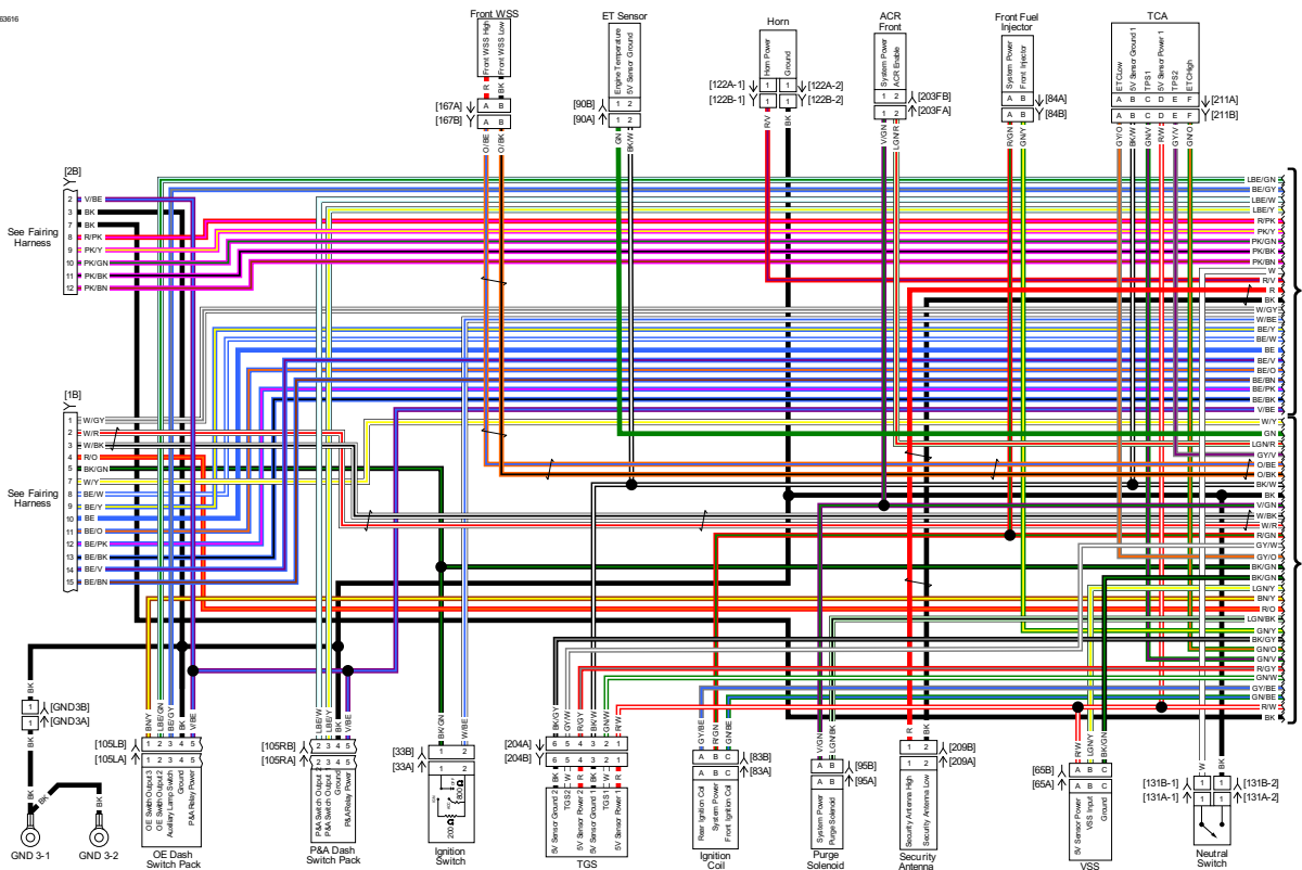
Main Harness (1 of 3): 2018 FLHTP
