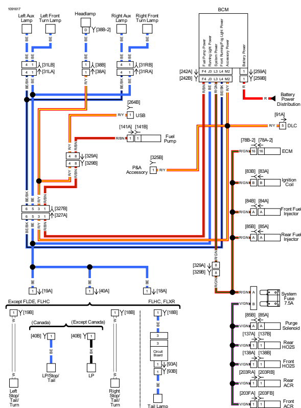
Ignition and Accessory Power Distribution
