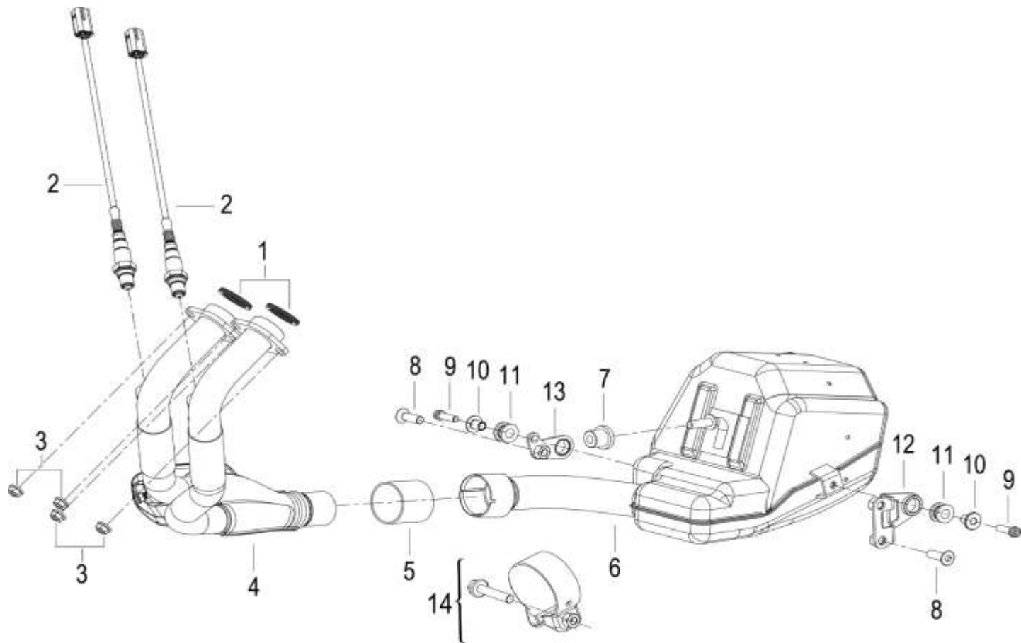
FIG 5 ESCAPE
