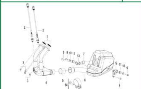
FIGURA N°5: ESCAPE
