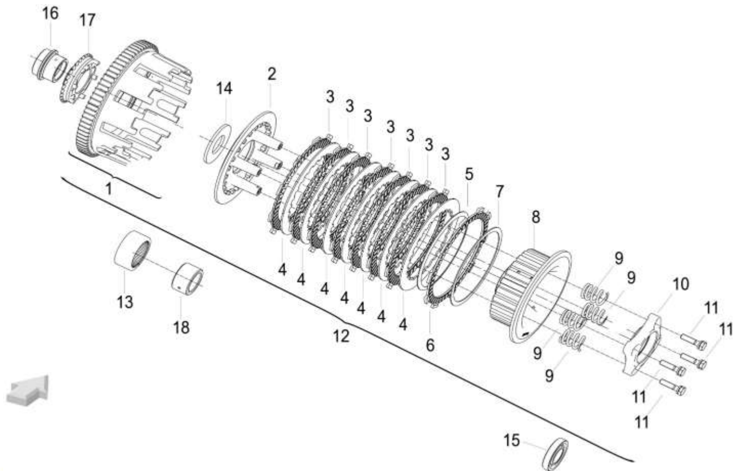
FIG 32 CLUTCH
