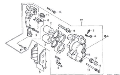
F-9 Front Brake Caliper
