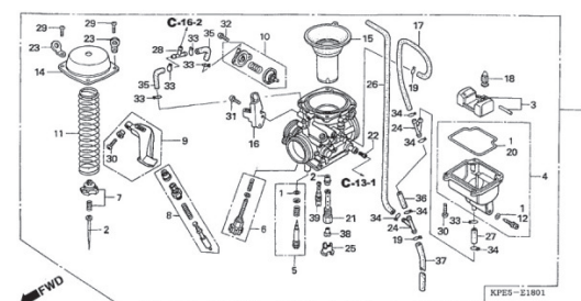
E-18 Carburetor
