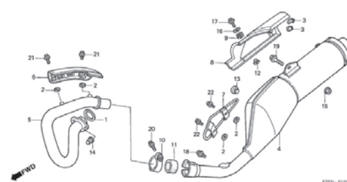
F-18 Exhaust Muffler
