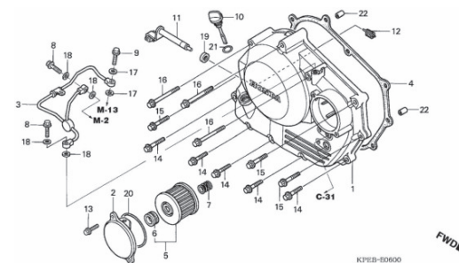
E-9 Left Crankcase Cover
