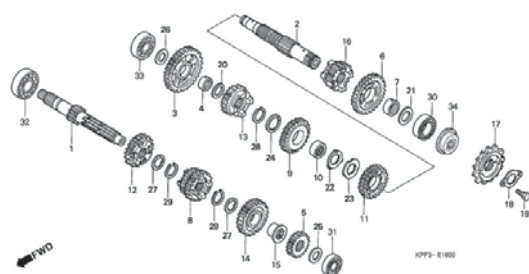
E-16 Transmission
