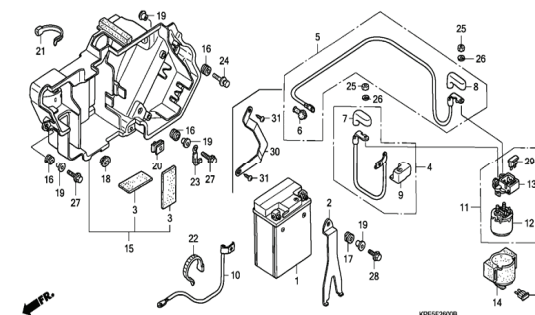
F-27 Battery
