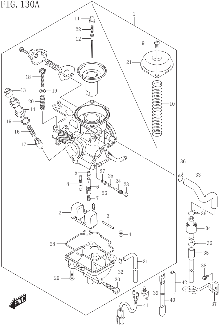
GS125QSL7_P09_130A CARBURETOR
