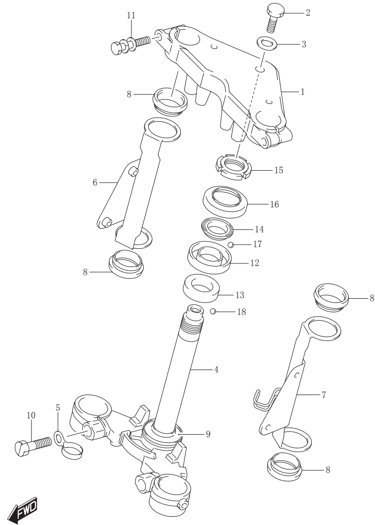
GS125QSL7_P09_524A STEERING STEM
