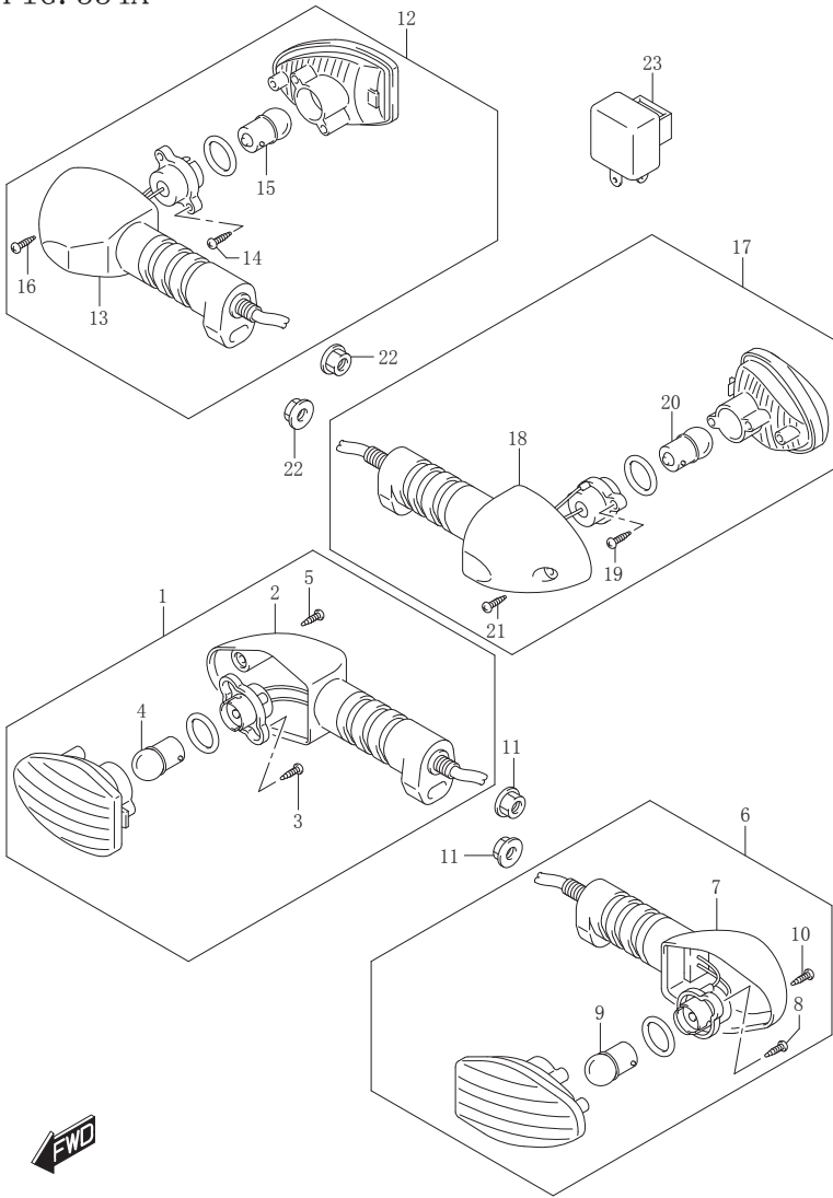
GS125QSL7_P09_334A TURN SIGNAL LAMP
