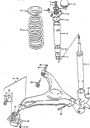
05-10 SUSPENSION TRASERA
