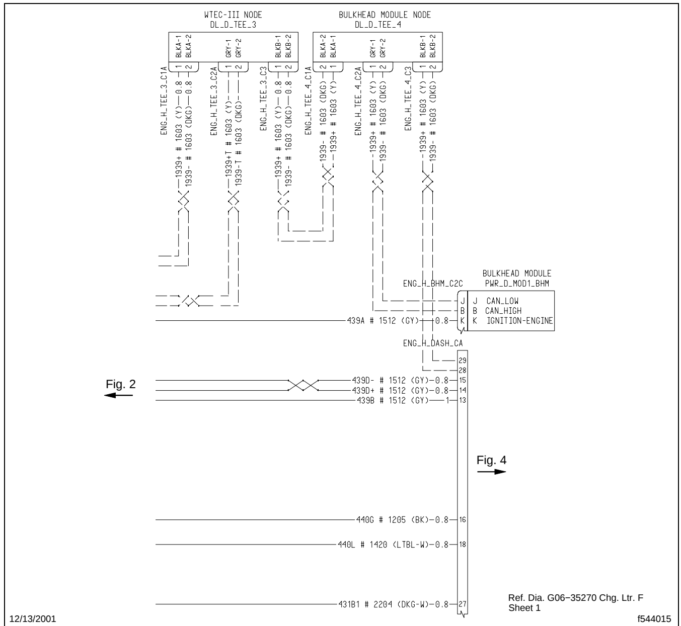
Fig. 3, MBE900 Engine Compartment Wiring Schematic, Automatic Transmission (detailed view, BHM)
