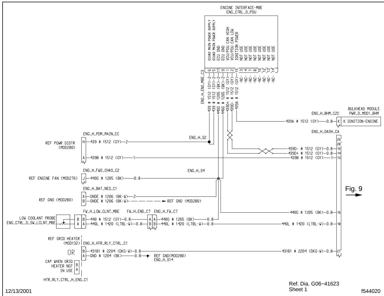
Fig. 8, MBE900 Engine Compartment Wiring Schematic, Manual Transmission
