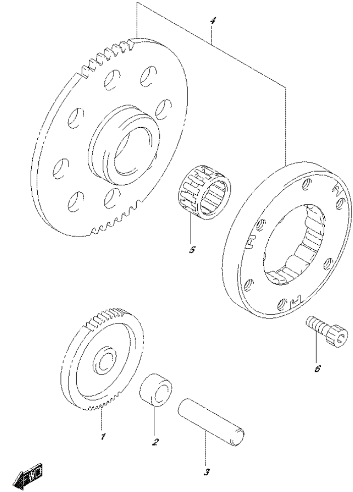
GSX150FL8_P10_122A STARTER CLUTCH
