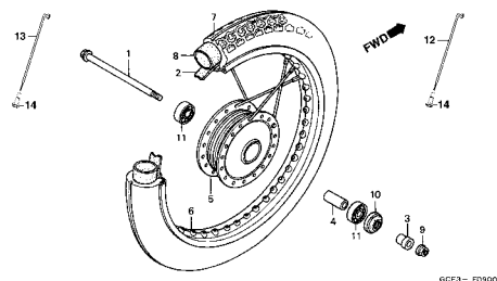
C-11 Roda Traseira / Rear Wheel / Rueda Trasera
