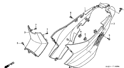
C-14 Carenagem Lateral / Body Cover / Cubretablero
