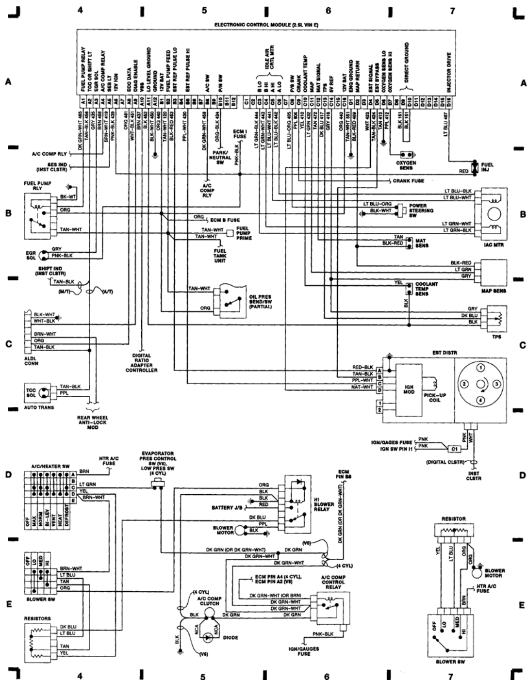
Fig. 2: Computer Engine Control (2.5L)
