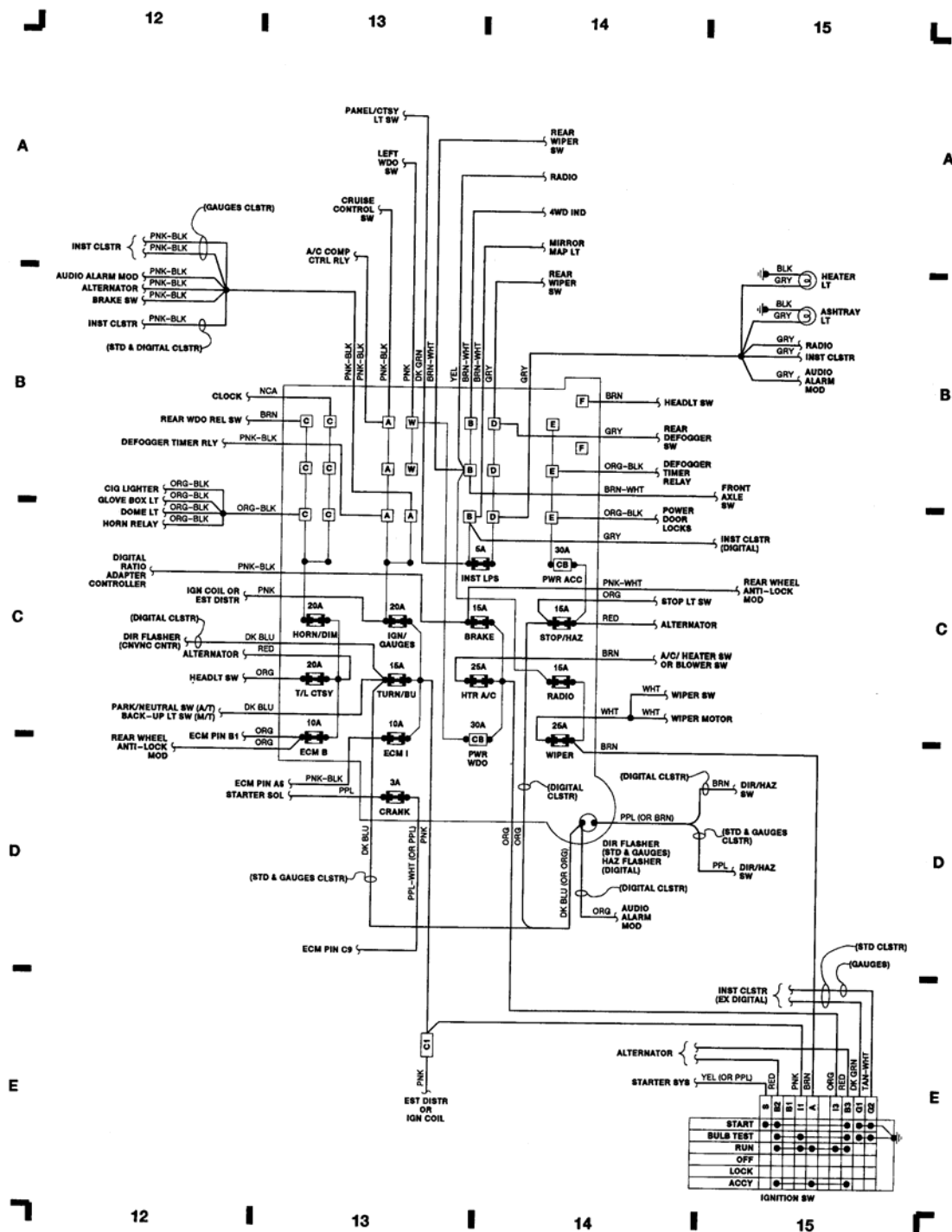
Fig. 4: Fuse Block
