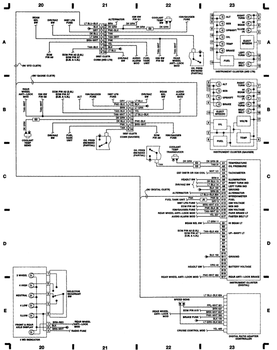
Fig. 6: Instrument Panel
