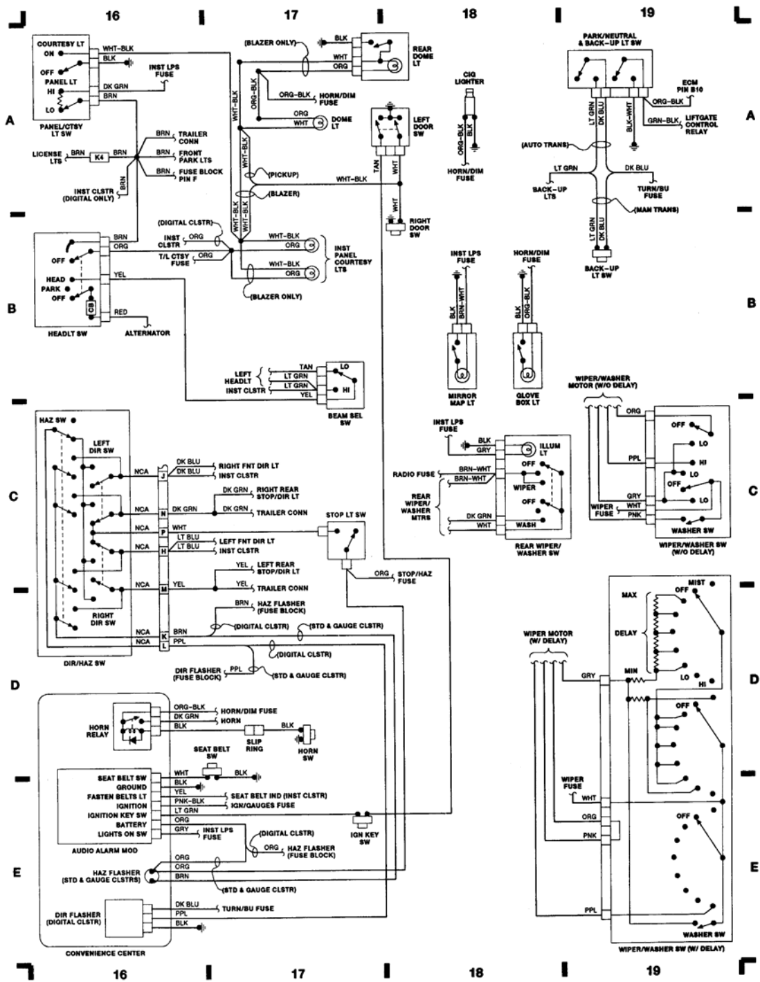
Fig. 5: Wiper/Washer System, Instrument Panel Switches
