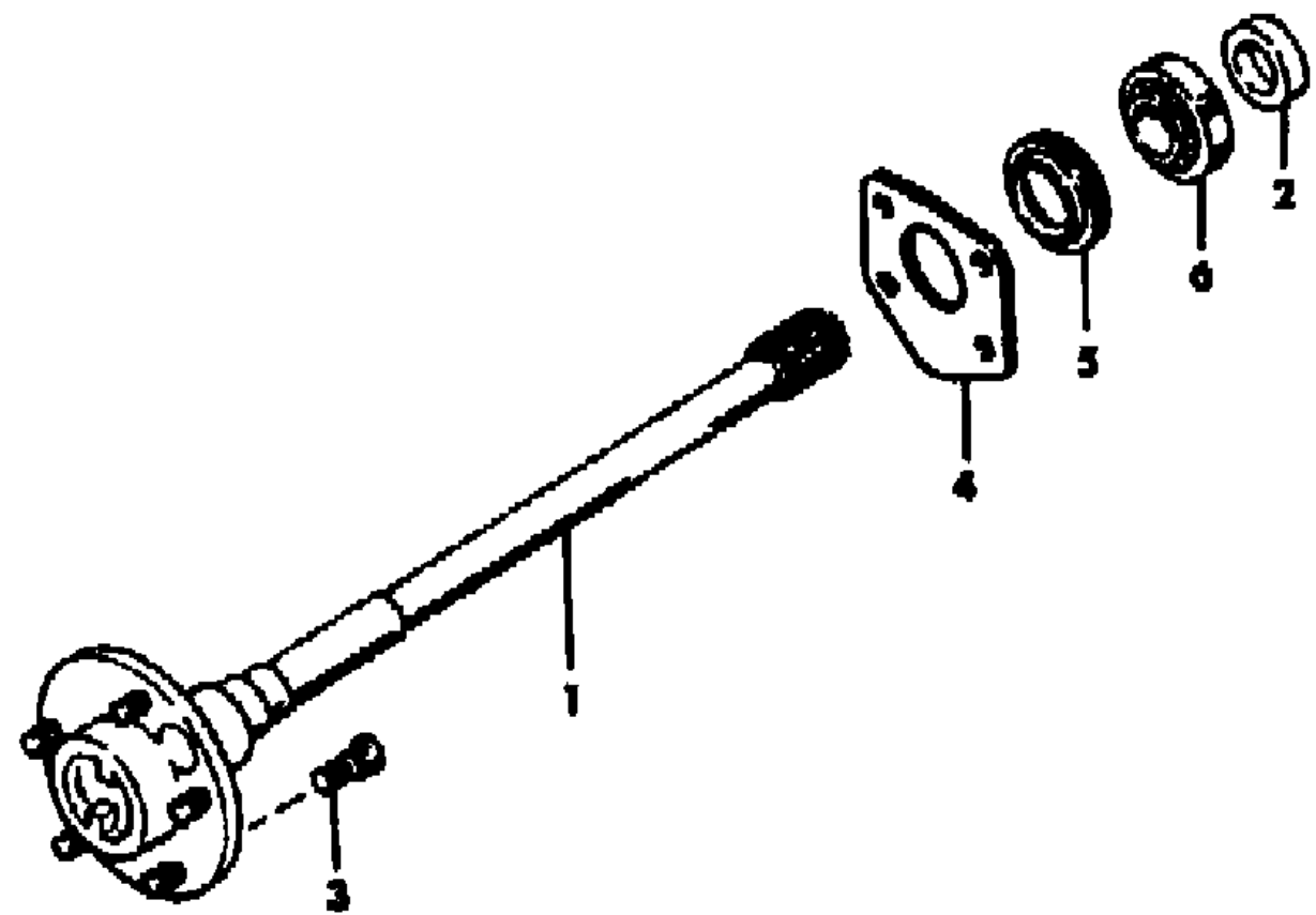
DANA MODEL 44 AXLE (REF.)
