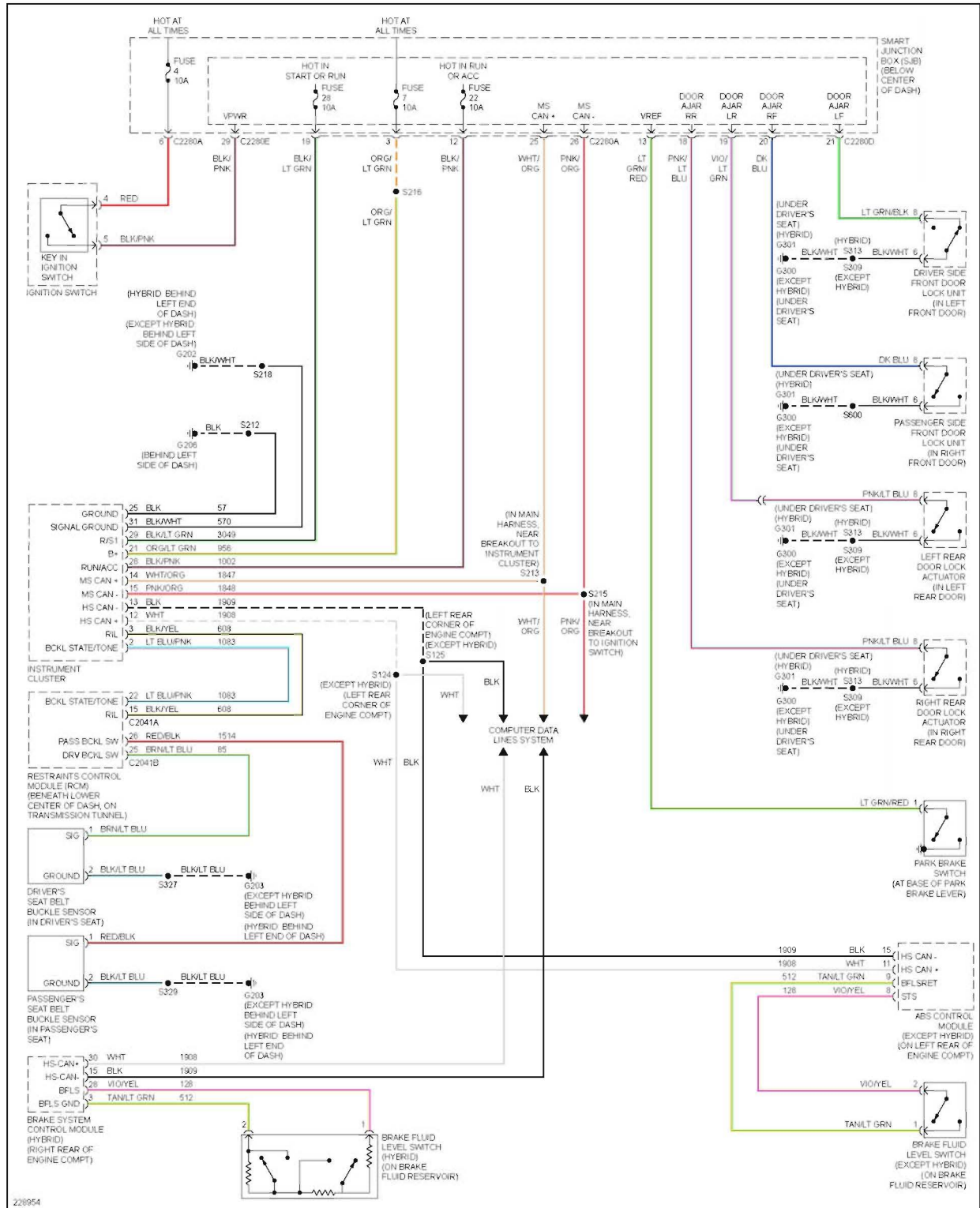
Fig. 101: Warning Systems Circuit
