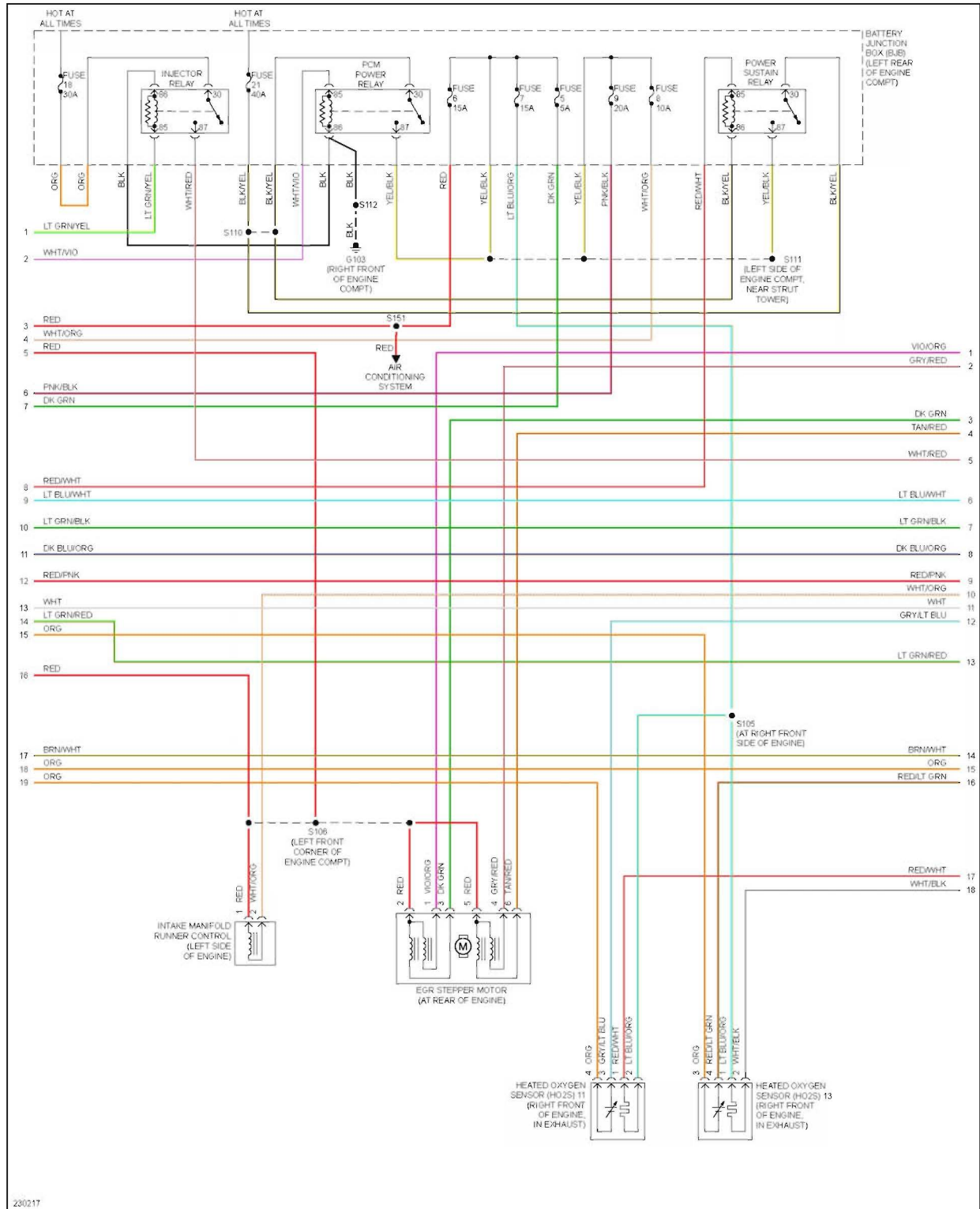
Fig. 40: 2.3L, Engine Performance Circuit, Hybrid (4 of 6)
