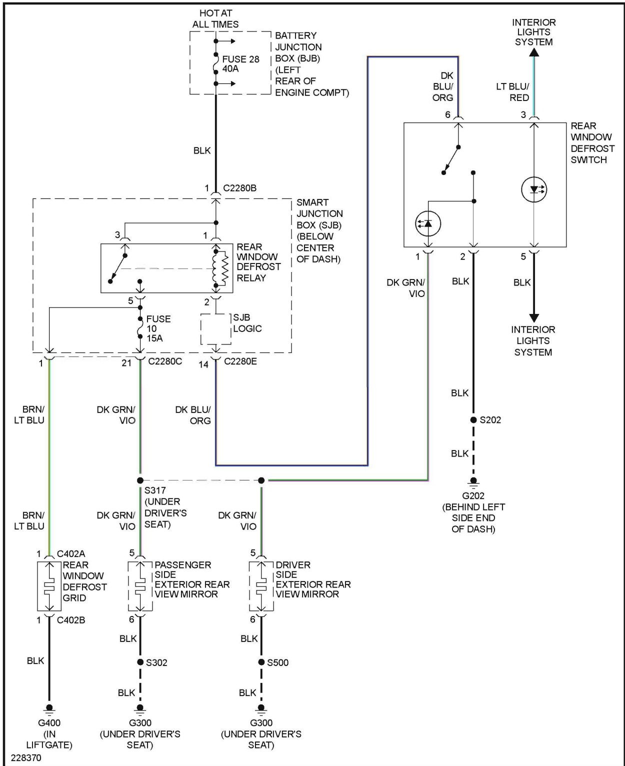
Fig. 30: Defoggers Circuit, Hybrid
