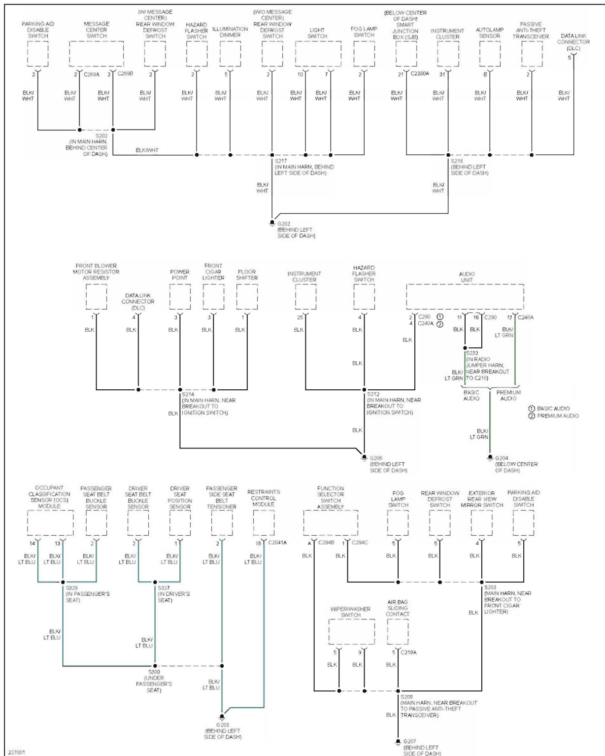
Fig. 56: Ground Distribution Circuit, Except Hybrid (2 of 3)
