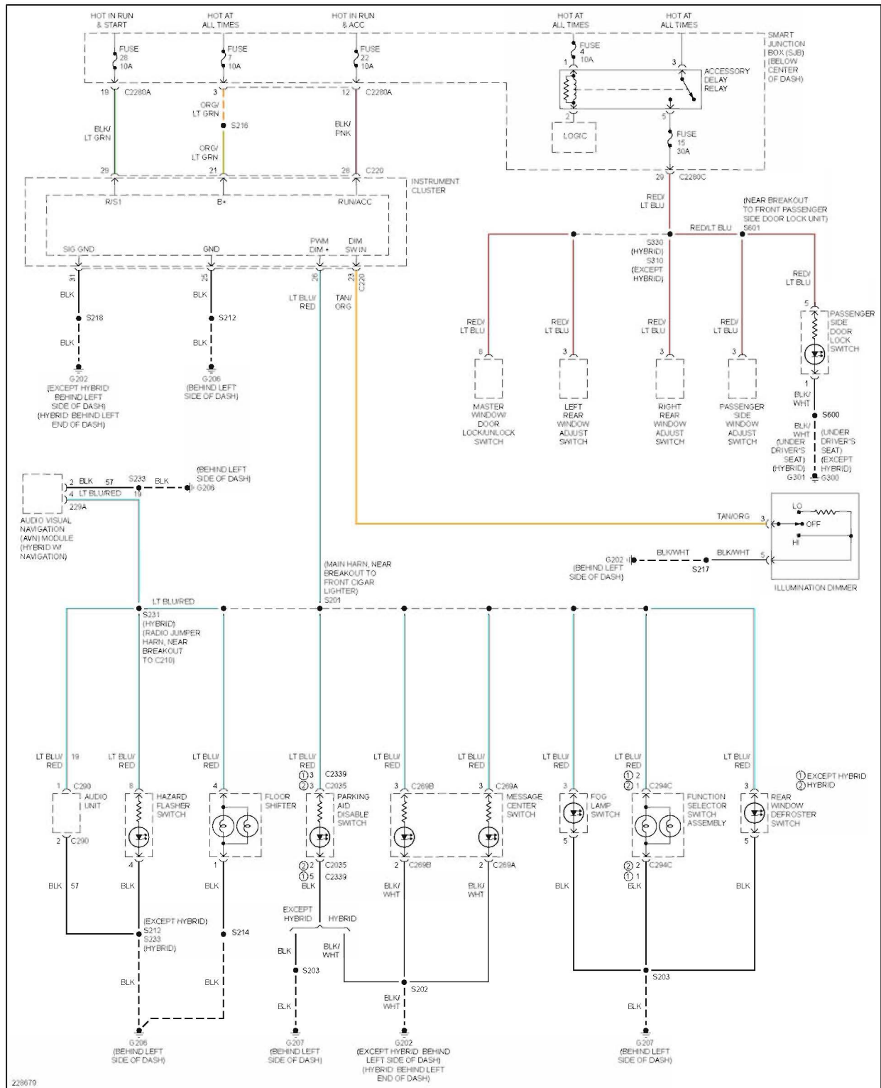
Fig. 68: Instrument Illumination Circuit
