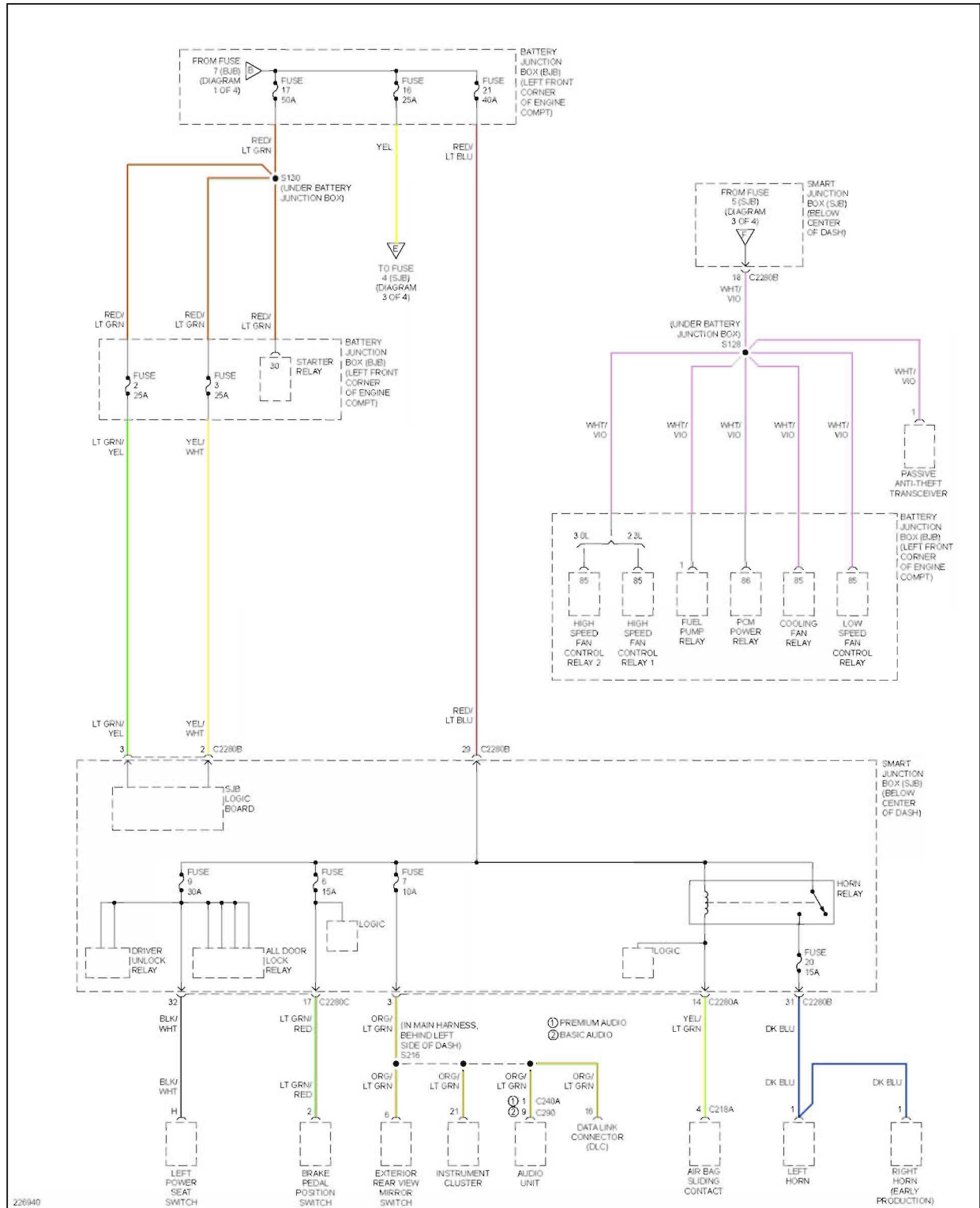
Fig. 73: Power Distribution Circuit, Except Hybrid (2 of 4)
