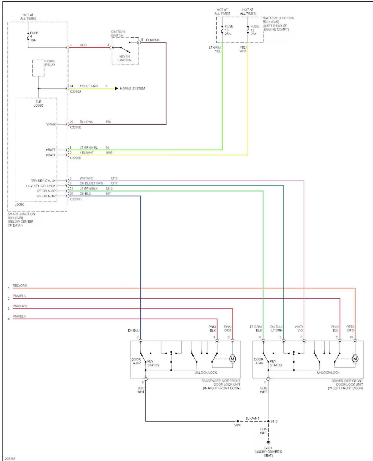
Fig. 13: Forced Entry Circuit, Hybrid (2 of 2)
