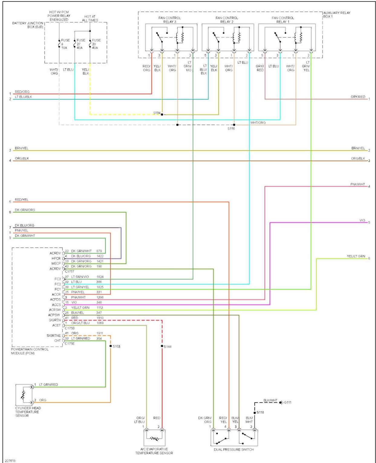
Fig. 4: 2.3L, Manual A/C Circuit, Hybrid (2 of 3)
