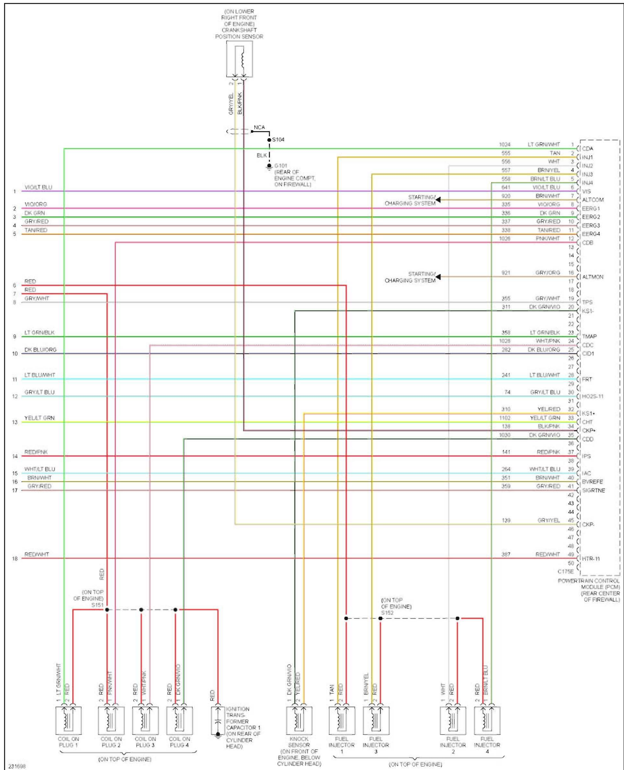
Fig. 36: 2.3L, Engine Performance Circuit, Except Hybrid (5 of 5)
