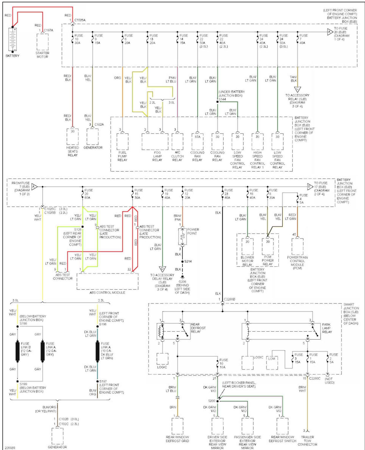
Fig. 72: Power Distribution Circuit, Except Hybrid (1 of 4)
