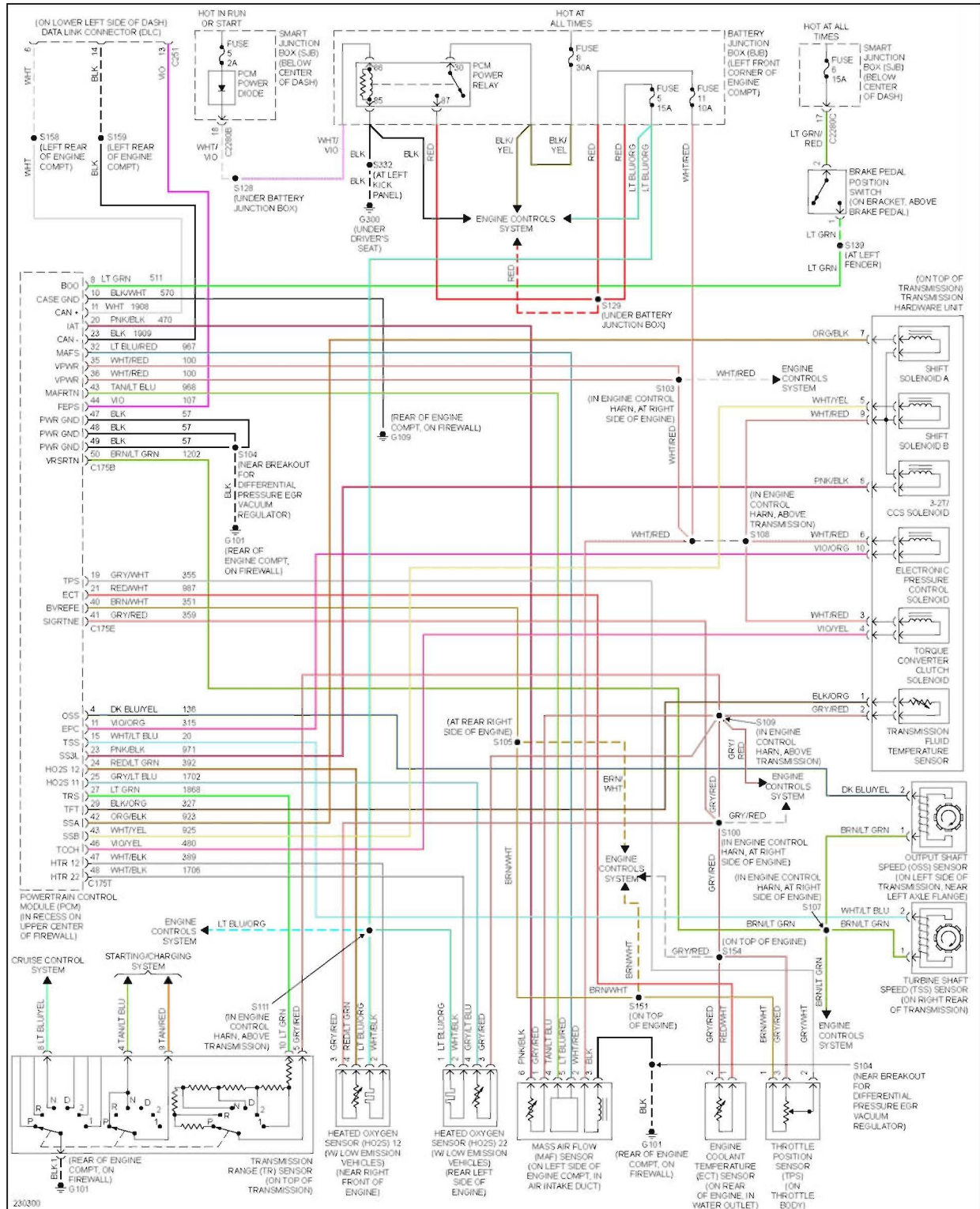
Fig. 100: 3.0L, A/T Circuit, Except Hybrid
