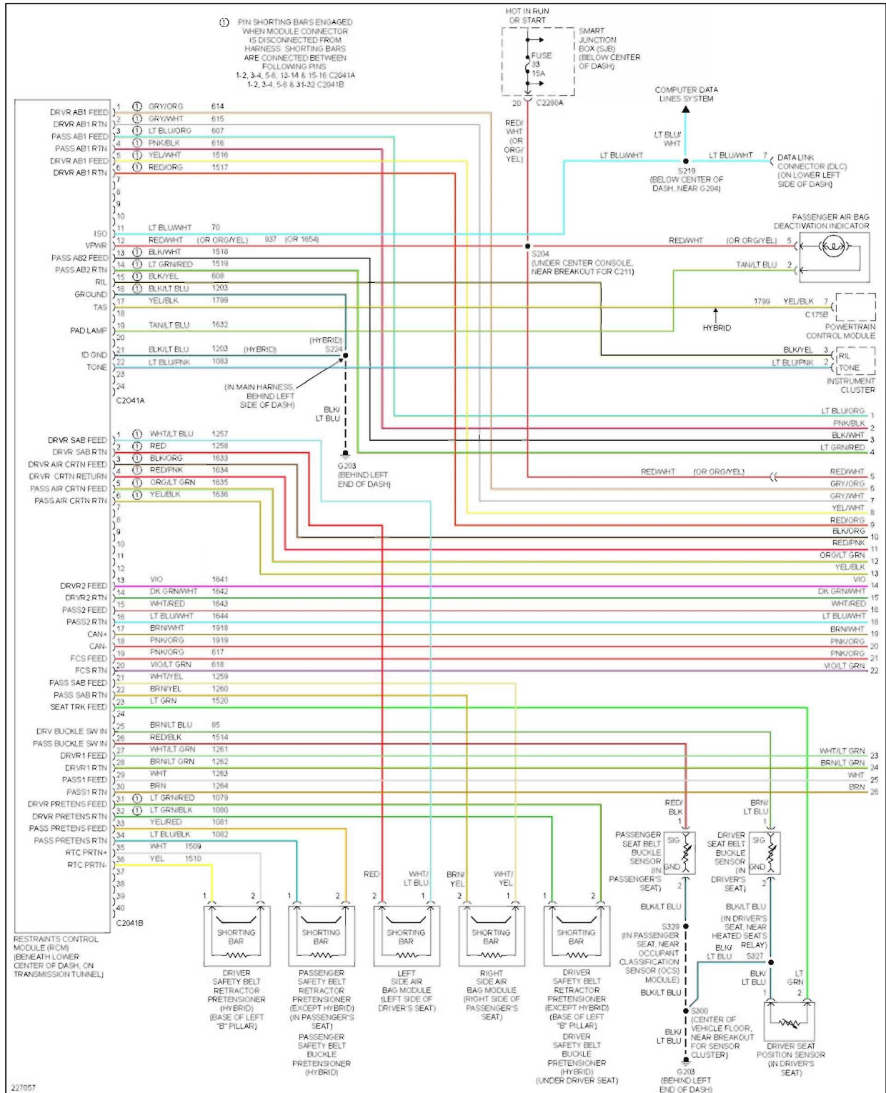
Fig. 95: Supplemental Restraints Circuit (1 of 2)
