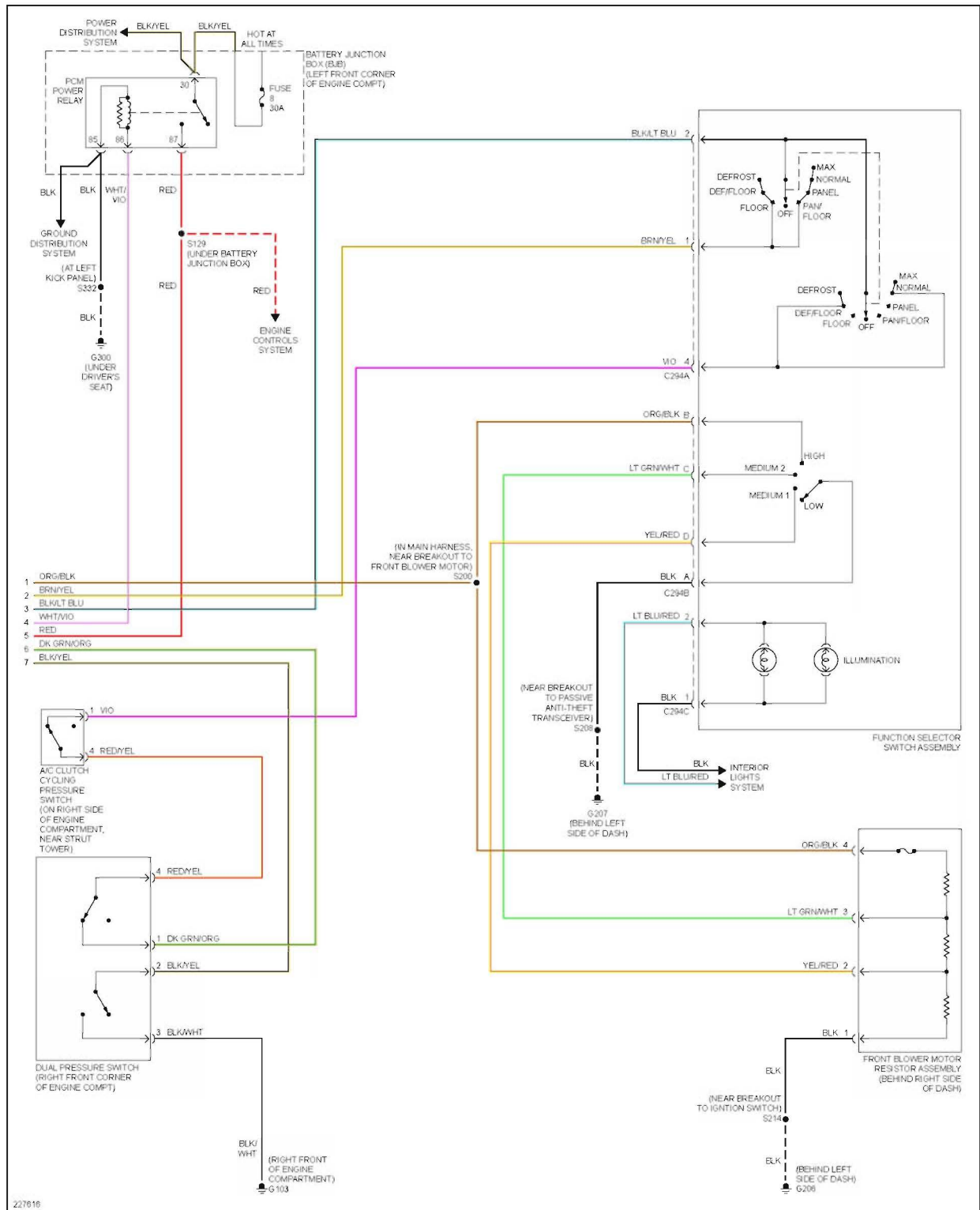
Fig. 7: 3.0L, Manual A/C Circuit, Except Hybrid (2 of 2)
