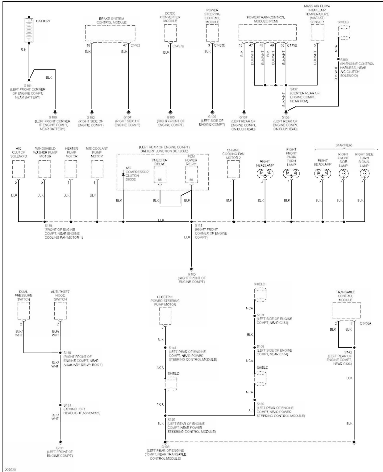
Fig. 58: Ground Distribution Circuit, Hybrid (1 of 4)
