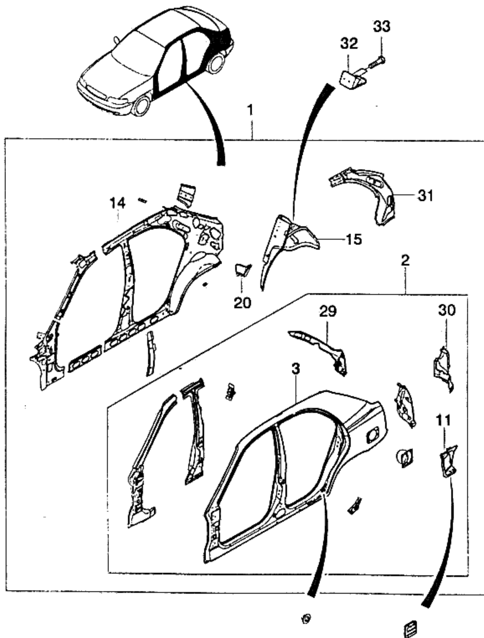
Ref. 6410 GROUP(SIDE BODY PANEL)
