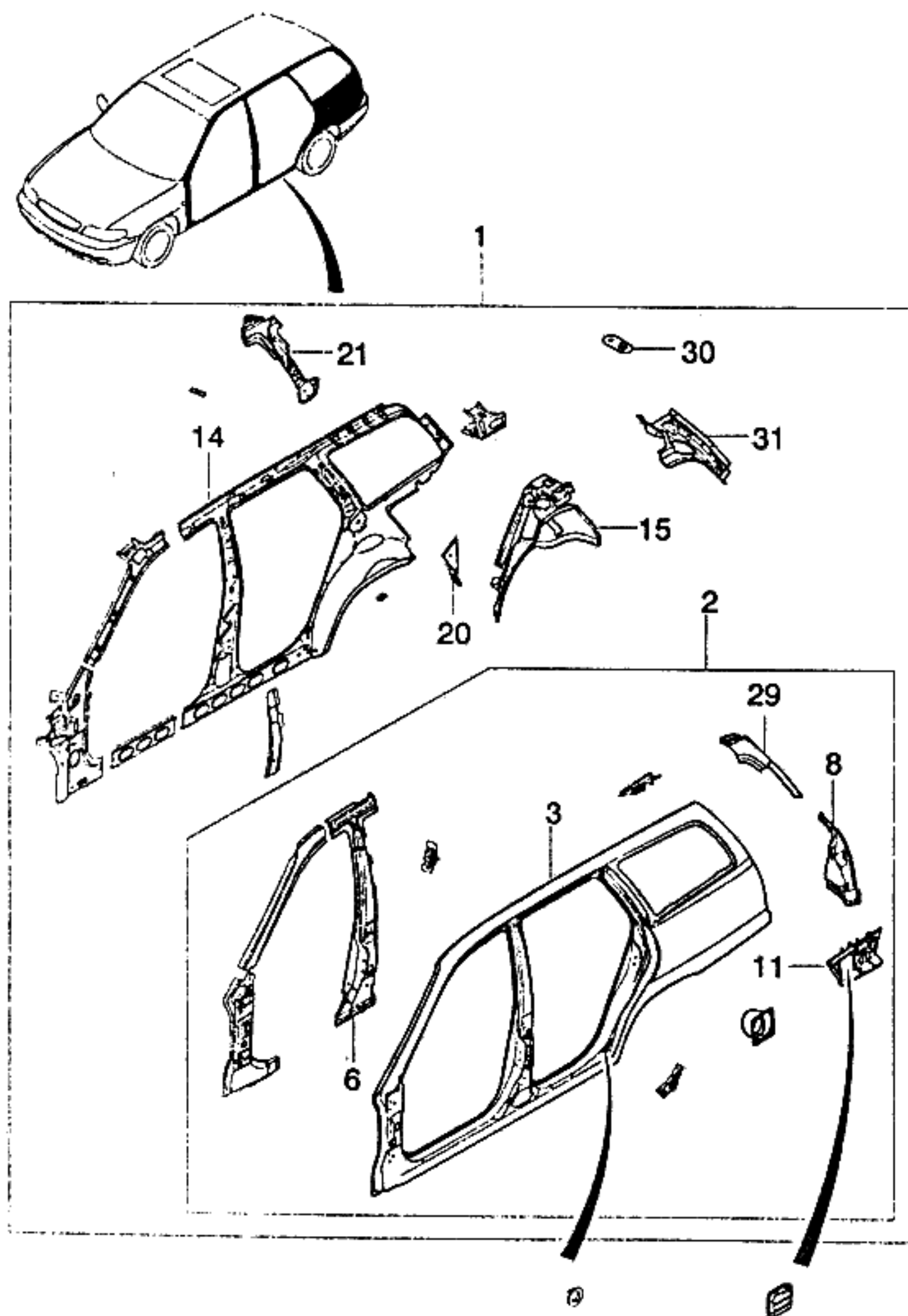
Ref. 6410 GROUP(SIDE BODY PANEL)
