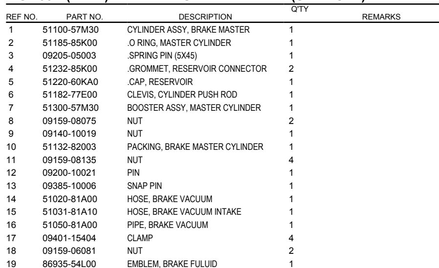
FIG.133A (2-I-14) BRAKE MASTER CYLINDER (SEE NOTE)
