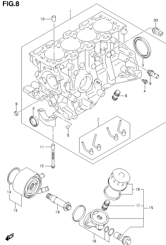
SN413V-5 E22_008 CYLINDER (2)
