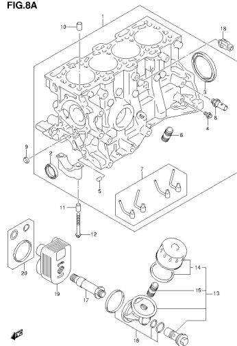
SN413V-5 E22_008A CYLINDER (3)
