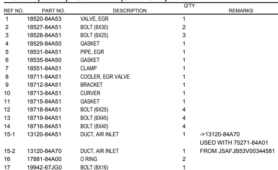
FIG.49A (1-G-11) EGR VALVE (SEE NOTE)
