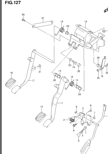
SN413V5 E22_127 PEDAL/PEDAL BRACKET (1)
