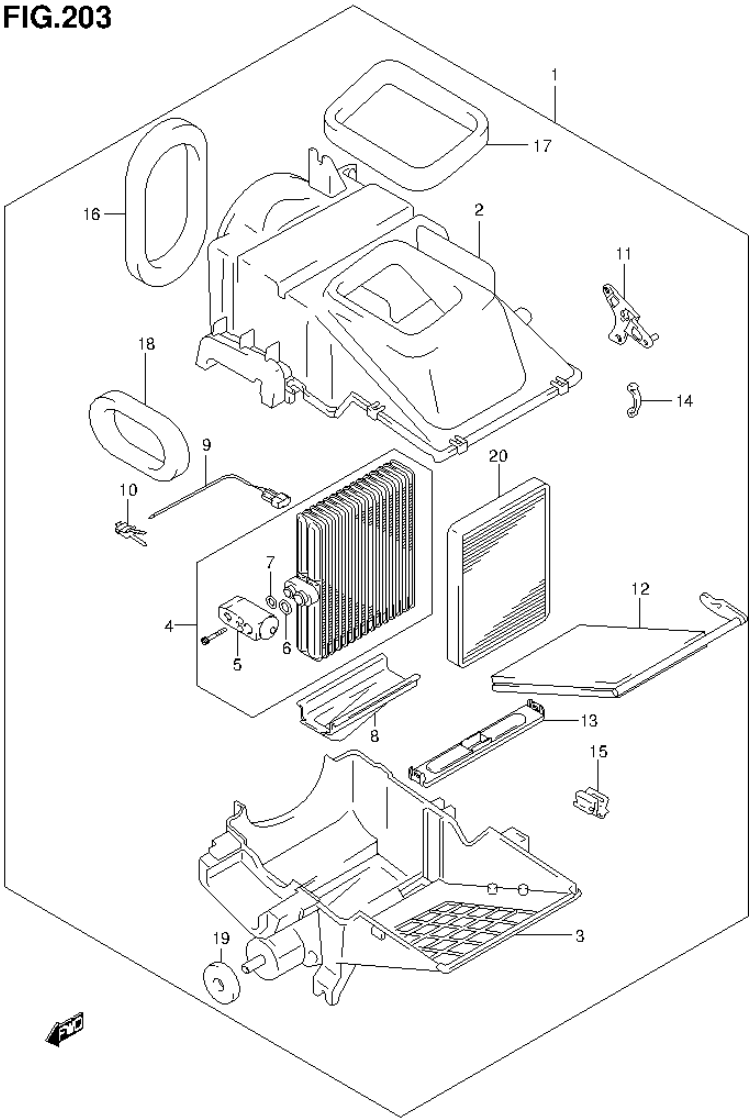
FIG.203 (4-J-10) COOLING UNIT (SN413V:RHD)
