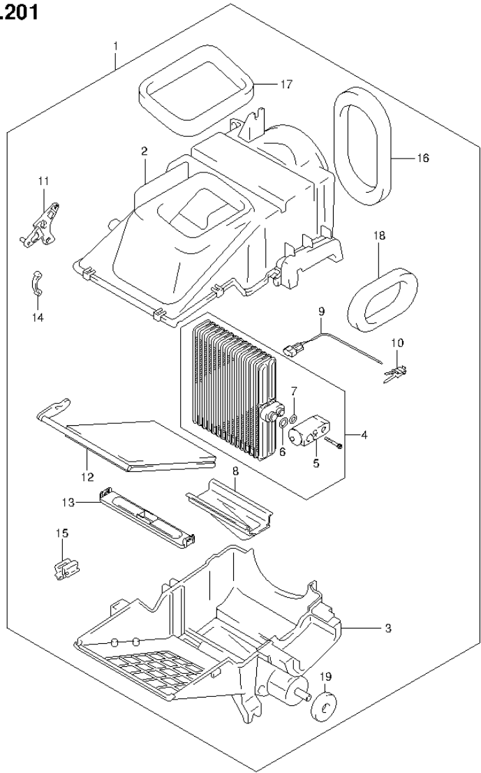
FIG.201 (4-J-8) COOLING UNIT (SN413V:LHD)
