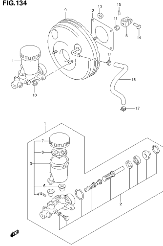
SN413V-5 E22_134 BRAKE MASTER CYLINDER (4)
