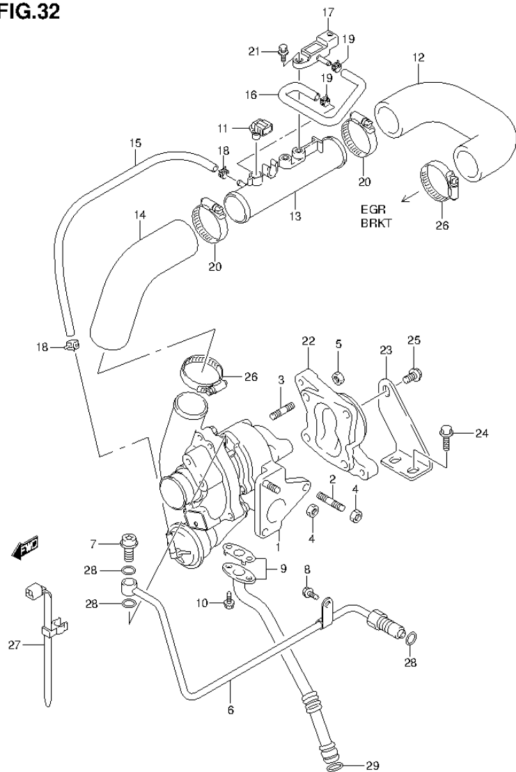
FIG.32 (1-E-9) TURBO CHARGER (SN415VD:TYPE 5)
