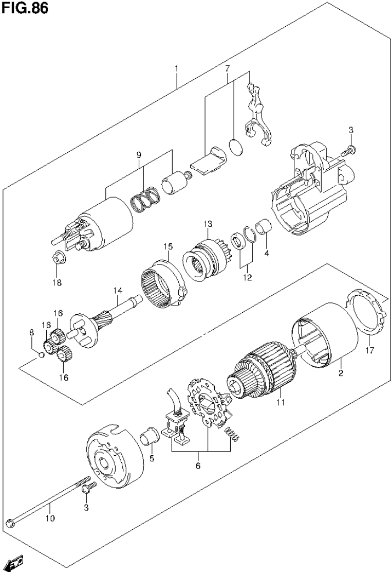
FIG.86 (1-K-13) STARTING MOTOR (SN415VD)
