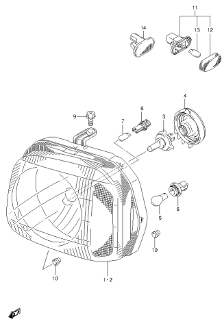
SN413V.5 E22_092 HEAD LAMP
