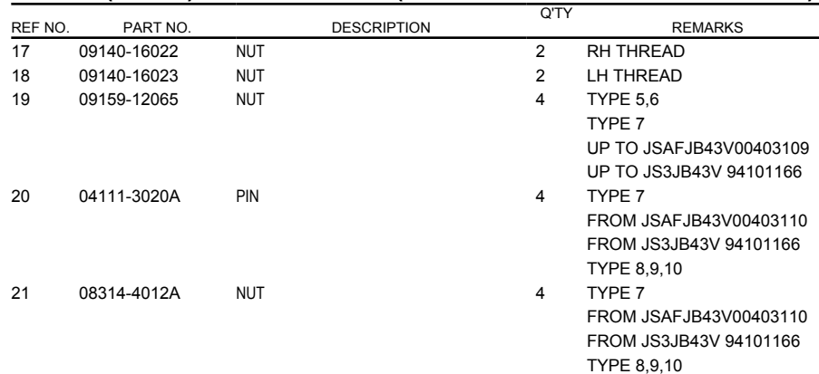
FIG.121 (2-H-12) STEERING UNIT (SN413V:RHD:N/POWER STEERING)
