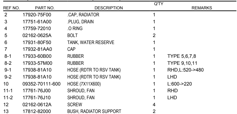
FIG.43 (1-F-14) RADIATOR (SN413V)
