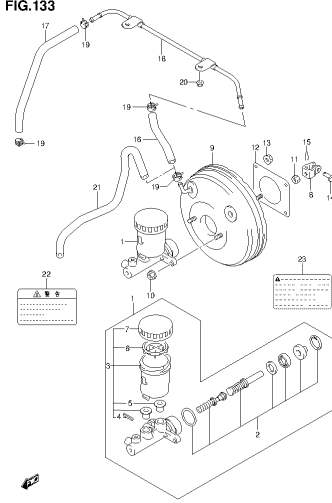
SN413V-5 E22_133 BRAKE MASTER CYLINDER (2)
