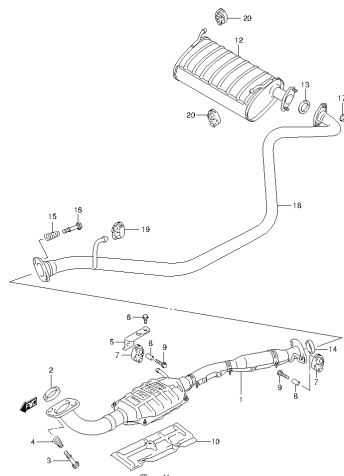
SN413V-5 E22_030 MUFFLER (2)
