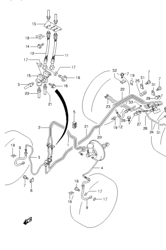
SN413V-5 E22_137 BRAKE PIPING (2)
