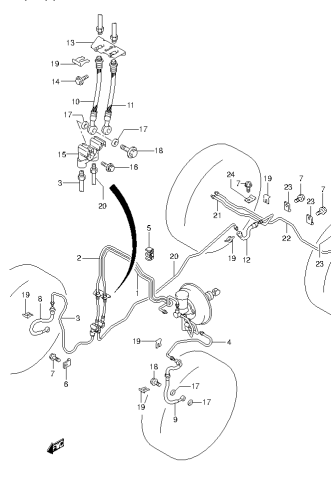
SN413V-5 E22_136 BRAKE PIPING (1)
