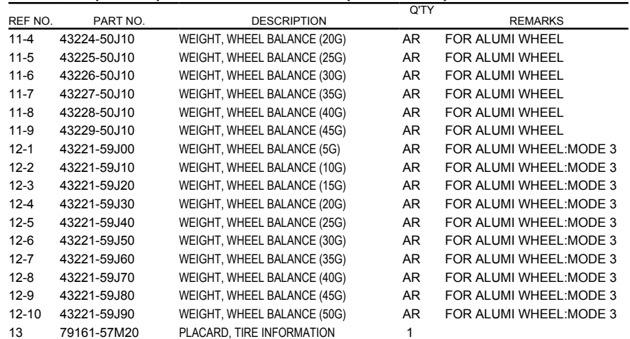
FIG.114B (2-G-14) ROAD WHEEL/TIRE (SEE NOTE)
