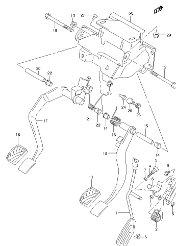
SN413V5 E22_129 PEDAL/PEDAL BRACKET (3)
