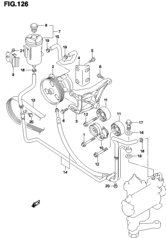
SN413V5 E22_126 POWER STEERING OIL PUMP (3)
