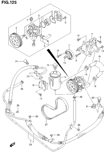
SN413V5 E22_125 POWER STEERING OIL PUMP (2)
