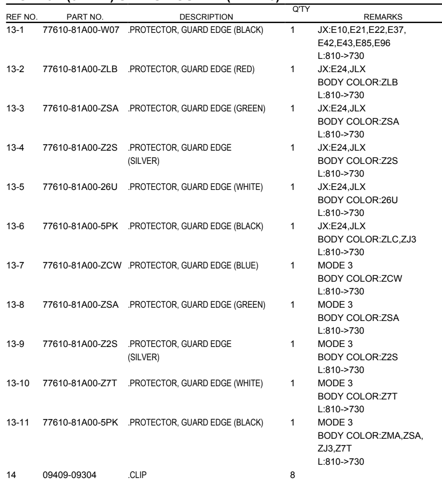
FIG.175A (3-E-14) SPLASH GUARD (TYPE 8)
