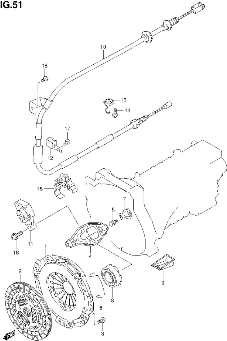
FIG.51 (1-G-15) MT CLUTCH (MT:SN413V:LHD)
