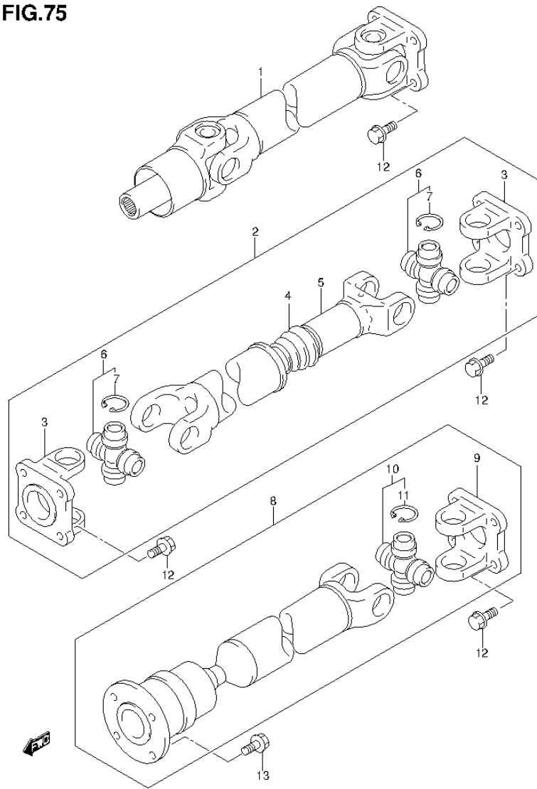
SN413V-5 E22_075 PROPELLER SHAFT (1)
