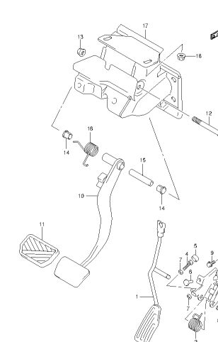
SN413V5 E22_130 PEDAL/PEDAL BRACKET (4)
