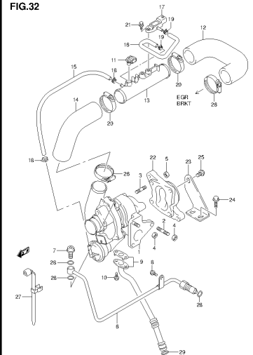
SN413V-5 E22_032 TURBO CHARGER (1)
