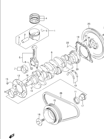
SN413V-5 E22_013 CRANKSHAFT (1)
