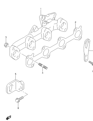
SN413V-5 E22_08A EXHAUST MANIFOLD (5)
