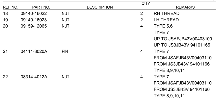
FIG.122 (2-H-14) STEERING UNIT (SN413V:RHD:W/POWER STEERING)
