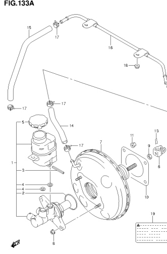
SN413V-5 E22_133A BRAKE MASTER CYLINDER (3)
