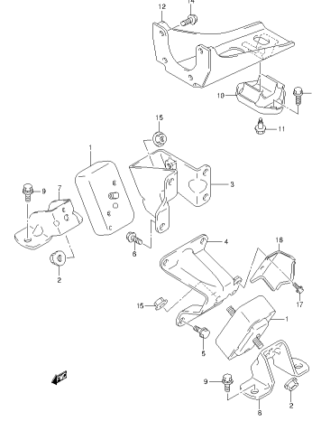
SN413V-5 E22_011A ENGINE MOUNTING (2)
