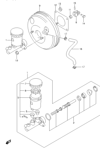
SN413V-5 E22_135 BRAKE MASTER CYLINDER (5)
