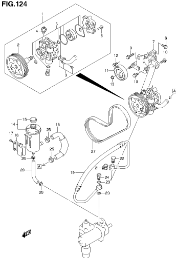
SN413V5 E22_124 POWER STEERING OIL PUMP (1)
