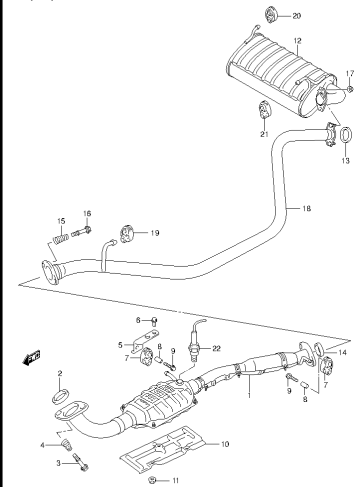
SN413V-5 E22_029 MUFFLER (1)
