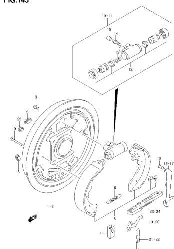
SN413V 5 E22_145 REAR WHEEL BRAKE
