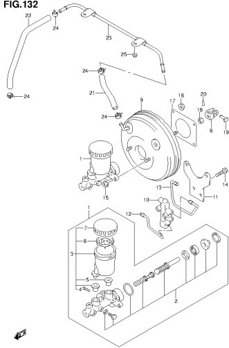
SN413V-5 E22_132 BRAKE MASTER CYLINDER (1)
