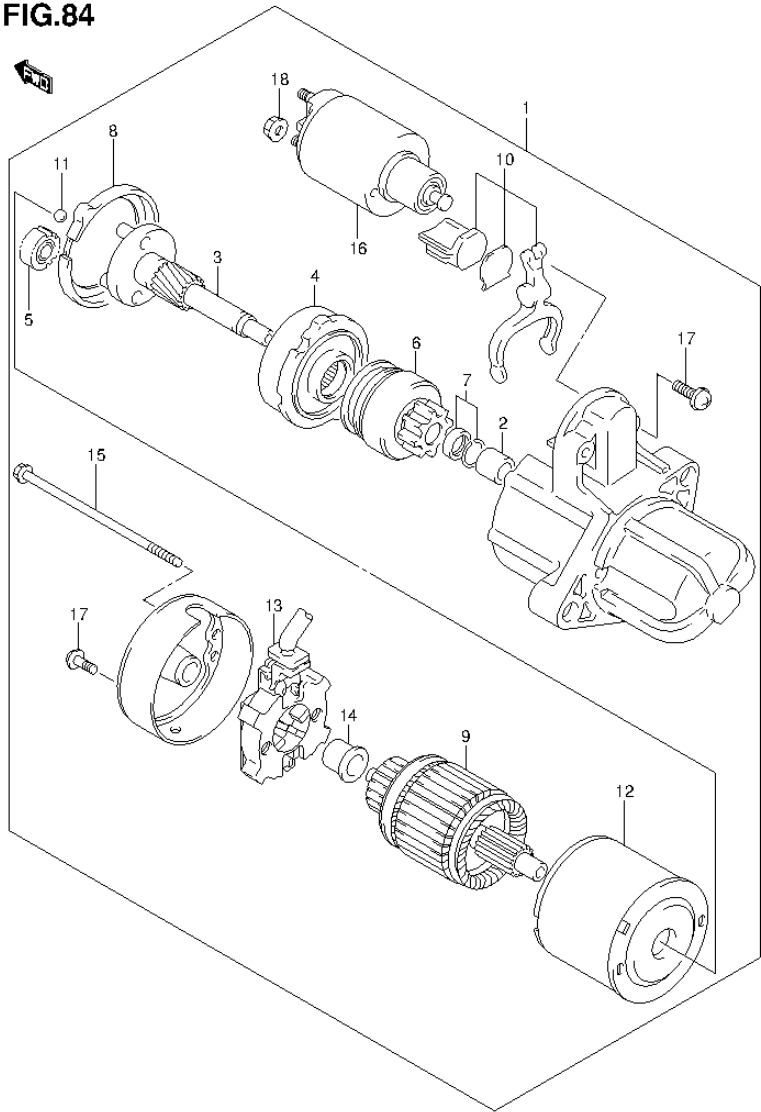
FIG.84 (1-K-10) STARTING MOTOR (TYPE 5:SN413V:E2,E22)
