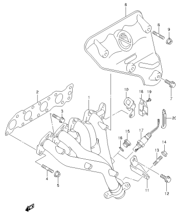
SN413V-5 E22_07A EXHAUST MANIFOLD (4)
