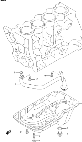
SN413V-5 E22_009 OIL PAN (1)
