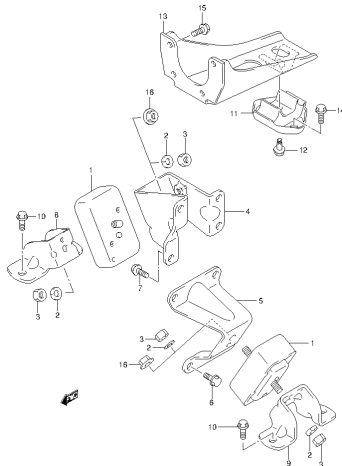
SN413V-5 E22_011 ENGINE MOUNTING (1)
