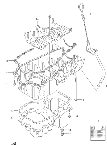
SN413V-5 E22_010 OIL PAN (2)
