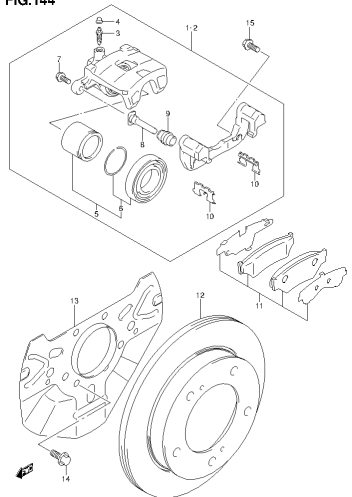
SN413V 5 E22_144 FRONT WHEEL BRAKE (2)
