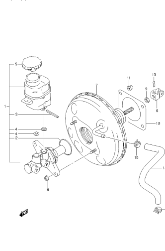
SN413V-5 E22_135A BRAKE MASTER CYLINDER (6)
