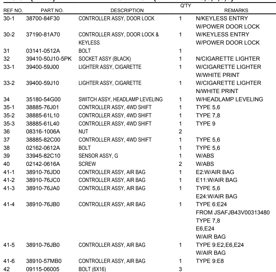
FIG.97 (2-E-6) ELECTRICAL CONTROL (RHD:TYPE 5,6,7,8,9)
