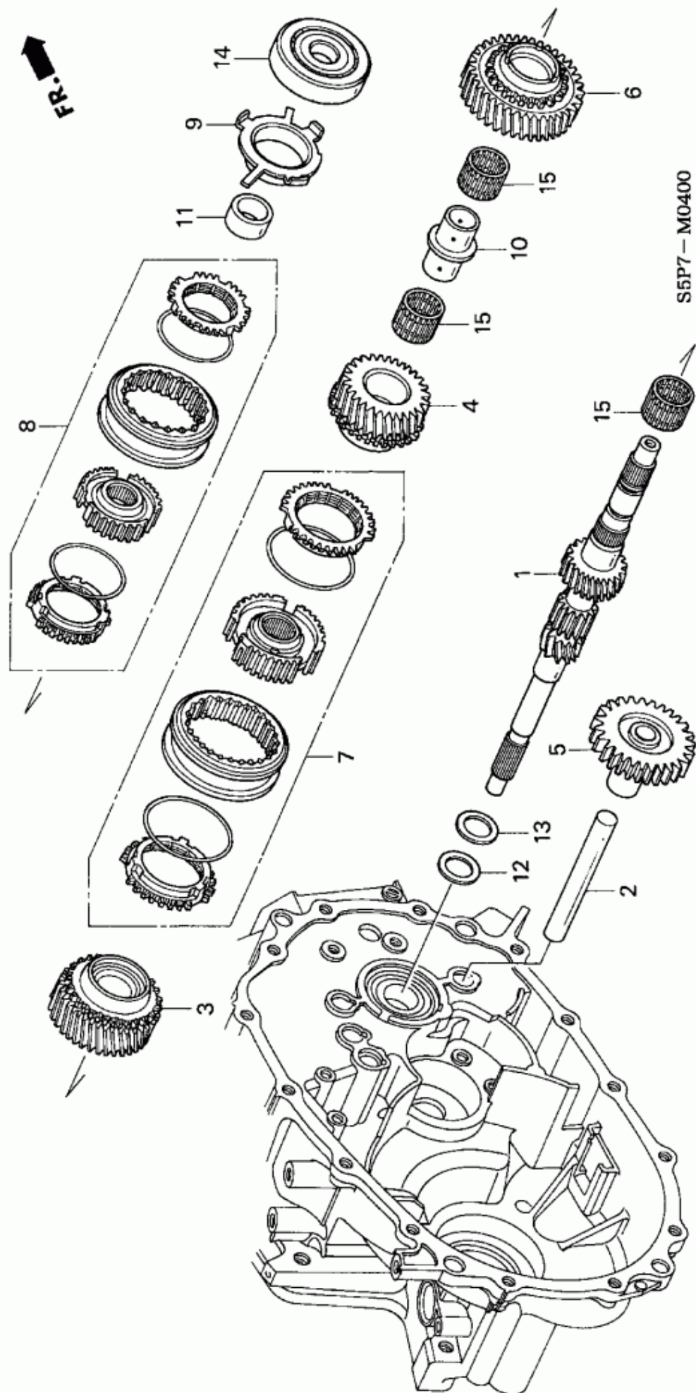
Figure 1: M-4 - MAINSHAFT
