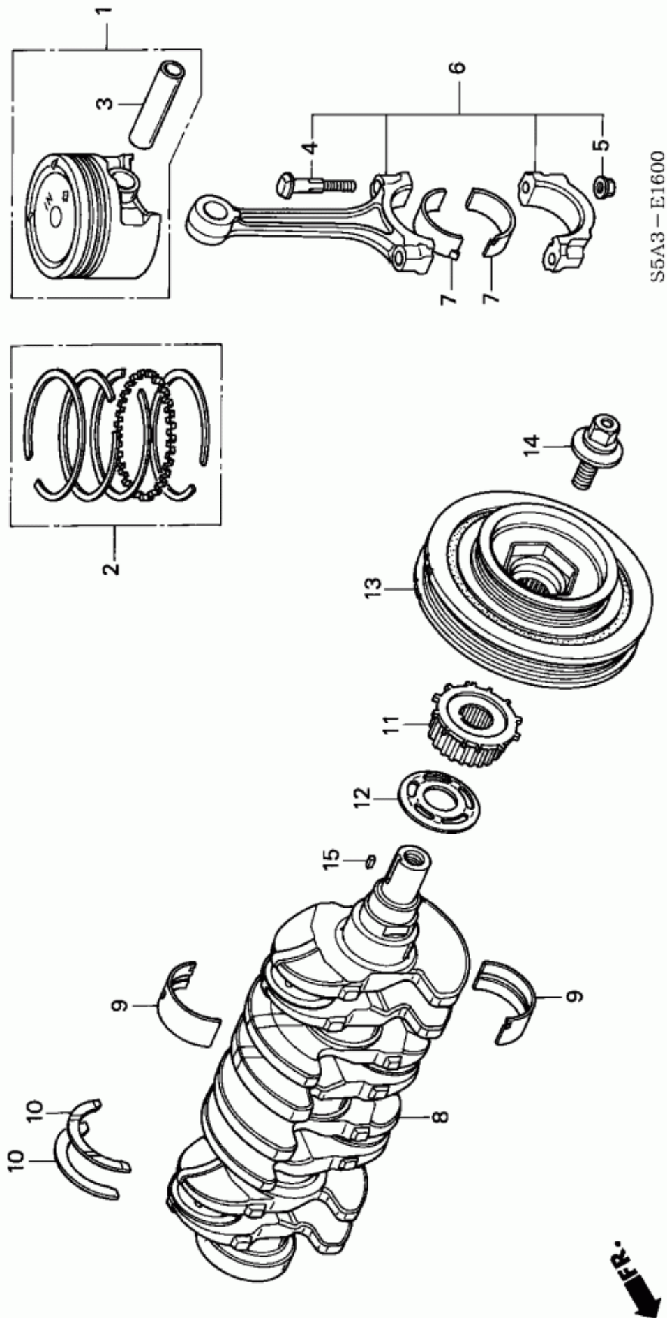
Figure 1: E-16 - PISTON/CRANKSHAFT
