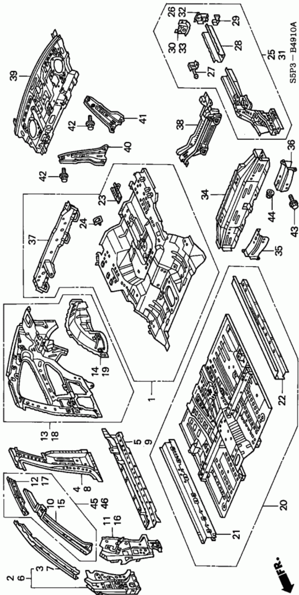
Figure 1: B-49-10 - INNER PANELS
