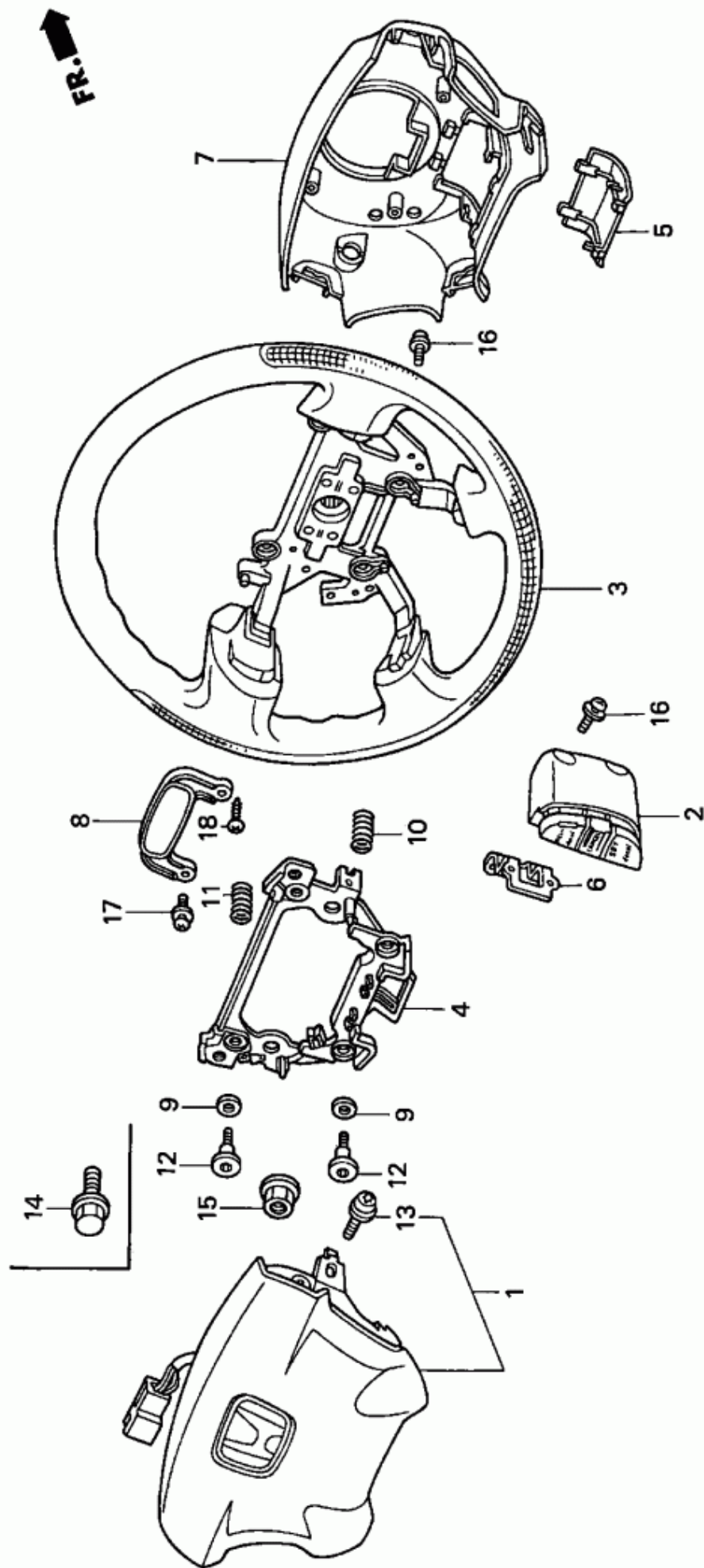
Figure 1: B-31-10 - STEERING WHEEL (SRS)
