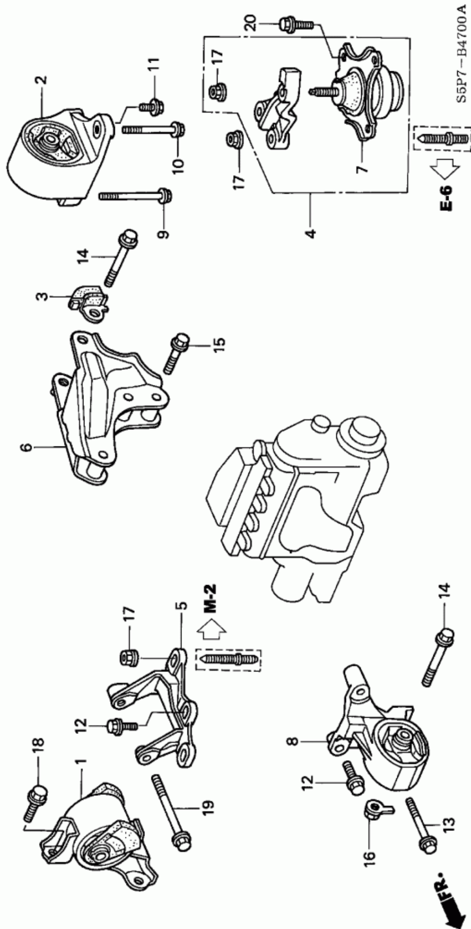
Figure 1: B-47 - ENGINE MOUNTS (MT)
