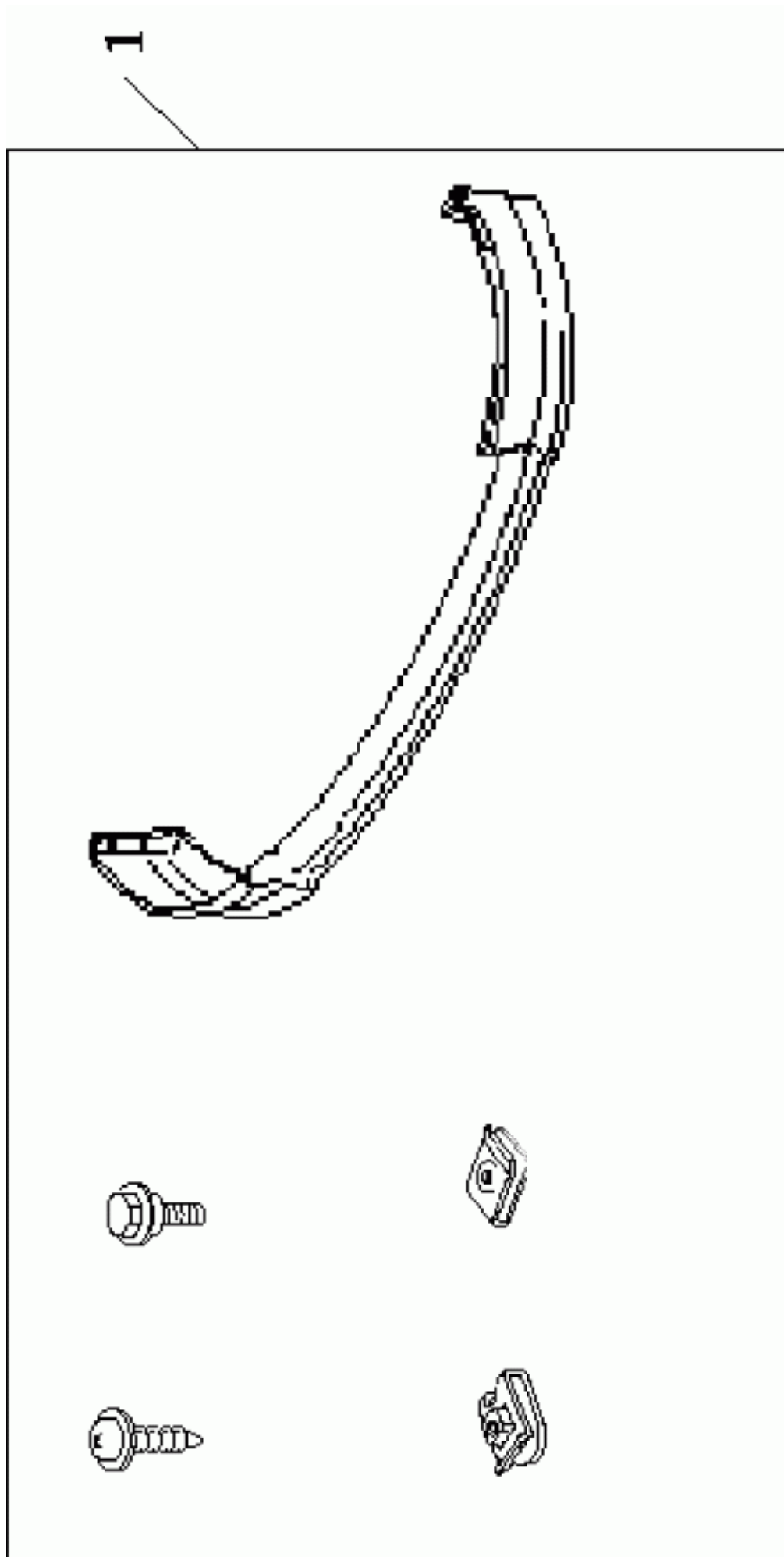
Figure 1: 08F-01-02 - SPOILER, FR PRIM
