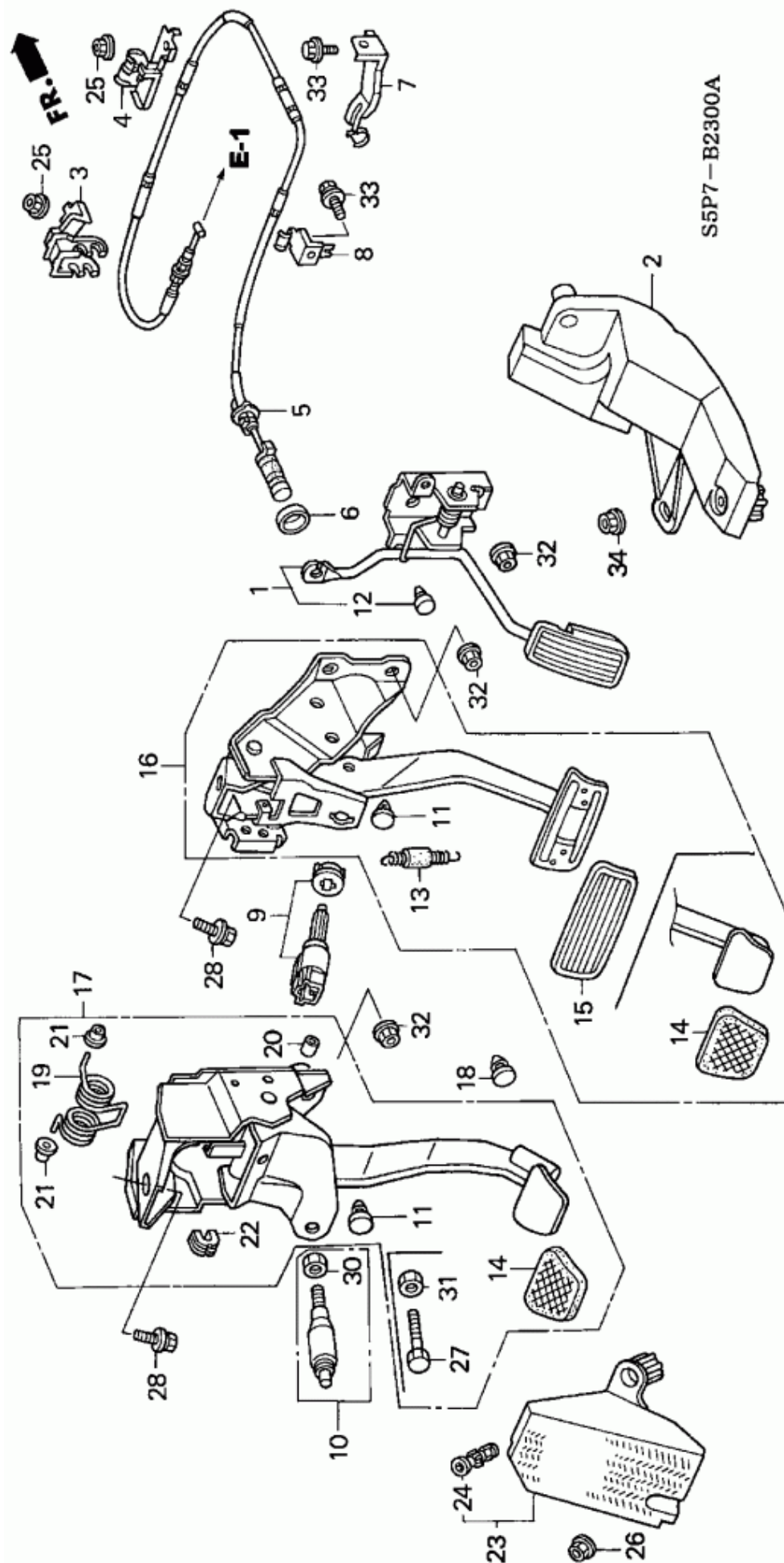
Figure 1: B-23 - PEDAL (LH)
