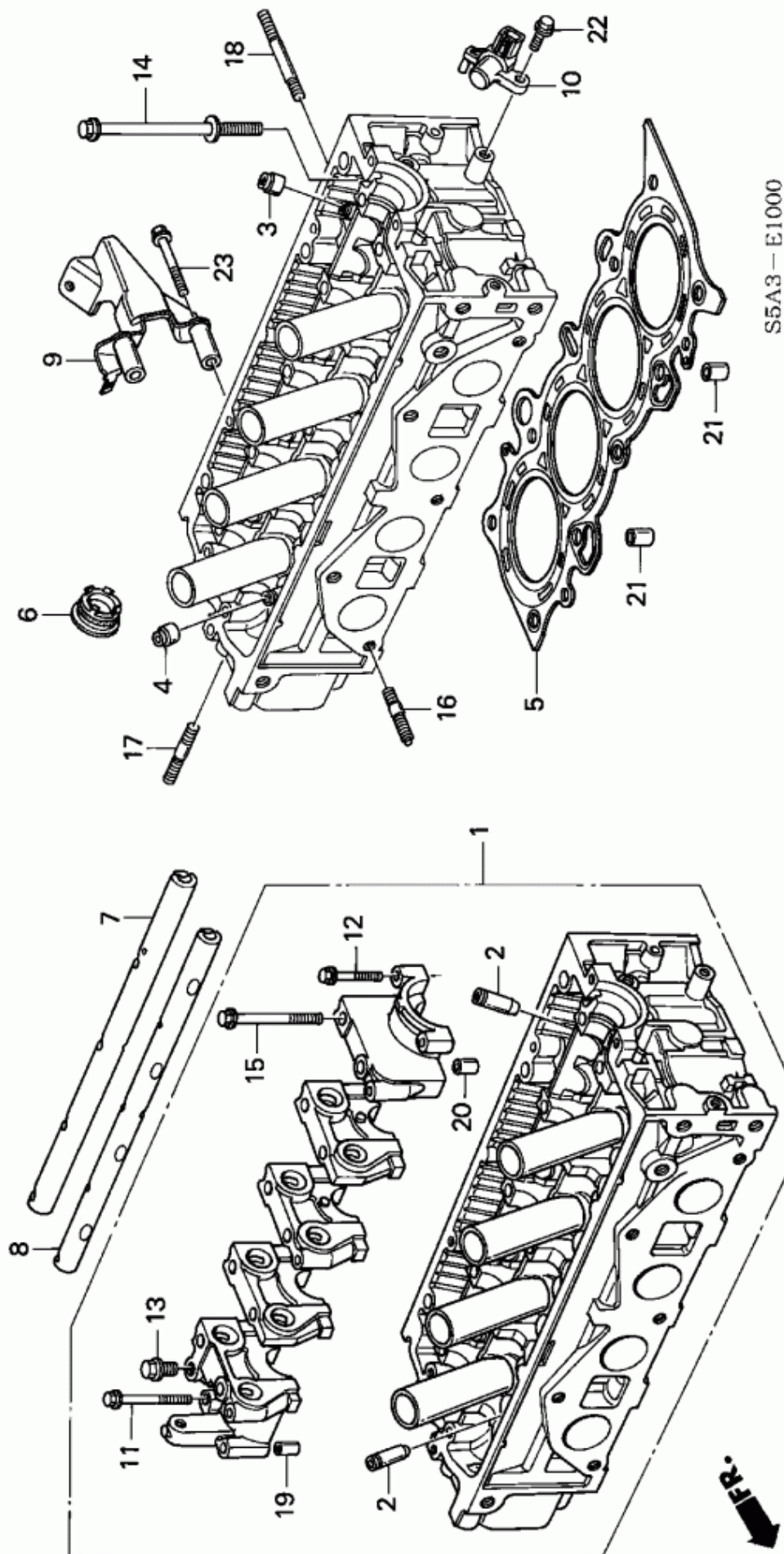
Figure 1: E-10 - CYLINDER HEAD (SOHC)
