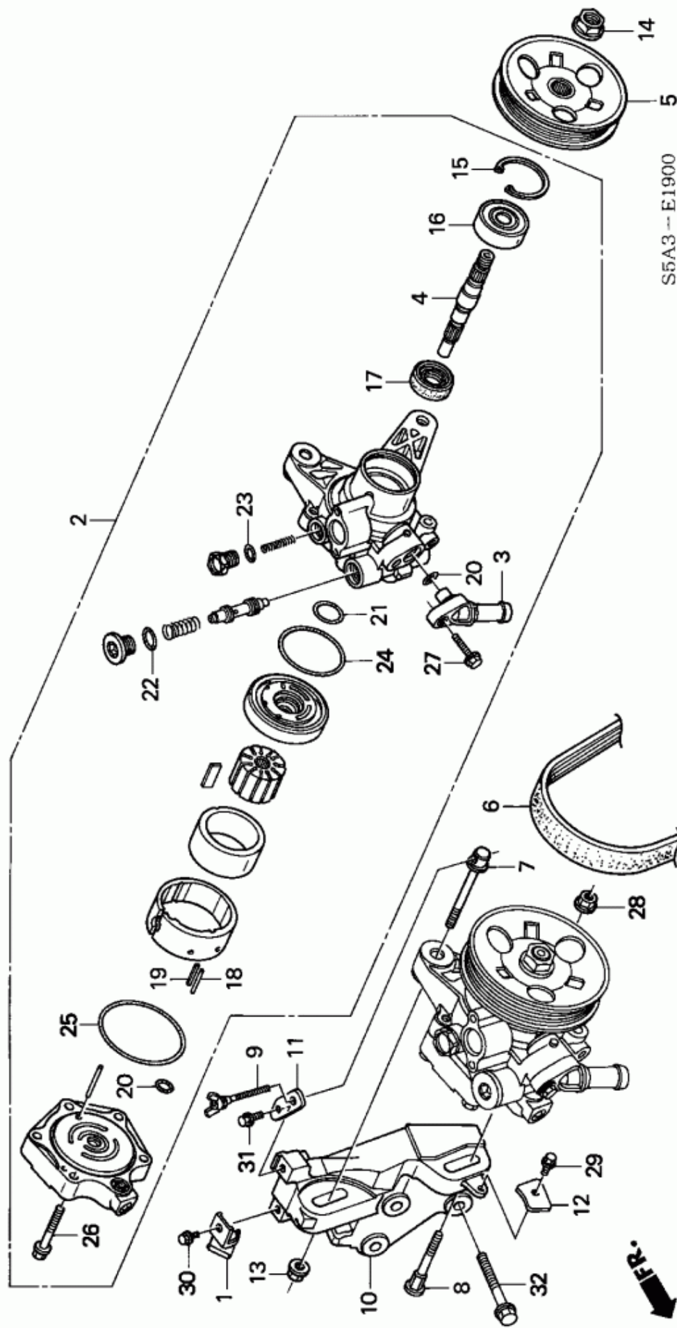
Figure 1: E-19 - POWER STEERING PUMP/ BRACKET
