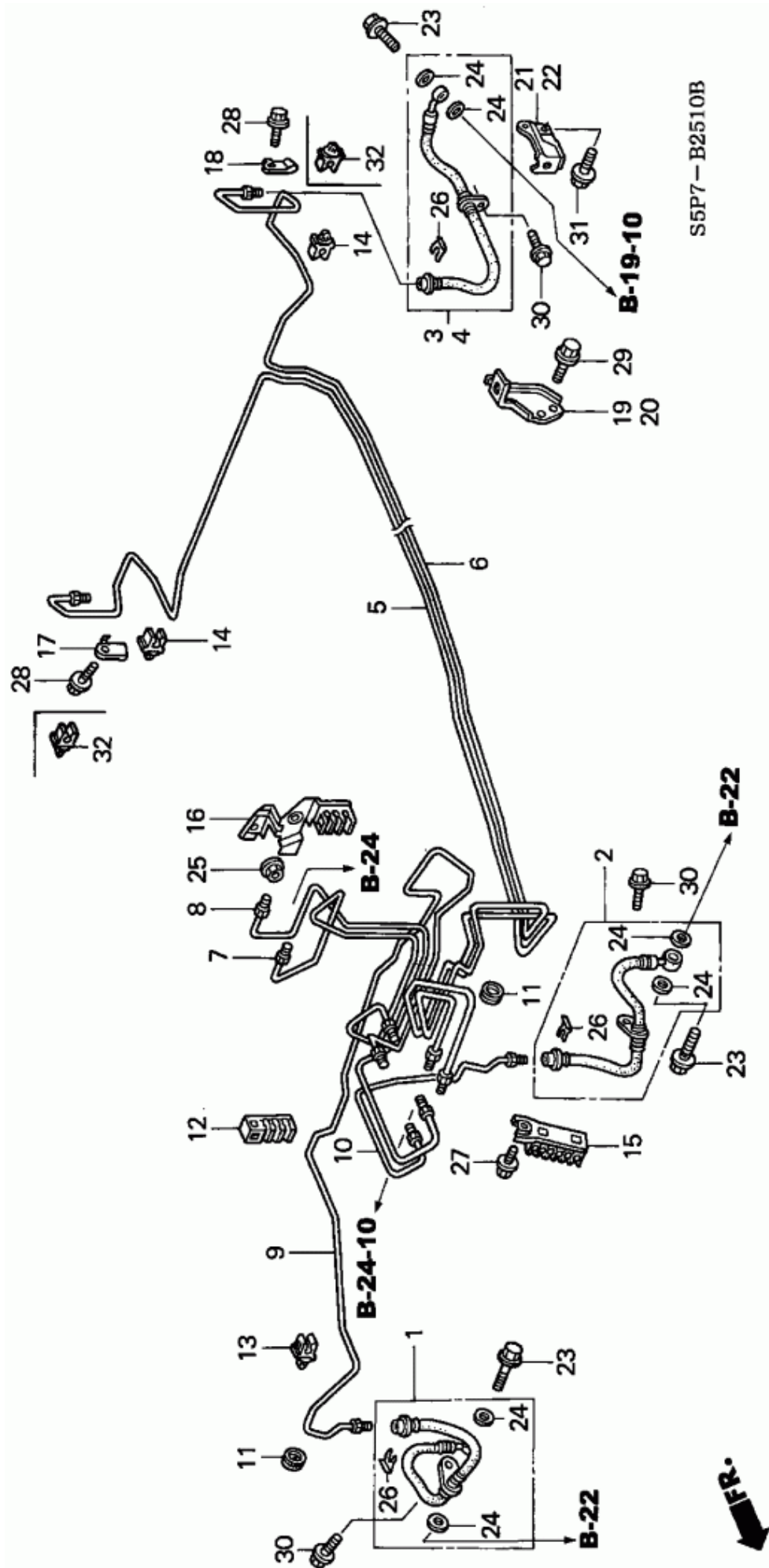
Figure 1: B-25-10 - BRAKE LINES (ABS) (LH) (1)
