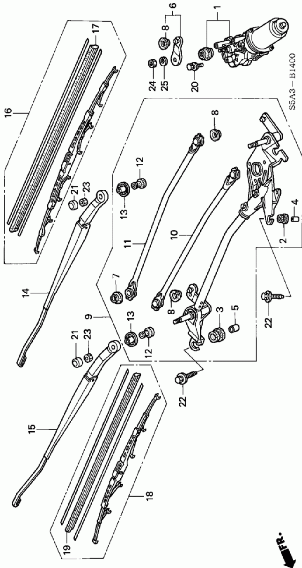
Figure 1: B-14 - FRONT WIPER (LH)
