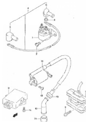
FIG.23 ELECTRICAL (D-12)
