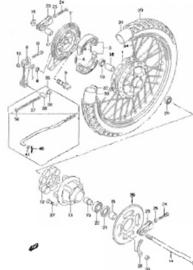
FIG.63 REAR WHEEL (EN125HUK9/HUZK9) (I-4)
