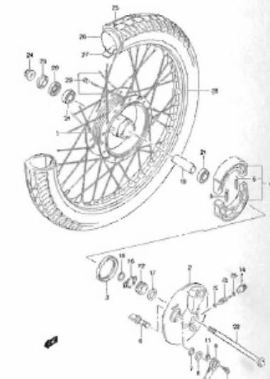
FIG.56 FRONT WHEEL (EN125HUK9/HUK9) (I-3)
