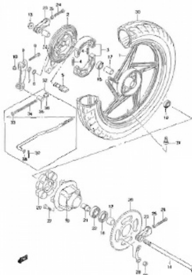
FIG.62 REAR WHEEL (EN125-2AK9) (I-2)
