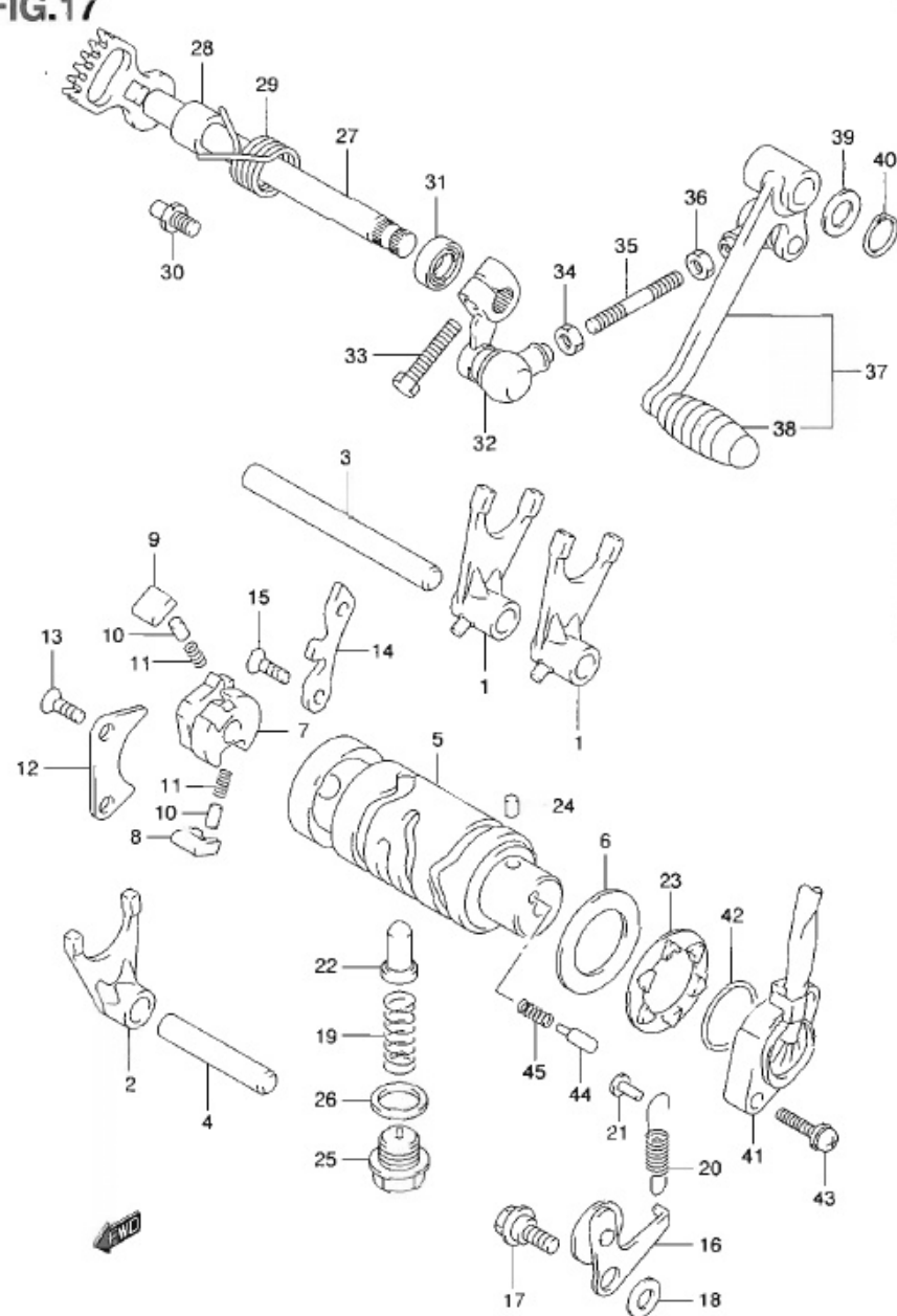
EN125-2AK9 P71_017 GEAR SHIFTING
