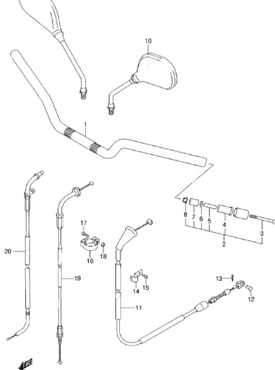
EN125-2AK9 P71_041 HANDLEBAR
