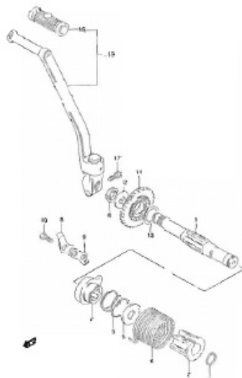
FIG.18 KICK STARTER (EN125HUK9/HUZK9) (D-7)
