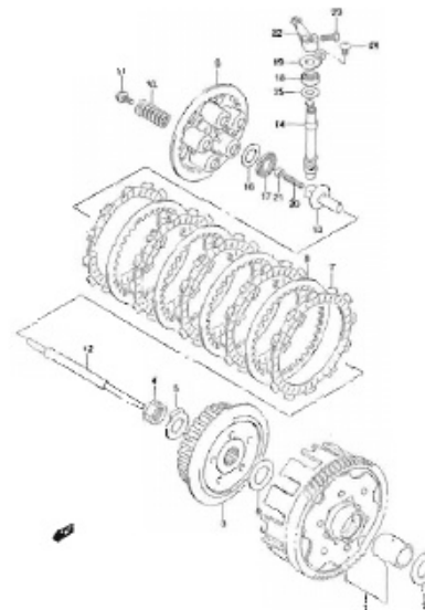
FIG.15 CLUTCH (D-2)
