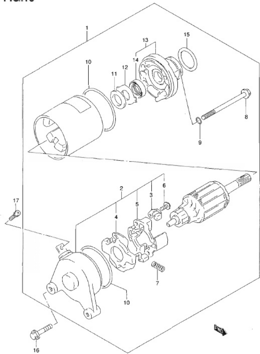
EN125-2AK9 P71_019 STARTING MOTOR
