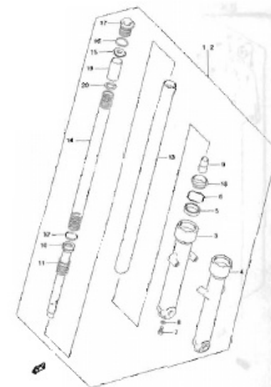
FIG.52 FRONT DAMPER (EN125HUK9/HUK9) (H-7)
