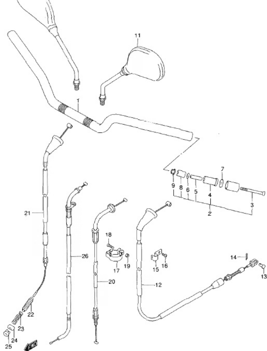
EN125-2AK9 P71_042 HANDLEBAR
