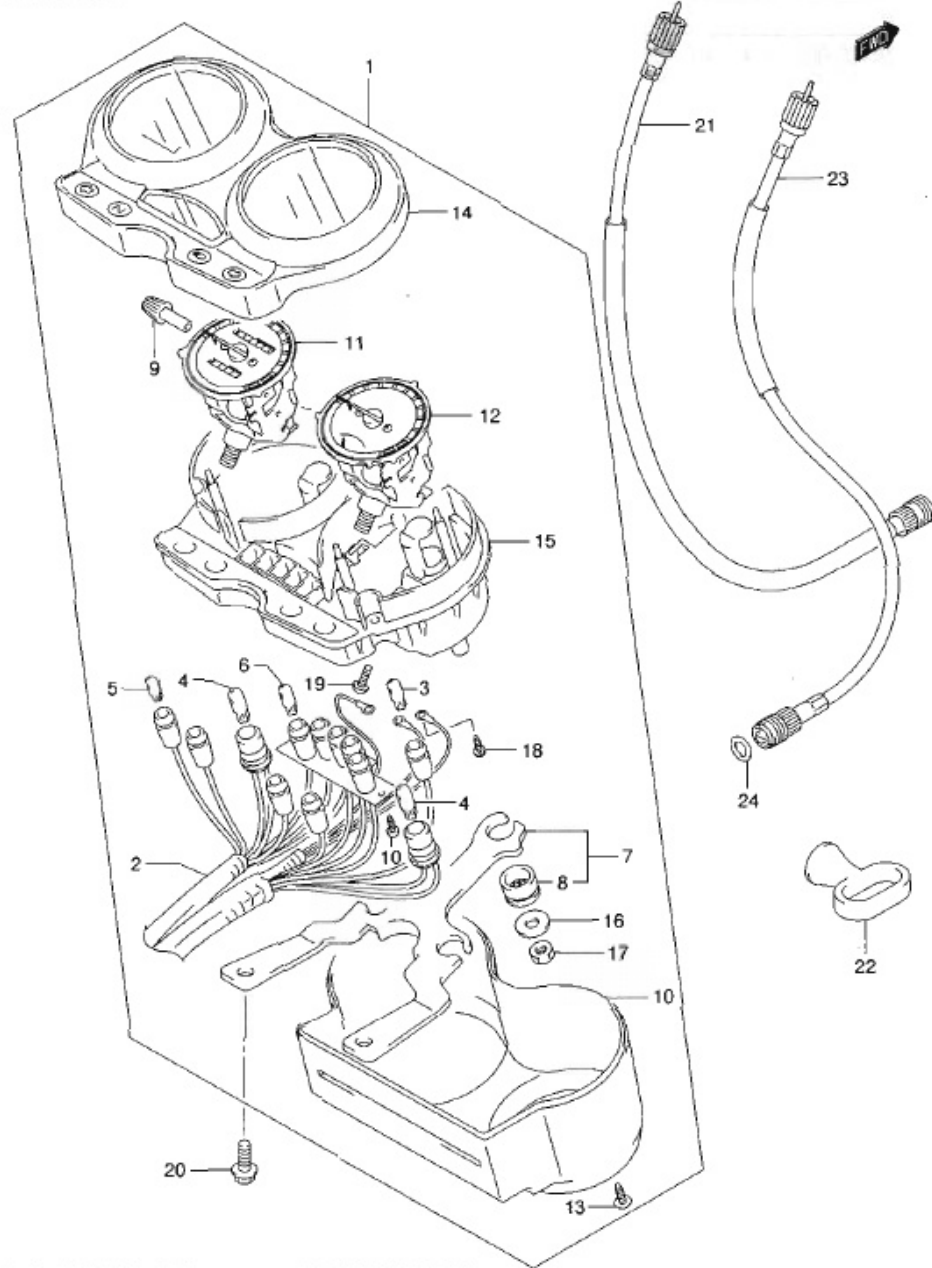
EN125-2AK9 P71_024 SPEEDOMETER
