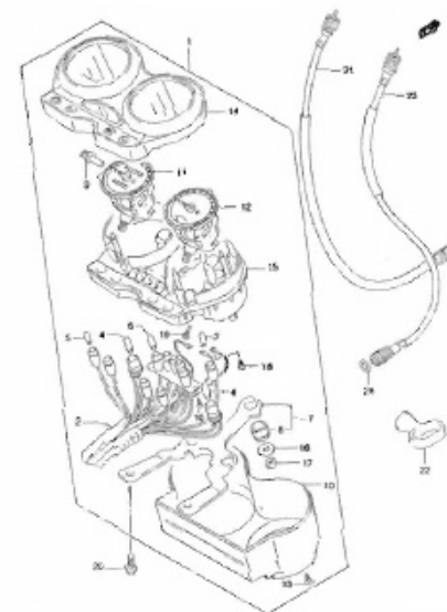
FIG.24 SPEEDOMETER (D-13)
