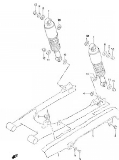
FIG.60 CHAIN CASE (EN125-2AK9) (I-7)
