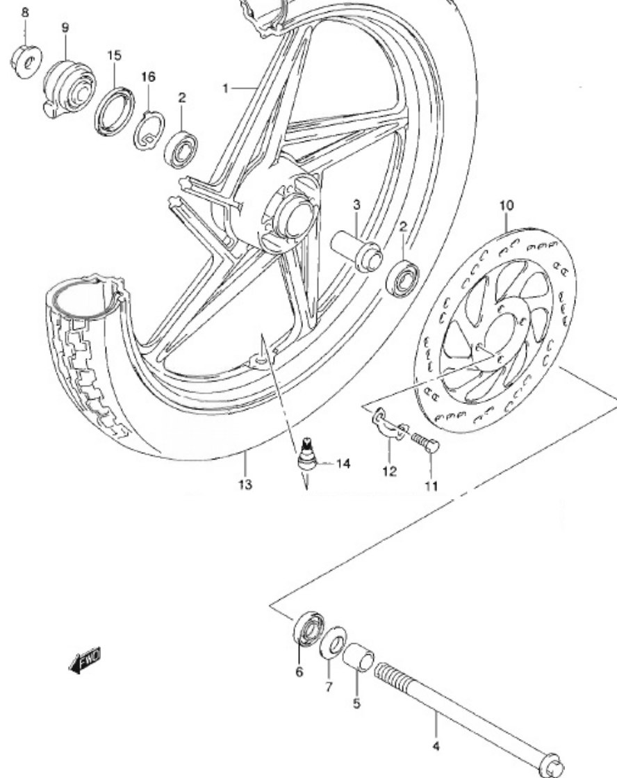
EN125-2AK9 P71_055 FRONT WHEEL
