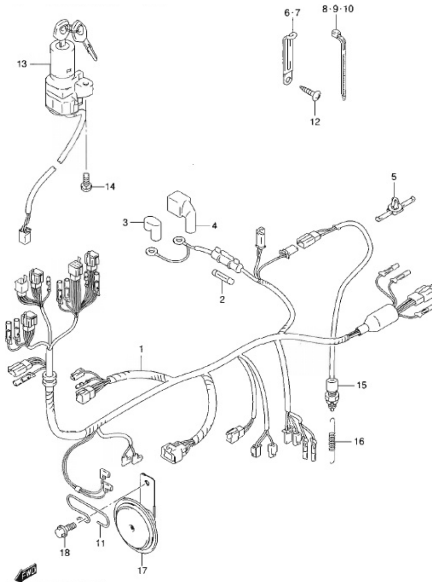
EN125-2AK9 P71_028 WIRING HARNESS
