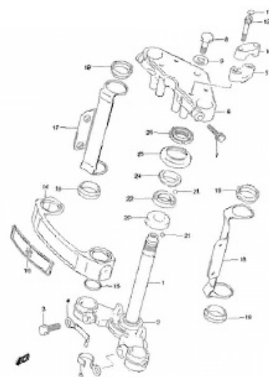
FIG.54 STEERING STEM (EN125HUK9/HUK9) (H-9)
