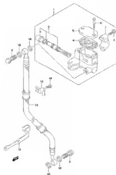
FIG.58 FRONT MASTER CYLINDER (EN125-2AK9) (I-5)
