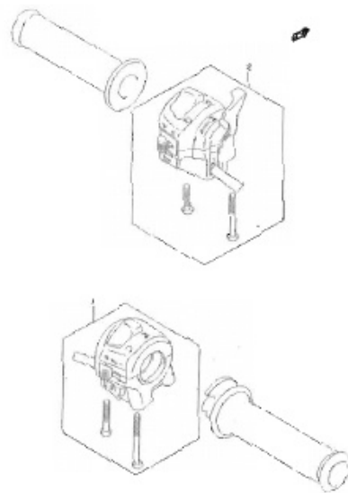
FIG.29 HANDLE SWITCH (E-6)
