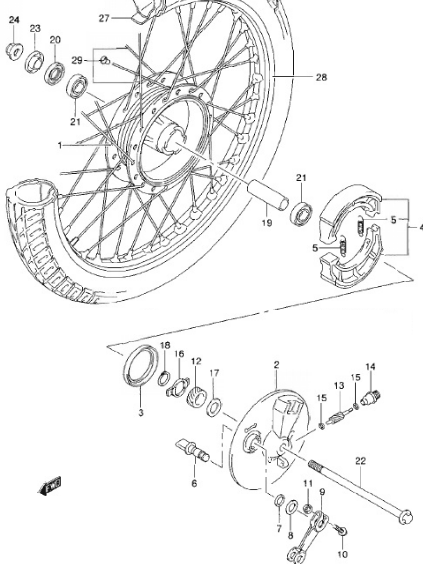
EN125-2AK9 P71_056 FRONT WHEEL
