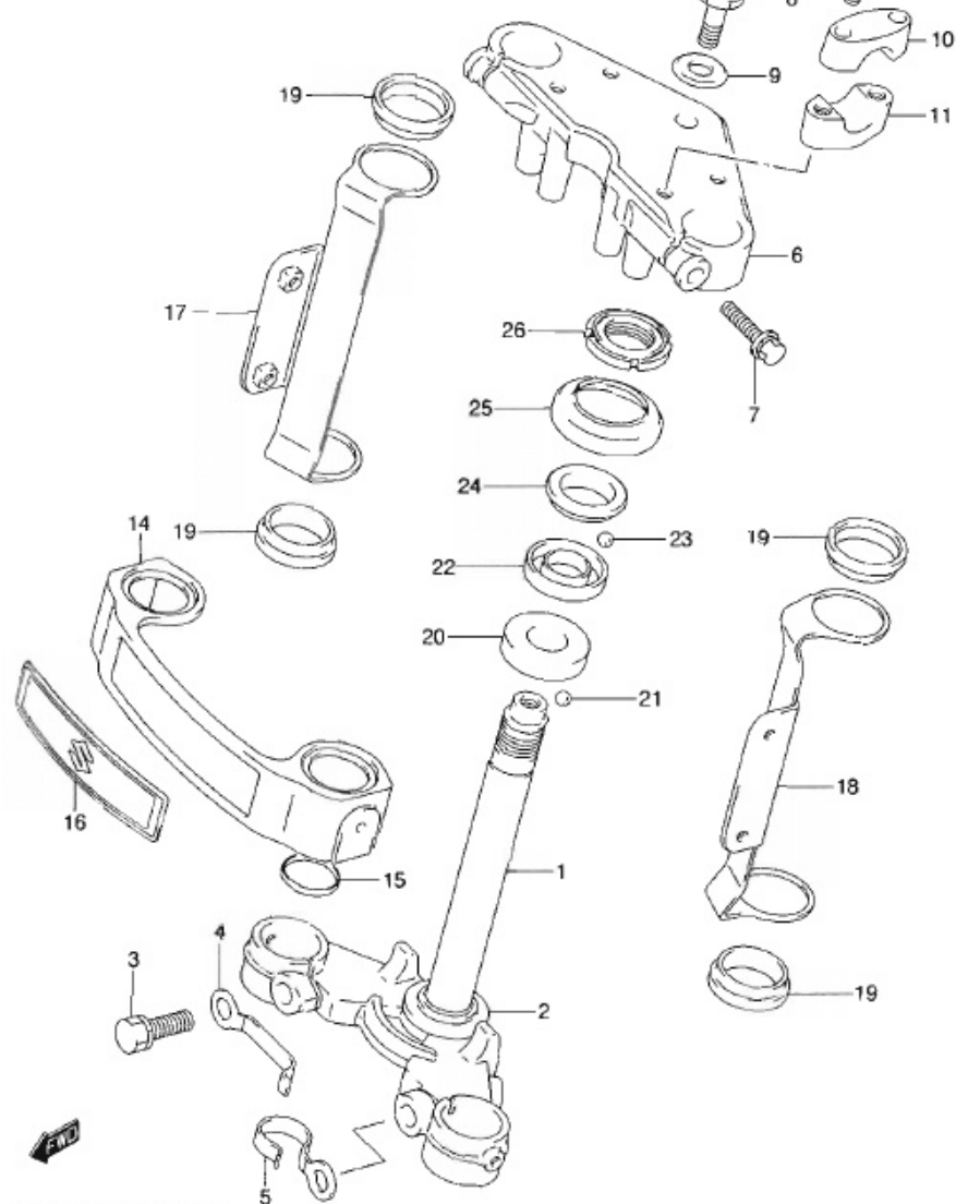
EN125-2AK9 P71_054 STEERING STEM
