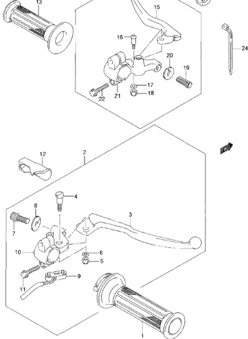
EN125-2AK9 P71_044 HANDLE LEVER
