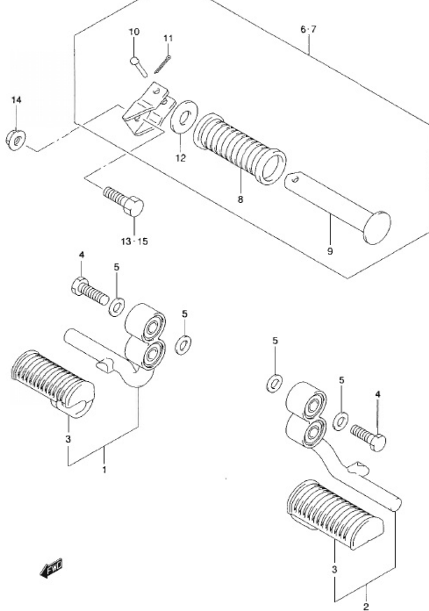
EN125-2AK9 P71_033 FOOTREST
