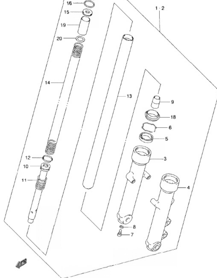
EN125-2AK9 P71_051 FRONT DAMPER
