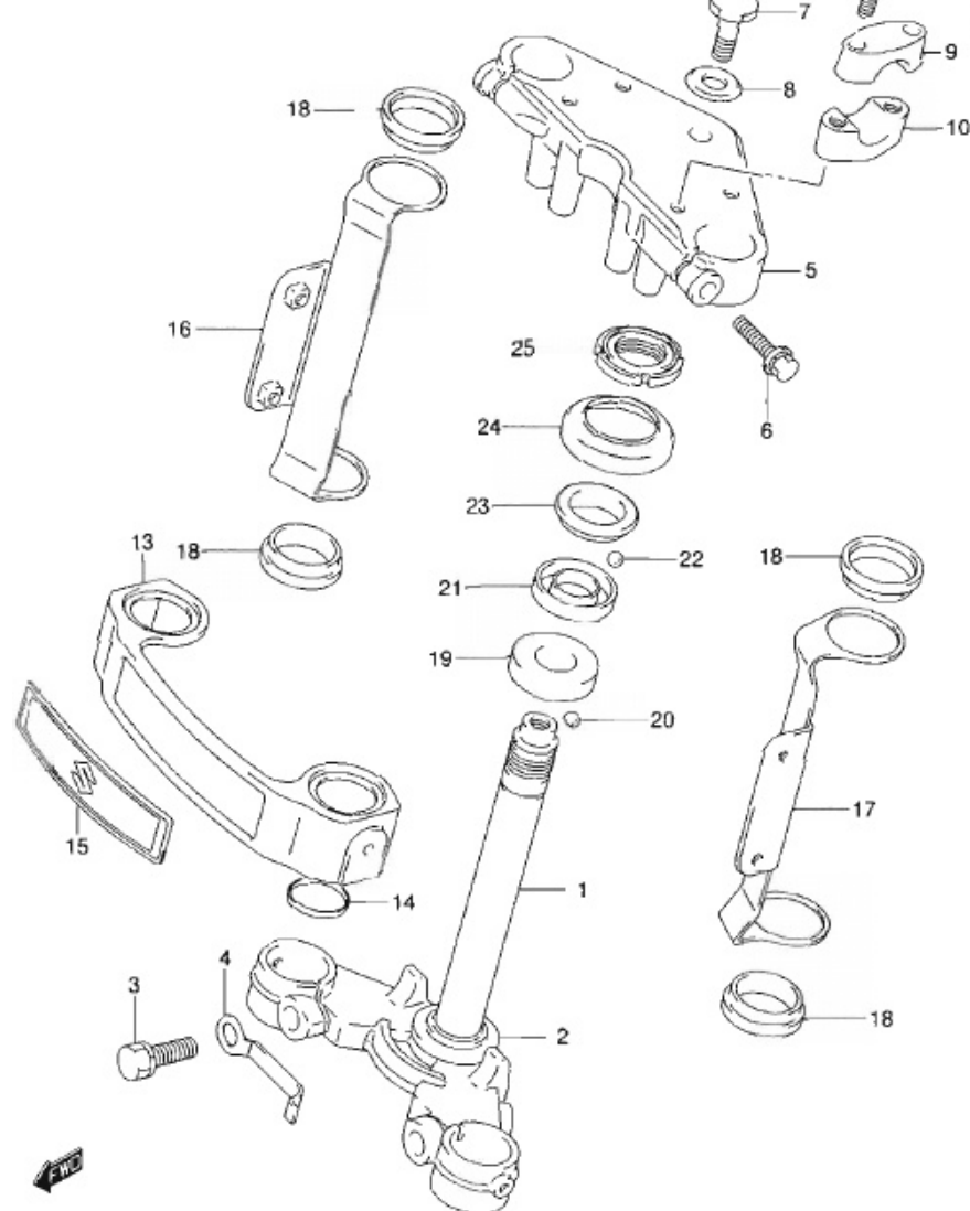
EN125-2AK9 P71_053 STEERING STEM
