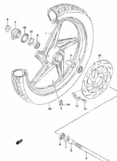
FIG.55 FRONT WHEEL (EN125-2AK9) (I-2)
