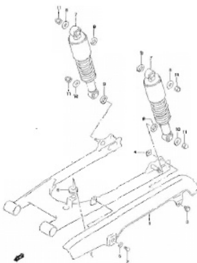
FIG.61 CHAIN CASE (EN125HUK9/HUZK9) (I-8)
