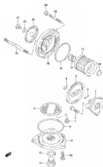
FIG.14 OIL PUMP (C-11)
