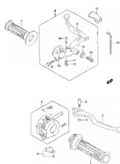
FIG.43 HANDLE LEVER (EN125-2A) (G-2)
