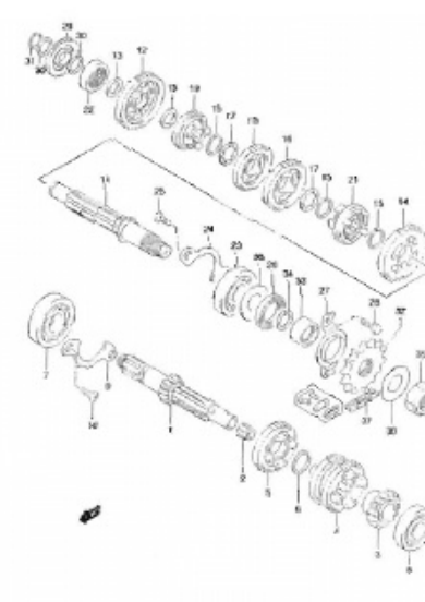
FIG.16 TRANSMISSION (D-3)
