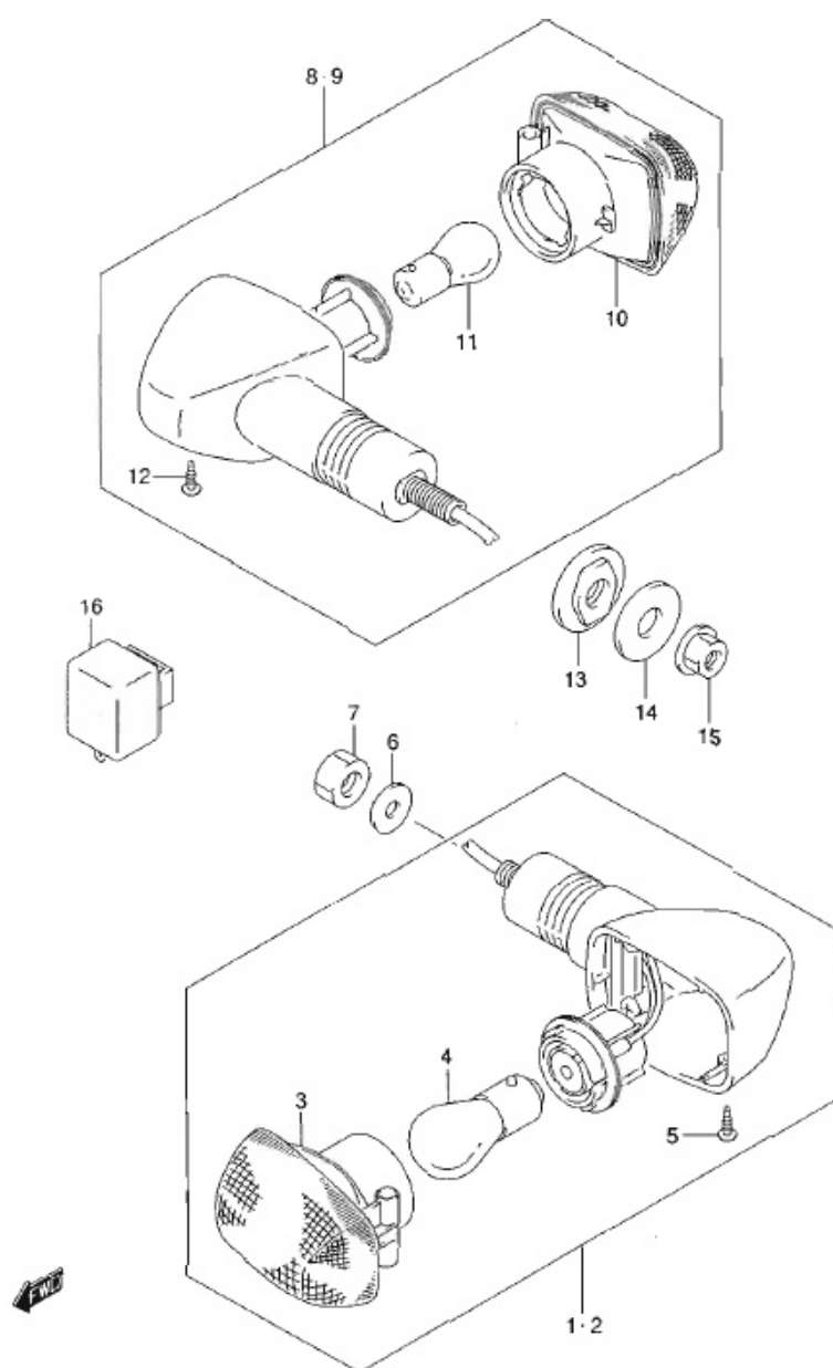
EN125-2AK9 P71_026 TURN SIGNAL LAMP
