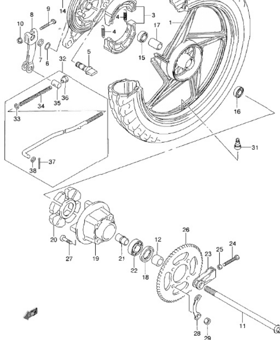
EN125-2AK9 P71_062 REAR WHEEL
