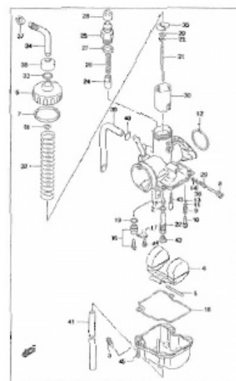
FIG.11 CARBURETOR (EN125HUK9/HUZK9) (C-7)
