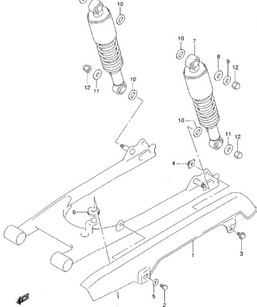
EN125-2AK9 P71_060 CHAIN CASE
