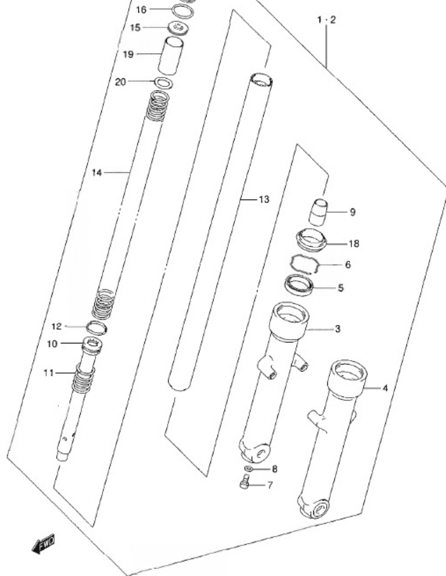
EN125-2AK9 P71_052 FRONT DAMPER
