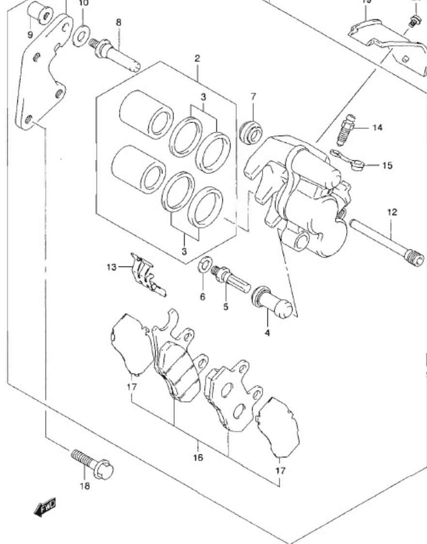
EN125-2AK9 P71_057 FRONT CALIPER
