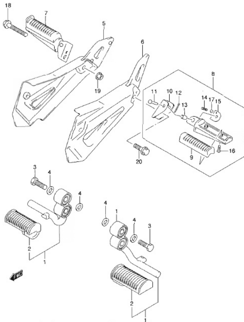
EN125-2AK9 P71_032 FOOTREST
