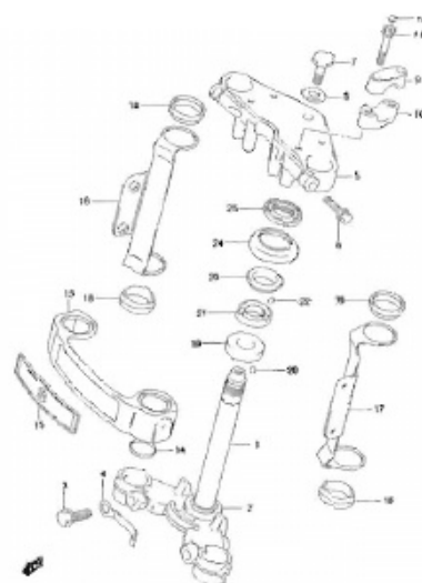
FIG.53 STEERING STEM (EN125-2AK9) (H-8)
