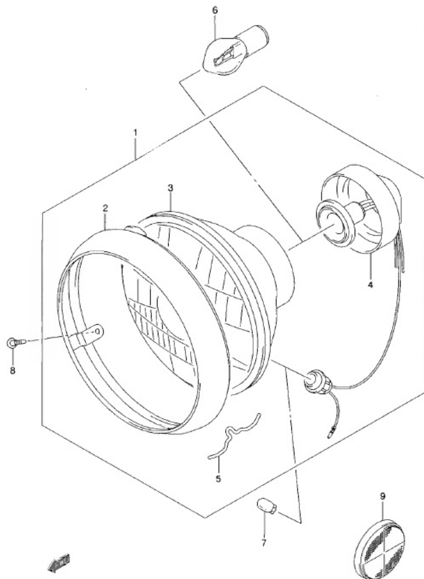
EN125-2AK9 P71_025 HEADLAMP
