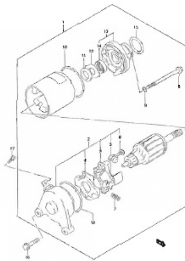
FIG.23 ELECTRICAL (D-12)
