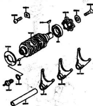
B-10 Gear Change Drum/Shift Fork(s)
