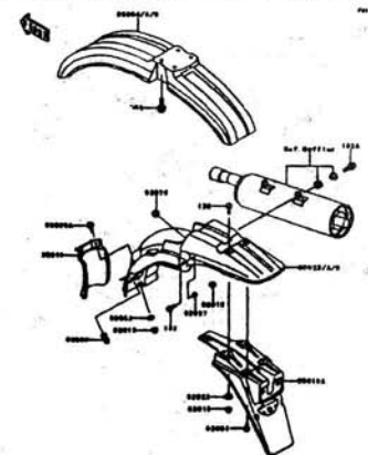
D-8 Fenders
