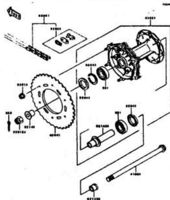
D-12 Rear Hub
