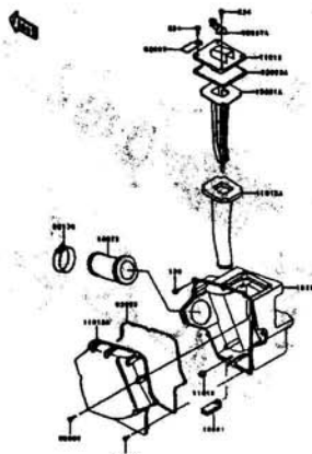
B-4 Air Cleaner
