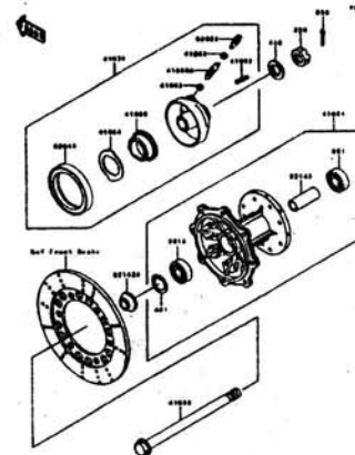
D-11 Front Hub
