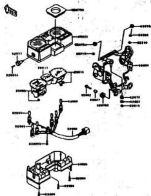
E-12 Meter(s)
