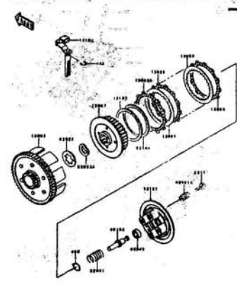
B-8 Clutch
