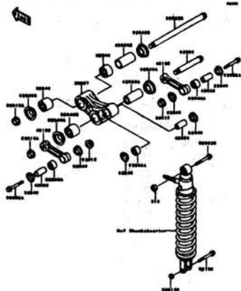
D-6 Suspension
