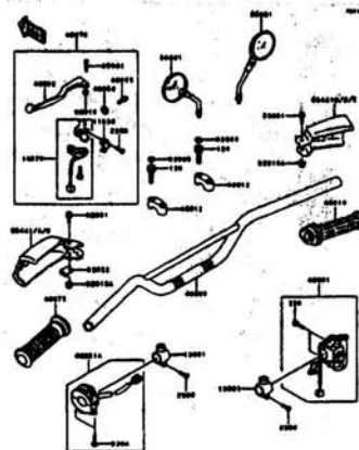
E-7 Handlebar
