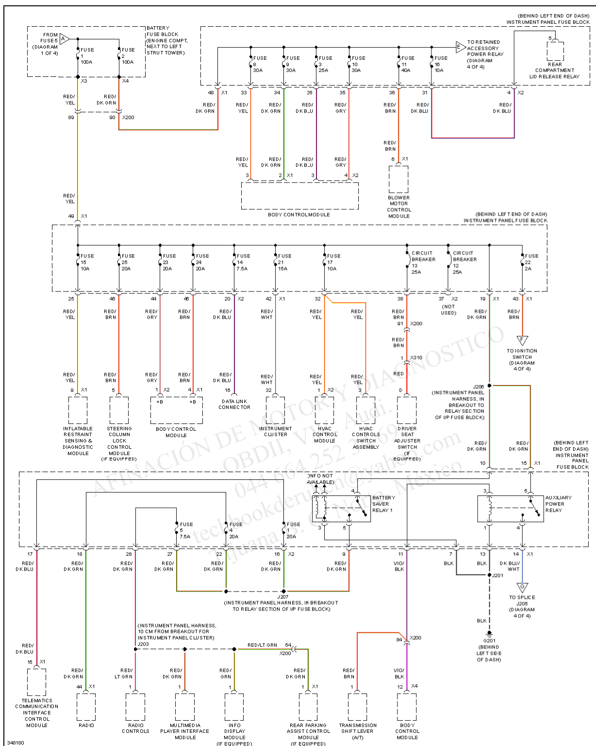
Fig. 49: Power Distribution Circuit (3 of 4)
