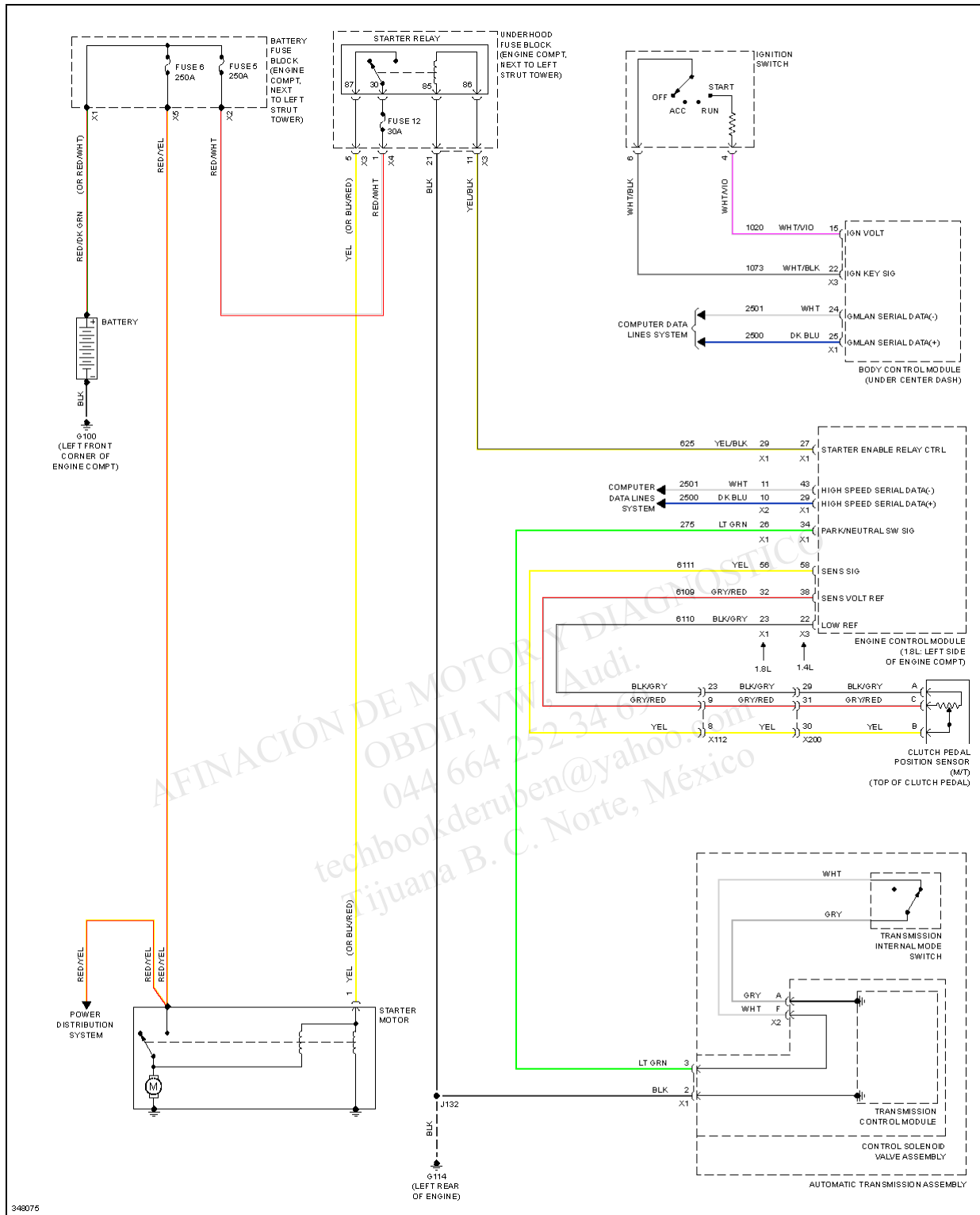
Fig. 70: Starting Circuit
