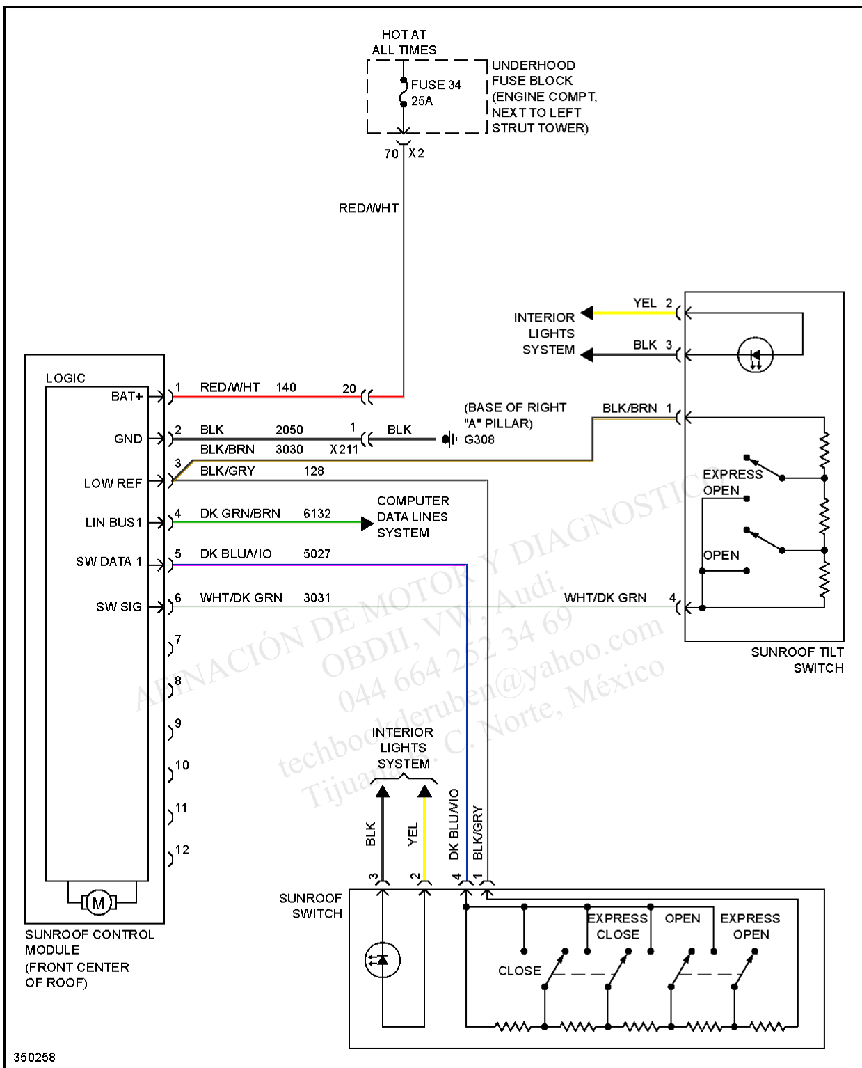
SYSTEM WIRING DIAGRAMS Fig. 57: Power Top/Sunroof Circuit
