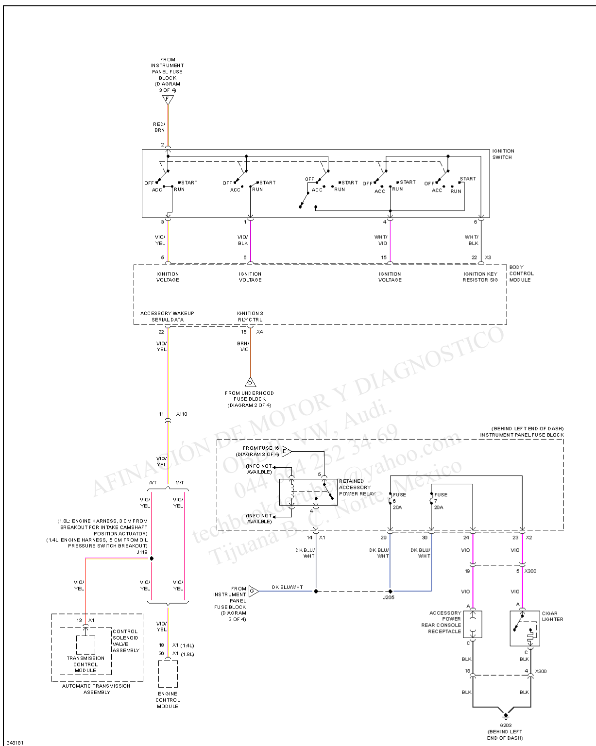
Fig. 50: Power Distribution Circuit (4 of 4)
