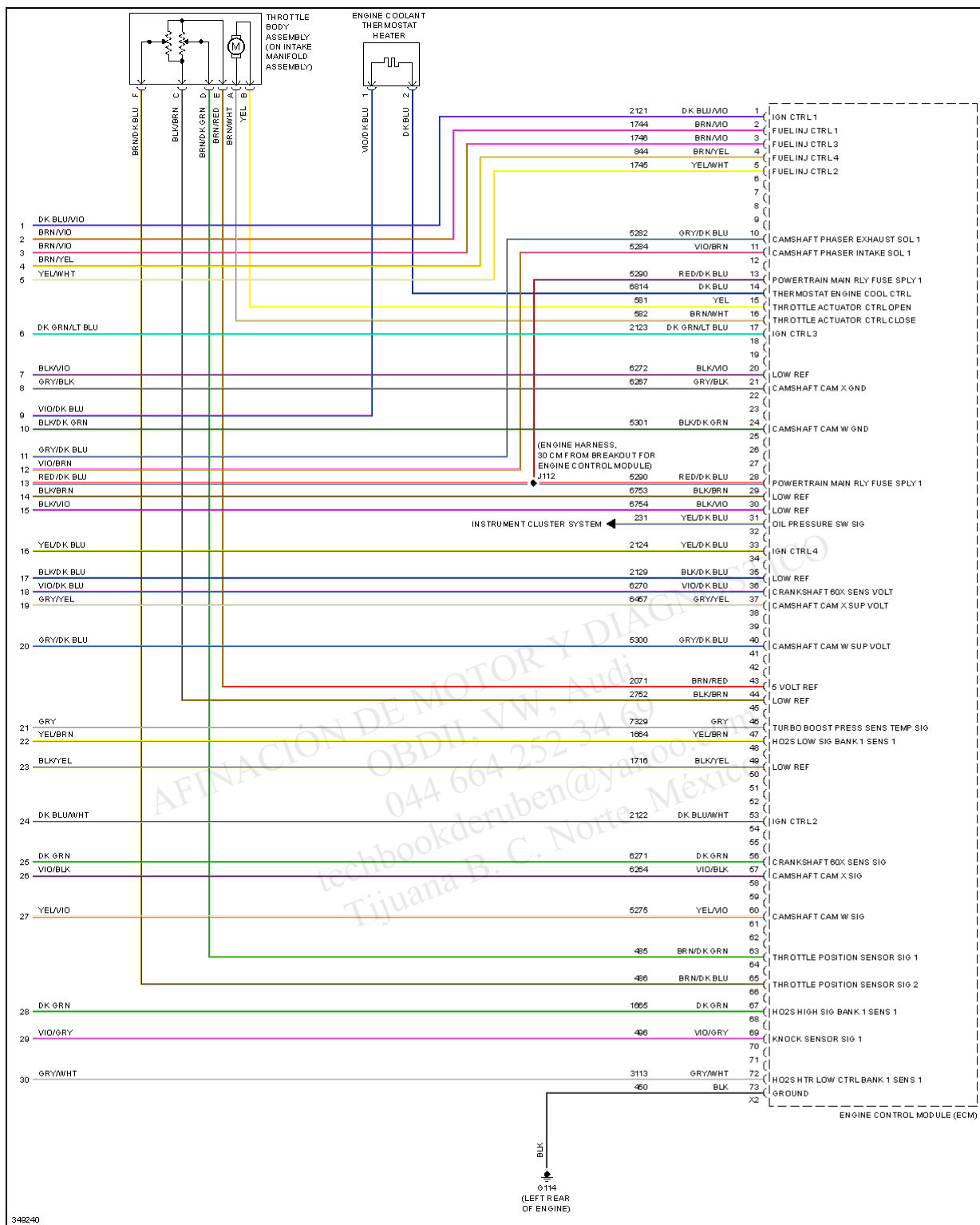
Fig. 23: 1.4L VIN 9, Engine Performance Circuit (6 of 6)
