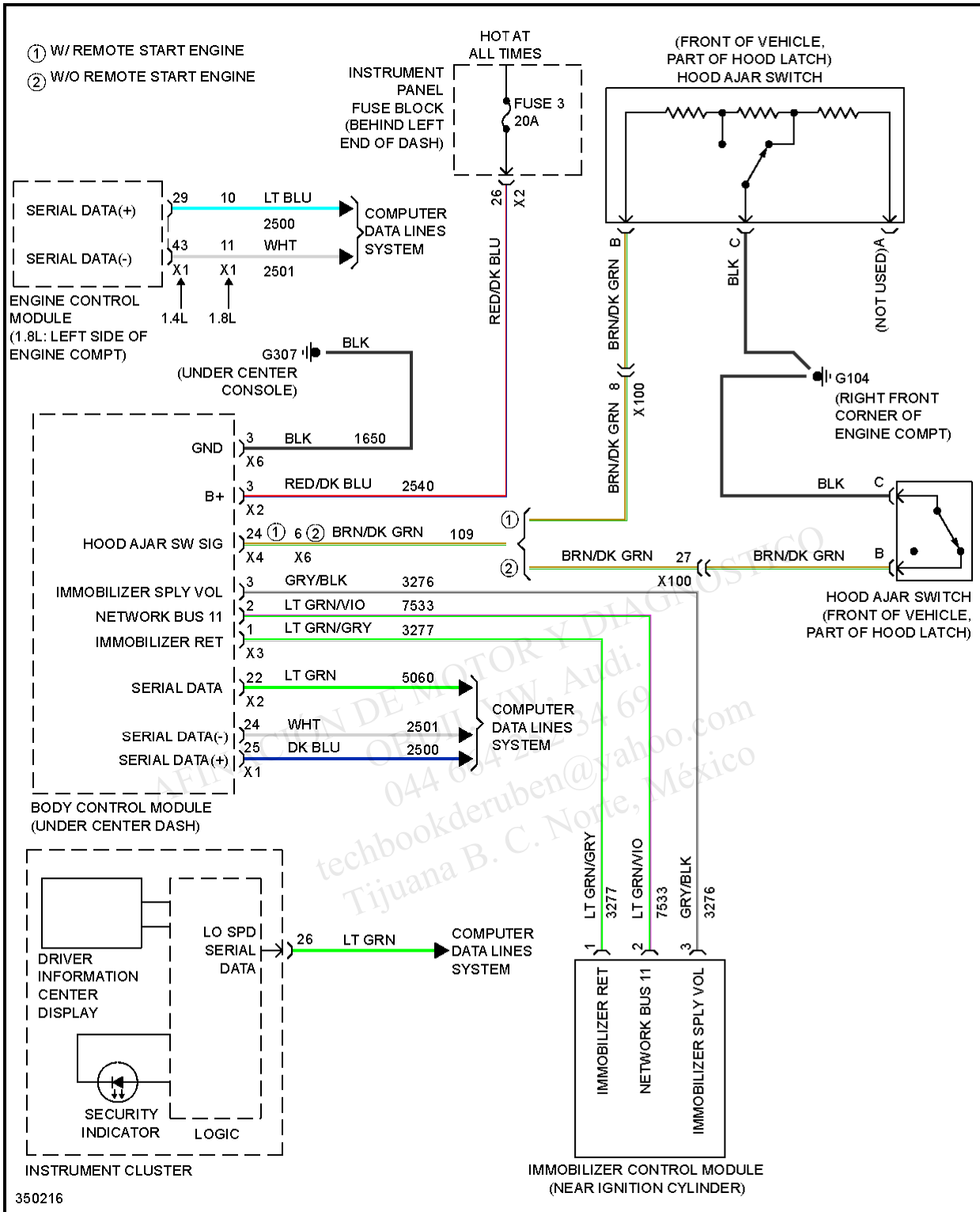
Fig. 9: Pass-Key Circuit
