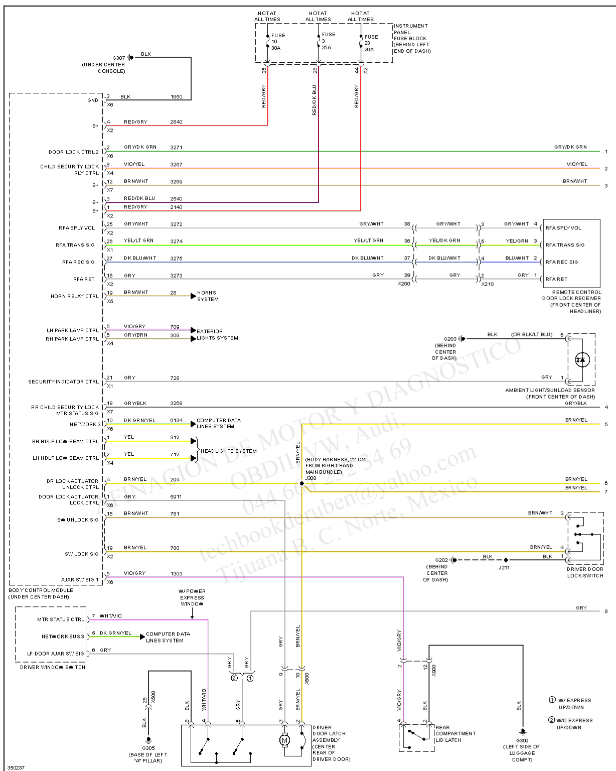
SYSTEM WIRING DIAGRAMS Fig. 7: Forced Entry Circuit (1 of 2)
