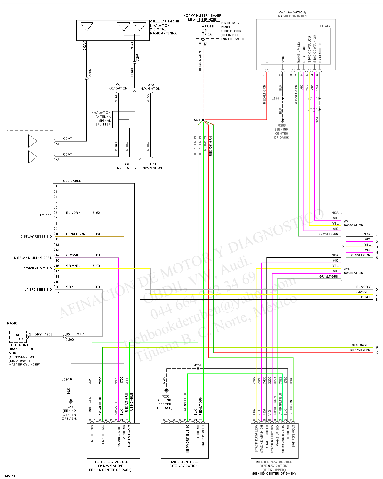
Fig. 60: Radio Circuit, W/ Amplifier (1 of 3)
