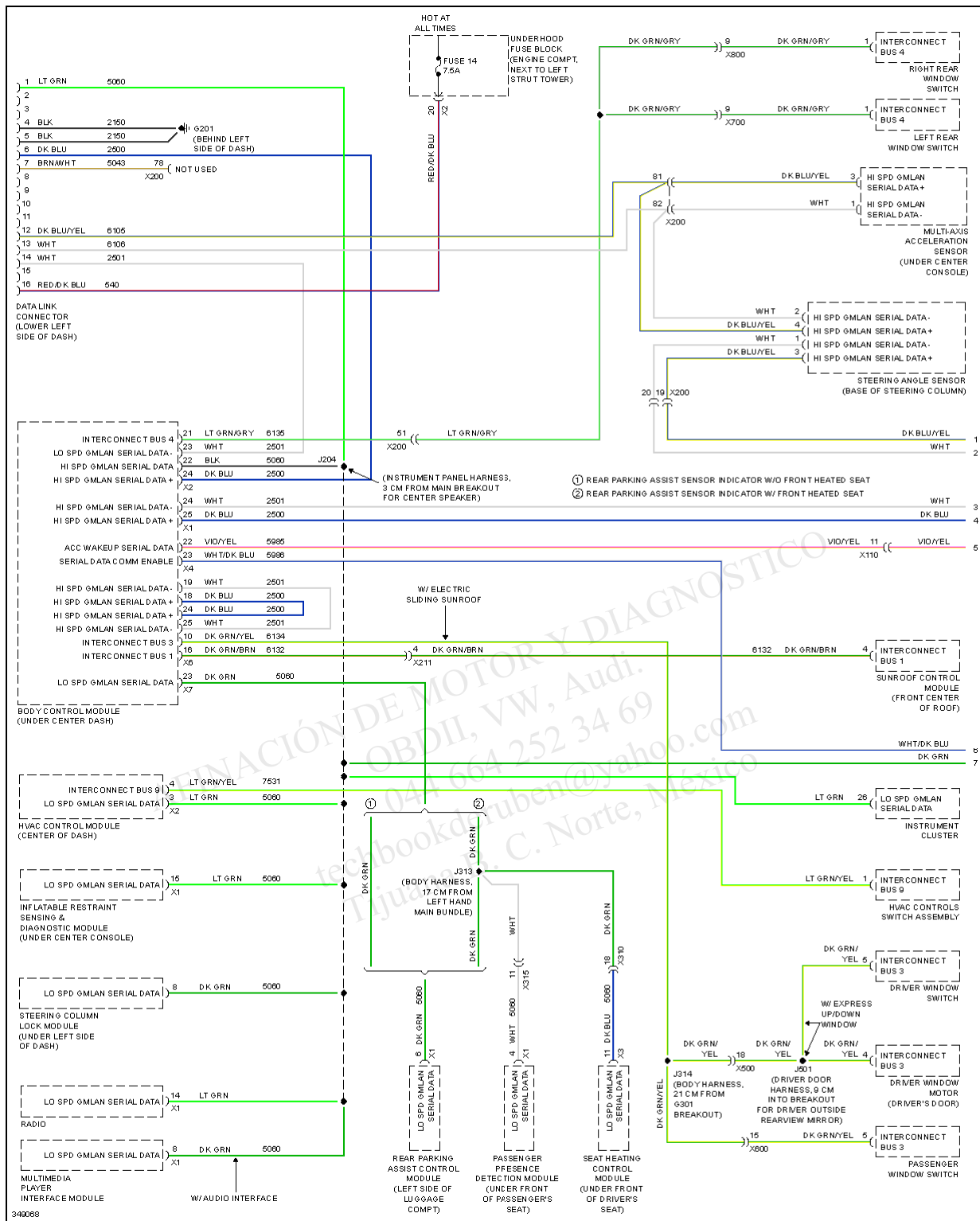
Fig. 12: Computer Data Lines Circuit (1 of 2)
