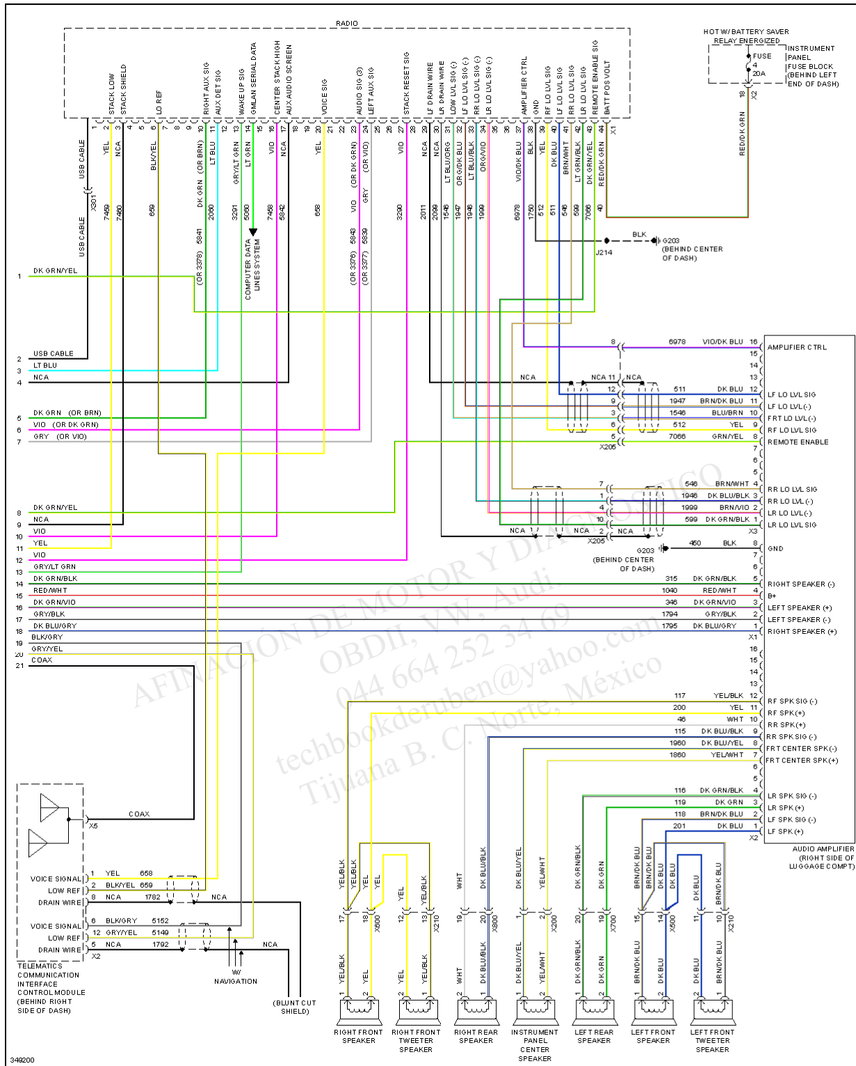
Fig. 42: Navigation Circuit, W/ Amplifier (3 of 3)
