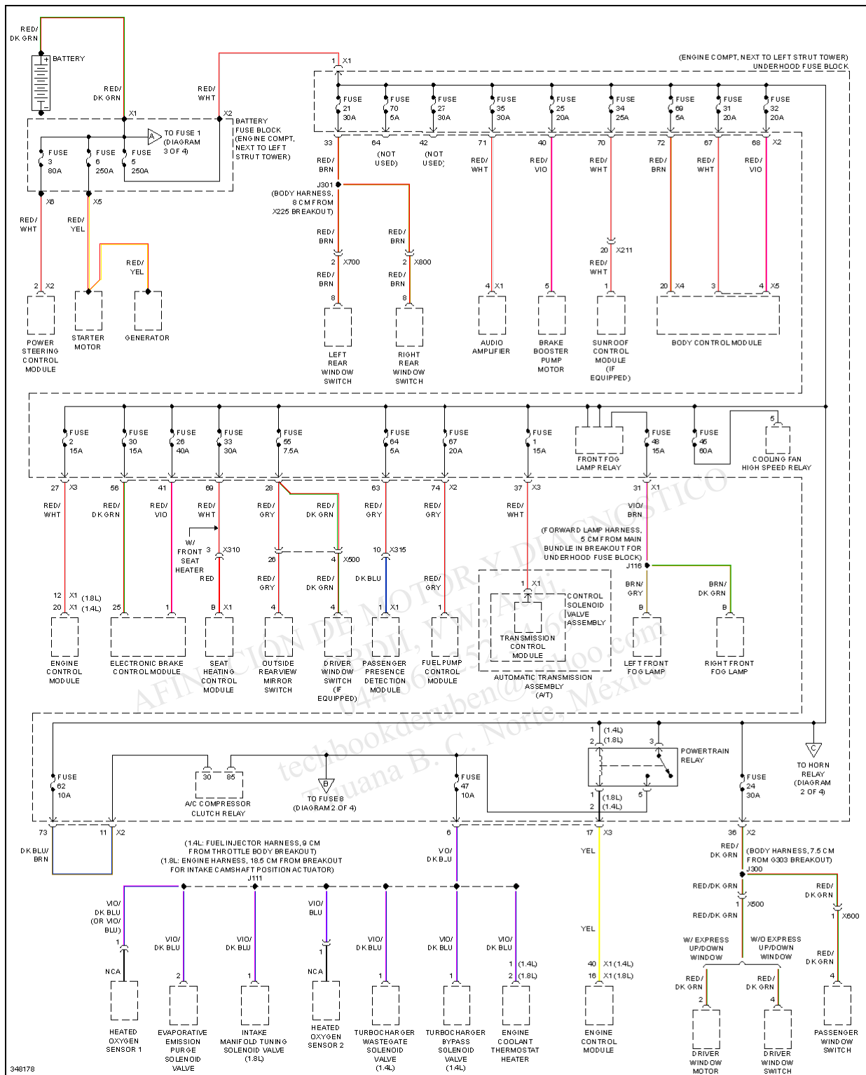
Fig. 47: Power Distribution Circuit (1 of 4)
