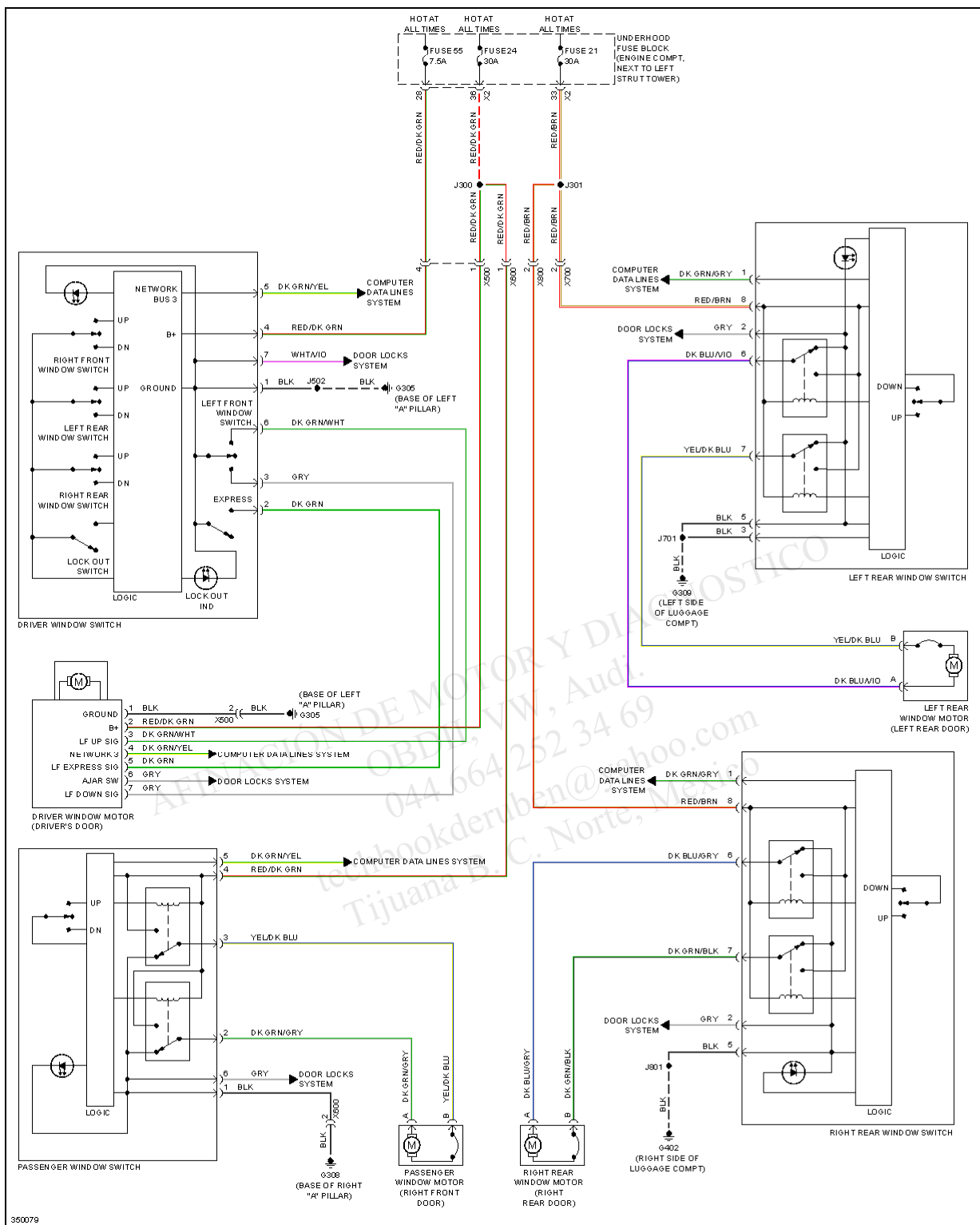
Fig. 58: Power Windows Circuit, W/ Express Up/Down
