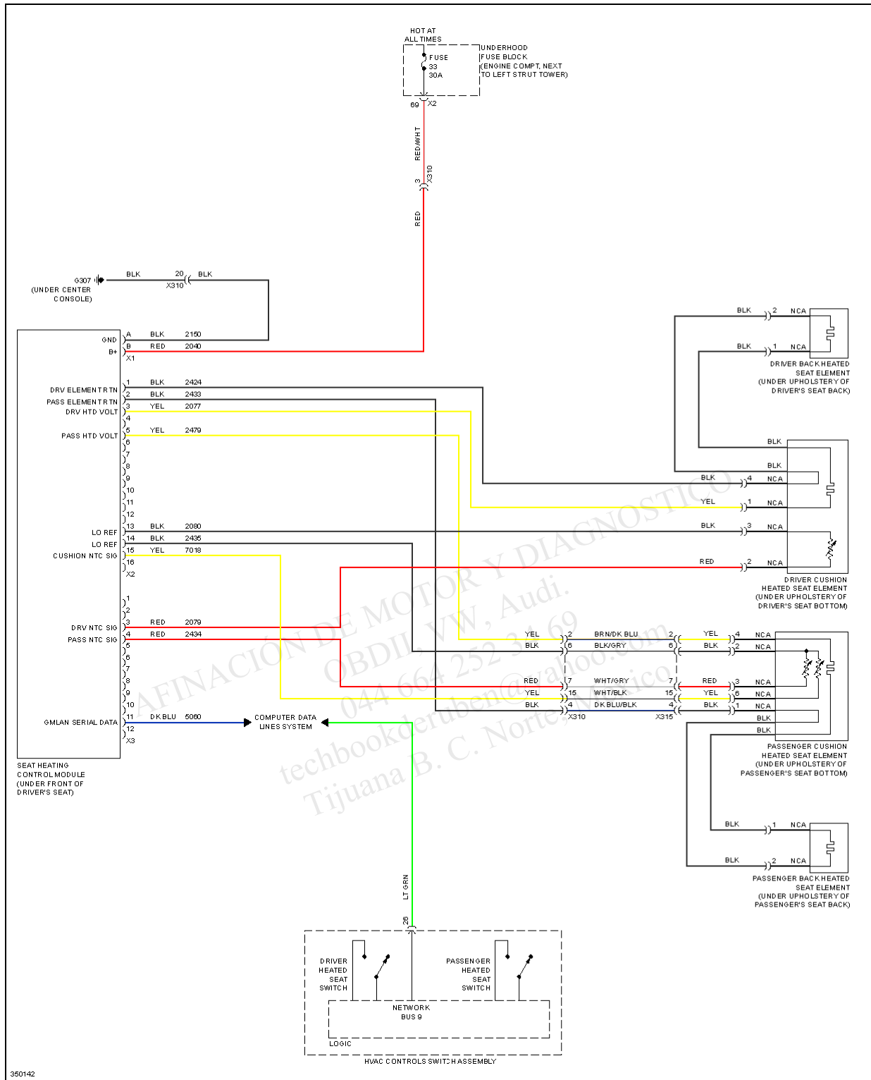
Fig. 56: Heated Seats Circuit
