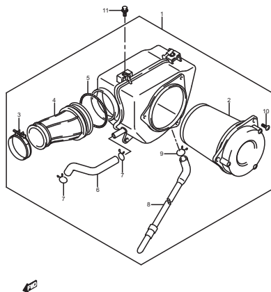
FIG.10 (B-11) AIR CLEANER
