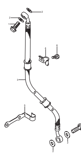
FIG.39 (G-2) FRONT BRAKE HOSE
