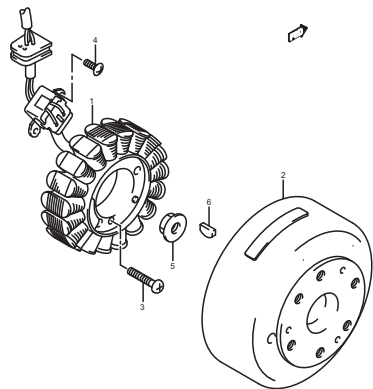
FIG.17 (D-2) MAGNETO
