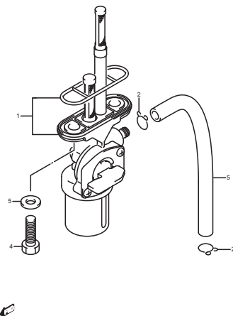
FIG.30 (E-7) FUEL COCK
