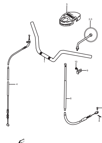
FIG.36 (F-6) HANDLE BAR CONTROL CABLE
