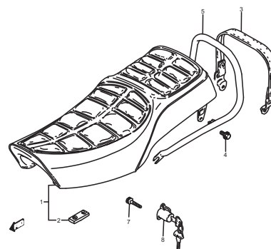
FIG.31 (E-8) SEAT
