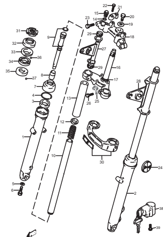
FIG.33 (F-3) FRONT FORK
