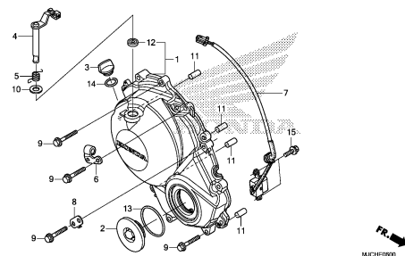
GENERATOR COVER
