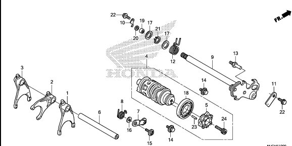
GEARSHIFT DRUM
