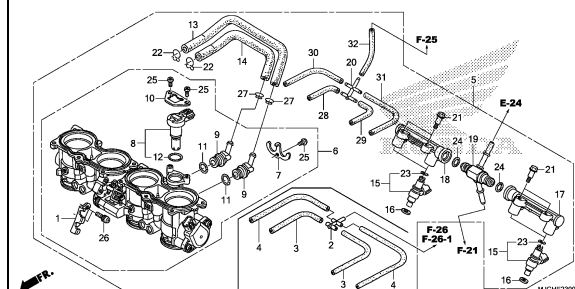
THROTTLE BODY
