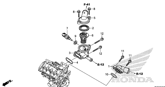
THERMOSTAT
