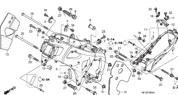
C-29 Chassi
