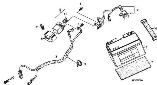
C-29 Chassi
