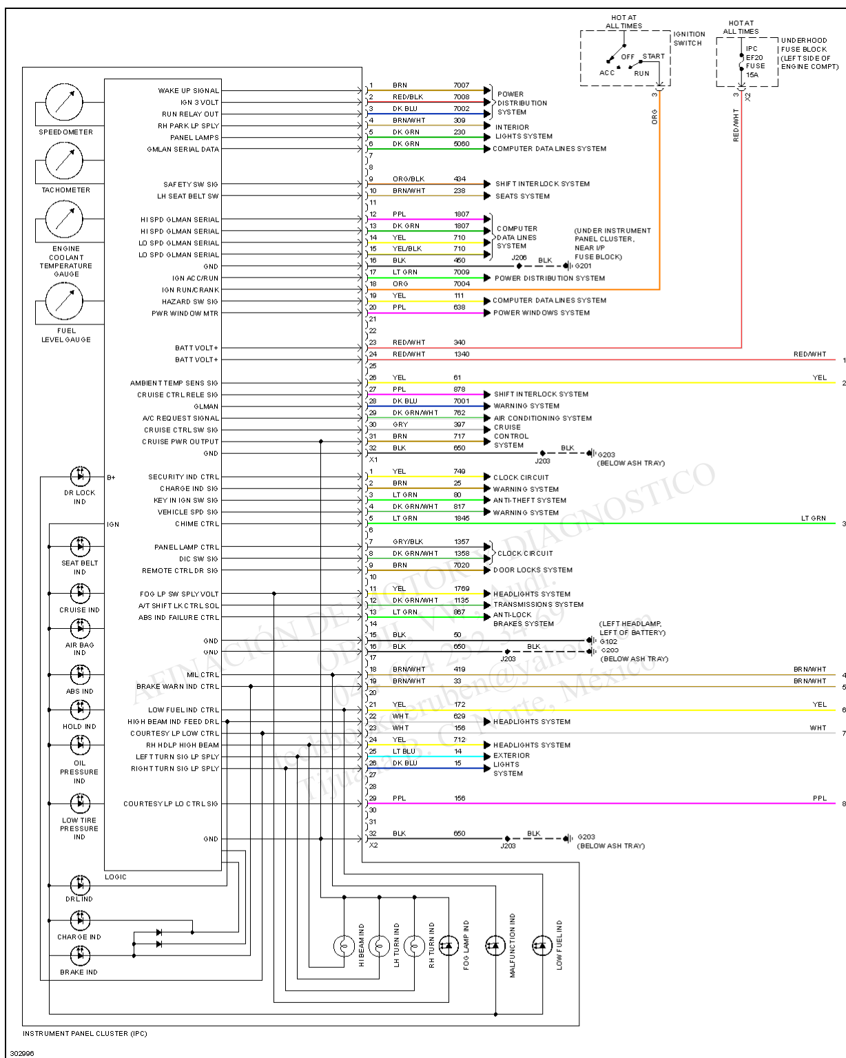
Fig. 30: Instrument Cluster Circuit (1 of 2)
