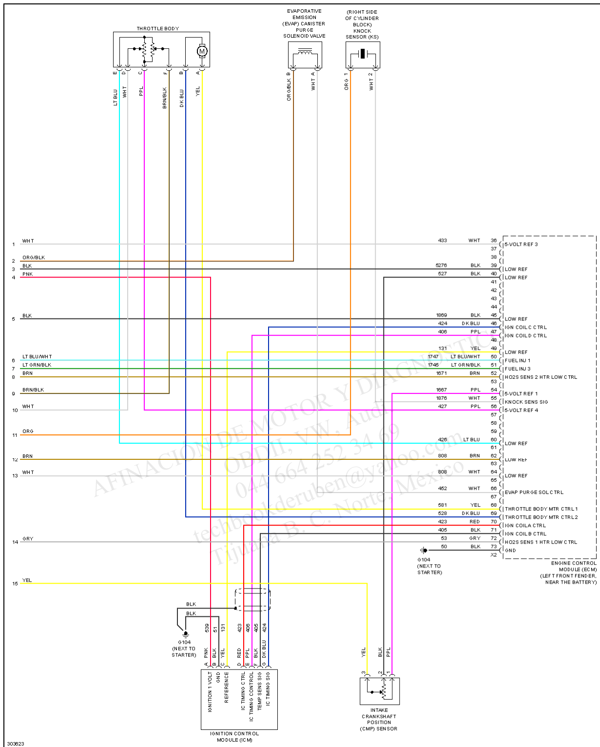
Fig. 18: 1.6L VIN E, Engine Performance Circuit (4 of 4)
