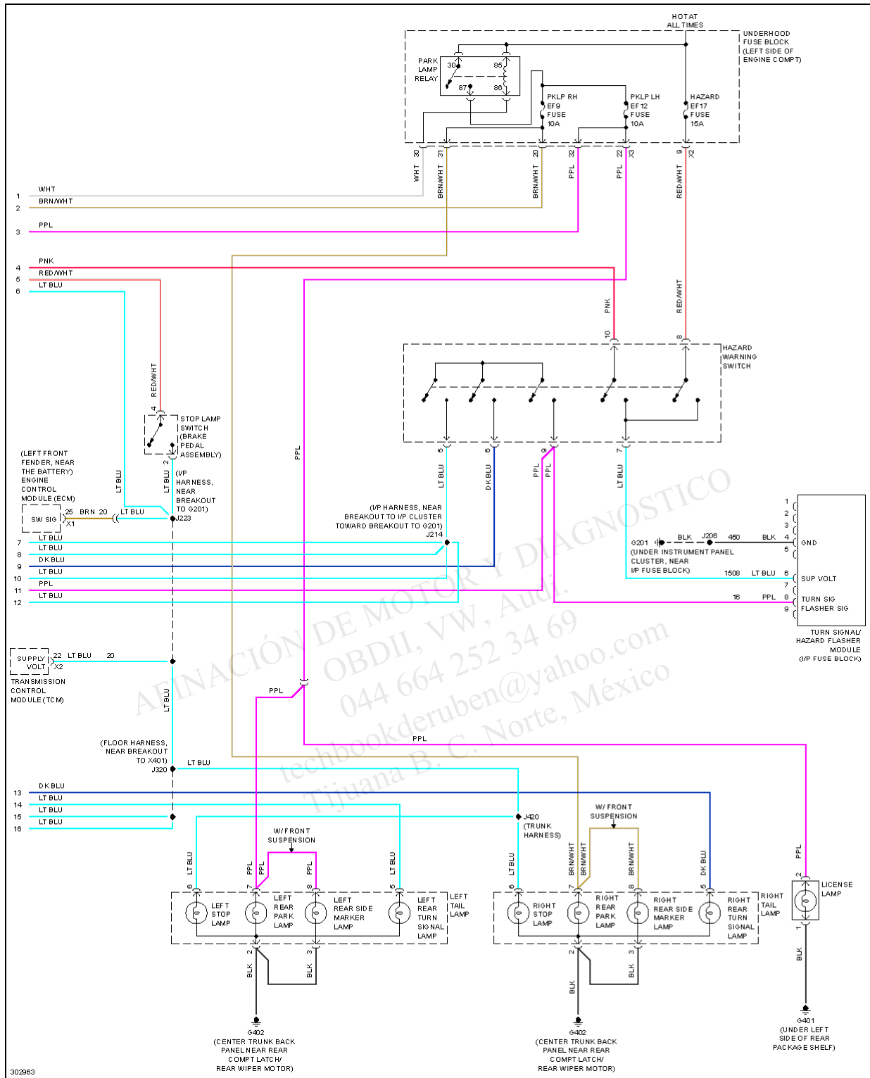
Fig. 24: Exterior Lamps Circuit, Notchback (2 of 2)
