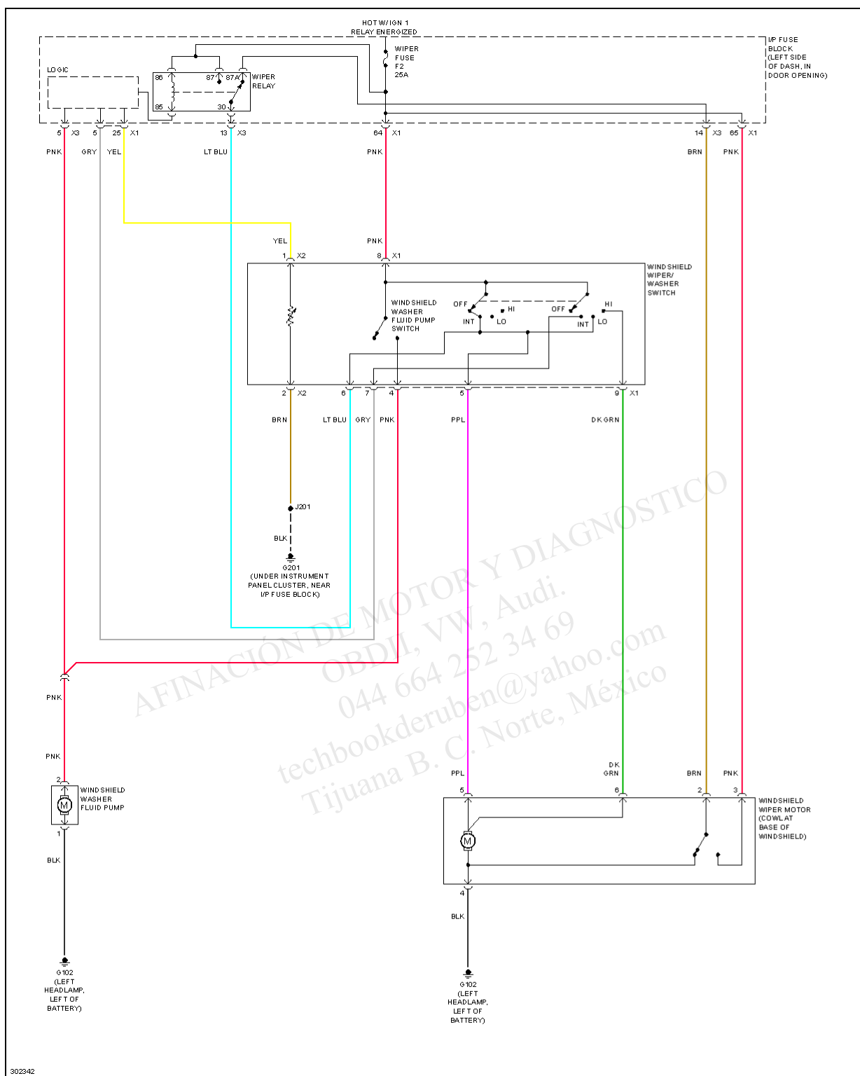
Fig. 56: Wiper/Washer Circuit, Notchback
