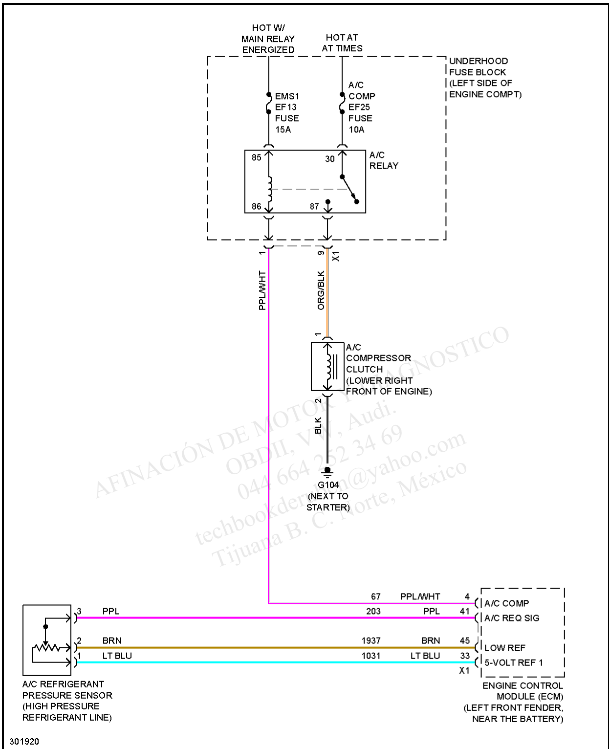
Fig. 3: Compressor Circuit, W/ Auto A/C
