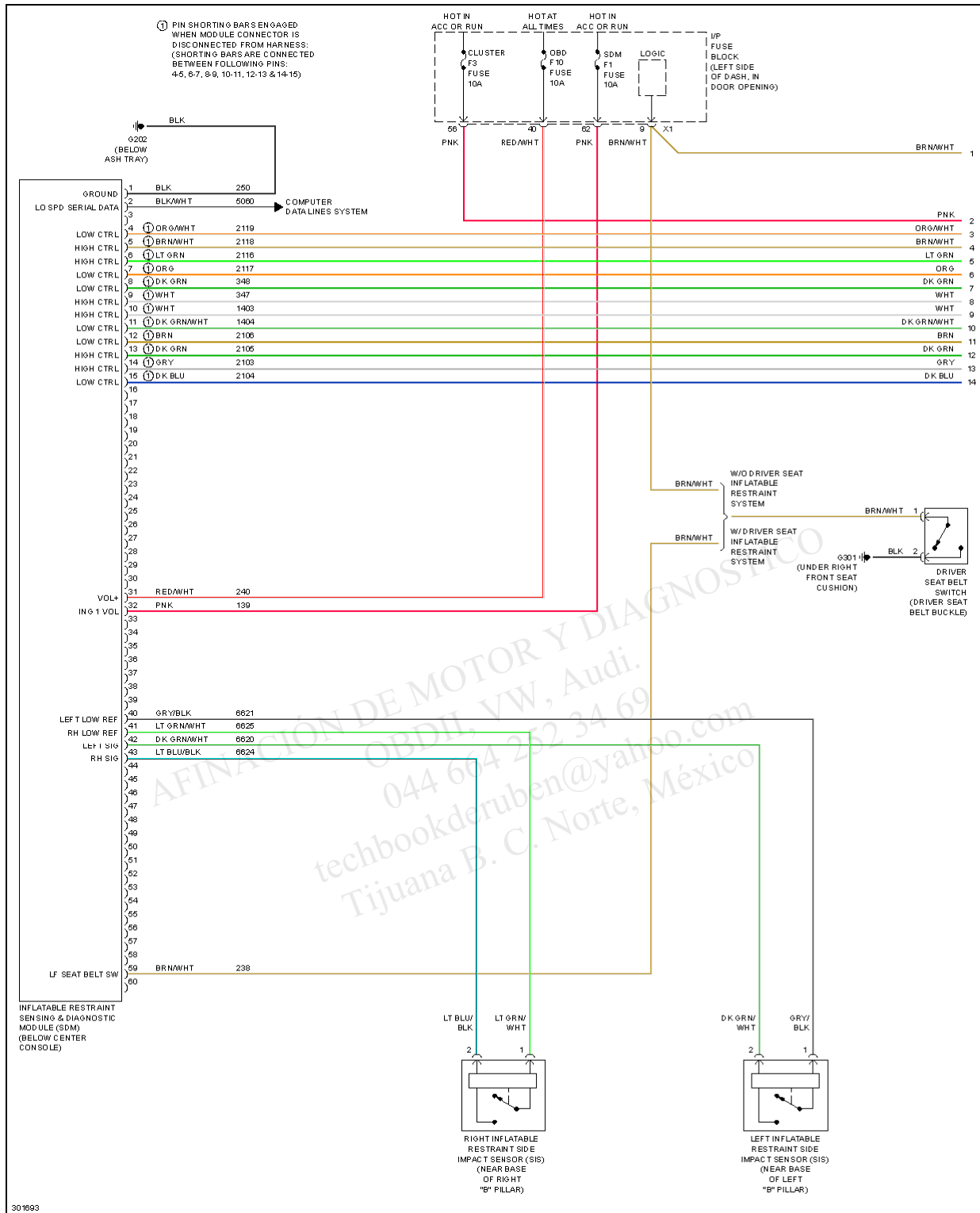
Fig. 49: Supplemental Restraints Circuit, W/O Restraint Suppression (1 of 2)
