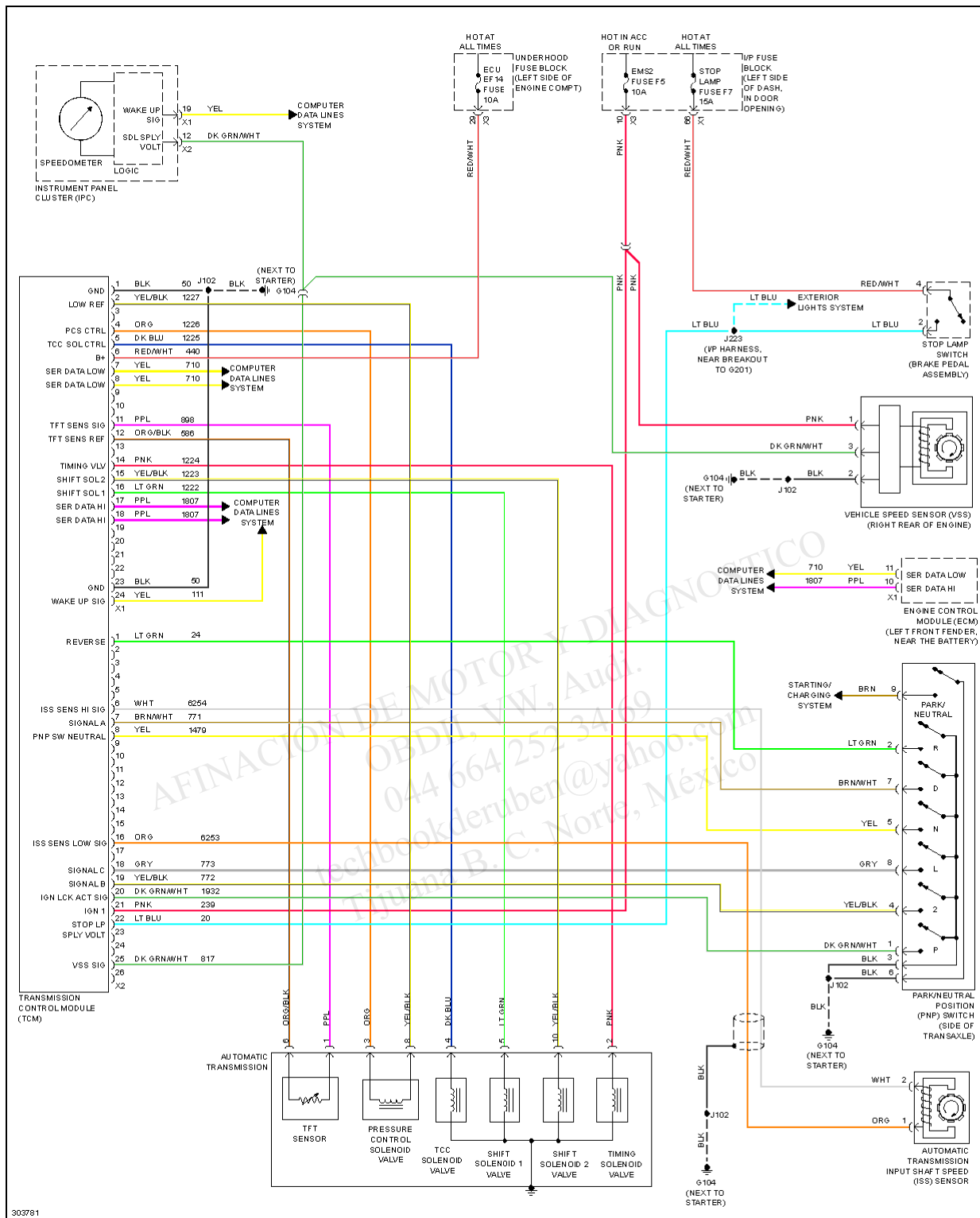
Fig. 51: Transmission Circuit
