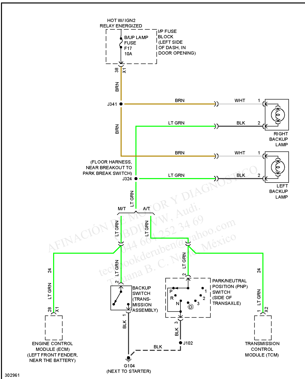
Fig. 19: Backup Lamps Circuit, Hatchback
