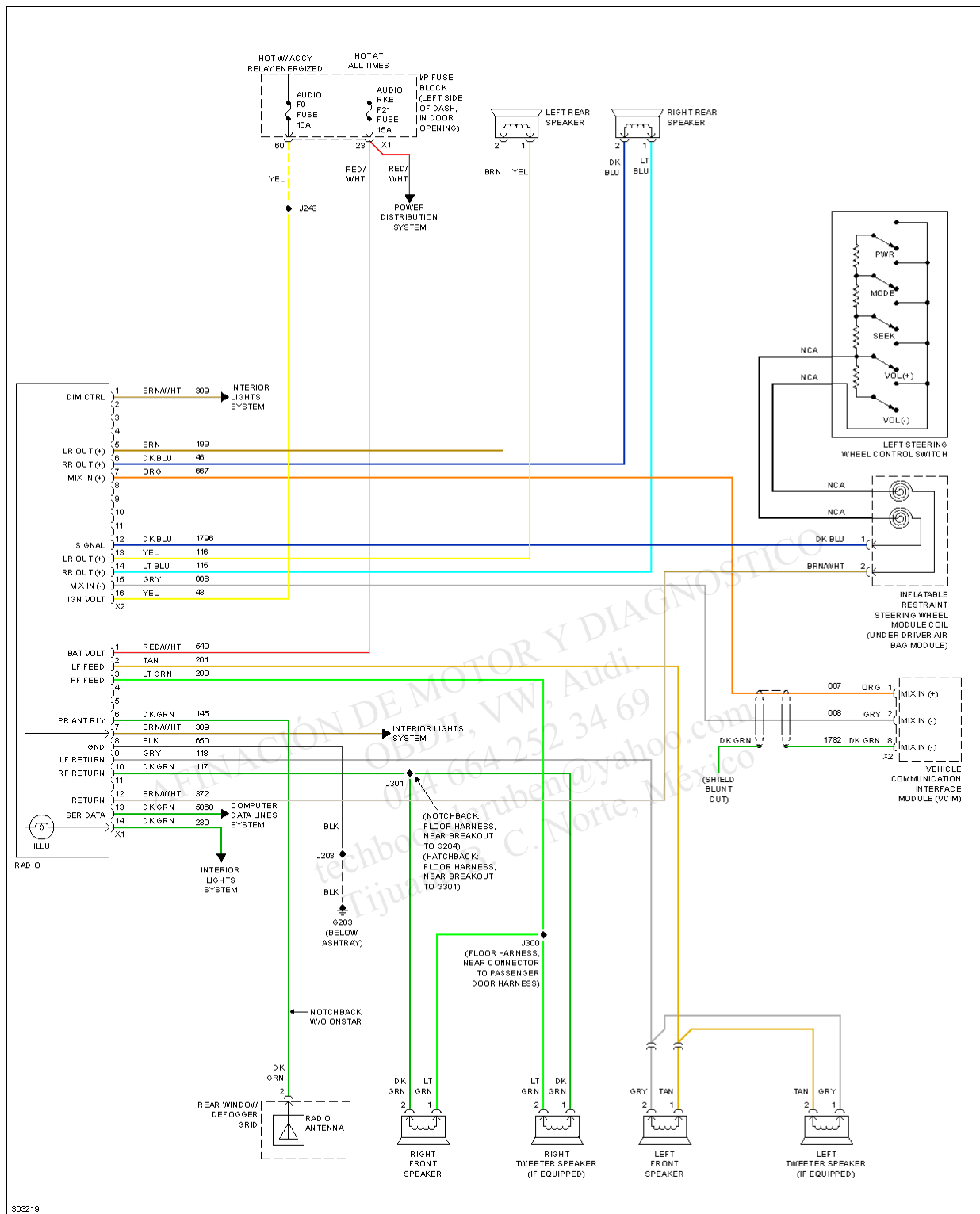
Fig. 43: Radio Circuit
