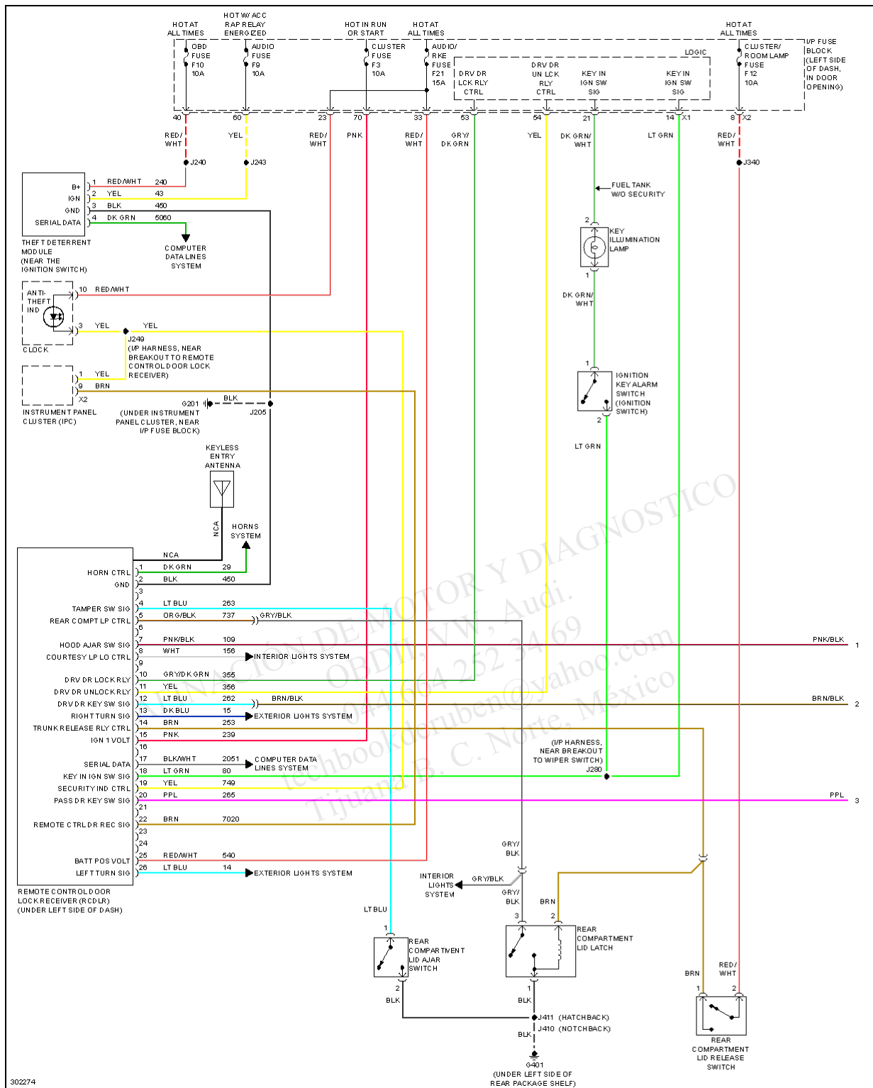
Fig. 38: Power Door Locks Circuit (1 of 2)
