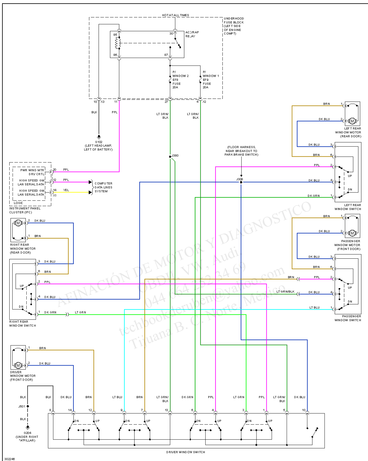
Fig. 42: Power Windows Circuit
