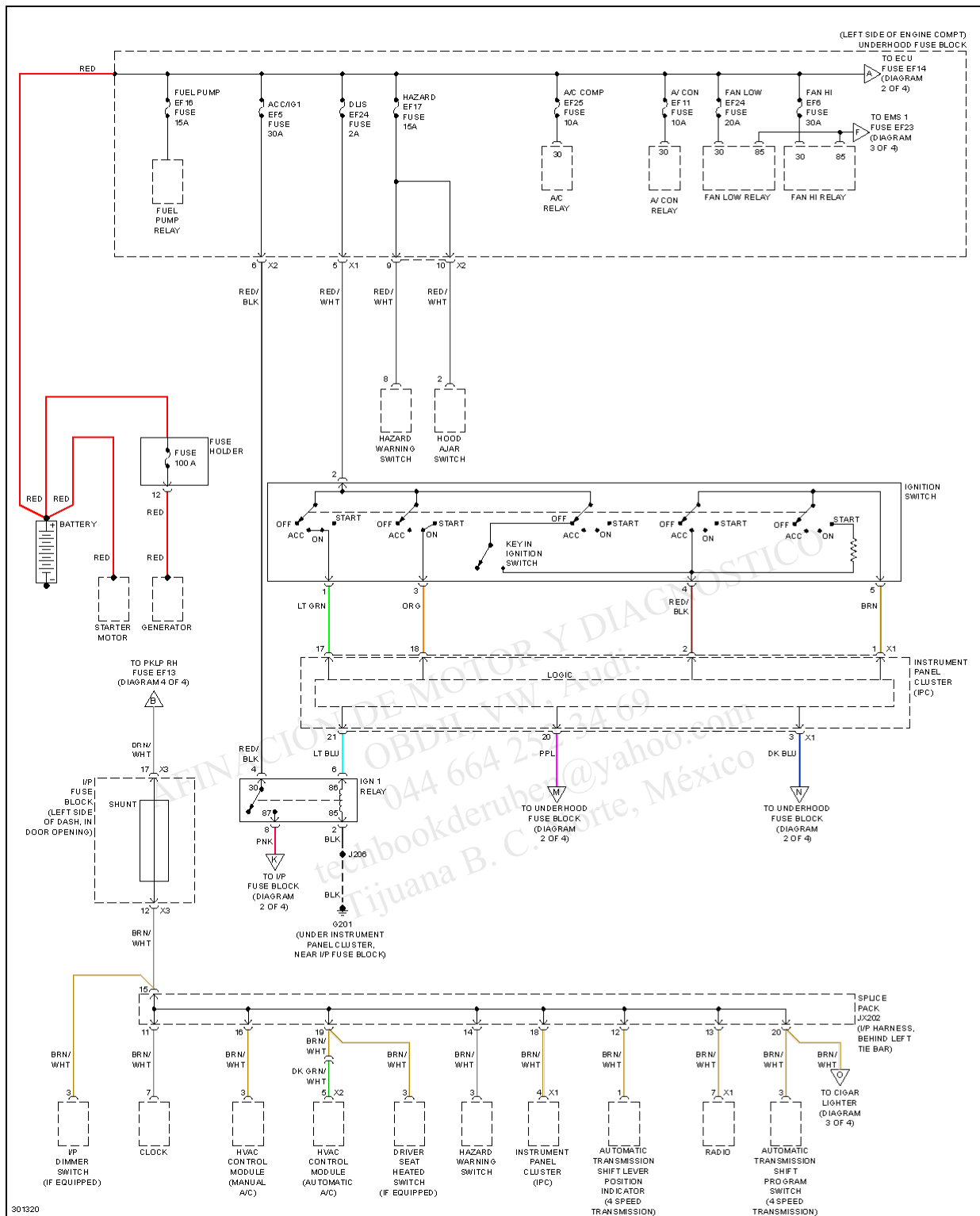
Fig. 34: Power Distribution Circuit (1 of 4)
