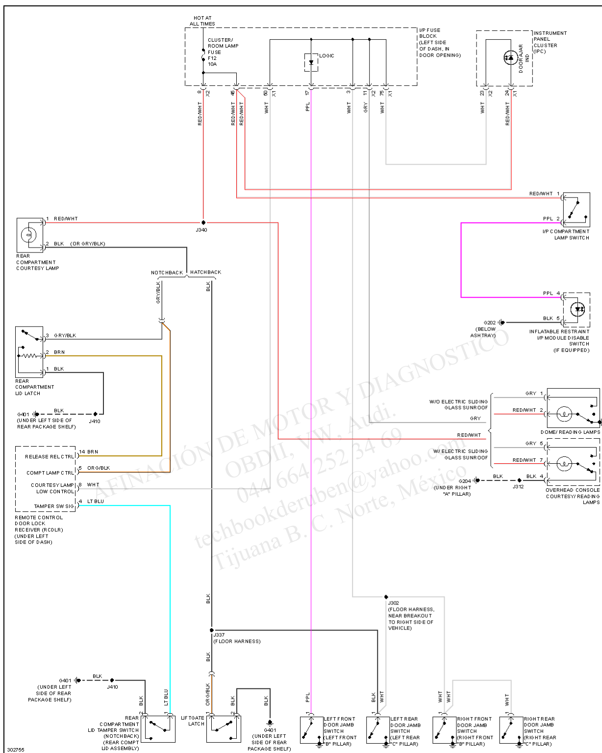
SYSTEM WIRING DIAGRAMS Fig. 32: Courtesy Lamps Circuit
