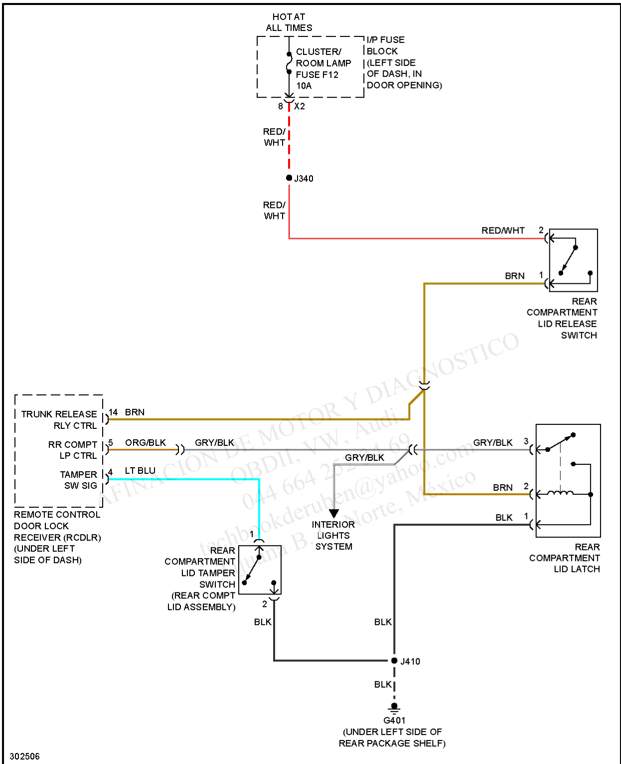
Fig. 52: Trunk Release Circuit
