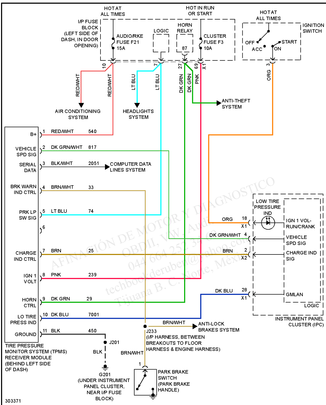
Fig. 54: Tire Pressure Monitoring Circuit
