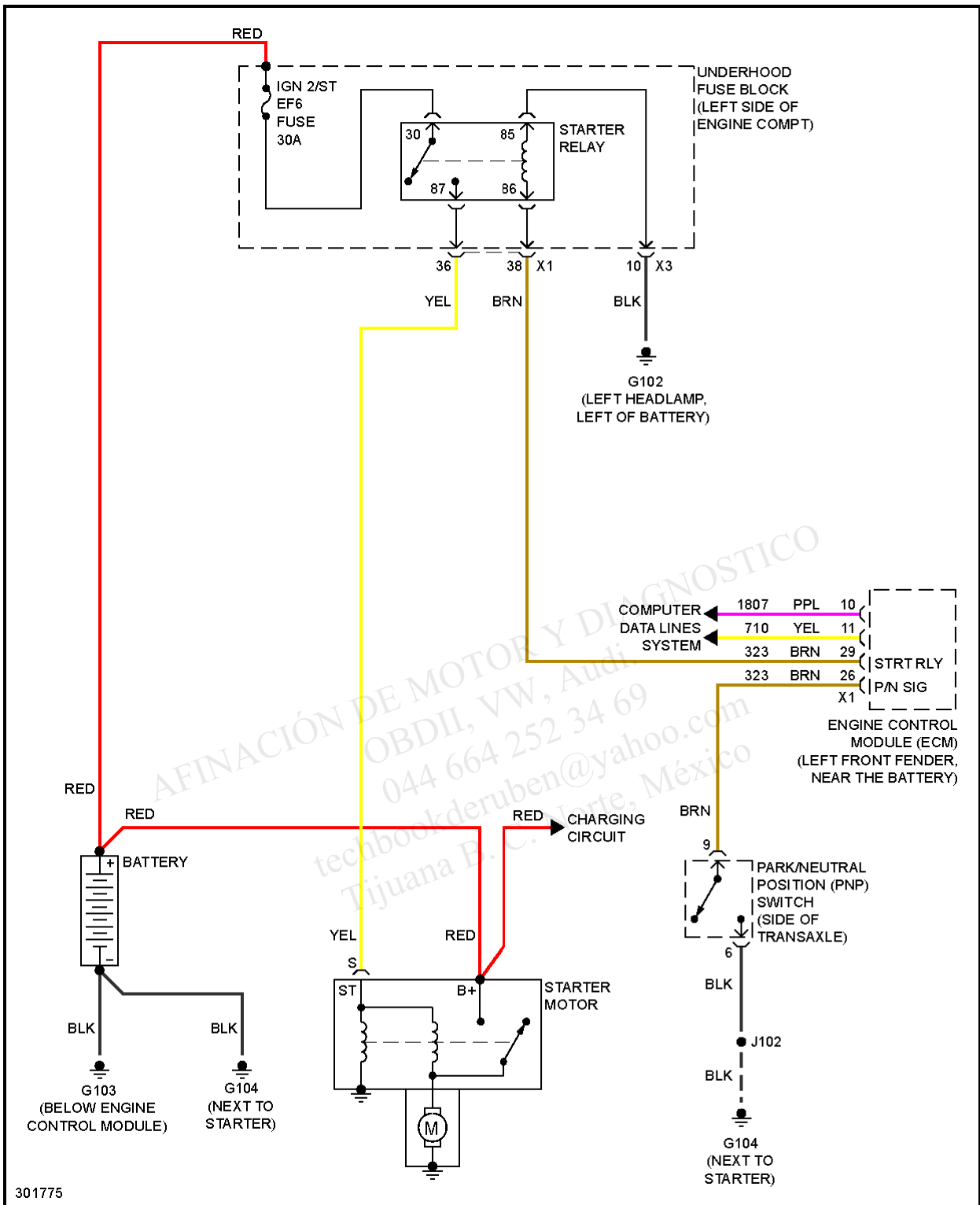
Fig. 46: Starting Circuit
