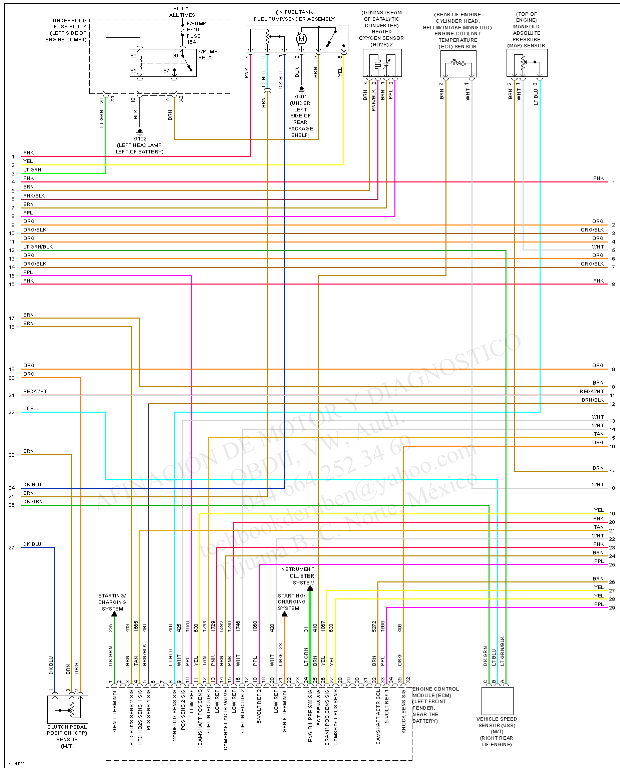
Fig. 16: 1.6L VIN E, Engine Performance Circuit (2 of 4)
