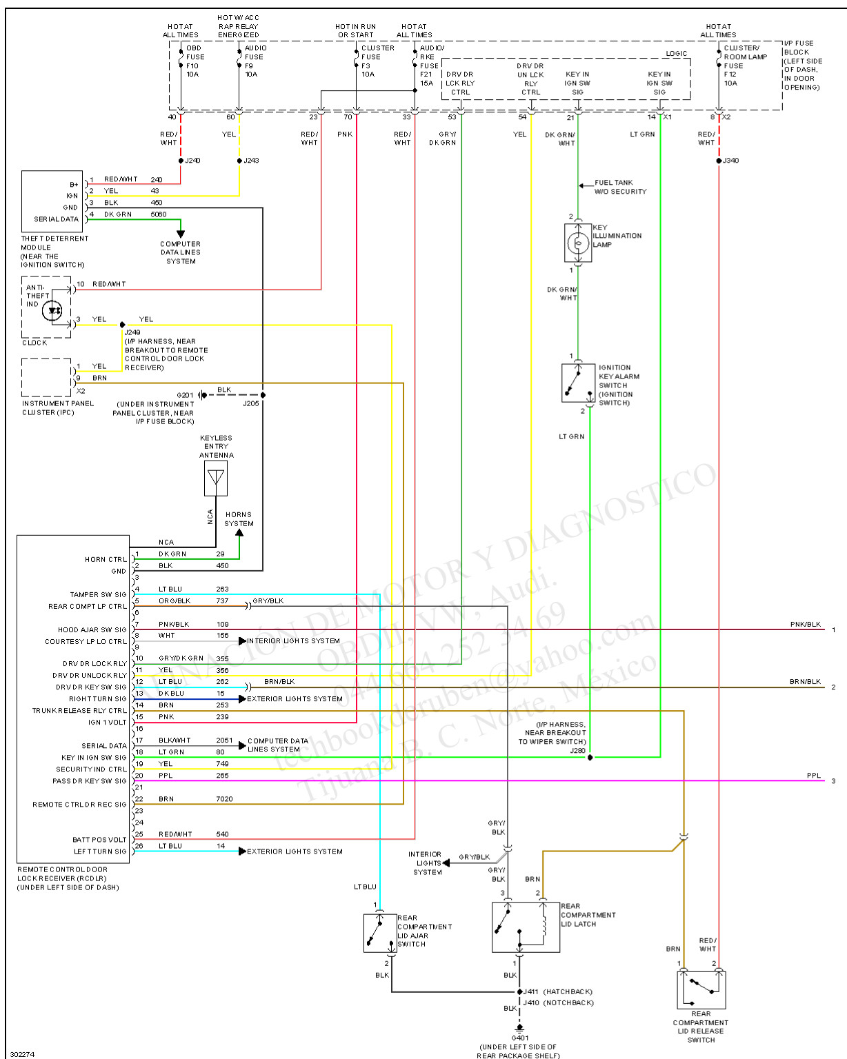
Fig. 9: Anti-theft Circuit (1 of 2)
