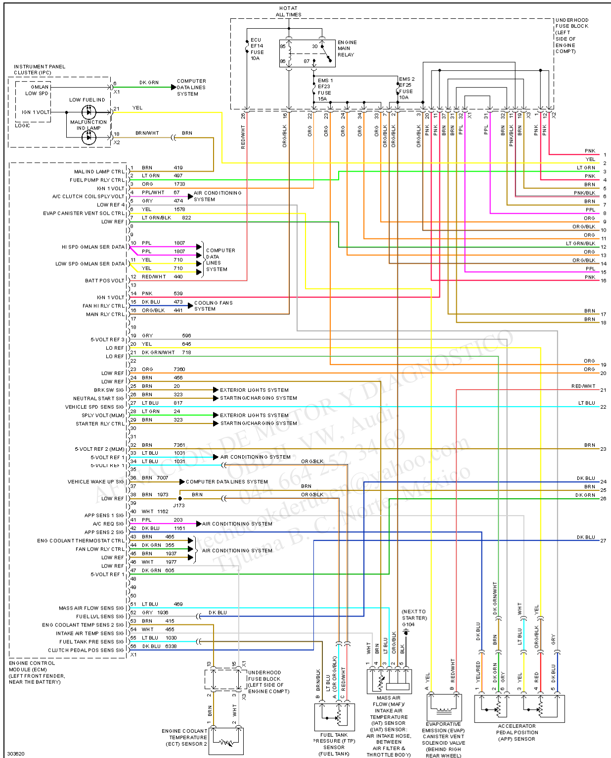
Fig. 15: 1.6L VIN E, Engine Performance Circuit (1 of 4)
