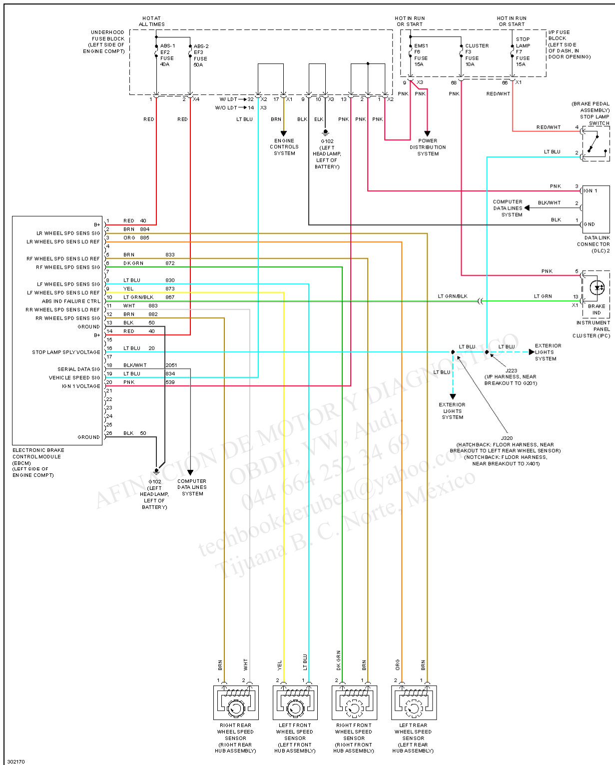
Fig. 8: Anti-lock Brakes Circuit
