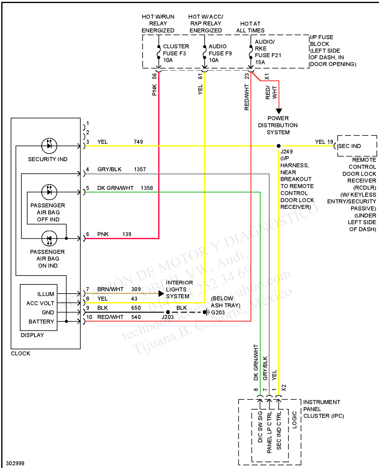
Fig. 29: Clock Circuit
