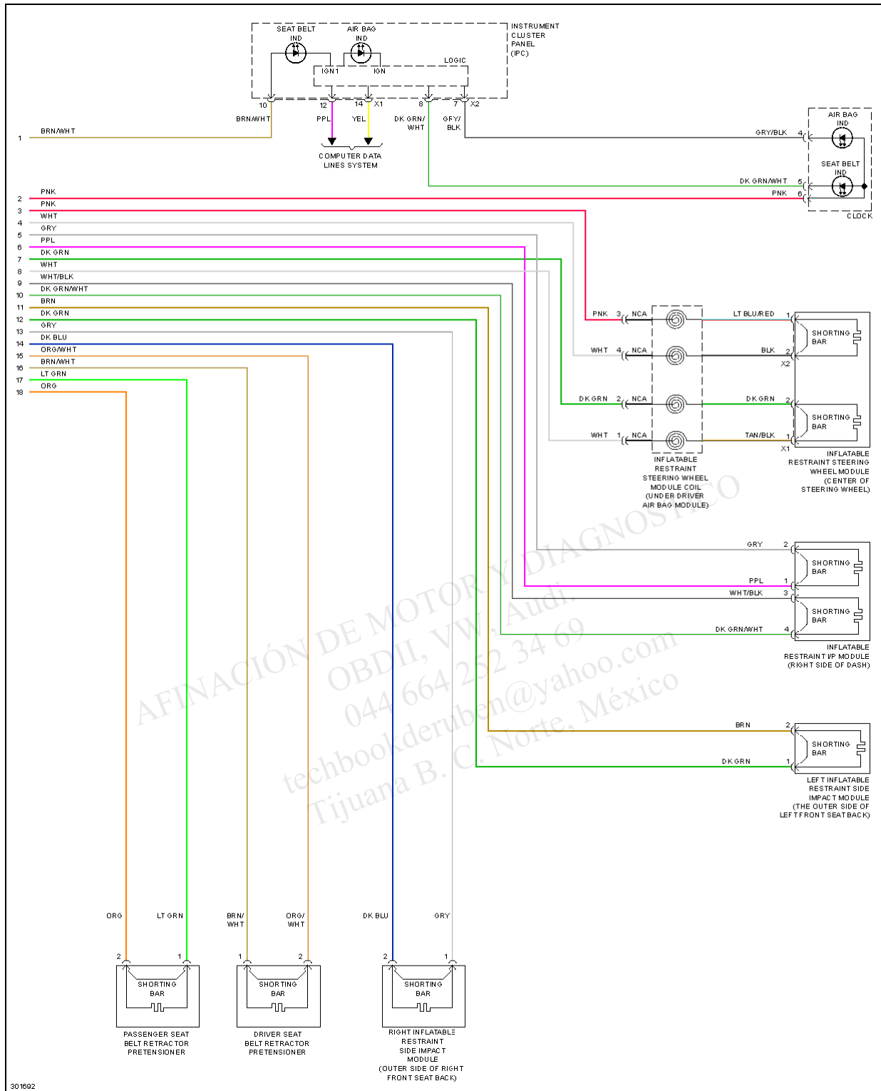
Fig. 48: Supplemental Restraints Circuit, W/ Restraint Suppression (2 of 2)
