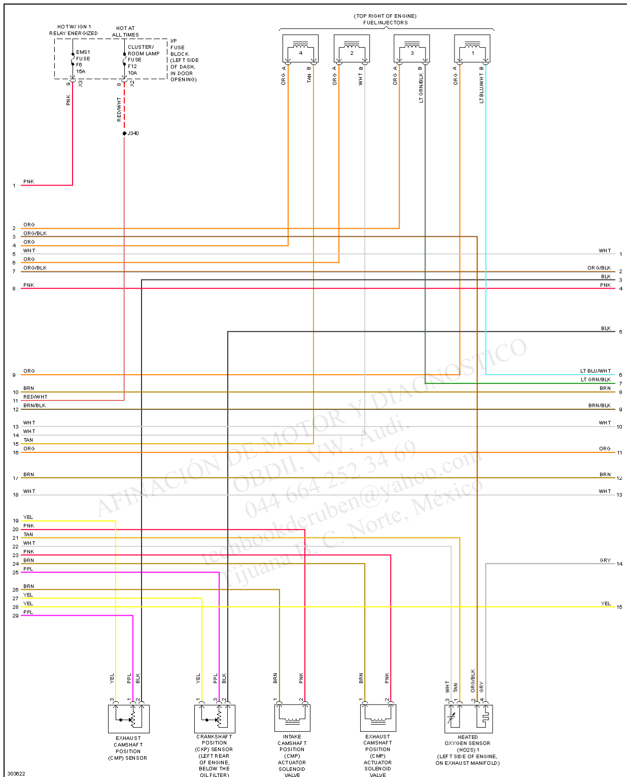
Fig. 17: 1.6L VIN E, Engine Performance Circuit (3 of 4)
