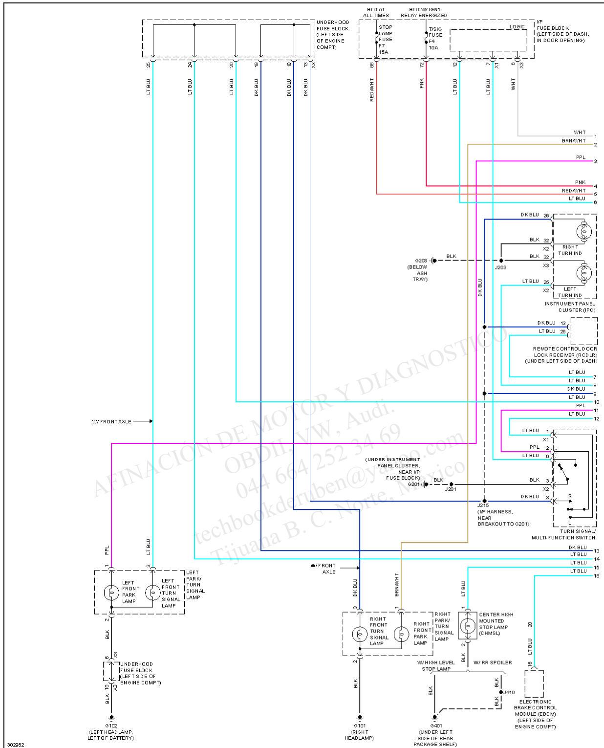
Fig. 23: Exterior Lamps Circuit, Notchback (1 of 2)
