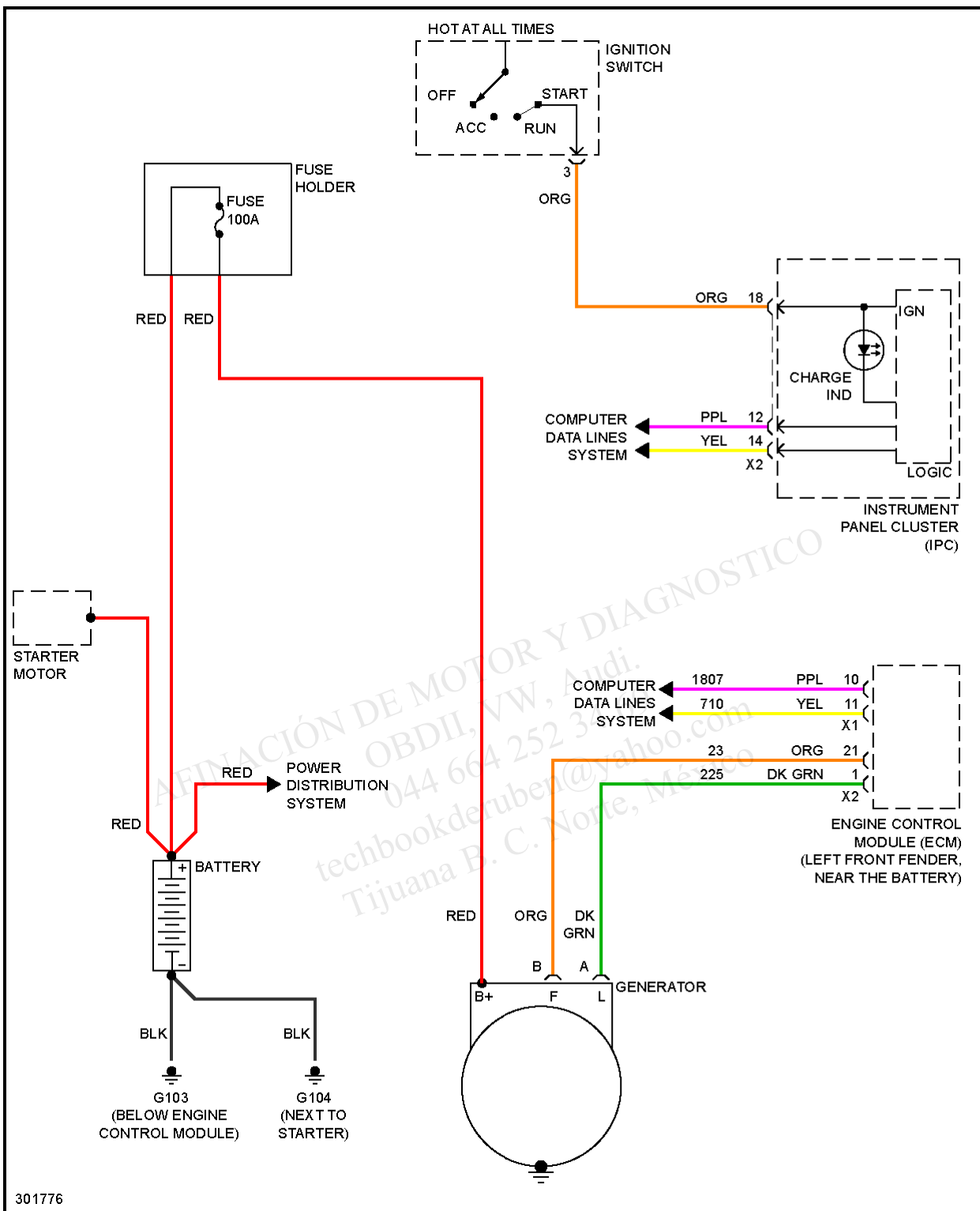
Fig. 45: Charging Circuit
