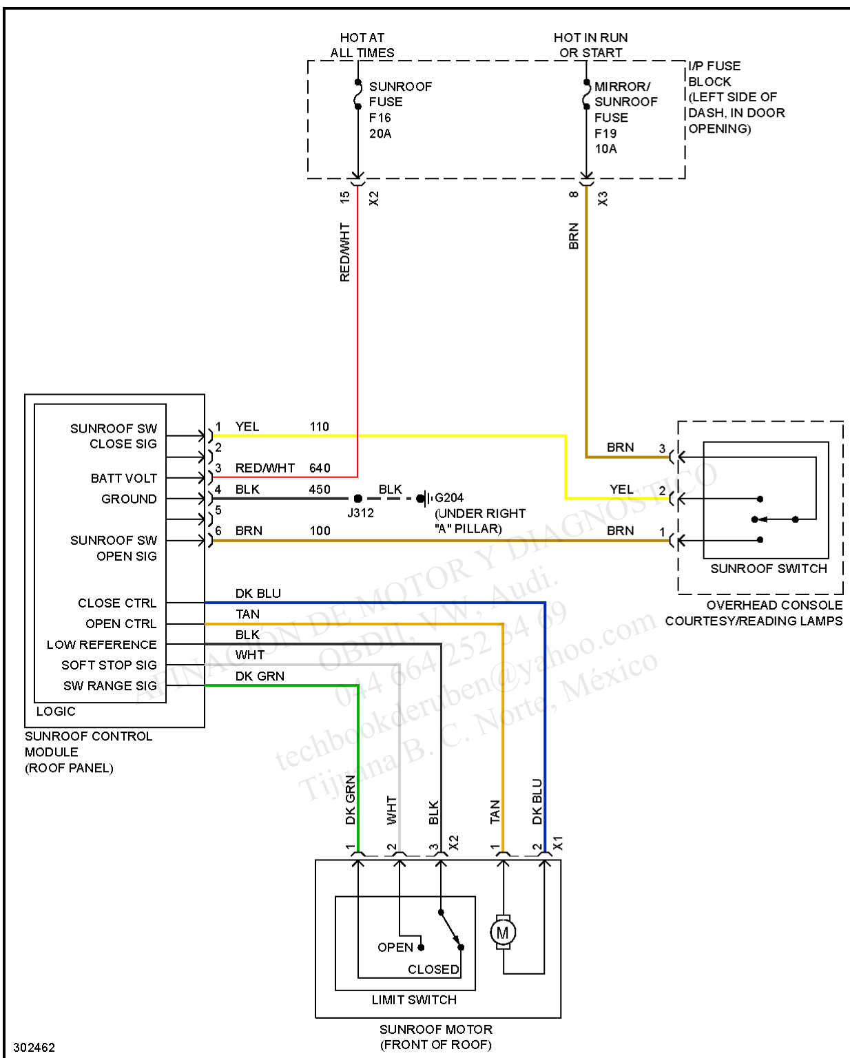
Fig. 41: Power Top/Sunroof Circuit
