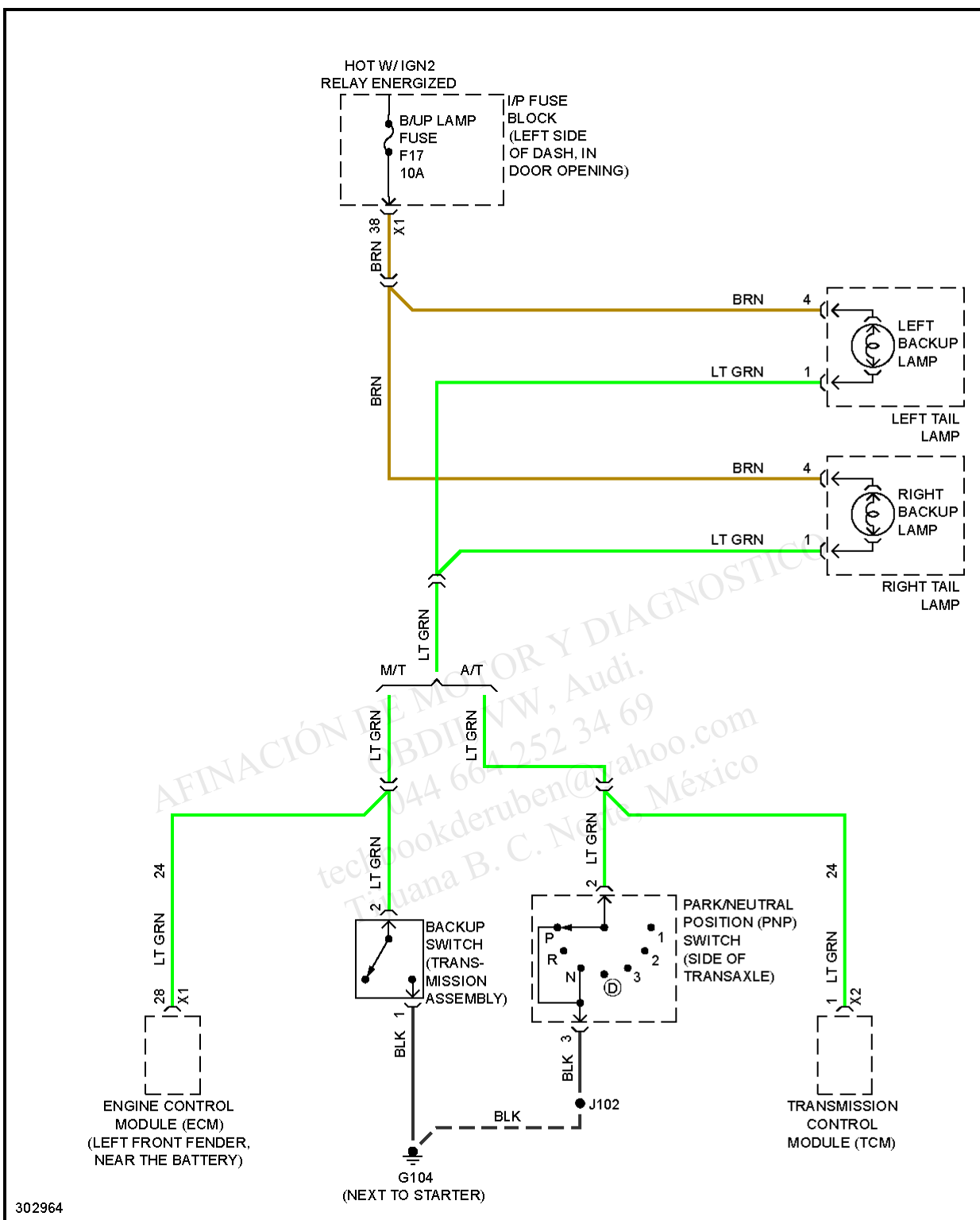
Fig. 20: Backup Lamps Circuit, Notchback
