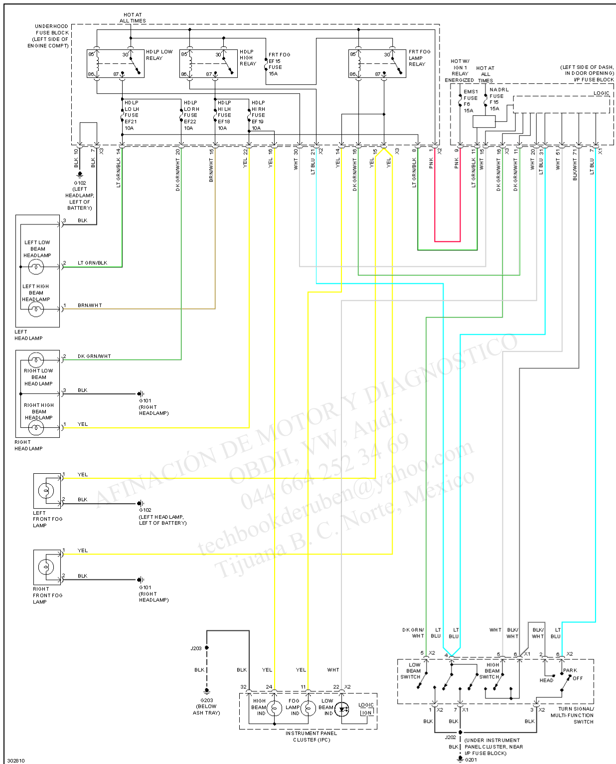
Fig. 27: Headlights Circuit
