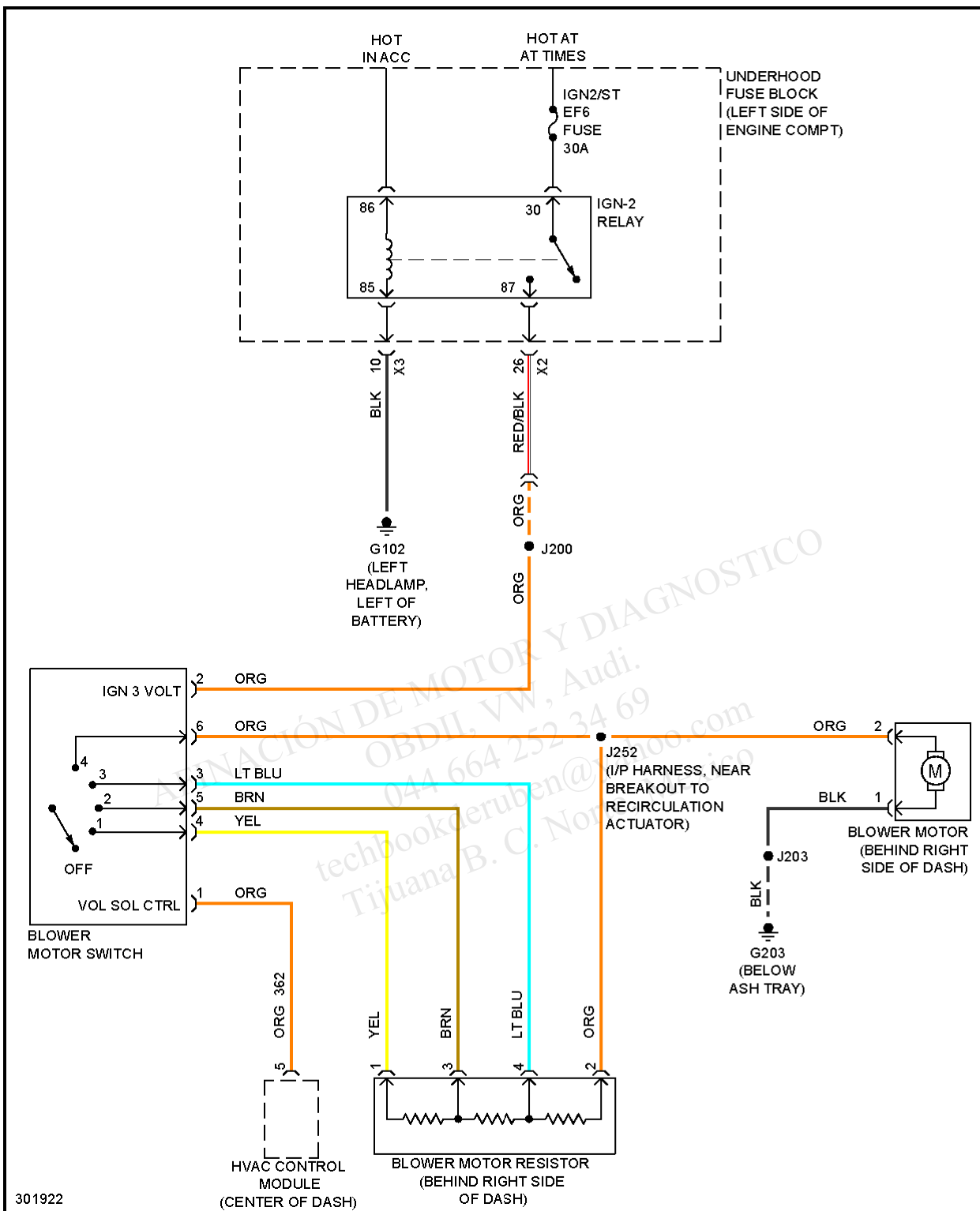
Fig. 5: Heater Circuit
