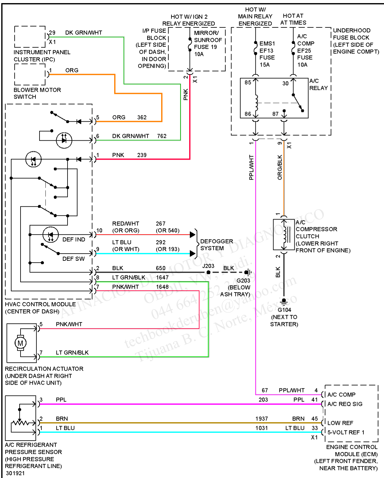
Fig. 4: Compressor Circuit, W/ Manual A/C
