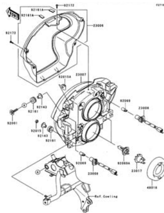
G-4 Headlight(s)
