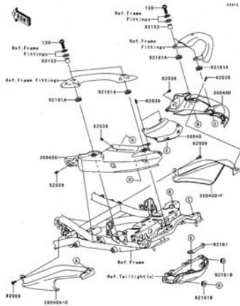
G-3 Seat Cover
