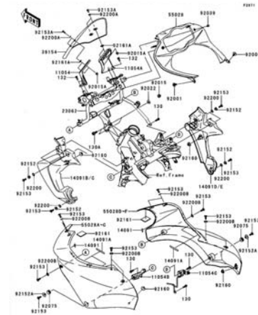
G-13 Cowling
