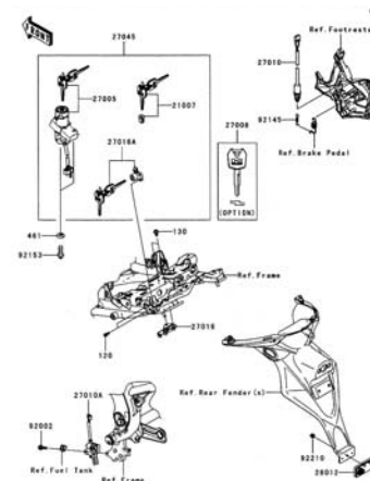
G-8 Ignition Switch
