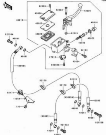
F-4 Front Master Cylinder
