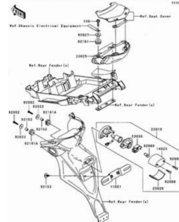
G-5 Taillight(s)
