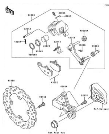
F-7 Rear Brake
