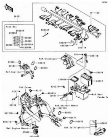
G-7 Chassis Electrical Equipment
