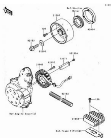
C-13 Generator
