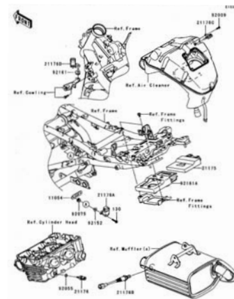
C-11 Fuel Injection
