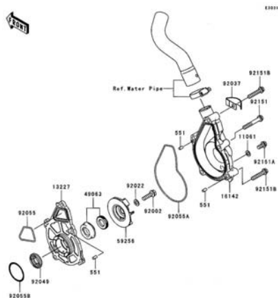
D-4 Water Pump
