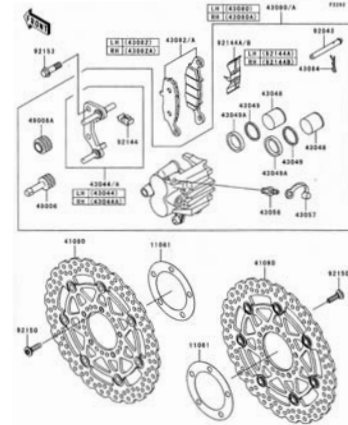
F-5 Front Brake
