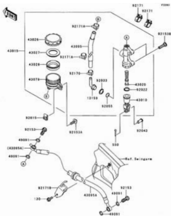
F-6 Rear Master Cylinder
