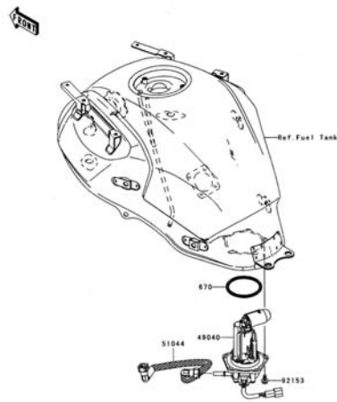
C-10 Fuel Pump
