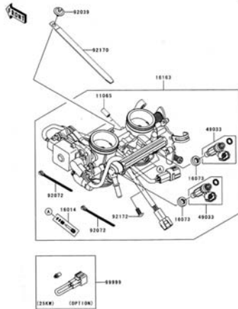
C-9 Throttle
