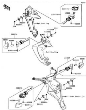
G-6 Turn Signals
